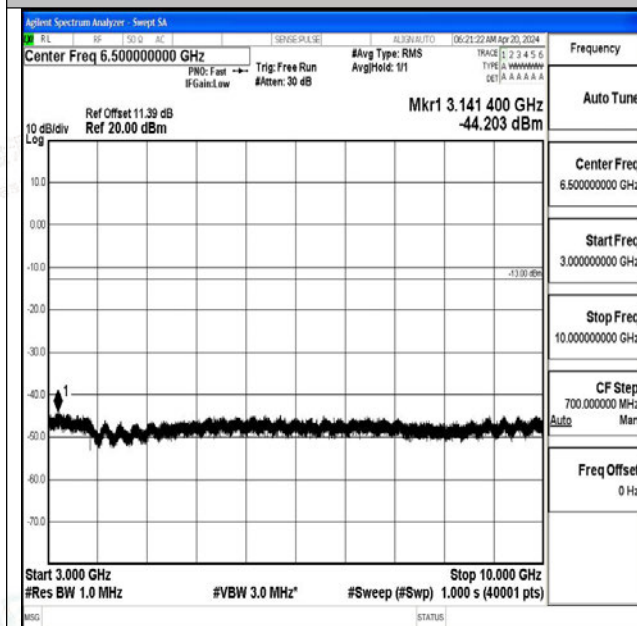
Band5_10MHz_QPSK_20600_1RB#0_3000~10000_300 0~10000
