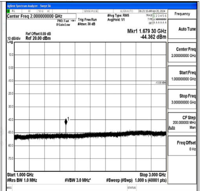
Band5_10MHz_QPSK_20600_1RB#0_1000~3000_1000 ~3000
