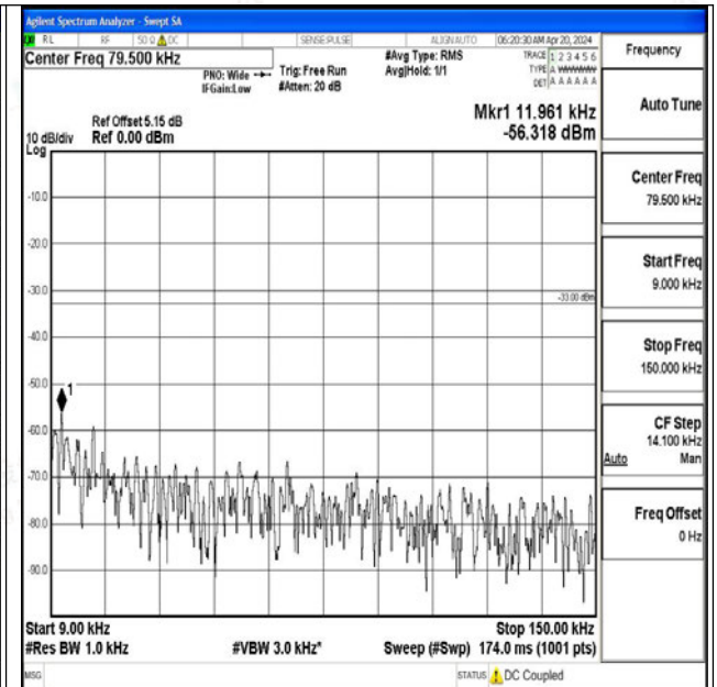
Band5_10MHz_16QAM_20525_1RB#0_0.009~0.15_0.0 09~0.15
