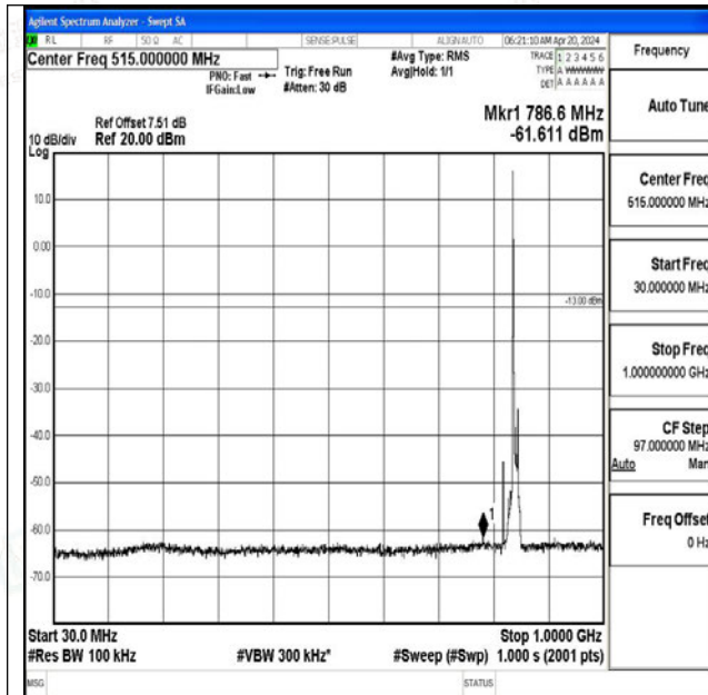
Band5_10MHz_QPSK_20600_1RB#0_30~1000_30~1000 0
