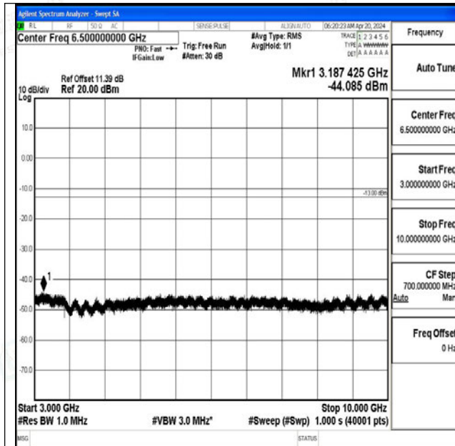
Band5_10MHz_QPSK_20525_1RB#0_3000~10000_300 0~10000
