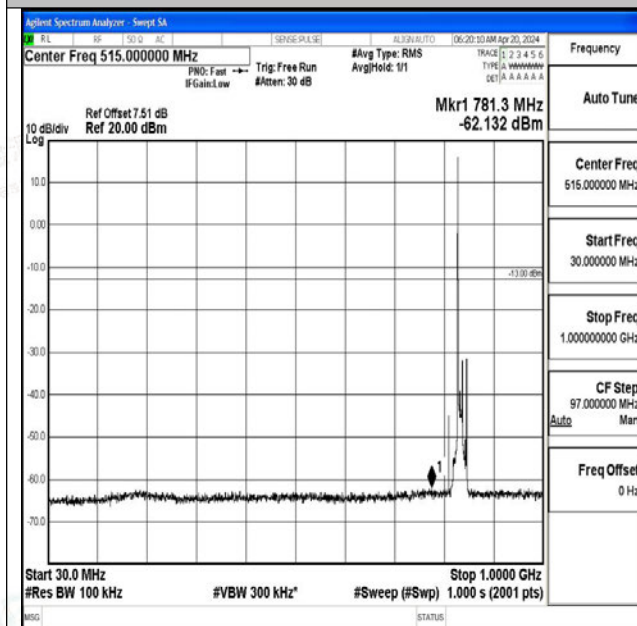
Band5_10MHz_QPSK_20525_1RB#0_30~1000_30~1000
