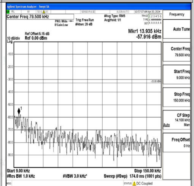
Band13_10MHz_16QAM_23230_1RB#0_0.009~0.15_0.009~0.15
