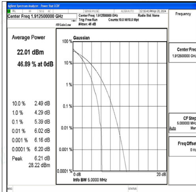
Band25-5MHz-QPSK-26665-1RB#0-PASS
