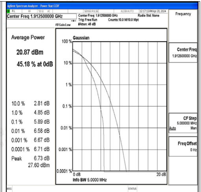
Band25-5MHz-16QAM-26665-1RB#0-PASS
