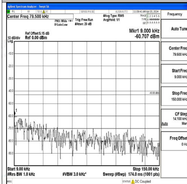
Band25_1.4MHz_QPSK_26365_1RB#0_0.009~0.15_0.0 09~0.15
