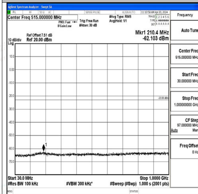
Band25_1.4MHz_QPSK_26683_1RB#0_30~1000_30~10
