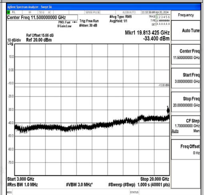
Band25_1.4MHz_16QAM_26365_1RB#0_3000~20000_ 3000~20000
