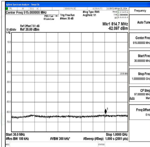
Band25_1.4MHz_QPSK_26365_1RB#0_30~1000_30~1000
