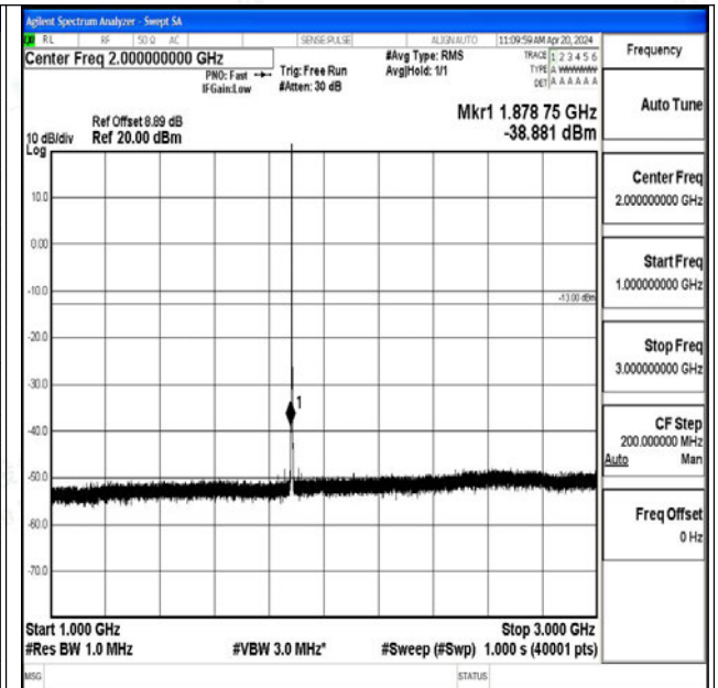
Band25_1.4MHz_QPSK_26365_1RB#0_1000~3000_1000~3000
