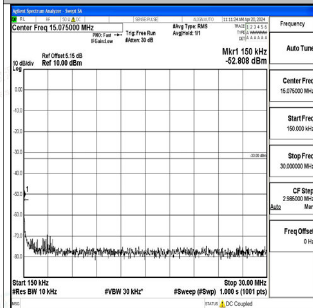
Band25_1.4MHz_16QAM_26683_1RB#0_0.15~30_0.15 ~30
