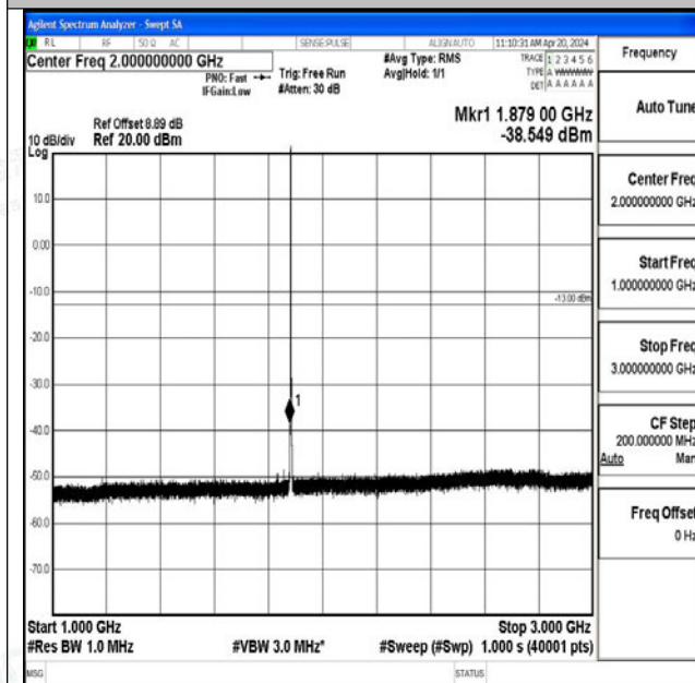
Band25_1.4MHz_16QAM_26365_1RB#0_1000~3000_1 000~3000
