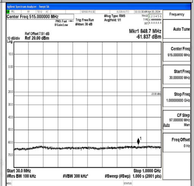
Band25_1.4MHz_16QAM_26683_1RB#0_30~1000_30~ 1000
