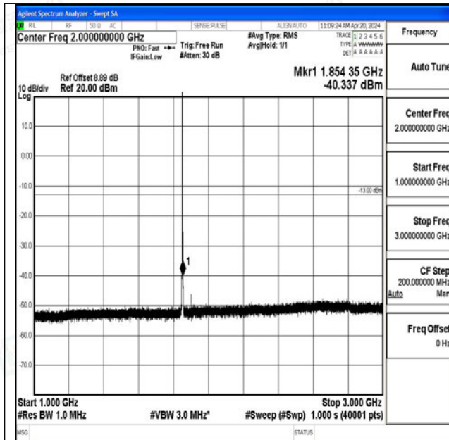
Band25_1.4MHz_16QAM_26047_1RB#0_1000~3000_1 000~3000
