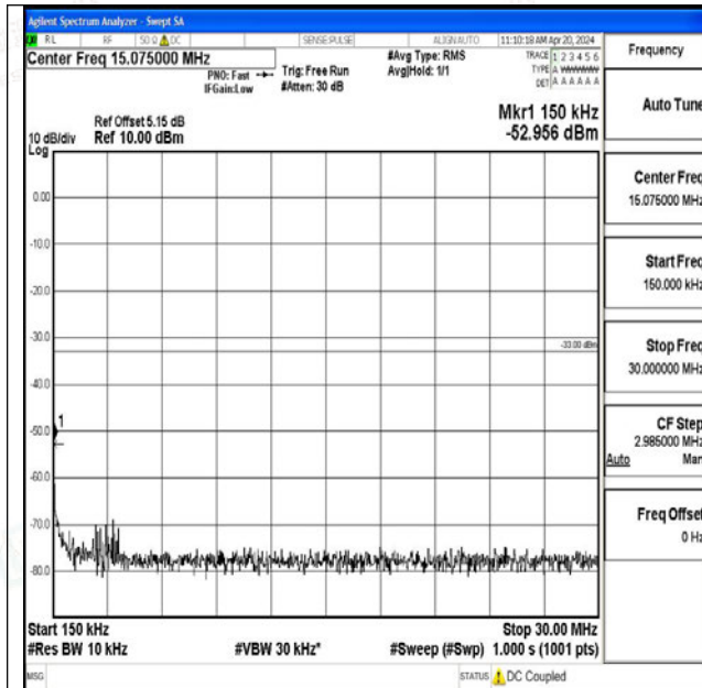
Band25_1.4MHz_16QAM_26365_1RB#0_0.15~30_0.15 ~30
