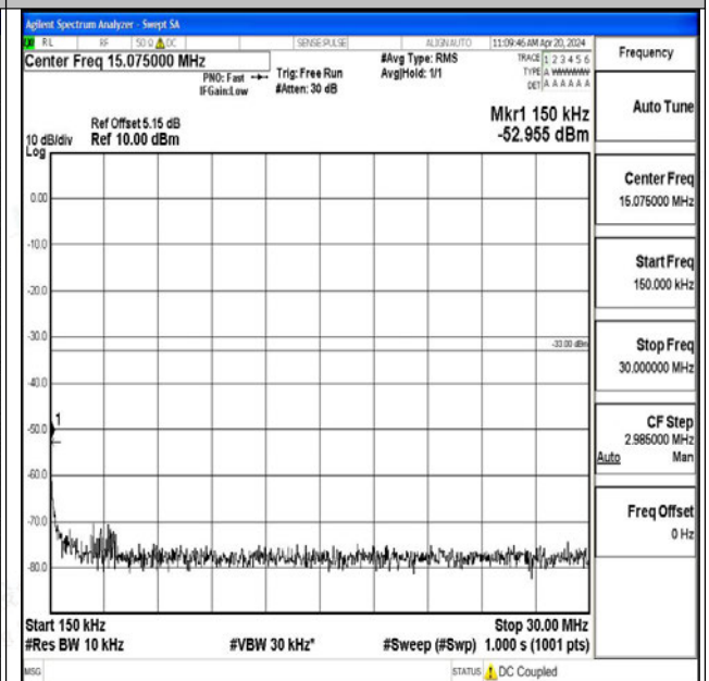
Band25_1.4MHz_QPSK_26365_1RB#0_0.15~30_0.15~3 0
