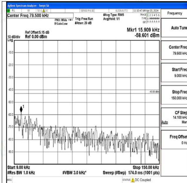
Band25_1.4MHz_QPSK_26683_1RB#0_0.009~0.15_0.09~0.15
