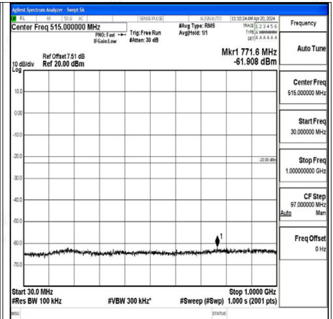
Band25_1.4MHz_16QAM_26365_1RB#0_30~1000_30~ 1000
