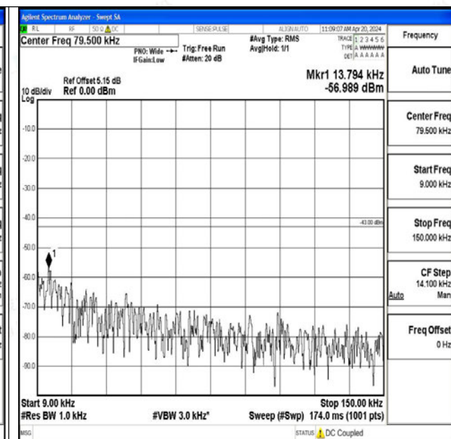
Band25_1.4MHz_16QAM_26047_1RB#0_0.009~0.15_0.009~0.15
