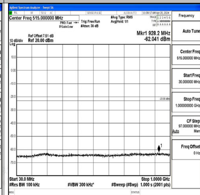
Band25_1.4MHz_16QAM_26047_1RB#0_30~1000_30~1000
