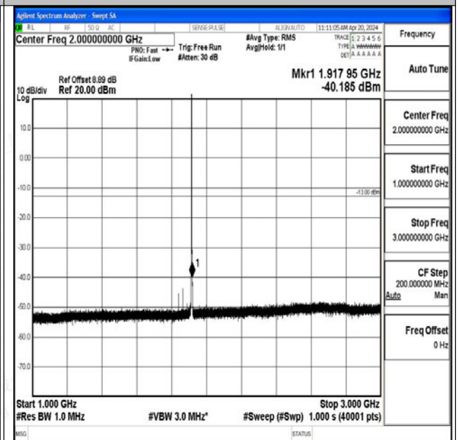
Band25_1.4MHz_QPSK_26683_1RB#0_1000~3000_1000~3000
