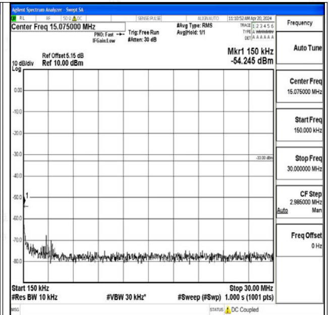
Band25_1.4MHz_QPSK_26683_1RB#0_0.15~30_0.15~3
