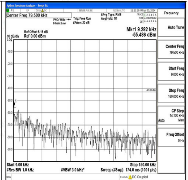
Band25_1.4MHz_16QAM_26683_1RB#0_0.009~0.15_0. 009~0.15
