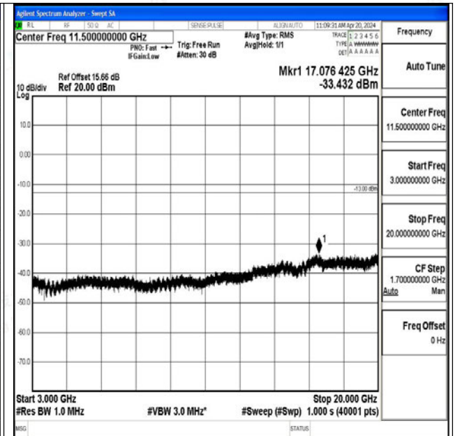
Band25_1.4MHz_16QAM_26047_1RB#0_3000~20000_ 3000~20000
