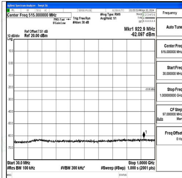
Band25_20MHz_QPSK_26140_1RB#0_30~1000_30~1000
