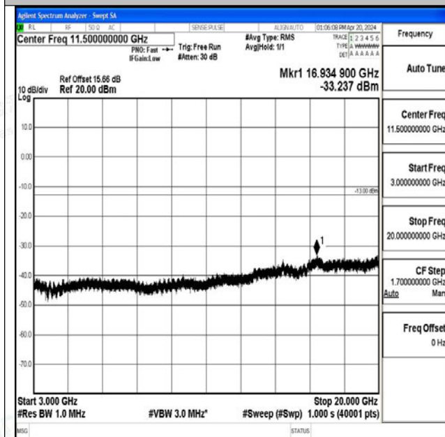
Band25_20MHz_QPSK_26140_1RB#0_3000~20000_3000~20000
