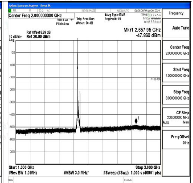
Band25_20MHz_QPSK_26140_1RB#0_1000~3000_1000~3000
