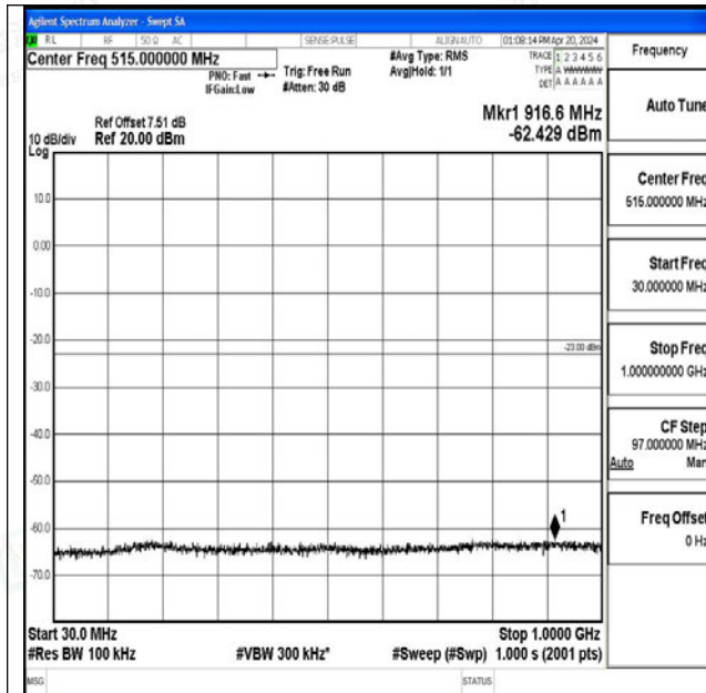
Band25_20MHz_QPSK_26590_1RB#0_30~1000_30~1000
