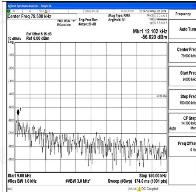
Band25_20MHz_QPSK_26365_1RB#0_0.009~0.15_0.00 9~0.15
