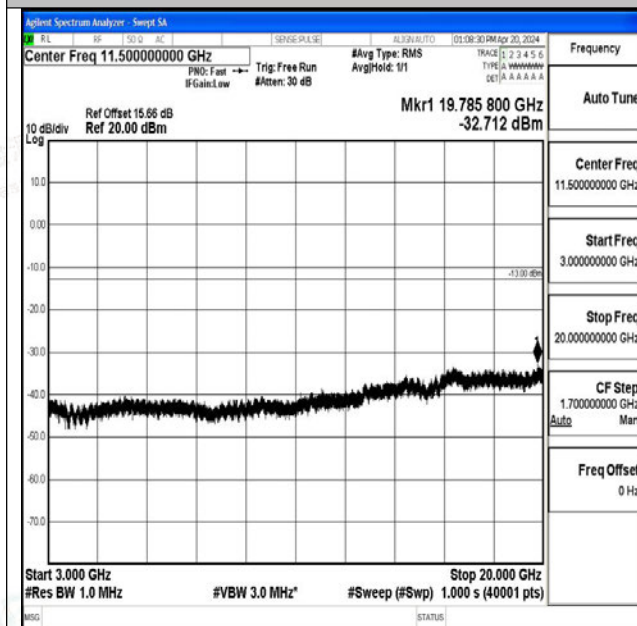
Band25_20MHz_QPSK_26590_1RB#0_3000~20000_3000~20000
