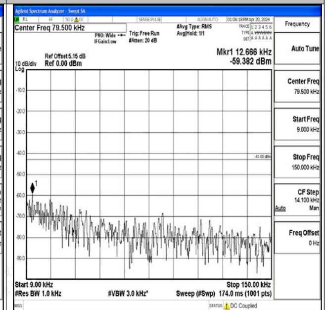
Band25_20MHz_16QAM_26140_1RB#0_0.009~0.15_0.009~0.15
