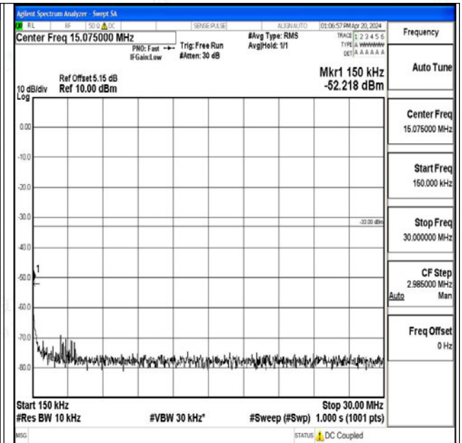
Band25_20MHz_QPSK_26365_1RB#0_0.15~30_0.15~3 0
