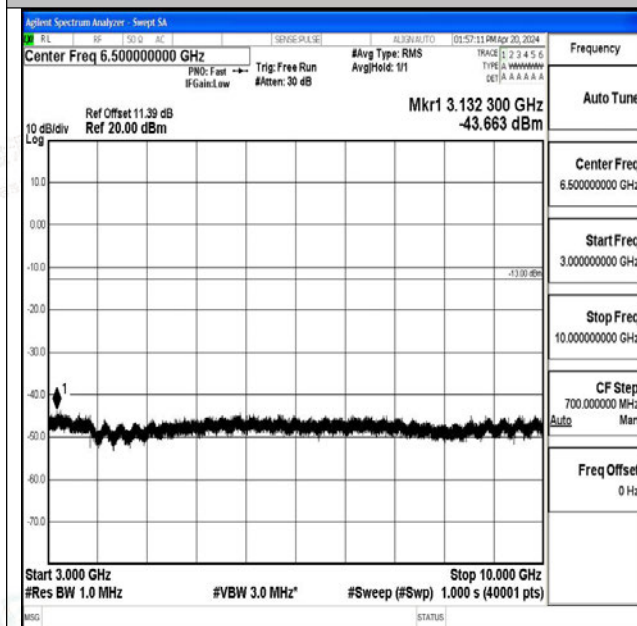
Band26_3MHz_QPSK_26705_1RB#0_3000~10000_300 0~10000
