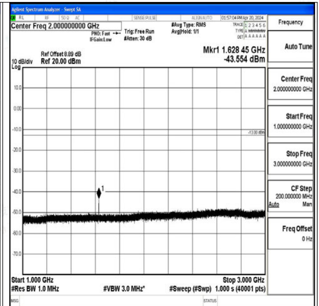
Band26_3MHz_QPSK_26705_1RB#0_1000~3000_1000 ~3000
