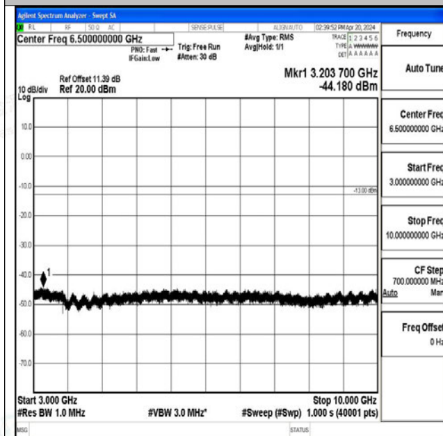
Band26_10MHz_QPSK_26740_1RB#0_3000~10000_3000~10000
