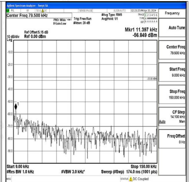
Band26_5MHz_16QAM_26765_1RB#0_0.009~0.15_0.0 09~0.15
