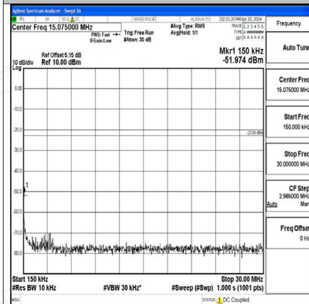
Band26_5MHz_16QAM_26715_1RB#0_0.15~30_0.15~3 0
