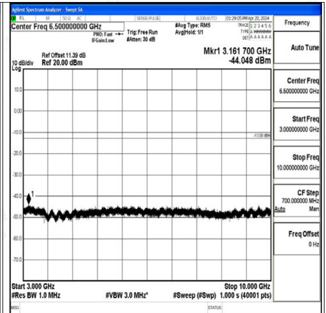
Band26_1.4MHz_16QAM_26783_1RB#0_3000~10000_ 3000~10000
