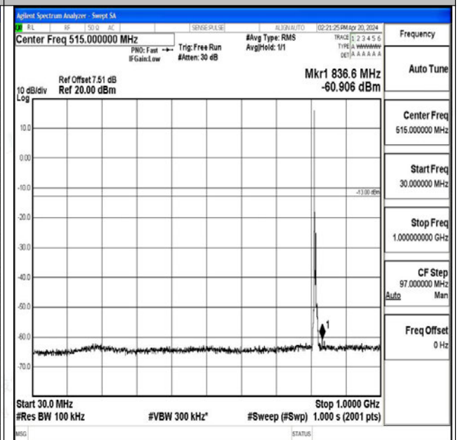
Band26_5MHz_16QAM_26715_1RB#0_30~1000_30~10 00
