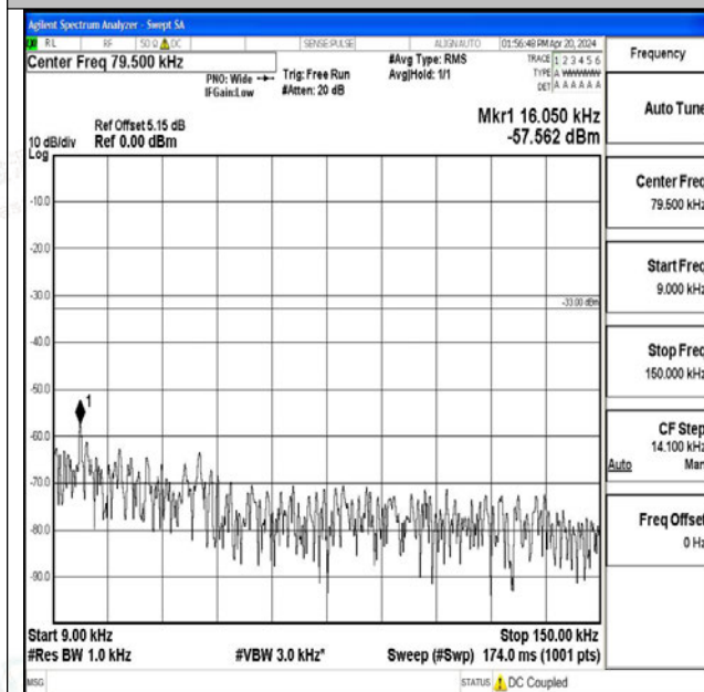
Band26_3MHz_QPSK_26705_1RB#0_0.009~0.15_0.009 ~0.15
