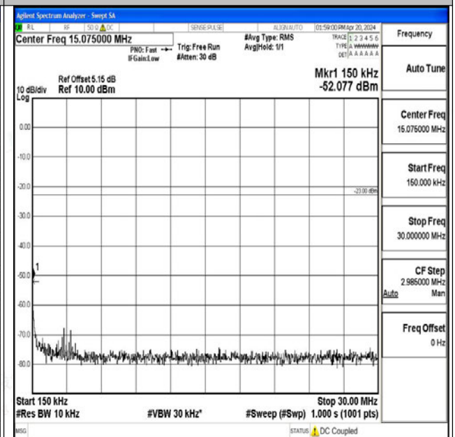
Band26_3MHz_QPSK_26775_1RB#0_0.15~30_0.15~30
