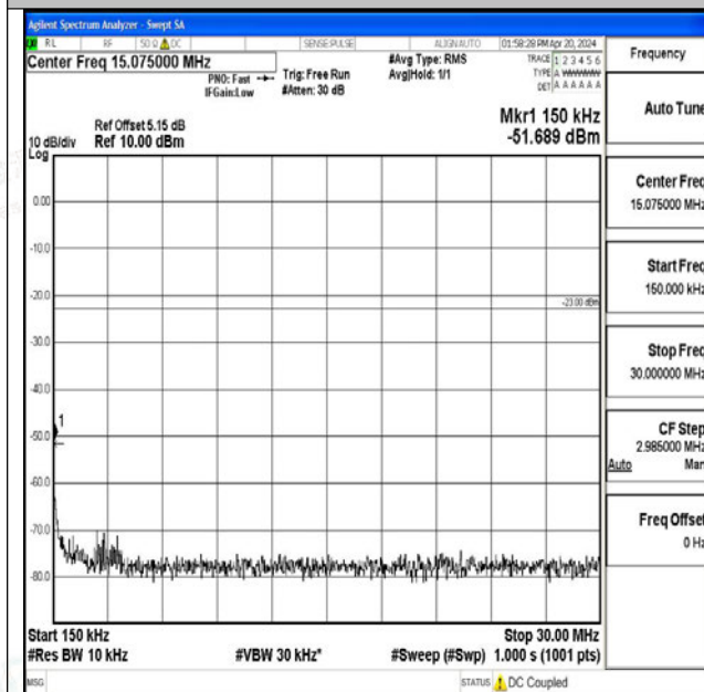
Band26_3MHz_16QAM_26740_1RB#0_0.15~30_0.15~3 0
