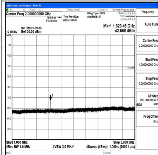
Band26_10MHz_16QAM_26740_1RB#0_1000~3000_1000~3000
