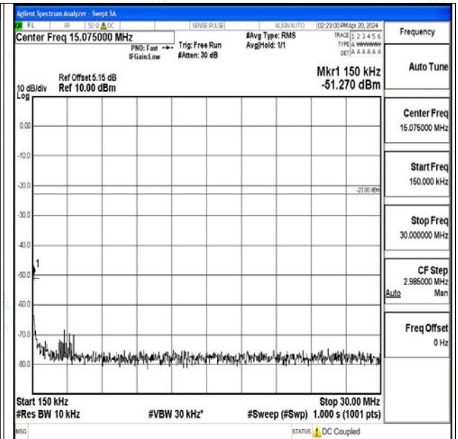
Band26_5MHz_QPSK_26765_1RB#0_0.15~30_0.15~30
