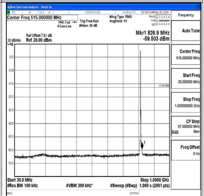
Band26_3MHz_16QAM_26740_1RB#0_30~1000_30~10 00
