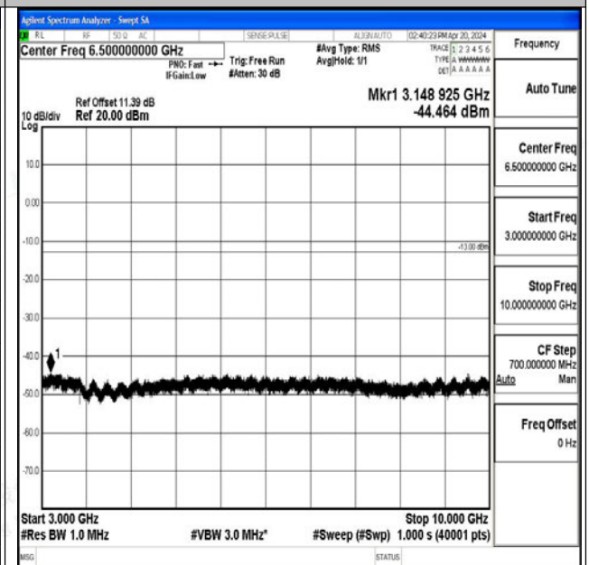
Band26_10MHz_16QAM_26740_1RB#0_3000~10000_3000~10000
