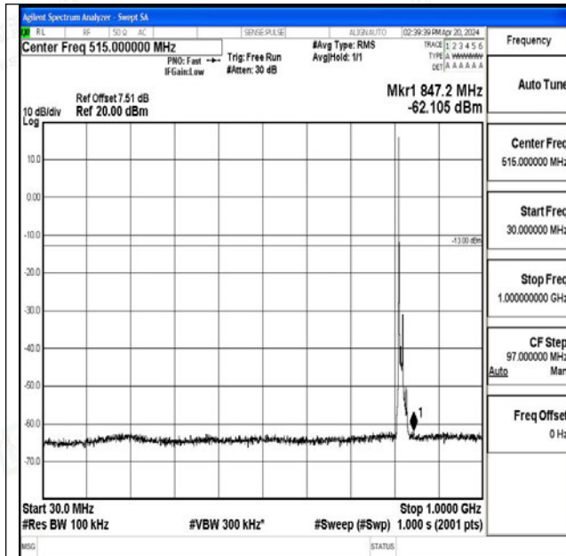
Band26_10MHz_QPSK_26740_1RB#0_30~1000_30~1000
