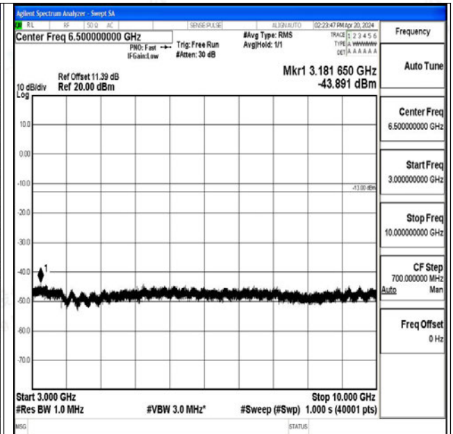
Band26_5MHz_16QAM_26765_1RB#0_3000~10000_30 00~10000
