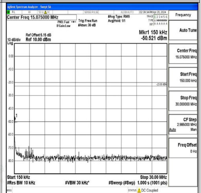
Band26_10MHz_QPSK_26740_1RB#0_0.15~30_0.15~3 0
