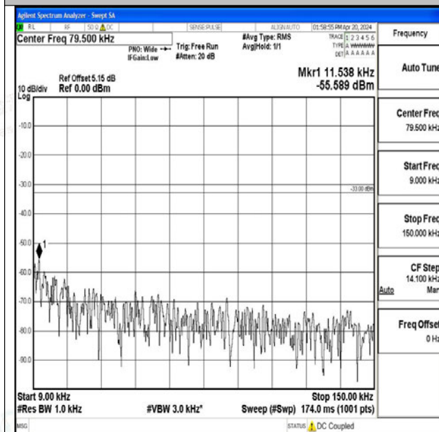
Band26_3MHz_QPSK_26775_1RB#0_0.009~0.15_0.009 ~0.15
