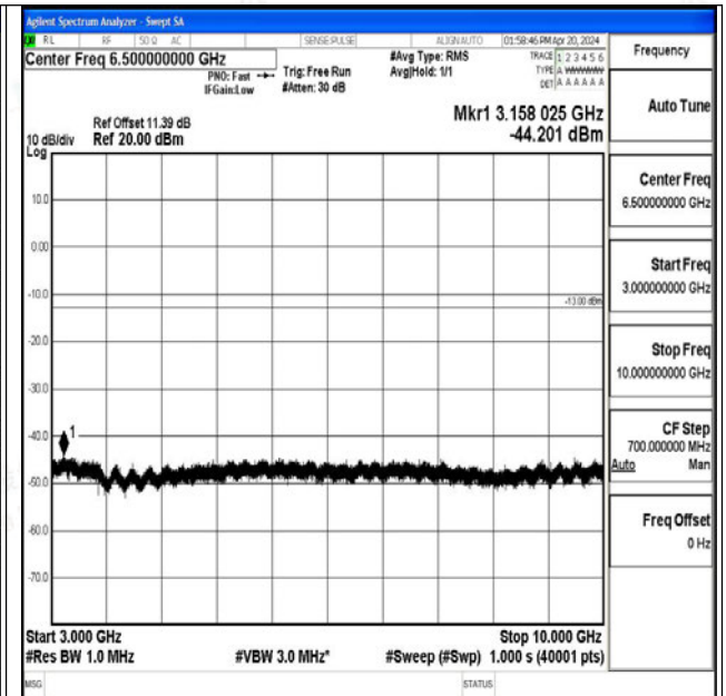
Band26_3MHz_16QAM_26740_1RB#0_3000~10000_30 00~10000
