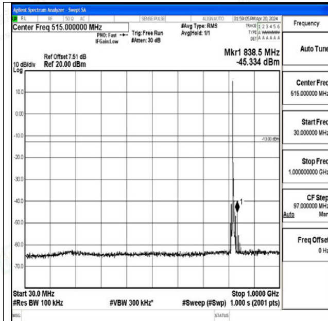
Band26_3MHz_QPSK_26775_1RB#0_30~1000_30~1000 0
