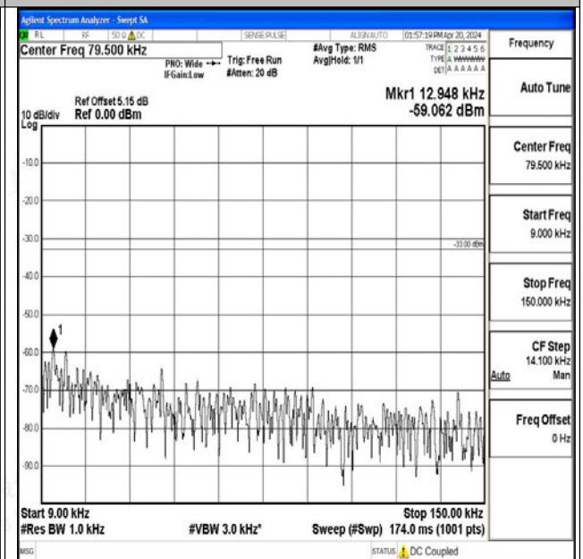
Band26_3MHz_16QAM_26705_1RB#0_0.009~0.15_0.0 09~0.15
