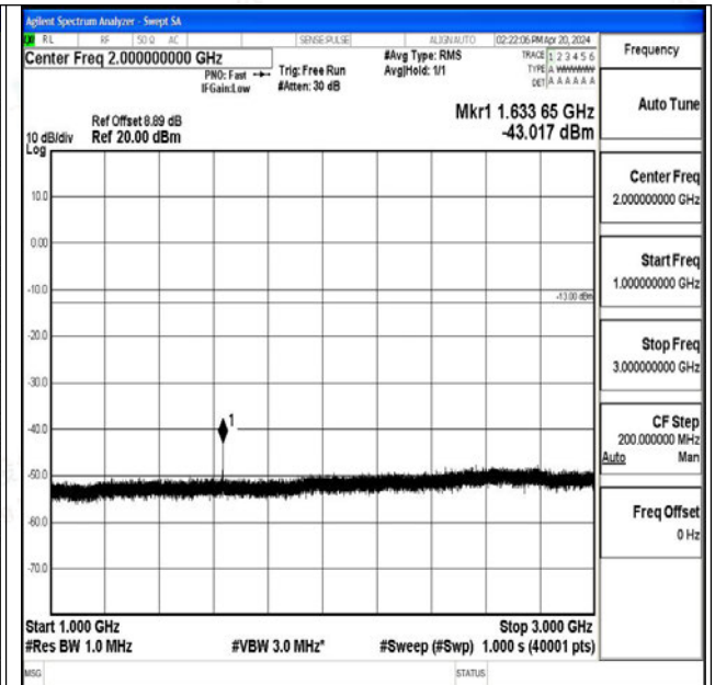
Band26_5MHz_QPSK_26740_1RB#0_1000~3000_1000 ~3000
