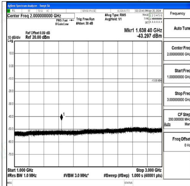
Band26_5MHz_16QAM_26765_1RB#0_1000~3000_100 0~3000
