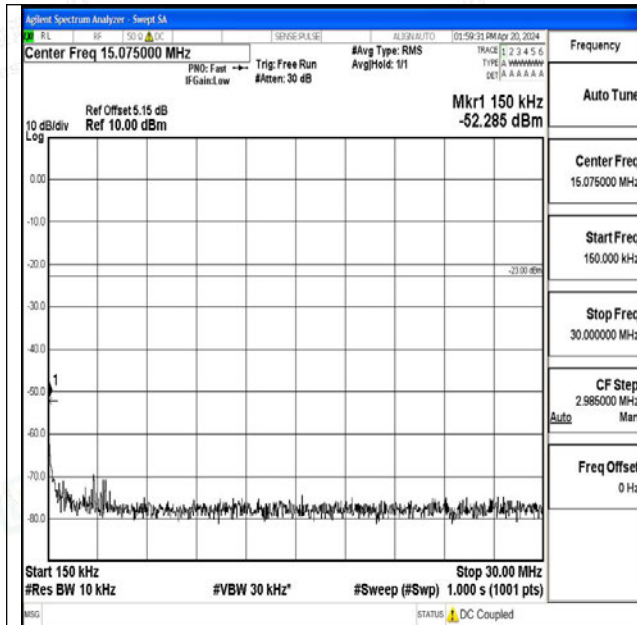
Band26_3MHz_16QAM_26775_1RB#0_0.15~30_0.15~3
