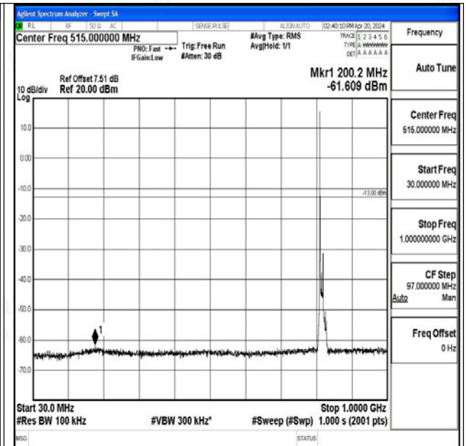
Band26_10MHz_16QAM_26740_1RB#0_30~1000_30~1000
