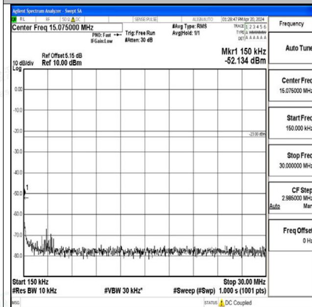
Band26_1.4MHz_16QAM_26783_1RB#0_0.15~30_0.15 ~30
