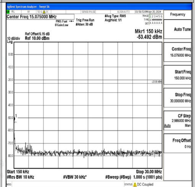
Band26_3MHz_QPSK_26705_1RB#0_0.15~30_0.15~30
