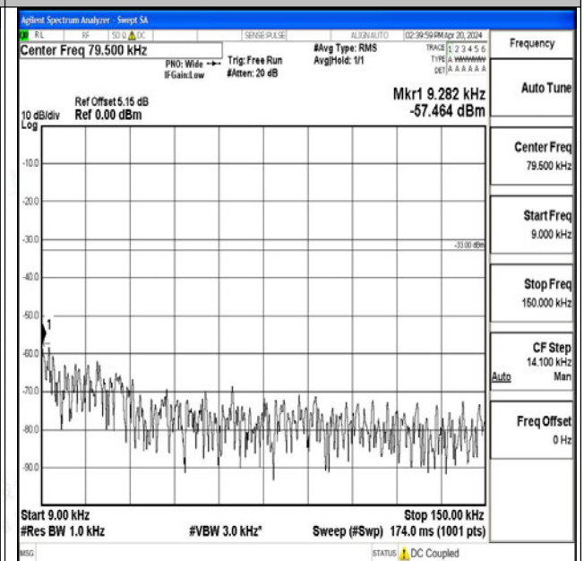
Band26_10MHz_16QAM_26740_1RB#0_0.009~0.15_0.009~0.15
