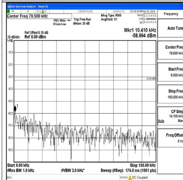
Band26_10MHz_QPSK_26740_1RB#0_0.009~0.15_0.00 9~0.15
