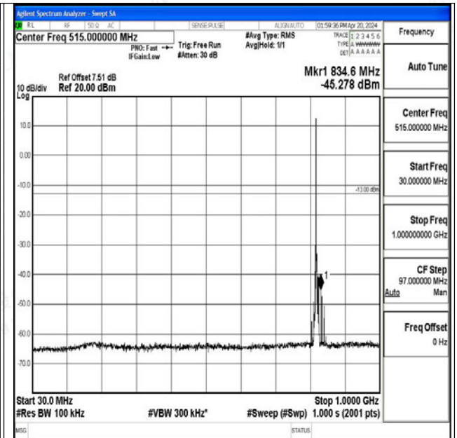
Band26_3MHz_16QAM_26775_1RB#0_30~1000_30~10
