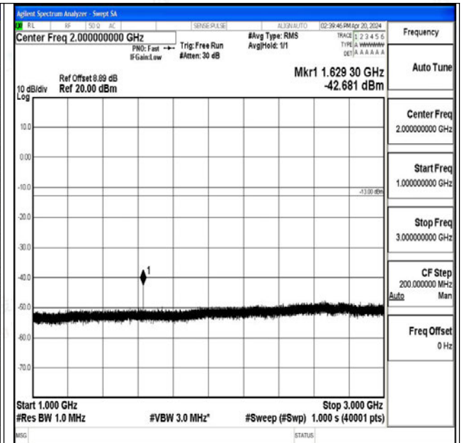
Band26_10MHz_QPSK_26740_1RB#0_1000~3000_1000~3000
