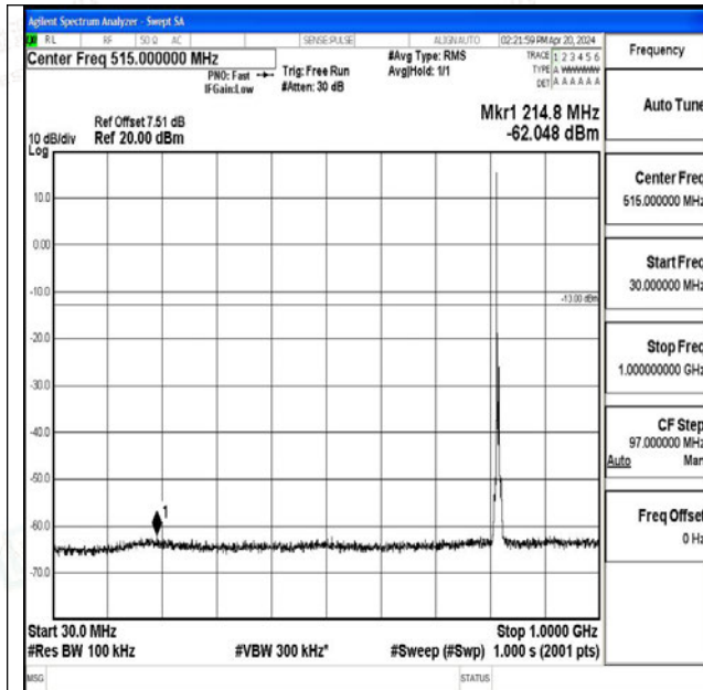
Band26_5MHz_QPSK_26740_1RB#0_30~1000_30~1000 0
