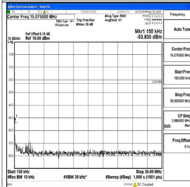
Band26_5MHz_16QAM_26765_1RB#0_0.15~30_0.15~3 0
