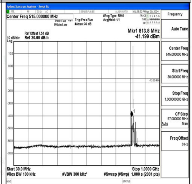
Band26_1.4MHz_16QAM_26783_1RB#0_30~1000_30~ 1000
