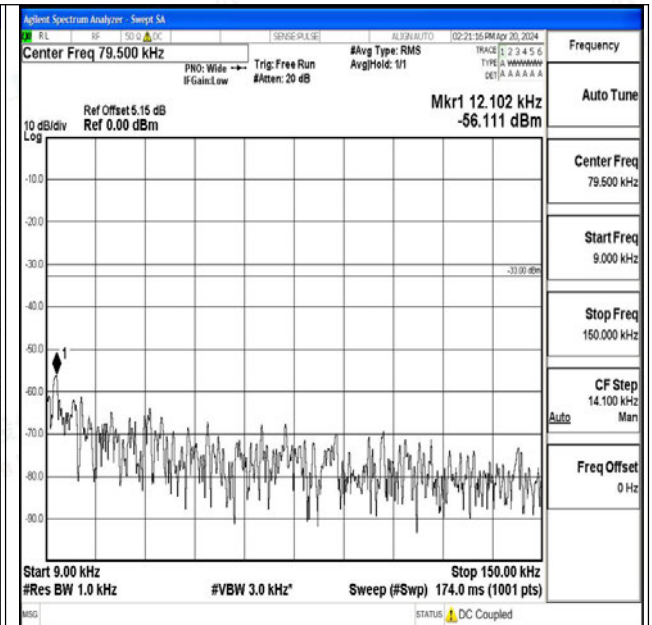
Band26_5MHz_16QAM_26715_1RB#0_0.009~0.15_0.0 09~0.15
