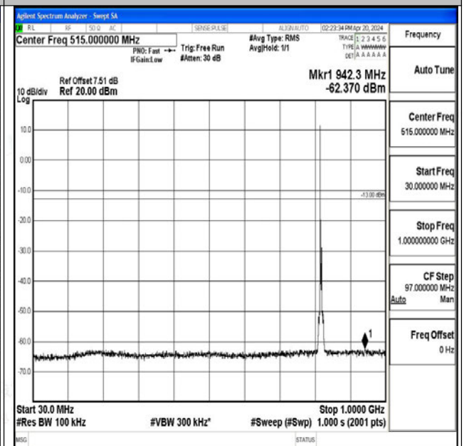
Band26_5MHz_16QAM_26765_1RB#0_30~1000_30~10 00
