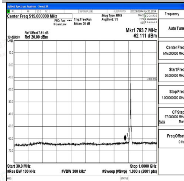
Band26_5MHz_QPSK_26765_1RB#0_30~1000_30~1000 0
