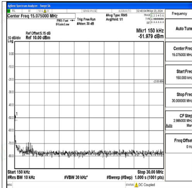
Band26_10MHz_16QAM_26740_1RB#0_0.15~30_0.15~30
