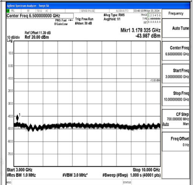
Band26_5MHz_16QAM_26915_1RB#0_3000~10000_30
