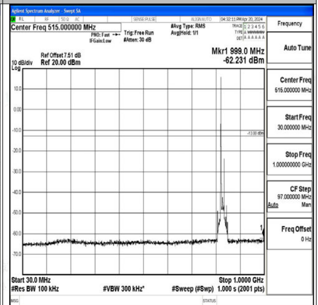
Band26_15MHz_16QAM_26865_1RB#0_30~1000_30~1 000
