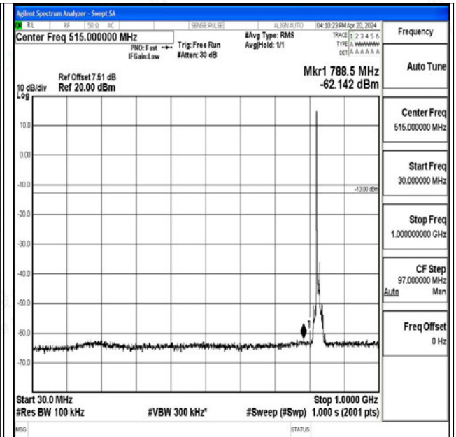
Band26_10MHz_16QAM_26840_1RB#0_30~1000_30~1000
