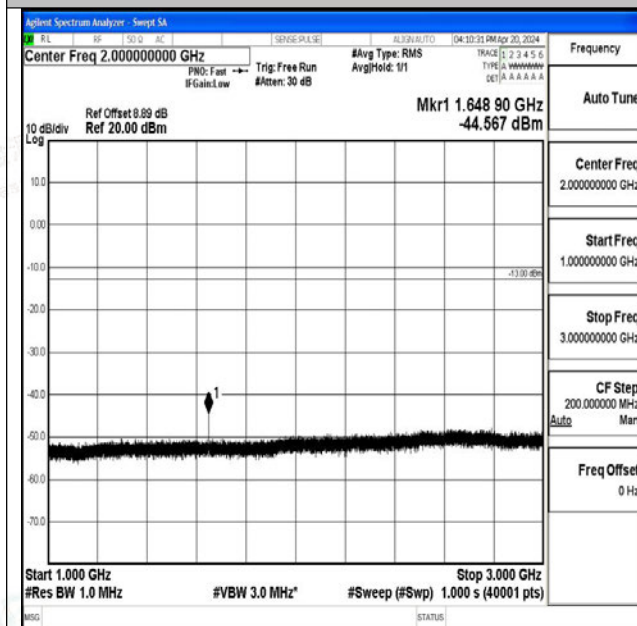
Band26_10MHz_16QAM_26840_1RB#0_1000~3000_1000~3000
