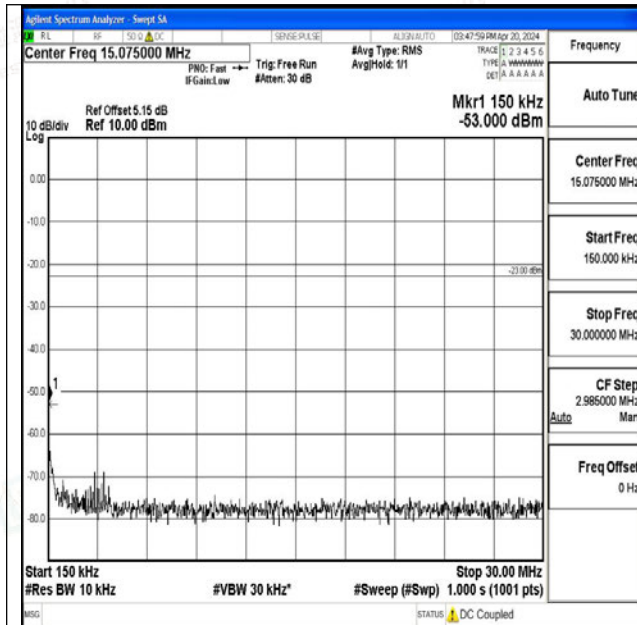
Band26_5MHz_16QAM_26915_1RB#0_0.15~30_0.15~3
