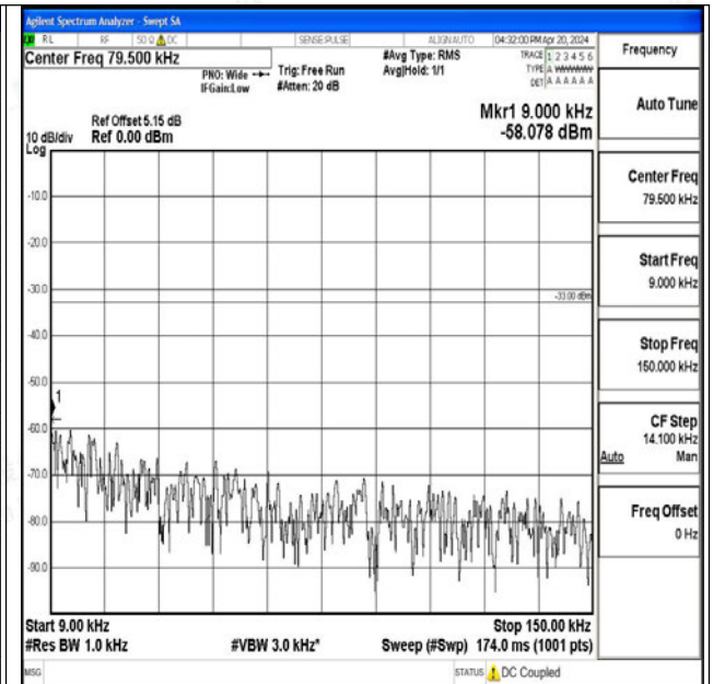
Band26_15MHz_16QAM_26865_1RB#0_0.009~0.15_0. 009~0.15
