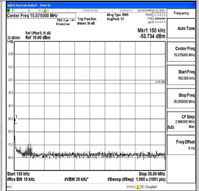
Band26_15MHz_QPSK_26965_1RB#0_0.15~30_0.15~3 0
