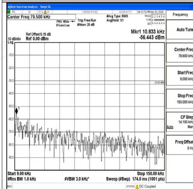
Band26_10MHz_QPSK_26990_1RB#0_0.009~0.15_0.00 9~0.15
