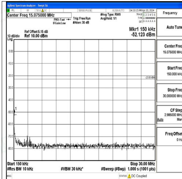
Band26_15MHz_16QAM_26915_1RB#0_0.15~30_0.15~30
