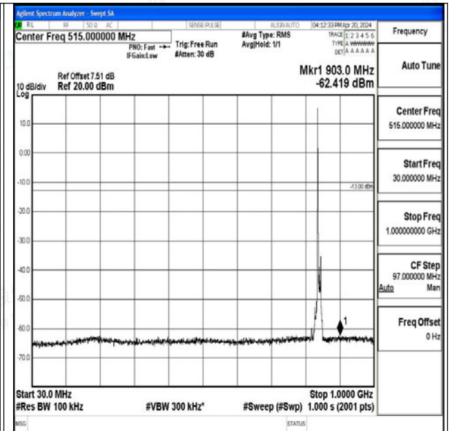
Band26_10MHz_16QAM_26990_1RB#0_30~1000_30~1000
