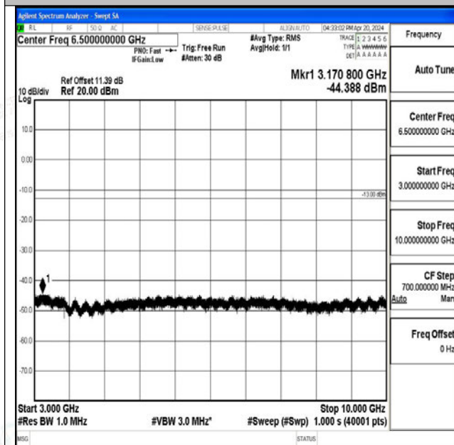
Band26_15MHz_QPSK_26915_1RB#0_3000~10000_30 00~10000
