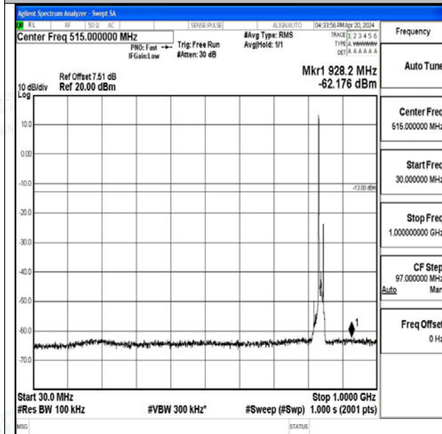
Band26_15MHz_QPSK_26965_1RB#0_30~1000_30~10 00
