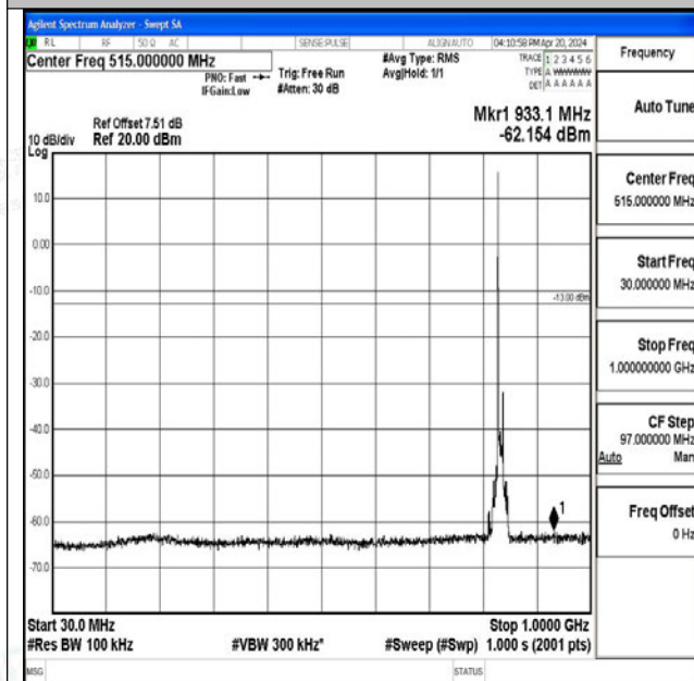
Band26_10MHz_QPSK_26915_1RB#0_30~1000_30~10 00
