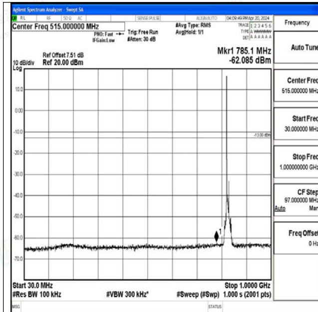
Band26_10MHz_QPSK_26840_1RB#0_30~1000_30~1000
