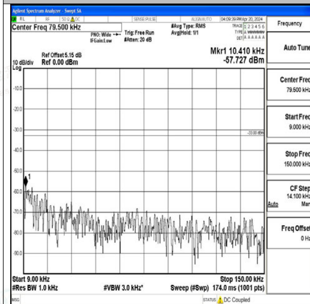
Band26_10MHz_QPSK_26840_1RB#0_0.009~0.15_0.00 9~0.15
