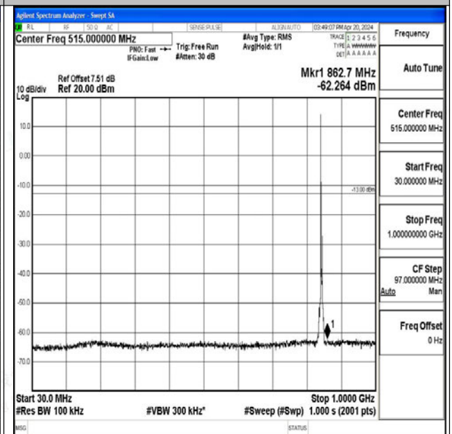
Band26_5MHz_16QAM_27015_1RB#0_30~1000_30~10 00
