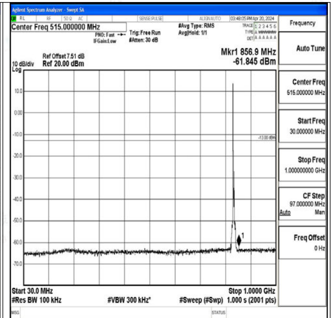
Band26_5MHz_16QAM_26915_1RB#0_30~1000_30~10
