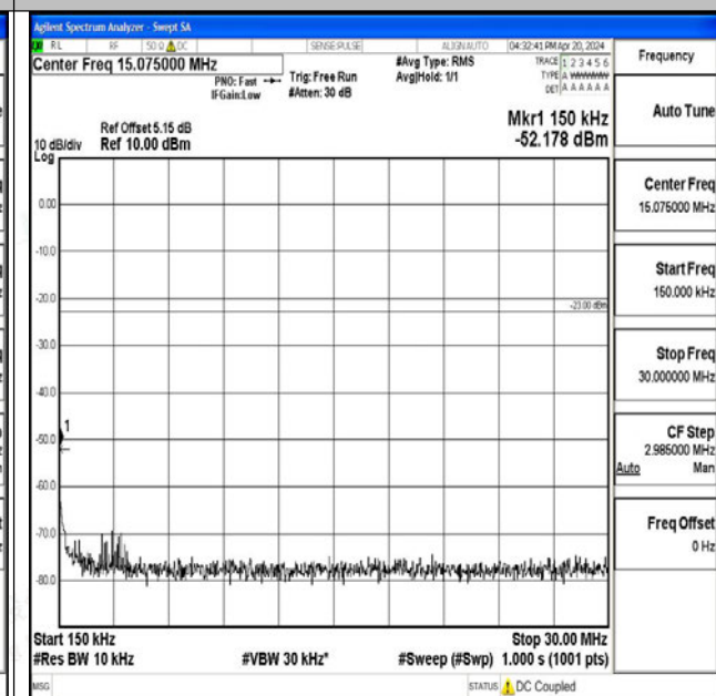
Band26_15MHz_QPSK_26915_1RB#0_0.15~30_0.15~30
