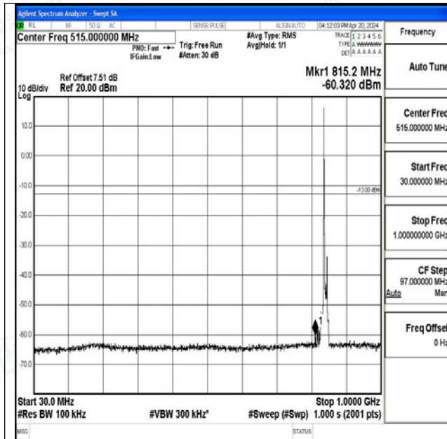
Band26_10MHz_QPSK_26990_1RB#0_30~1000_30~10 00
