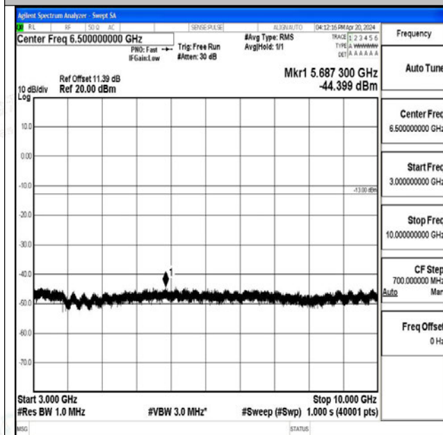
Band26_10MHz_QPSK_26990_1RB#0_3000~10000_30 00~10000
