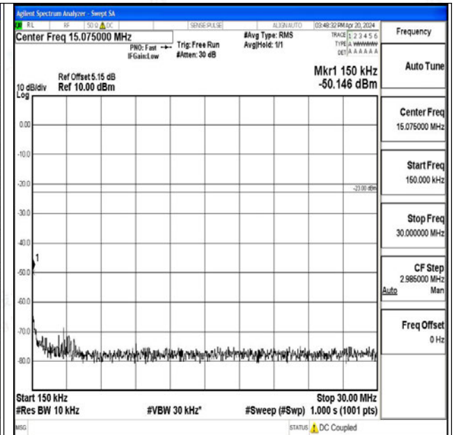
Band26_5MHz_QPSK_27015_1RB#0_0.15~30_0.15~30
