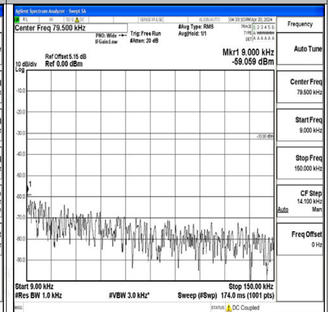
Band26_15MHz_16QAM_26915_1RB#0_0.009~0.15_0. 009~0.15
