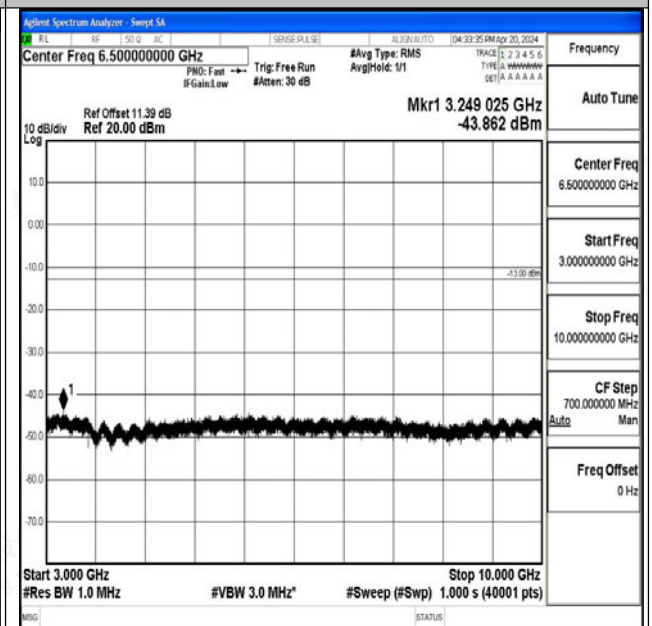
Band26_15MHz_16QAM_26915_1RB#0_3000~10000_3000~10000
