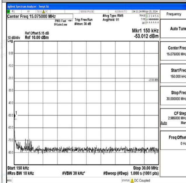
Band26_10MHz_16QAM_26915_1RB#0_0.15~30_0.15~ 30
