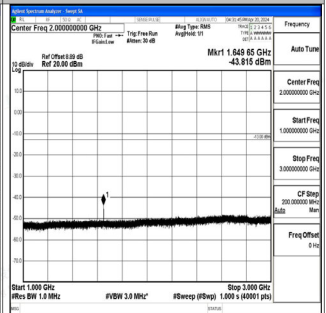
Band26_15MHz_QPSK_26865_1RB#0_1000~3000_100 0~3000
