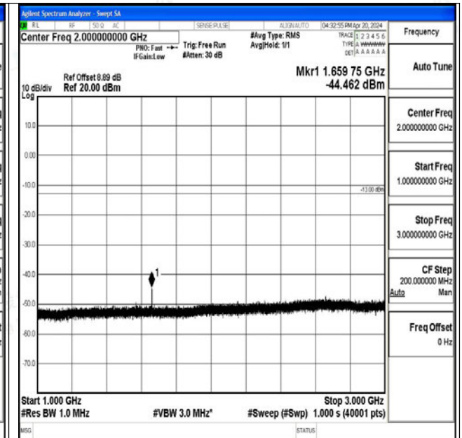
Band26_15MHz_QPSK_26915_1RB#0_1000~3000_100 0~3000
