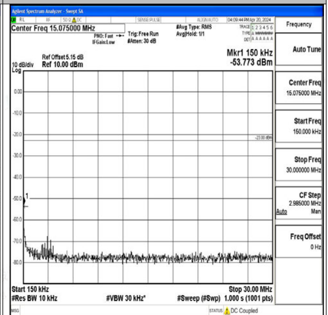
Band26_10MHz_QPSK_26840_1RB#0_0.15~30_0.15~3 0
