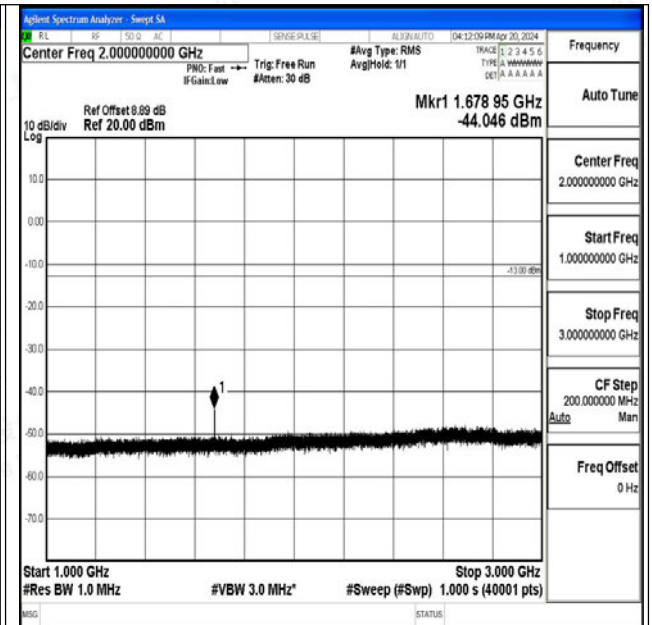
Band26_10MHz_QPSK_26990_1RB#0_1000~3000_100 0~3000
