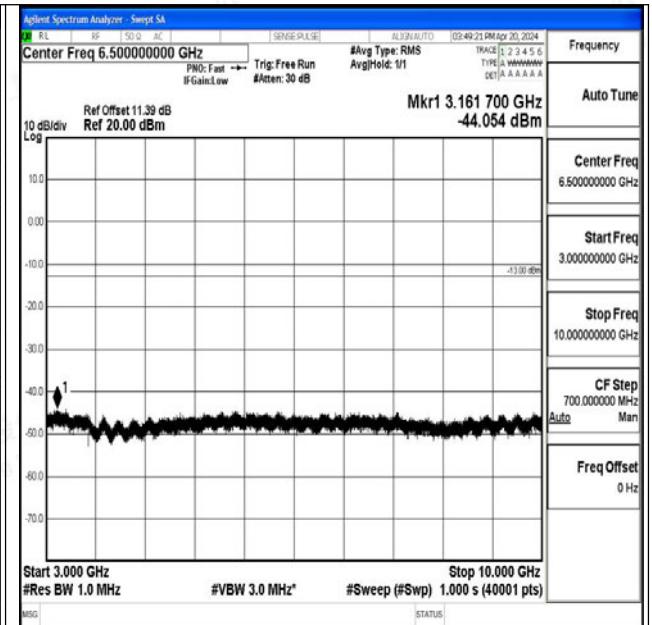
Band26_5MHz_16QAM_27015_1RB#0_3000~10000_30 00~10000
