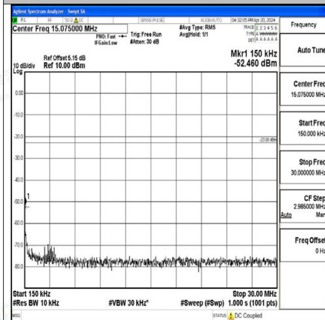
Band26_15MHz_16QAM_26865_1RB#0_0.15~30_0.15~ 30
