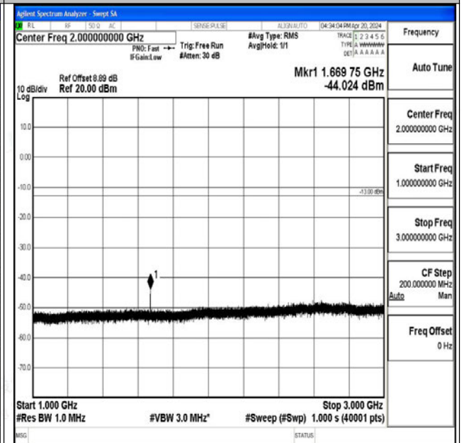
Band26_15MHz_QPSK_26965_1RB#0_1000~3000_100 0~3000
