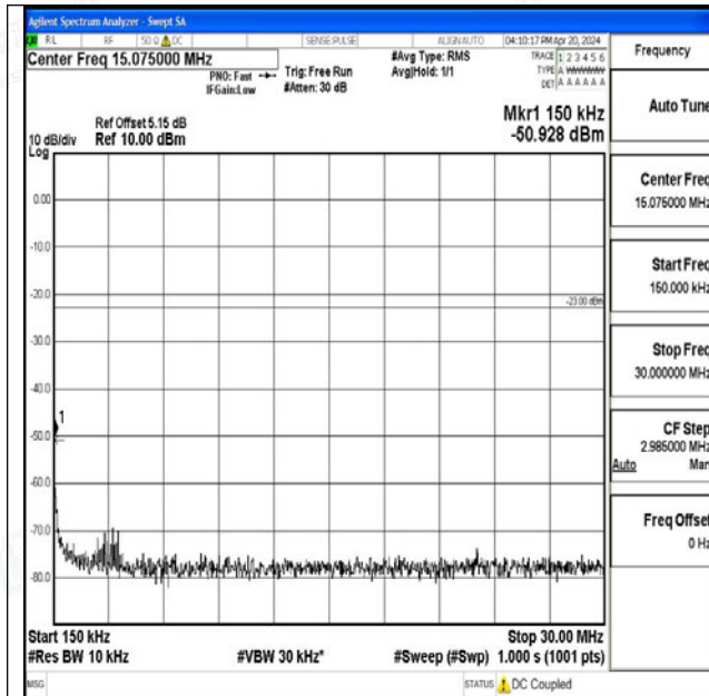
Band26_10MHz_16QAM_26840_1RB#0_0.15~30_0.15~30
