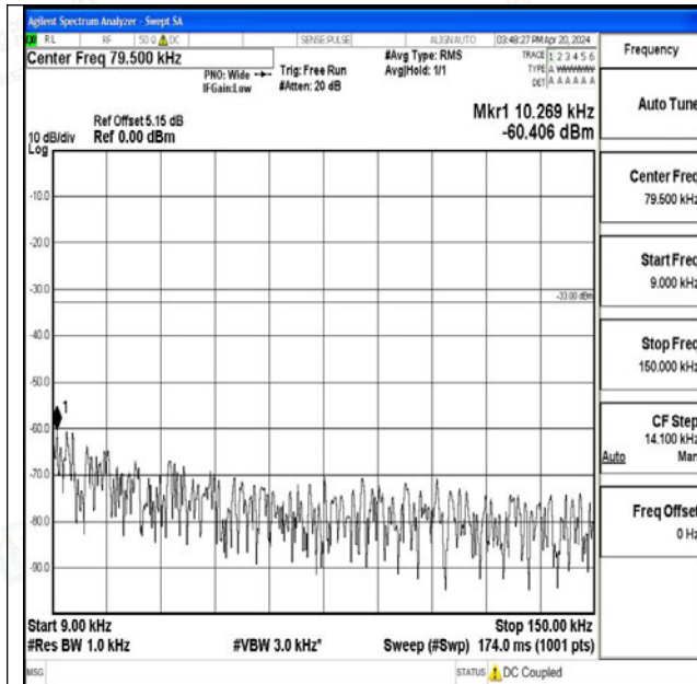
Band26_5MHz_QPSK_27015_1RB#0_0.009~0.15_0.009 ~0.15
