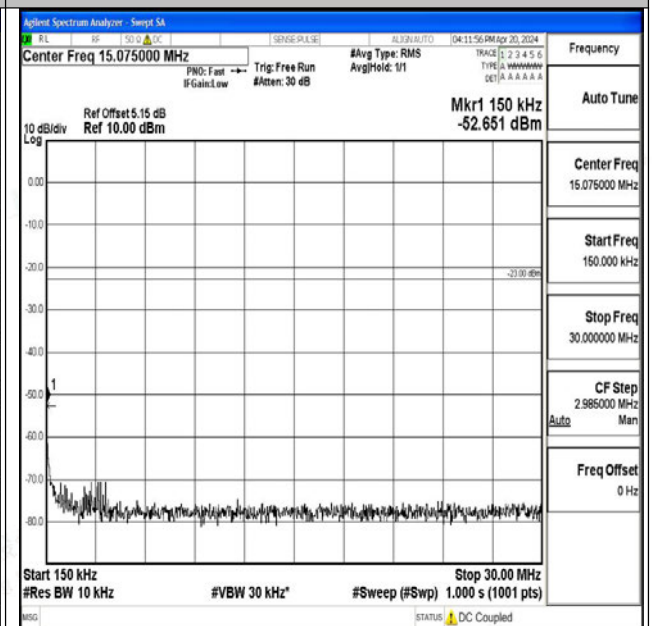
Band26_10MHz_QPSK_26990_1RB#0_0.15~30_0.15~3 0
