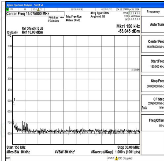
Band26_10MHz_16QAM_26990_1RB#0_0.15~30_0.15~30
