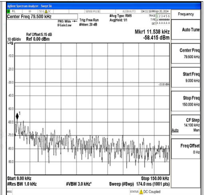
Band26_10MHz_16QAM_26915_1RB#0_0.009~0.15_0. 009~0.15
