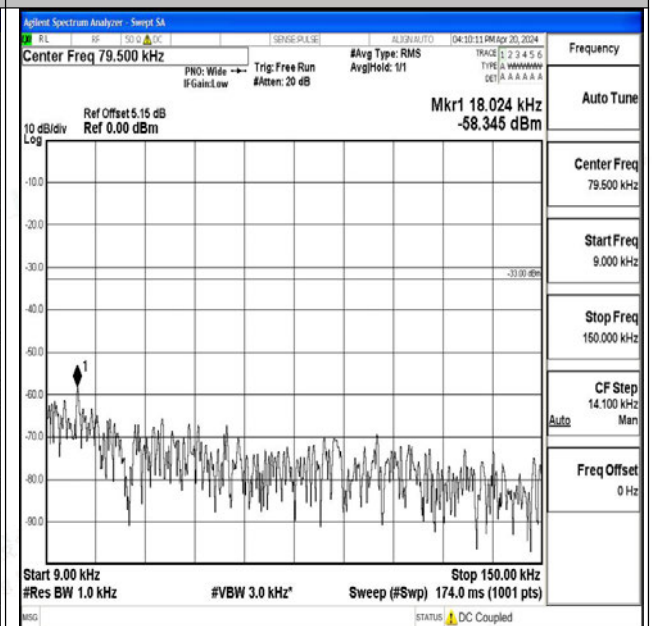
Band26_10MHz_16QAM_26840_1RB#0_0.009~0.15_0.009~0.15
