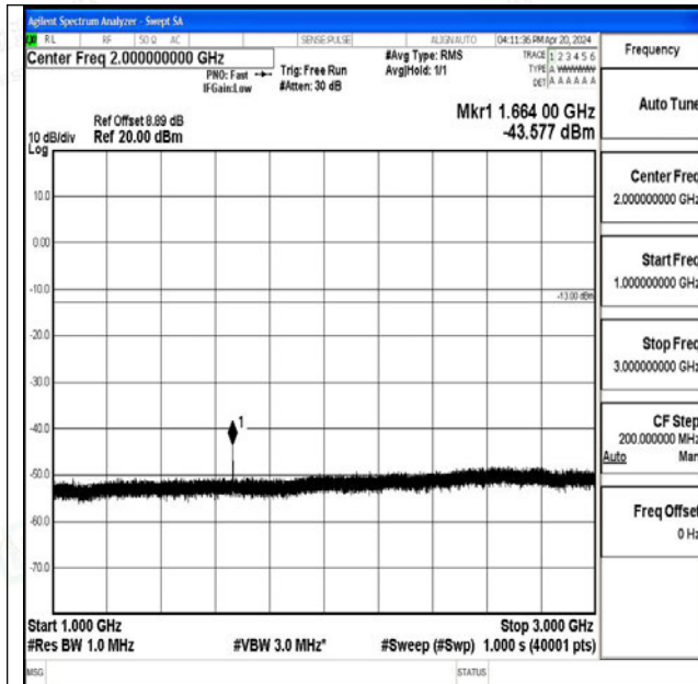
Band26_10MHz_16QAM_26915_1RB#0_1000~3000_10 00~3000
