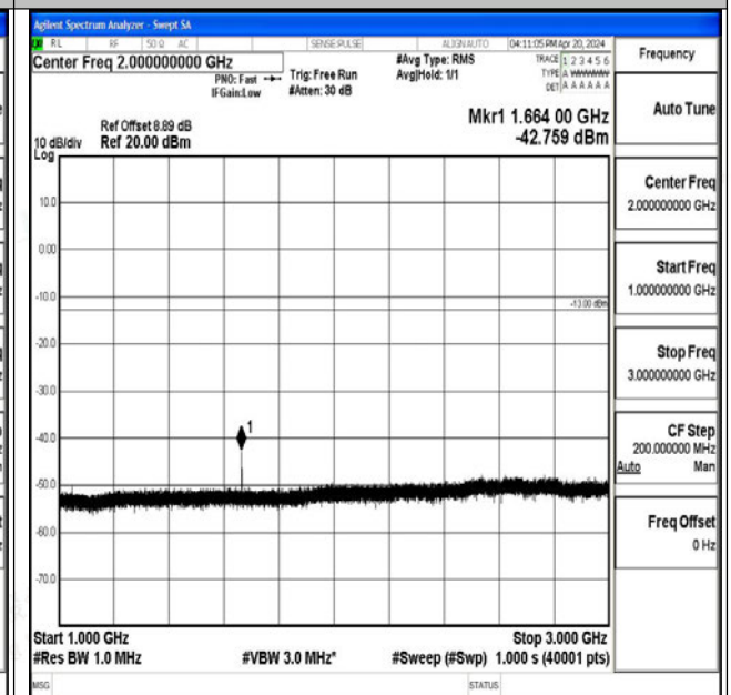
Band26_10MHz_QPSK_26915_1RB#0_1000~3000_100 0~3000
