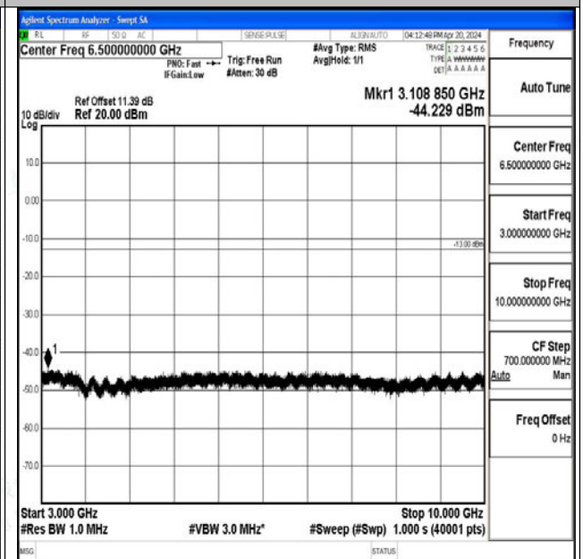
Band26_10MHz_16QAM_26990_1RB#0_3000~10000_3000~10000
