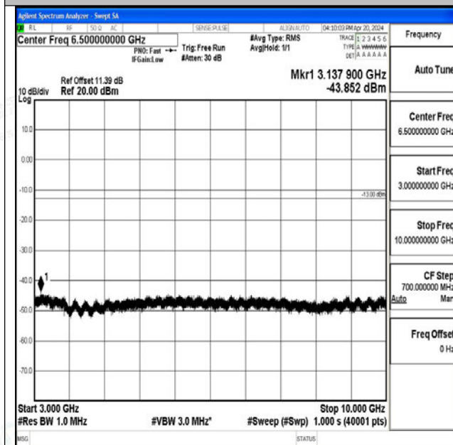
Band26_10MHz_QPSK_26840_1RB#0_3000~10000_3000~10000
