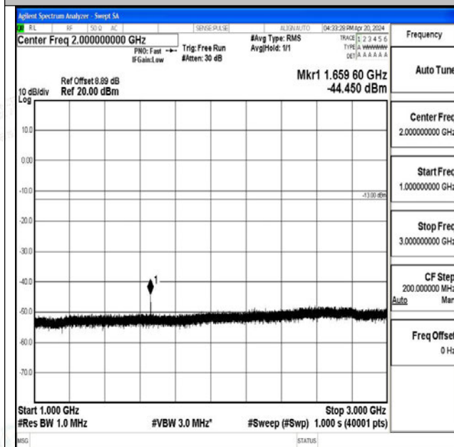
Band26_15MHz_16QAM_26915_1RB#0_1000~3000_1000~3000
