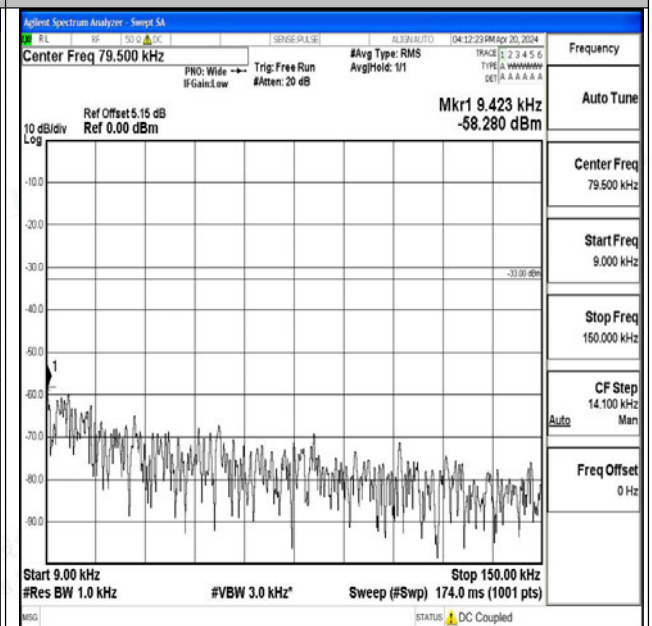
Band26_10MHz_16QAM_26990_1RB#0_0.009~0.15_0. 009~0.15
