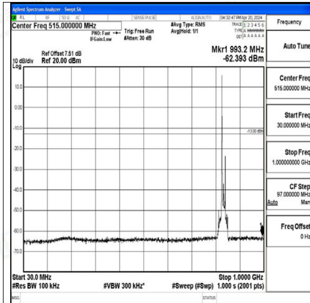
Band26_15MHz_QPSK_26915_1RB#0_30~1000_30~10 00
