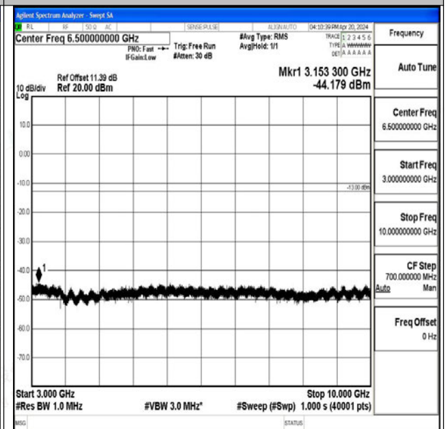
Band26_10MHz_16QAM_26840_1RB#0_3000~10000_3000~10000
