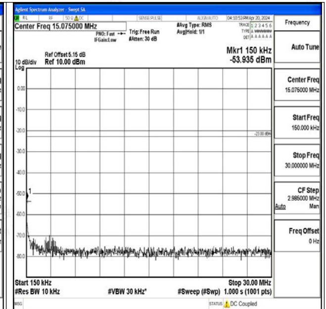
Band26_10MHz_QPSK_26915_1RB#0_0.15~30_0.15~3 0
