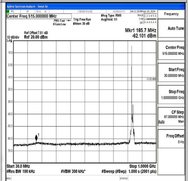
Band26_10MHz_16QAM_26915_1RB#0_30~1000_30~1 000
