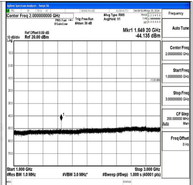
Band26_10MHz_QPSK_26840_1RB#0_1000~3000_1000~3000
