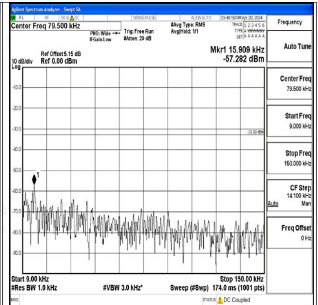
Band26_5MHz_16QAM_27015_1RB#0_0.009~0.15_0.0 09~0.15
