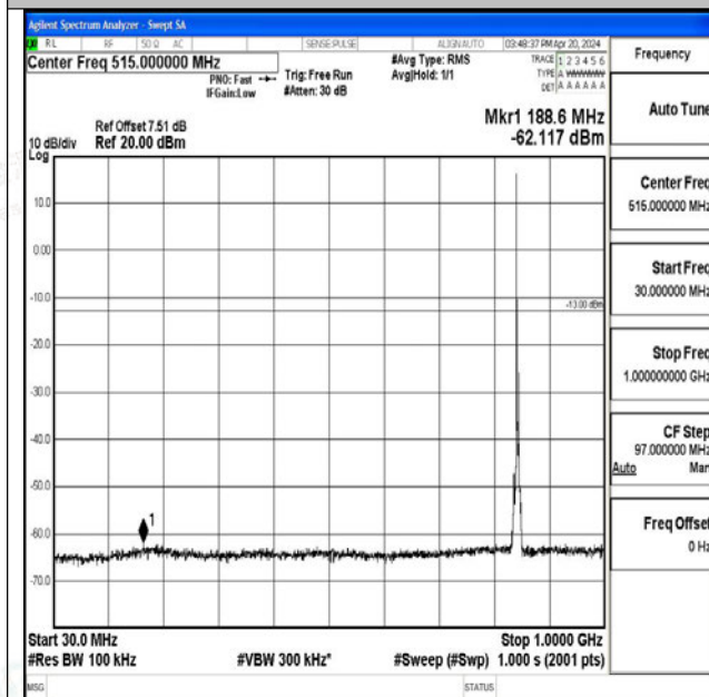
Band26_5MHz_QPSK_27015_1RB#0_30~1000_30~1000 0
