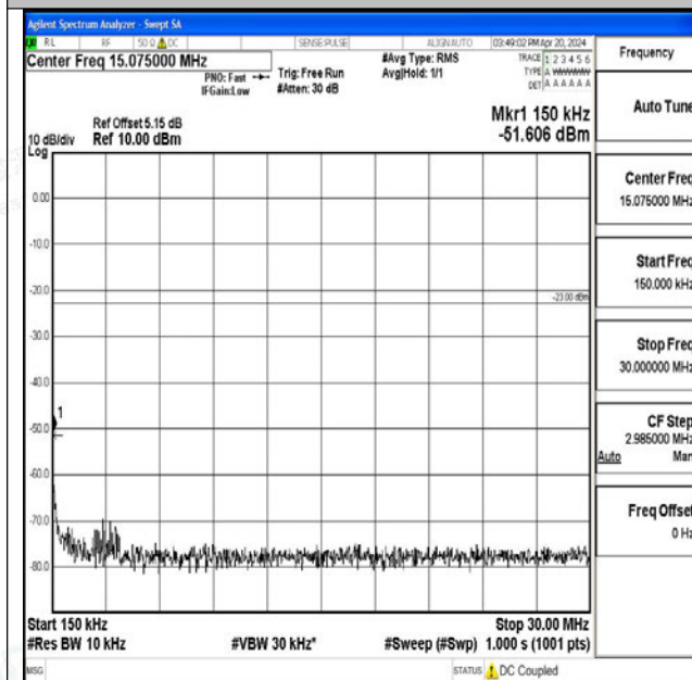
Band26_5MHz_16QAM_27015_1RB#0_0.15~30_0.15~3 0
