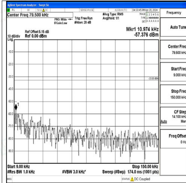
Band26_15MHz_QPSK_26965_1RB#0_0.009~0.15_0.00 9~0.15
