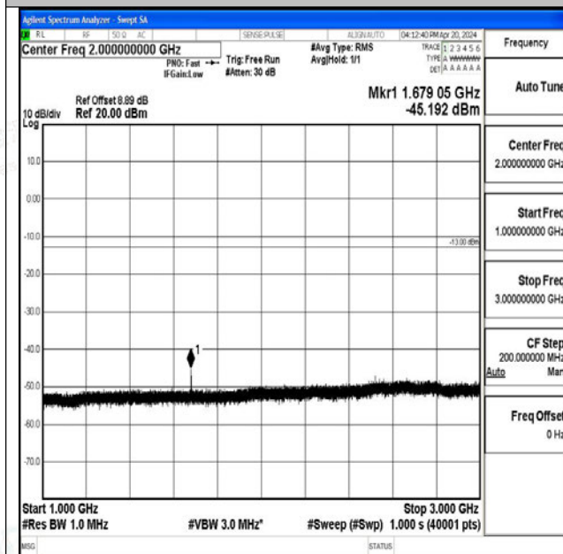
Band26_10MHz_16QAM_26990_1RB#0_1000~3000_1000~3000
