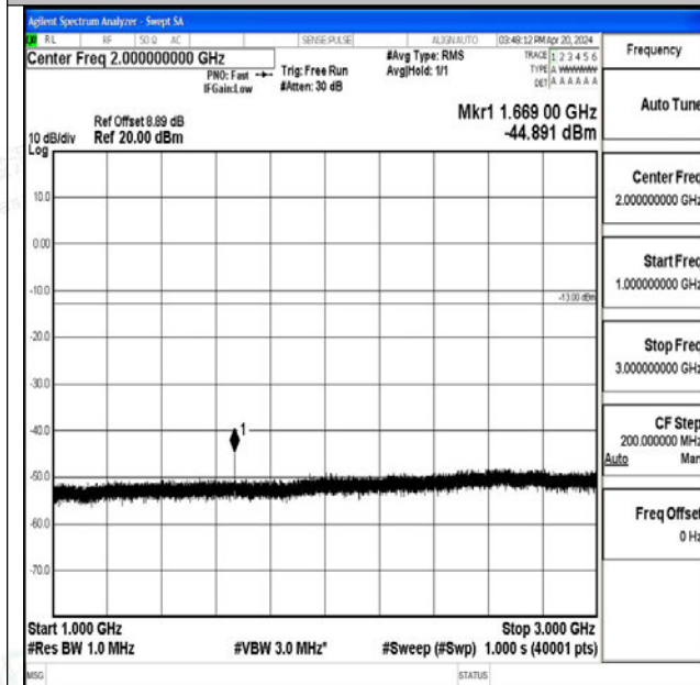
Band26_5MHz_16QAM_26915_1RB#0_1000~3000_100
