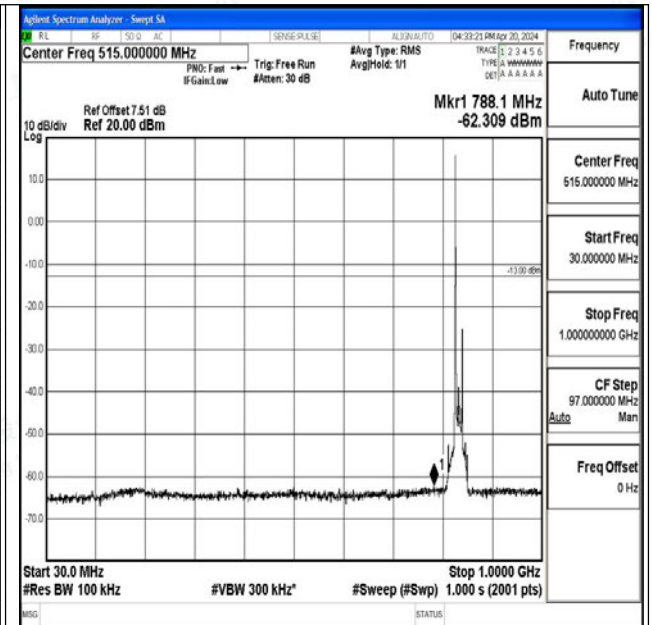
Band26_15MHz_16QAM_26915_1RB#0_30~1000_30~1000
