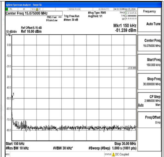
Band26_15MHz_QPSK_26865_1RB#0_0.15~30_0.15~3 0
