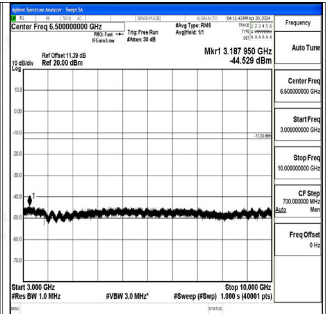
Band26_10MHz_16QAM_26915_1RB#0_3000~10000_3 000~10000
