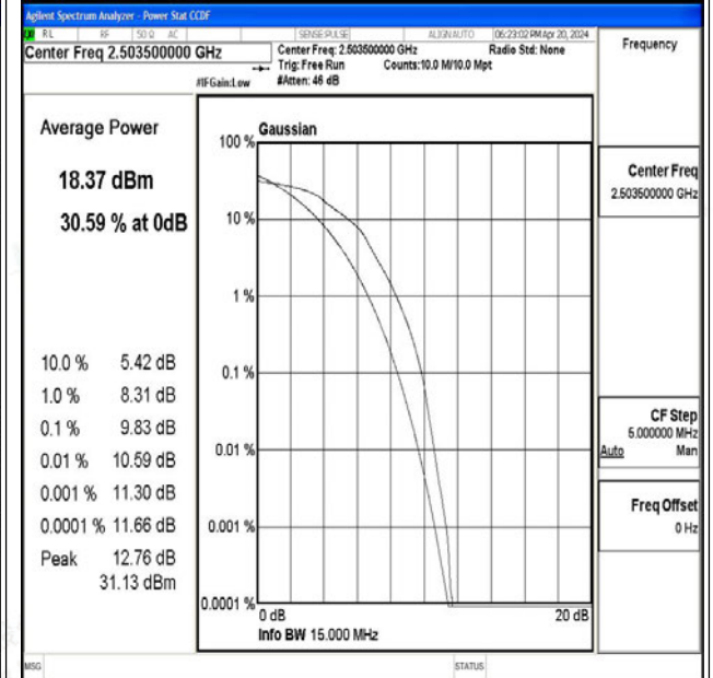
Band41-15MHz-16QAM-39725-75RB#0-PASS
