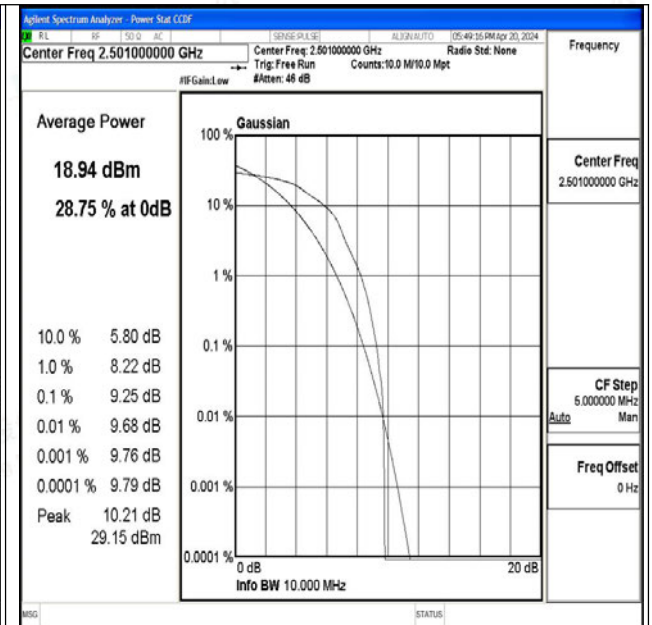
Band41-10MHz-16QAM-39700-1RB#0-PASS
