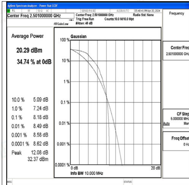
Band41-10MHz-QPSK-39700-1RB#0-PASS
