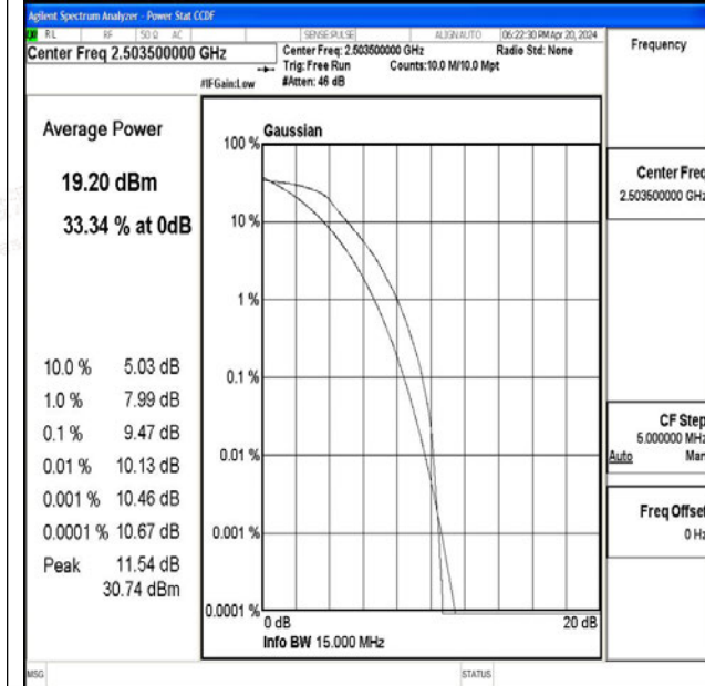
Band41-15MHz-QPSK-39725-75RB#0-PASS
