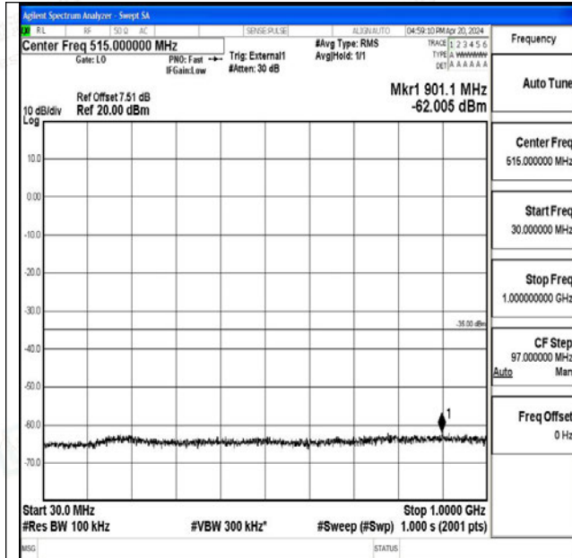
Band41_5MHz_QPSK_40620_1RB#0_30~1000_30~100
