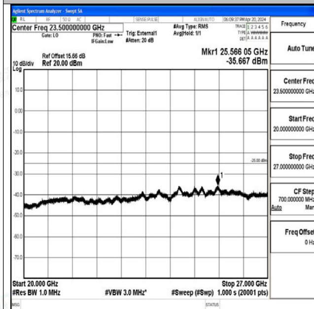
Band41_15MHz_QPSK_40620_1RB#0_20000~27000_20000~27000
