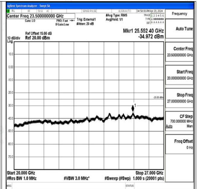
Band41_5MHz_16QAM_39675_1RB#0_20000~27000_2 0000~27000
