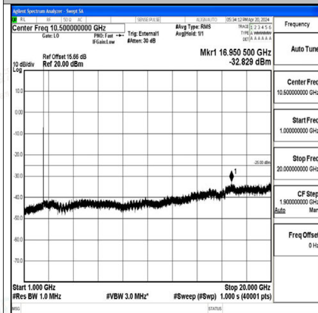
Band41_10MHz_16QAM_39700_1RB#0_1000~20000_1000~20000
