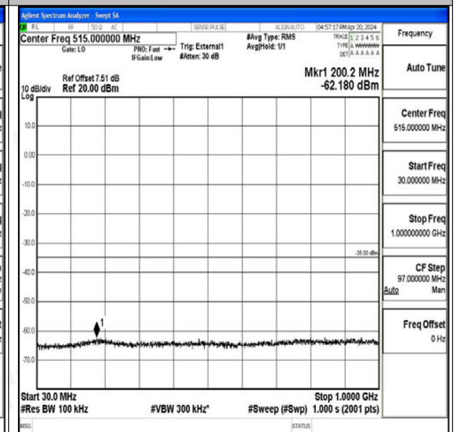
Band41_5MHz_16QAM_39675_1RB#0_30~1000_30~1000
