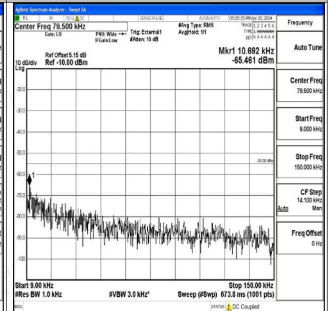
Band41_5MHz_16QAM_40620_1RB#0_0.009~0.15_0.0
