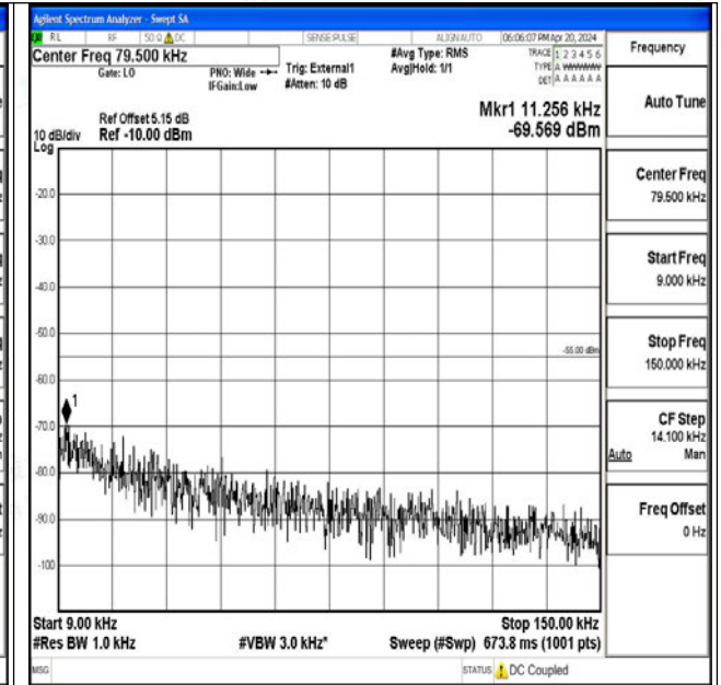
Band41_15MHz_16QAM_39725_1RB#0_0.009~0.15_0. 009~0.15
