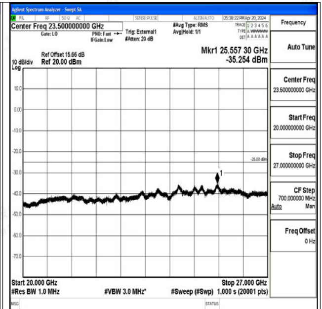
Band41_10MHz_16QAM_40620_1RB#0_20000~27000_20000~27000
