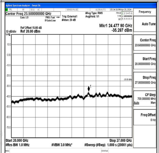
Band41_10MHz_16QAM_39700_1RB#0_20000~27000_20000~27000
