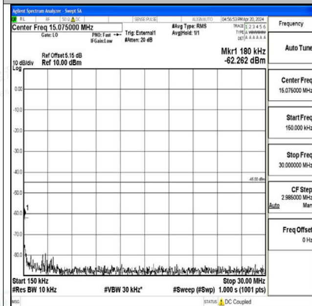
Band41_5MHz_16QAM_39675_1RB#0_0.15~30_0.15~30
