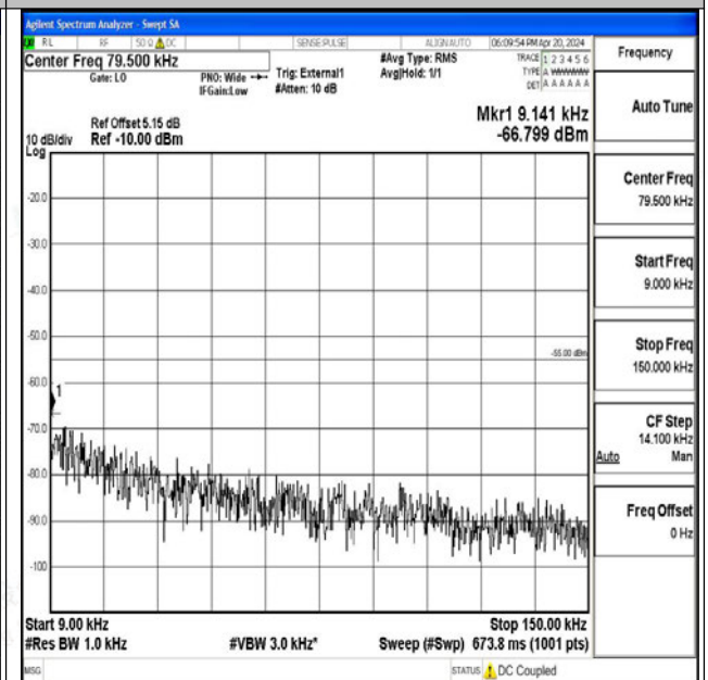
Band41_15MHz_16QAM_40620_1RB#0_0.009~0.15_0.009~0.15
