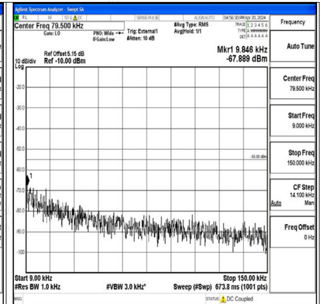
Band41_5MHz_16QAM_39675_1RB#0_0.009~0.15_0.009~0.15
