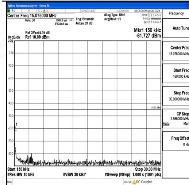
Band41_15MHz_16QAM_39725_1RB#0_0.15~30_0.15~ 30
