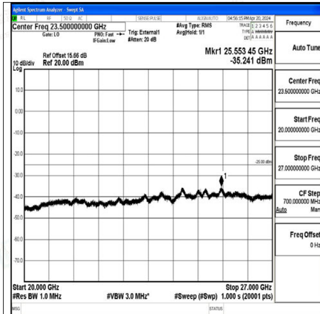
Band41_5MHz_QPSK_39675_1RB#0_20000~27000_2000~27000
