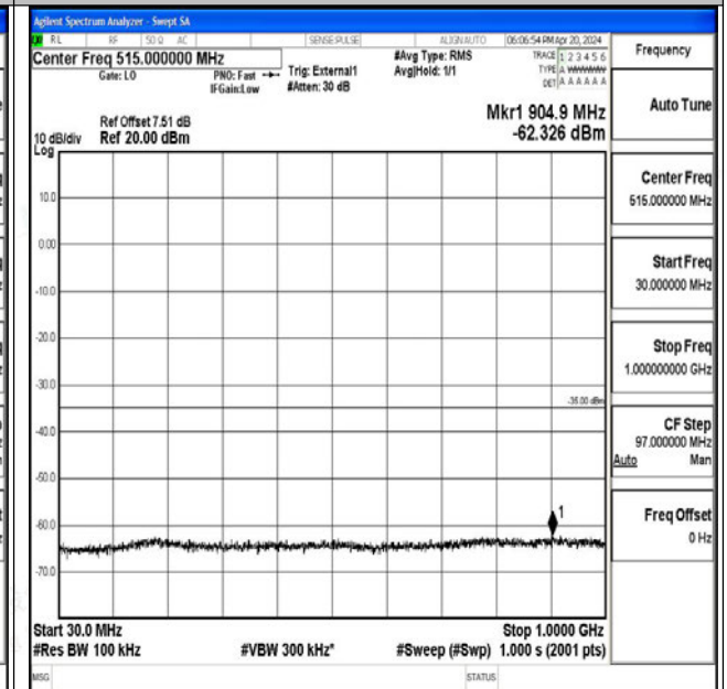
Band41_15MHz_16QAM_39725_1RB#0_30~1000_30~1 000
