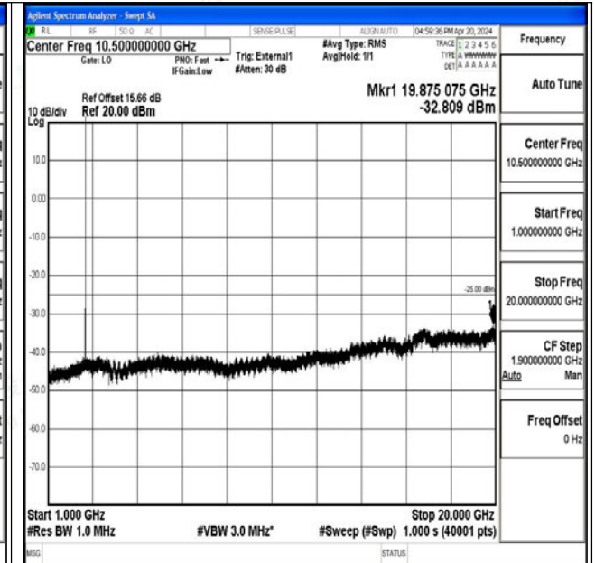
Band41_5MHz_QPSK_40620_1RB#0_1000~20000_100
