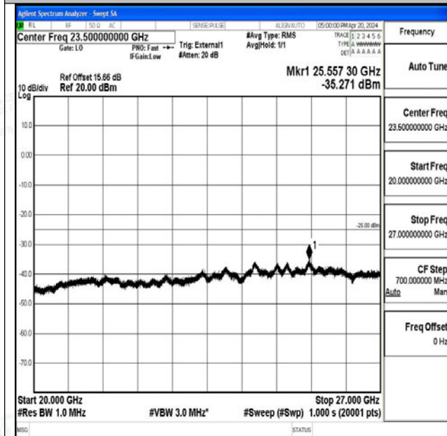
Band41_5MHz_QPSK_40620_1RB#0_20000~27000_20
