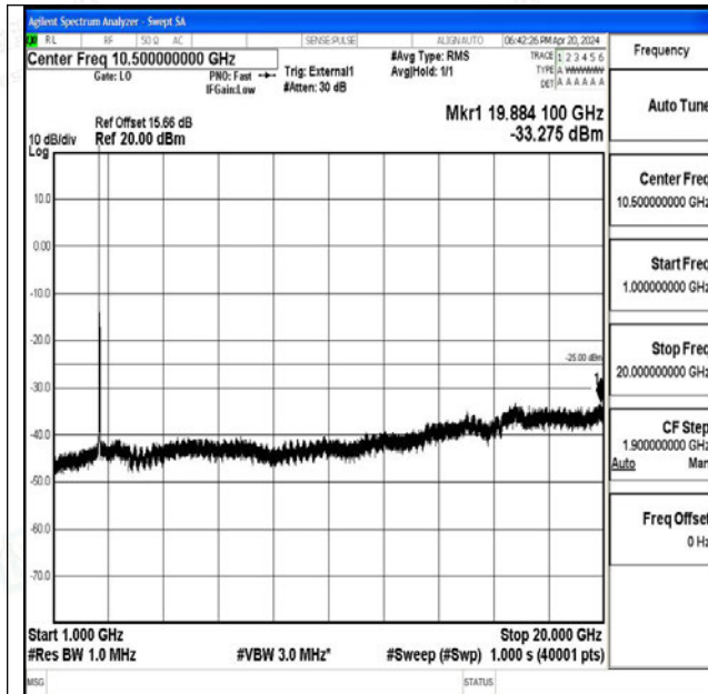
Band41_20MHz_16QAM_40620_1RB#0_1000~20000_1 000~20000
