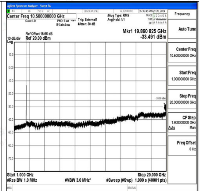
Band41_20MHz_QPSK_39750_1RB#0_1000~20000_1000~20000
