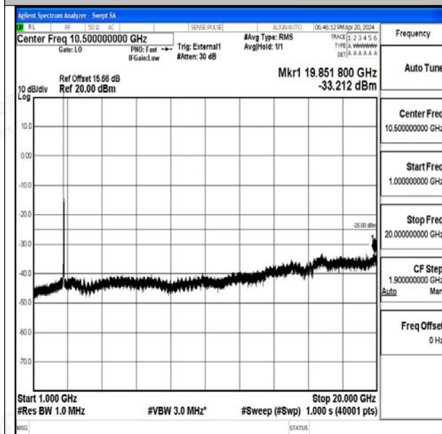
Band41_20MHz_16QAM_41490_1RB#0_1000~20000_1000~20000
