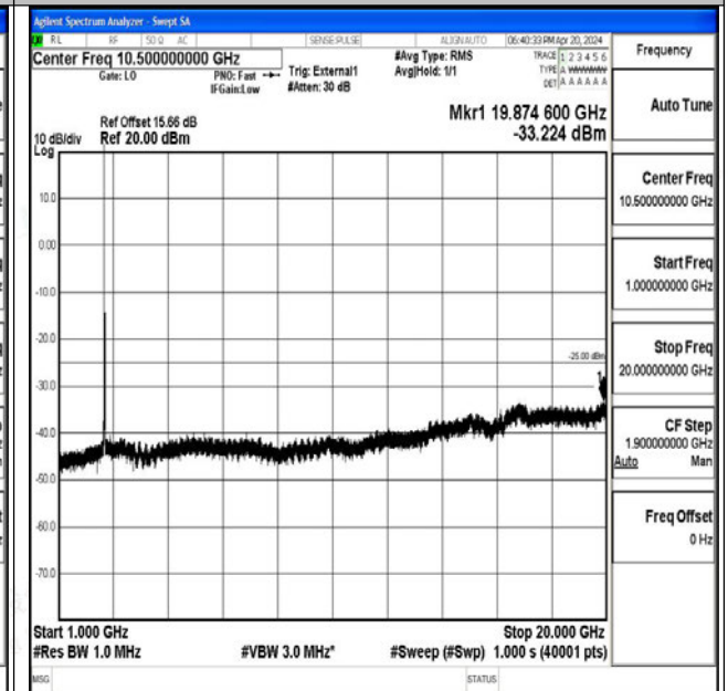
Band41_20MHz_QPSK_40620_1RB#0_1000~20000_10 00~20000
