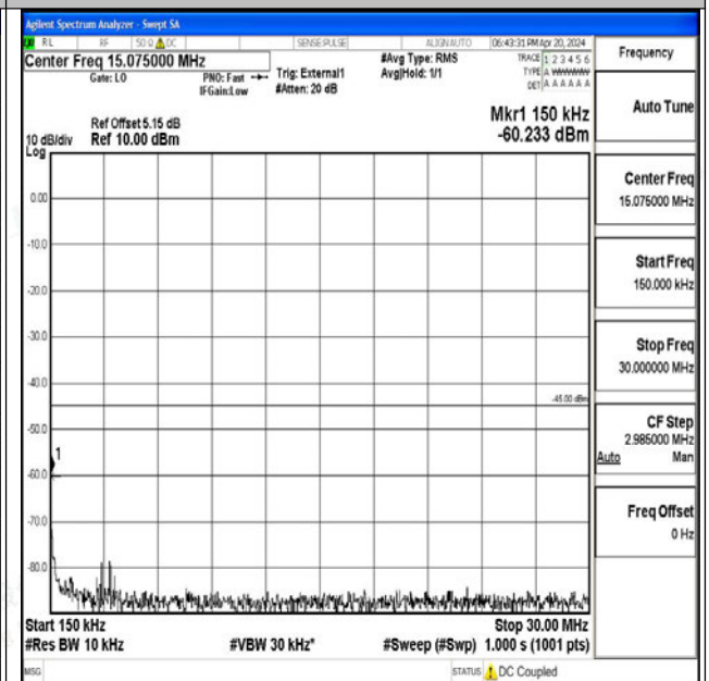
Band41_20MHz_QPSK_41490_1RB#0_0.15~30_0.15~3 0
