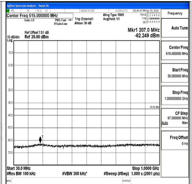
Band41_20MHz_16QAM_41490_1RB#0_30~1000_30~1000
