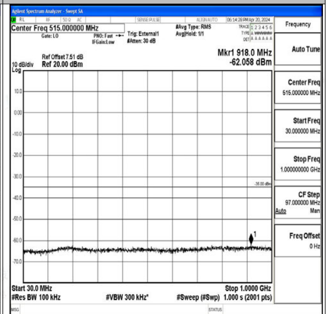
Band41_15MHz_16QAM_41515_1RB#0_30~1000_30~1 000
