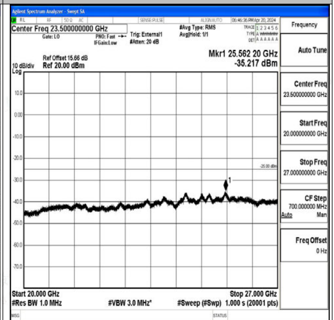
Band41_20MHz_16QAM_41490_1RB#0_20000~27000_20000~27000
