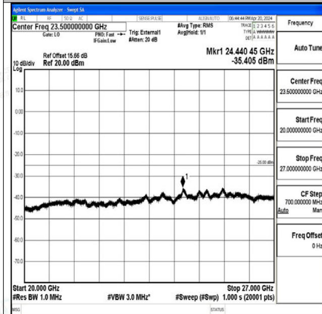
Band41_20MHz_QPSK_41490_1RB#0_20000~27000_20000~27000
