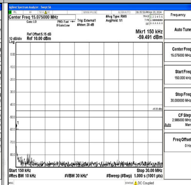
Band41_20MHz_QPSK_39750_1RB#0_0.15~30_0.15~3 0
