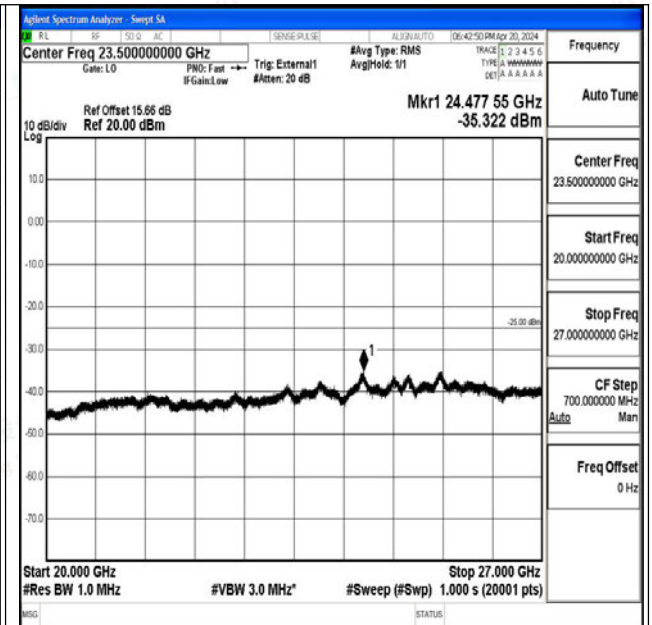
Band41_20MHz_16QAM_40620_1RB#0_20000~27000_ 20000~27000
