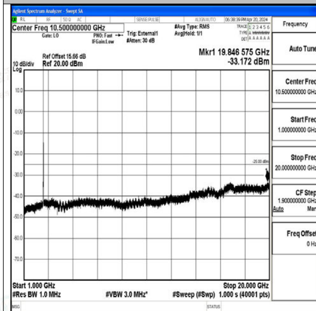
Band41_20MHz_16QAM_39750_1RB#0_1000~20000_1000~20000
