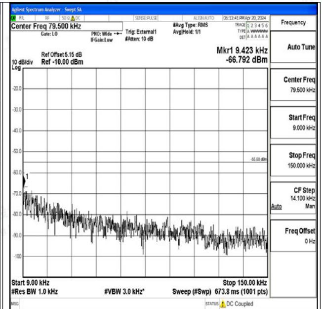
Band41_15MHz_16QAM_41515_1RB#0_0.009~0.15_0. 009~0.15
