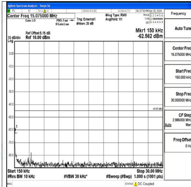
Band41_20MHz_16QAM_39750_1RB#0_0.15~30_0.15~30
