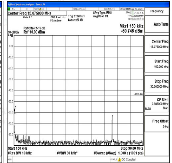
Band41_20MHz_QPSK_40620_1RB#0_0.15~30_0.15~3 0
