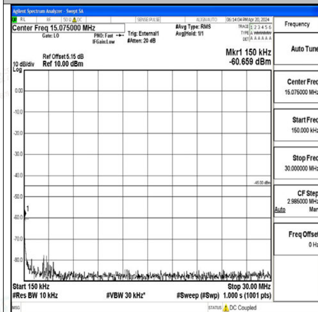
Band41_15MHz_16QAM_41515_1RB#0_0.15~30_0.15~ 30
