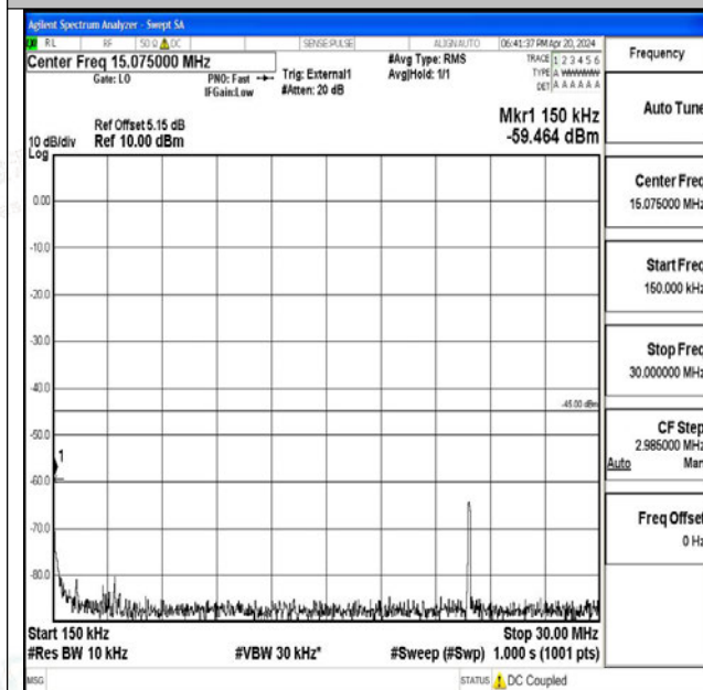
Band41_20MHz_16QAM_40620_1RB#0_0.15~30_0.15~30 30
