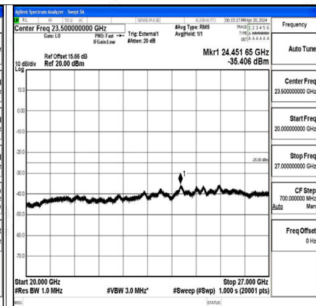
Band41_15MHz_16QAM_41515_1RB#0_20000~27000_20000~27000
