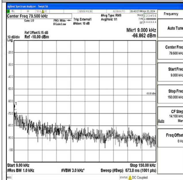
Band41_20MHz_QPSK_41490_1RB#0_0.009~0.15_0.00 9~0.15
