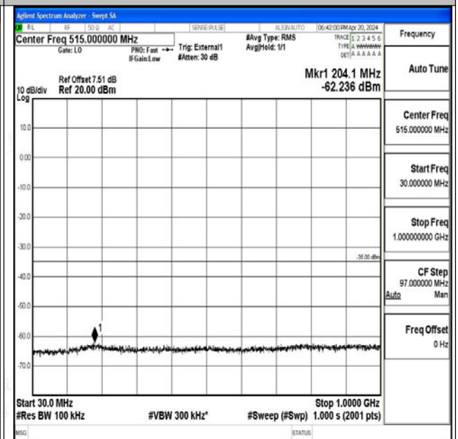
Band41_20MHz_16QAM_40620_1RB#0_30~1000_30~1000 000
