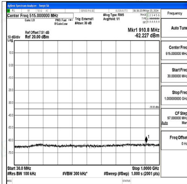
Band41_20MHz_QPSK_39750_1RB#0_30~1000_30~1000
