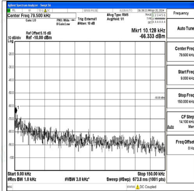
Band41_20MHz_QPSK_40620_1RB#0_0.009~0.15_0.00 9~0.15
