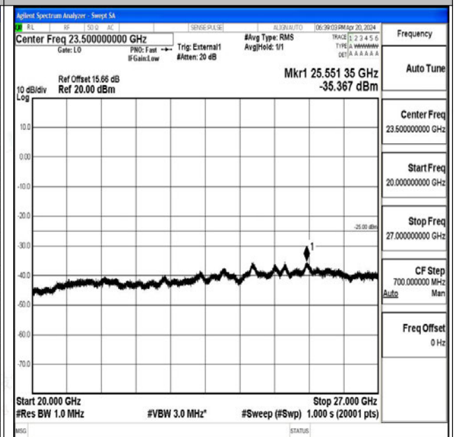
Band41_20MHz_16QAM_39750_1RB#0_20000~27000_20000~27000
