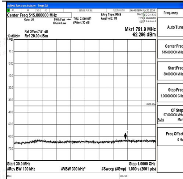
Band41_20MHz_QPSK_40620_1RB#0_30~1000_30~10 00
