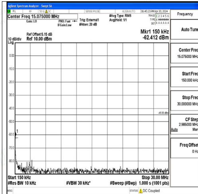
Band41_20MHz_16QAM_41490_1RB#0_0.15~30_0.15~30
