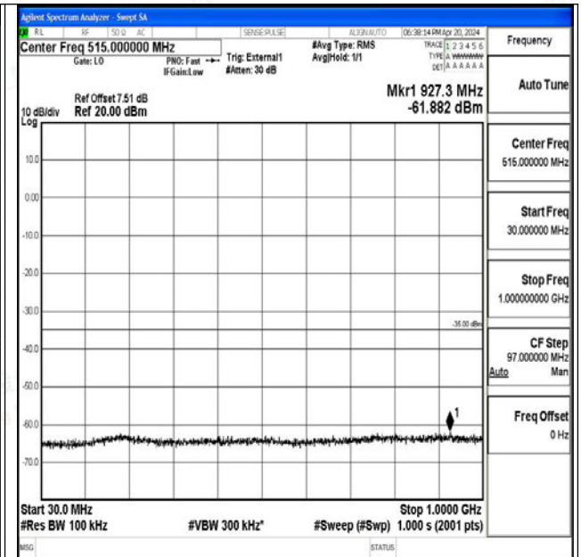
Band41_20MHz_16QAM_39750_1RB#0_30~1000_30~1000
