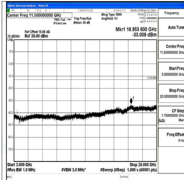
Band66_15MHz_QPSK_132047_1RB#0_3000~20000_3000~20000
