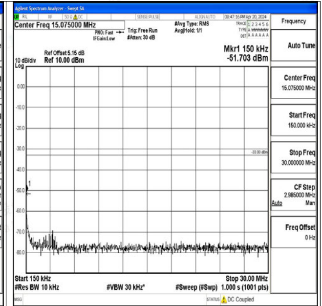
Band66_15MHz_QPSK_132597_1RB#0_0.15~30_0.15~ 30
