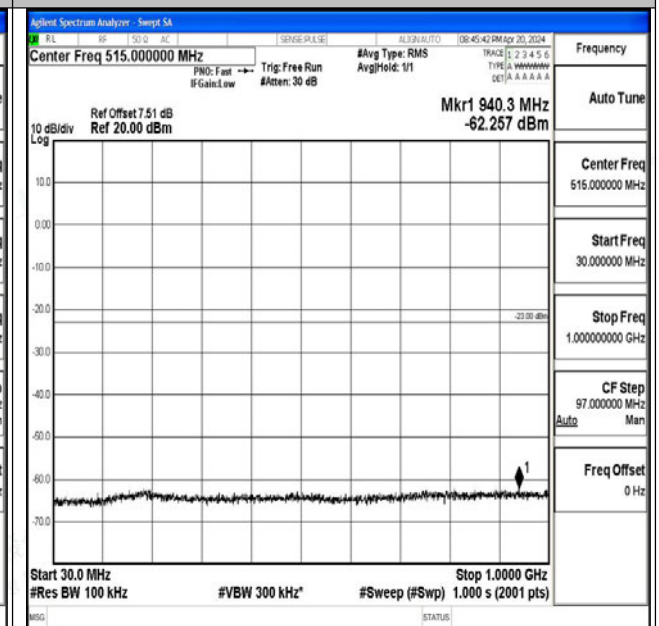
Band66_15MHz_16QAM_132047_1RB#0_30~1000_30~1000
