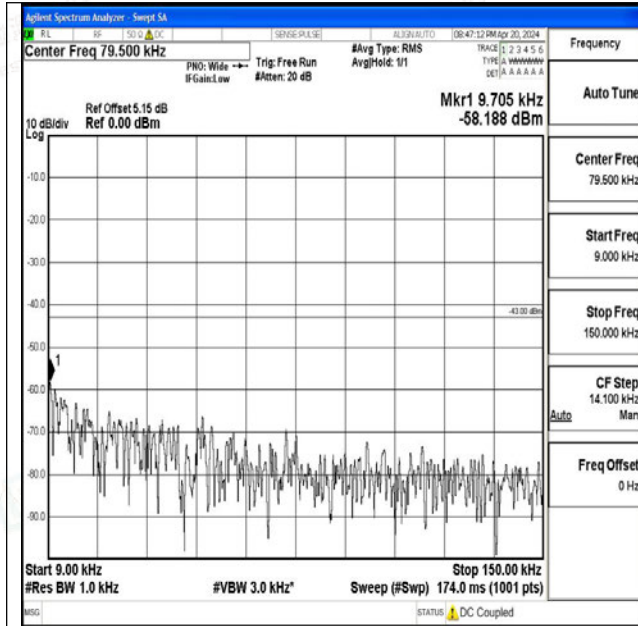
Band66_15MHz_QPSK_132597_1RB#0_0.009~0.15_0.0 09~0.15
