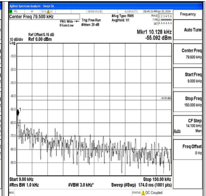
Band66_15MHz_16QAM_132047_1RB#0_0.009~0.15_0.009~0.15
