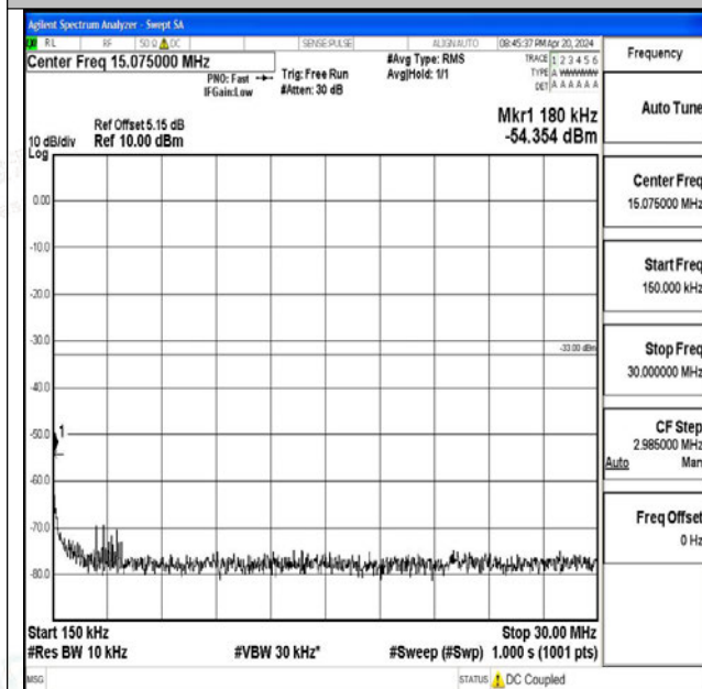
Band66_15MHz_16QAM_132047_1RB#0_0.15~30_0.15~30
