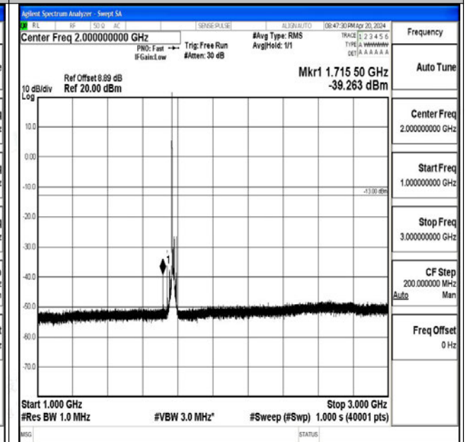
Band66_15MHz_QPSK_132597_1RB#0_1000~3000_10 00~3000
