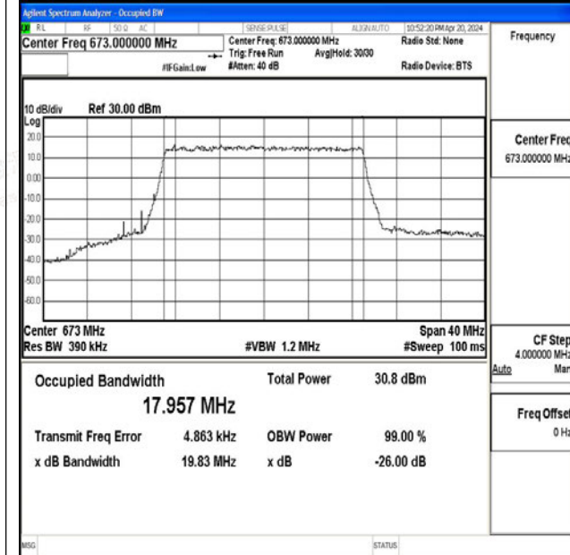
Band71-20MHz-QPSK-133222-100RB#0-PASS
