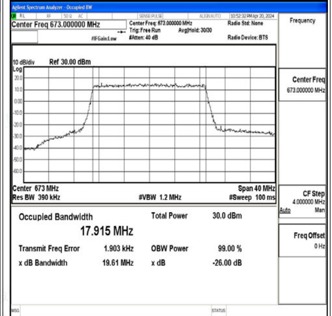
Band71-20MHz-16QAM-133222-100RB#0-PASS
