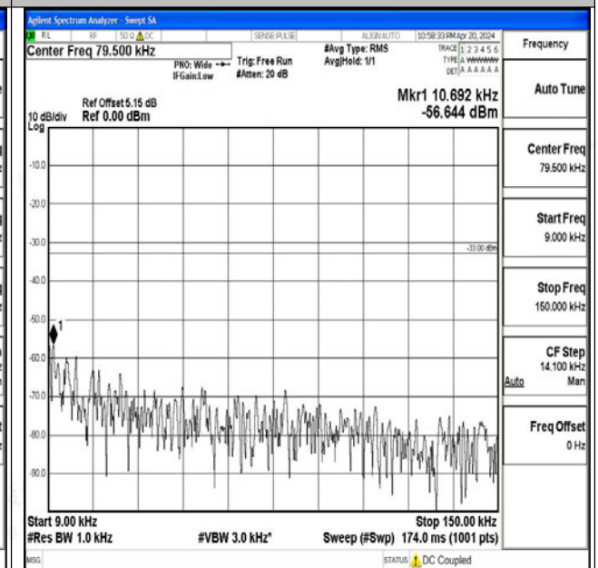
Band71_20MHz_16QAM_133322_1RB#0_0.009~0.15_0 .009~0.15
