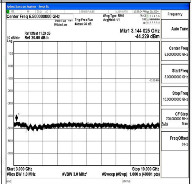
Band71_20MHz_16QAM_133322_1RB#0_3000~10000_3000~10000
