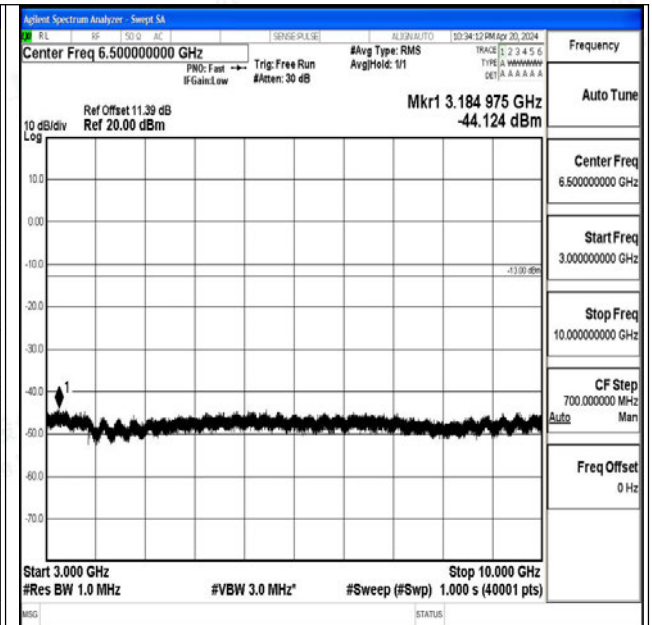
Band71_15MHz_16QAM_133397_1RB#0_3000~10000_ 3000~10000
