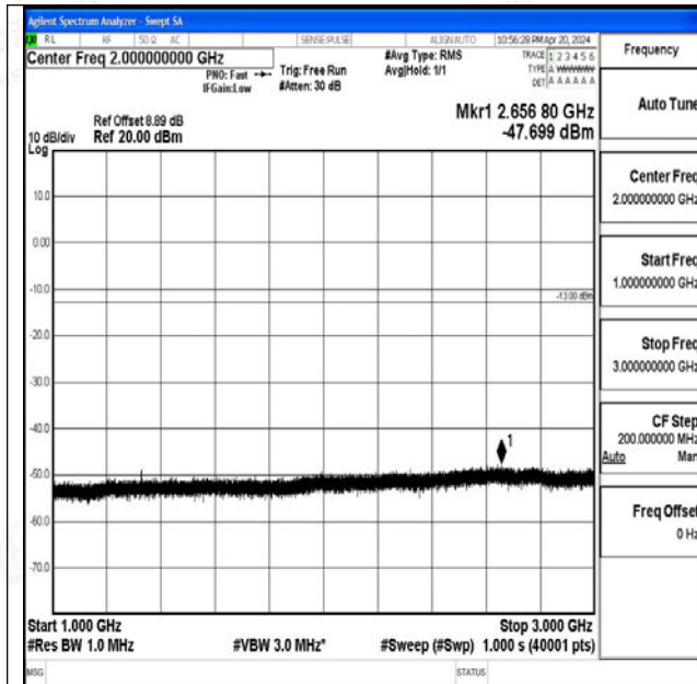
Band71_20MHz_16QAM_133222_1RB#0_1000~3000_1 000~3000
