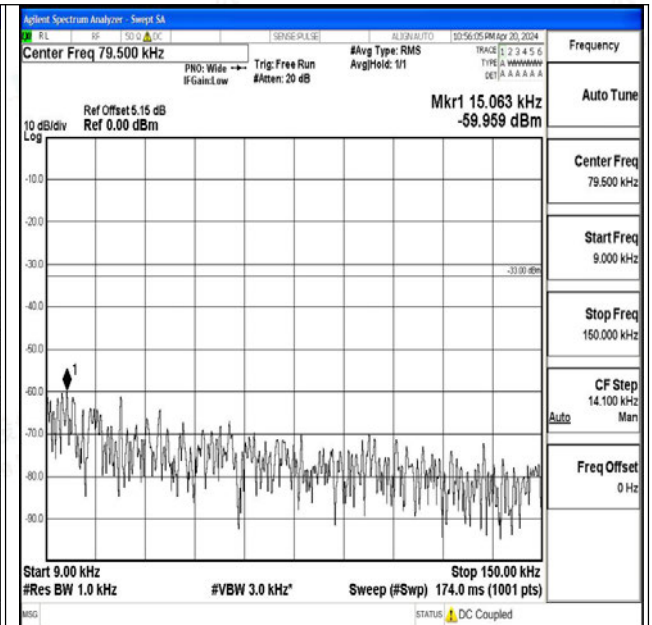
Band71_20MHz_16QAM_133222_1RB#0_0.009~0.15_0 .009~0.15
