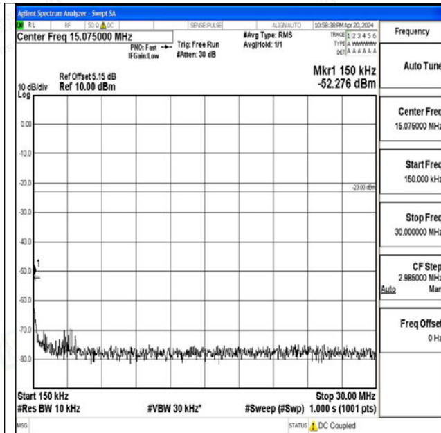
Band71_20MHz_16QAM_133322_1RB#0_0.15~30_0.15~30
