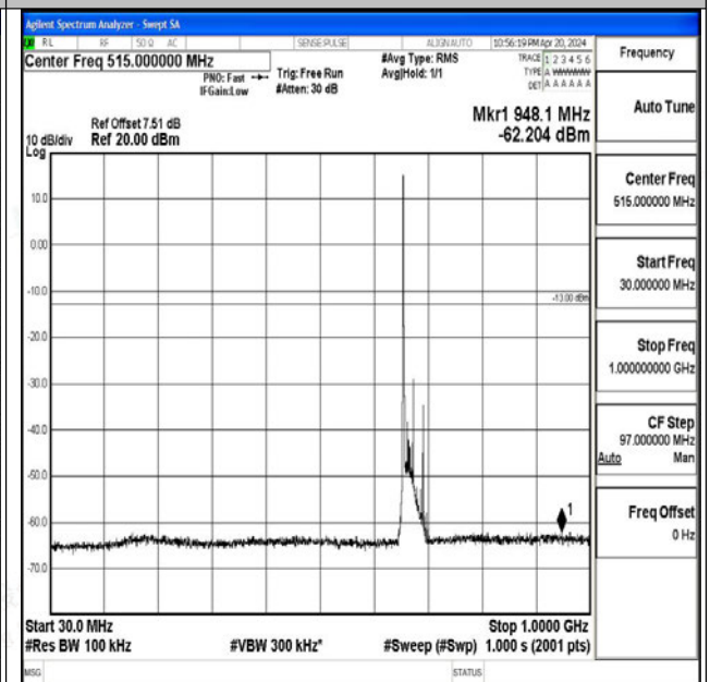
Band71_20MHz_16QAM_133222_1RB#0_30~1000_30~ 1000
