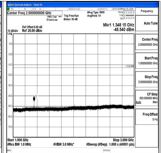
Band71_20MHz_QPSK_133322_1RB#0_1000~3000_10 00~3000
