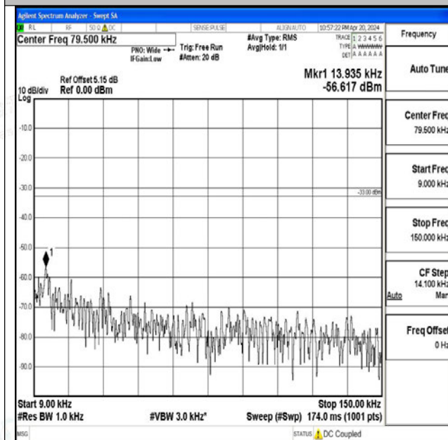
Band71_20MHz_QPSK_133322_1RB#0_0.009~0.15_0.0 09~0.15
