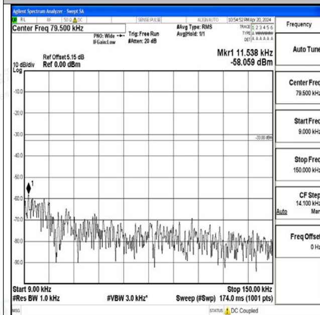
Band71_20MHz_QPSK_133222_1RB#0_0.009~0.15_0.0 09~0.15
