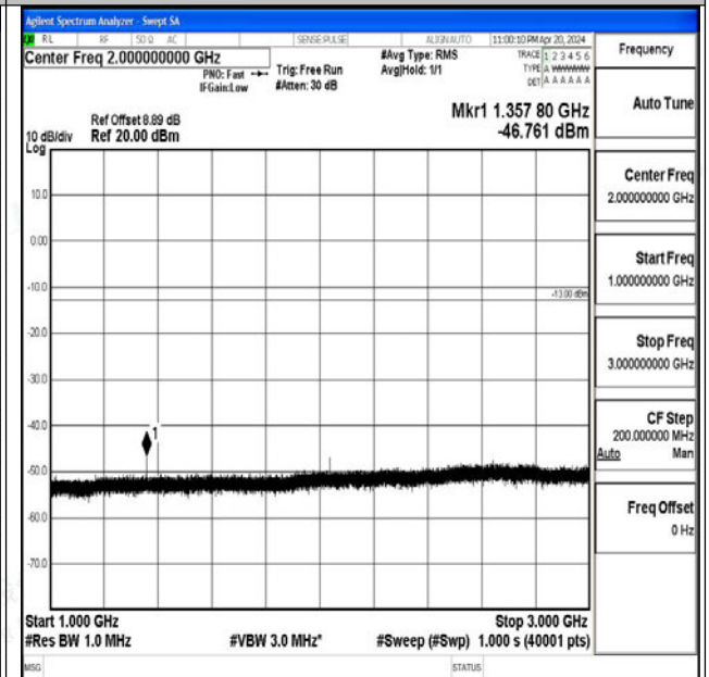
Band71_20MHz_QPSK_133372_1RB#0_1000~3000_10 00~3000
