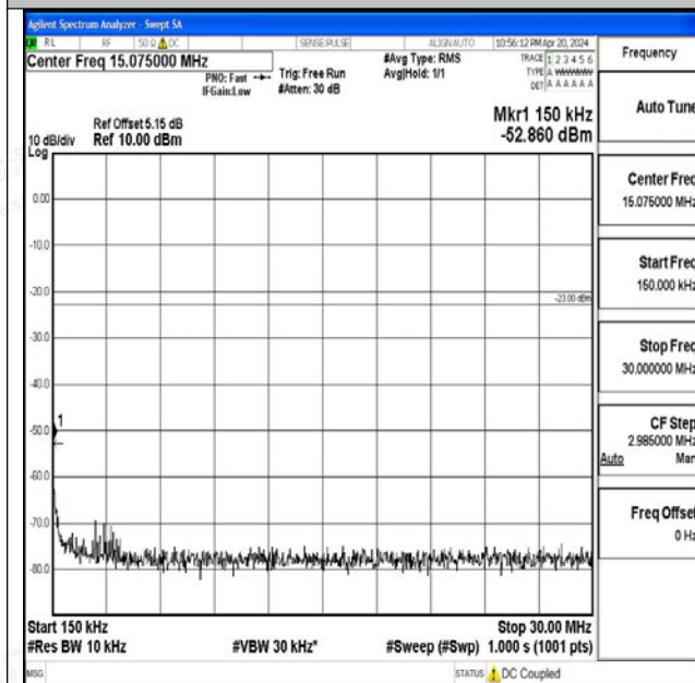
Band71_20MHz_16QAM_133222_1RB#0_0.15~30_0.15 ~30
