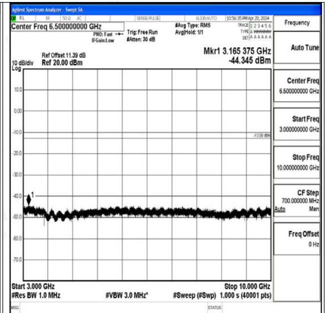
Band71_20MHz_16QAM_133222_1RB#0_3000~10000_ 3000~10000
