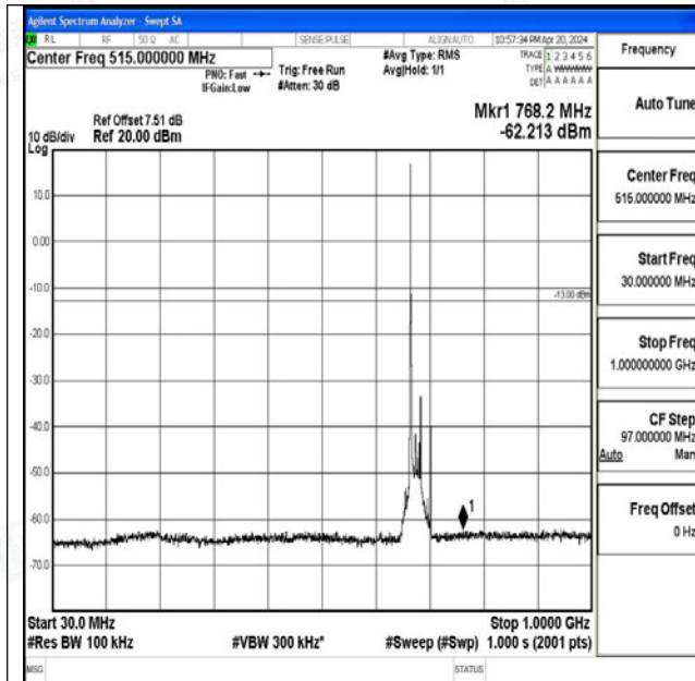
Band71_20MHz_QPSK_133322_1RB#0_30~1000_30~1 000
