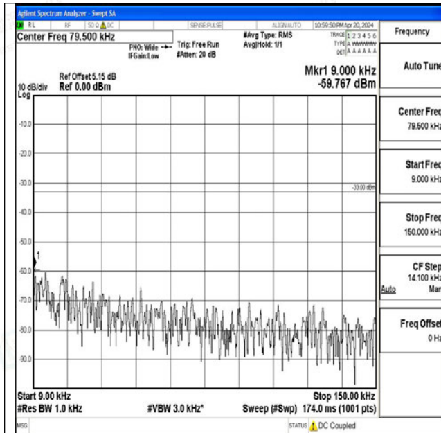
Band71_20MHz_QPSK_133372_1RB#0_0.009~0.15_0.0 09~0.15
