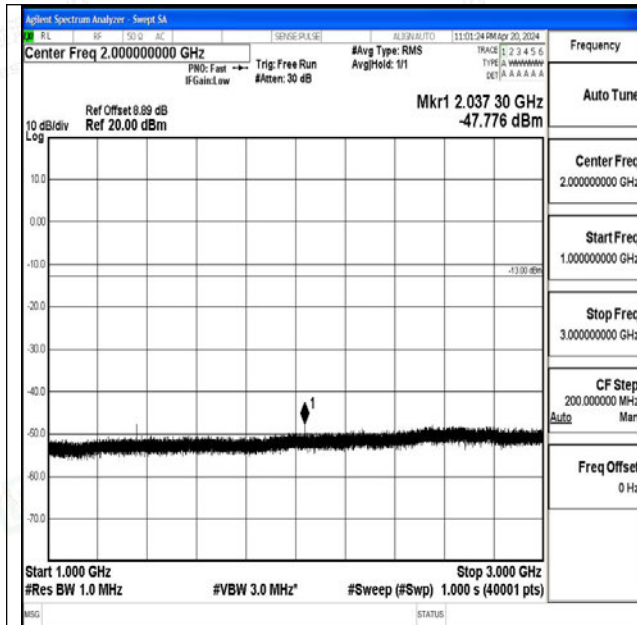
Band71_20MHz_16QAM_133372_1RB#0_1000~3000_1 000~3000
