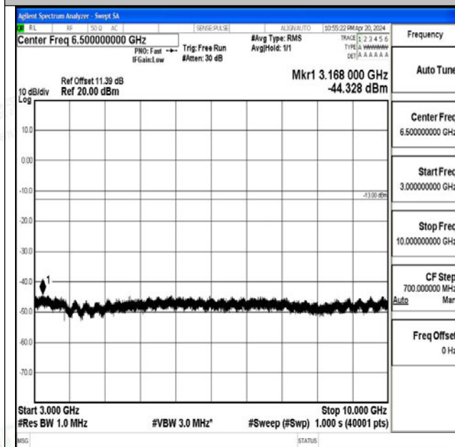
Band71_20MHz_QPSK_133222_1RB#0_3000~10000_3000~10000
