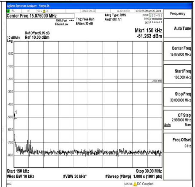
Band71_20MHz_QPSK_133372_1RB#0_0.15~30_0.15~ 30
