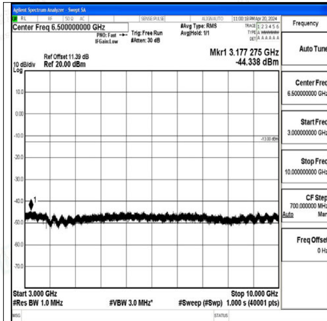
Band71_20MHz_QPSK_133372_1RB#0_3000~10000_3000~10000
