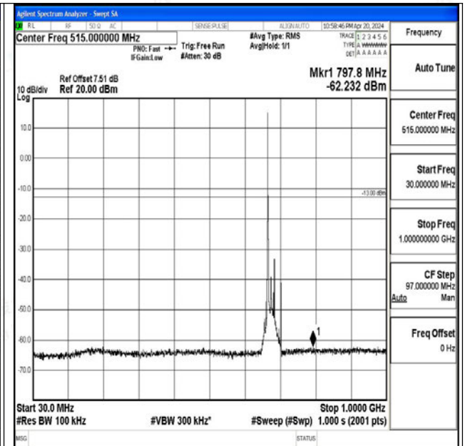
Band71_20MHz_16QAM_133322_1RB#0_30~1000_30~1000
