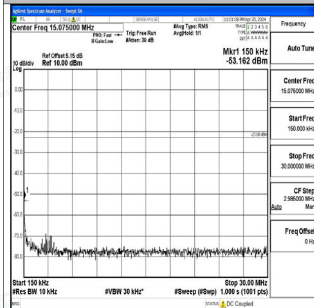
Band71_20MHz_16QAM_133372_1RB#0_0.15~30_0.15~30
