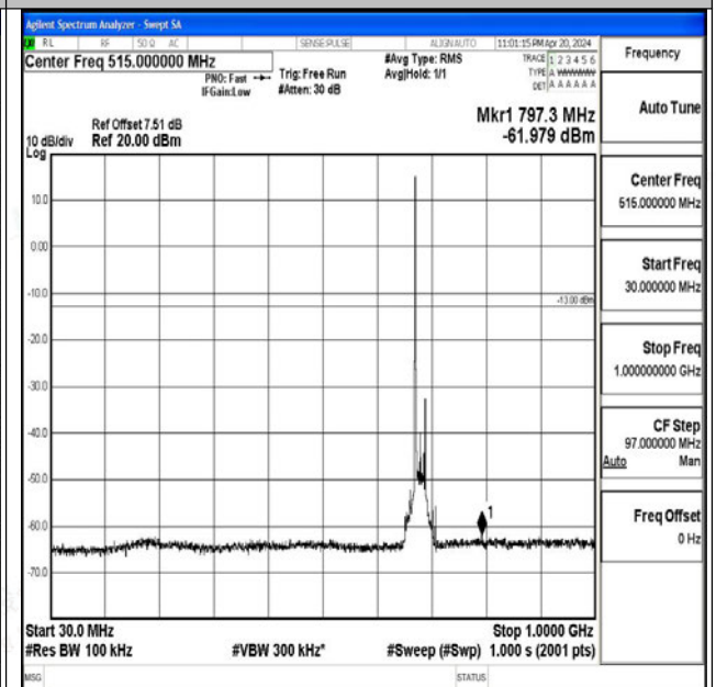
Band71_20MHz_16QAM_133372_1RB#0_30~1000_30~1000
