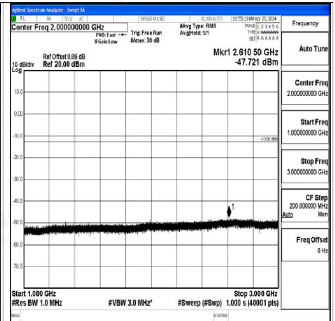
Band71_20MHz_QPSK_133222_1RB#0_1000~3000_1000~3000
