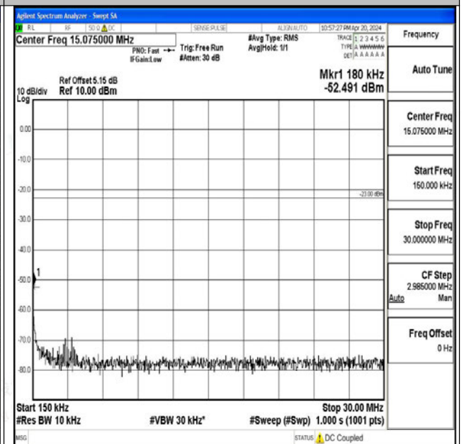
Band71_20MHz_QPSK_133322_1RB#0_0.15~30_0.15~ 30
