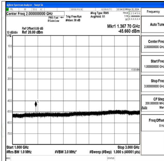
Band71_15MHz_16QAM_133397_1RB#0_1000~3000_1 000~3000
