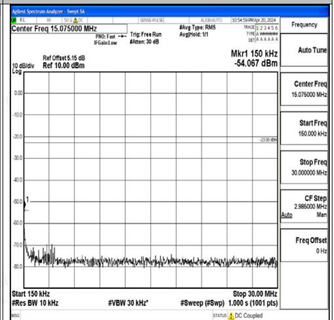
Band71_20MHz_QPSK_133222_1RB#0_0.15~30_0.15~ 30
