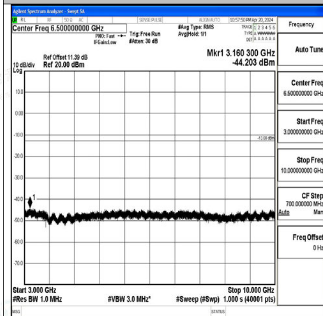
Band71_20MHz_QPSK_133322_1RB#0_3000~10000_3 000~10000
