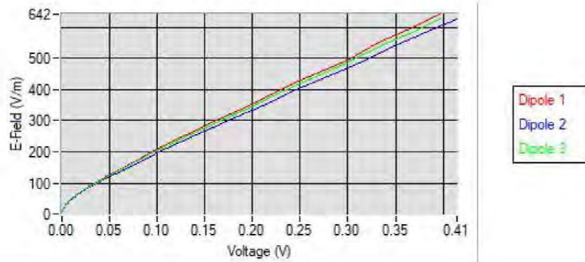
Calibration curves
