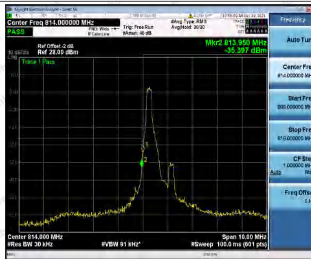
Band26-1.4MHz-QPSK-26697-1RB#5
