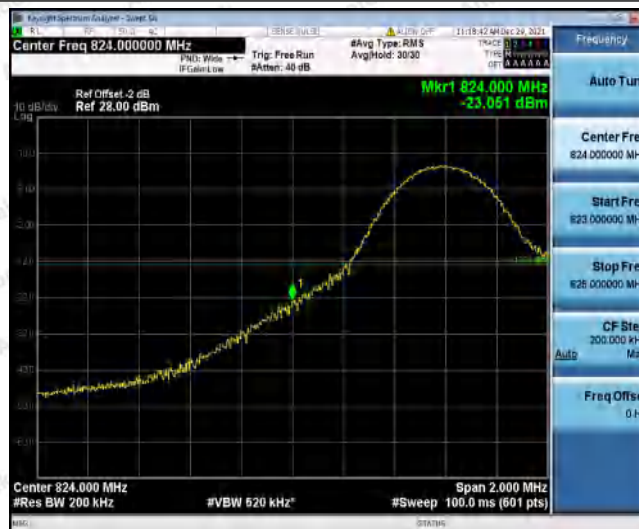
Band26-10MHz-16QAM-26840-1RB#49
