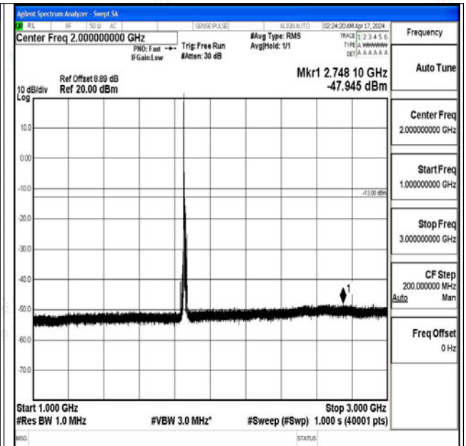
Band2_10MHz_QPSK_18650_1RB#0_1000~3000_1000 ~3000
