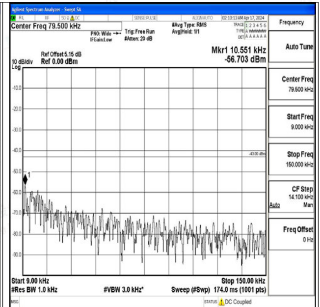
Band2_5MHz_16QAM_19175_1RB#0_0.009~0.15_0.00 9~0.15
