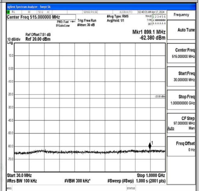
Band2_15MHz_16QAM_18675_1RB#0_30~1000_30~10 00
