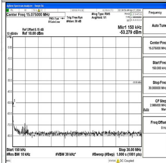
Band2_15MHz_16QAM_18675_1RB#0_0.15~30_0.15~3 0
