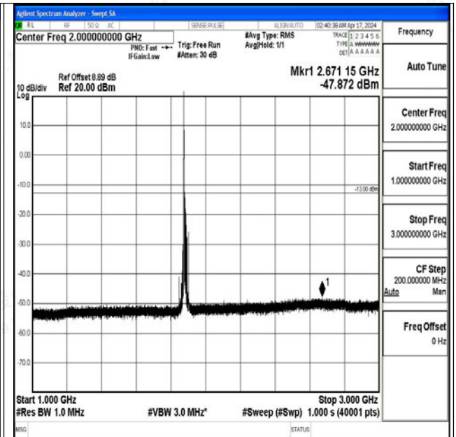
Band2_15MHz_QPSK_18900_1RB#0_1000~3000_1000 ~3000
