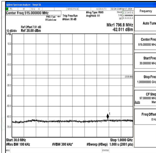
Band2_10MHz_QPSK_18650_1RB#0_30~1000_30~1000 0
