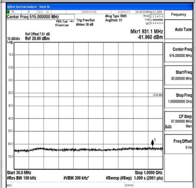
Band2_5MHz_16QAM_19175_1RB#0_30~1000_30~100 0
