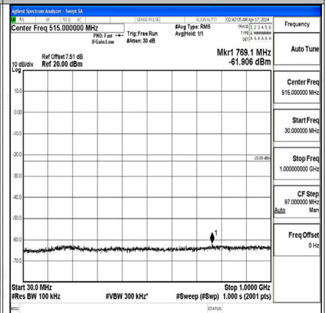
Band2_15MHz_16QAM_19125_1RB#0_30~1000_30~10 00
