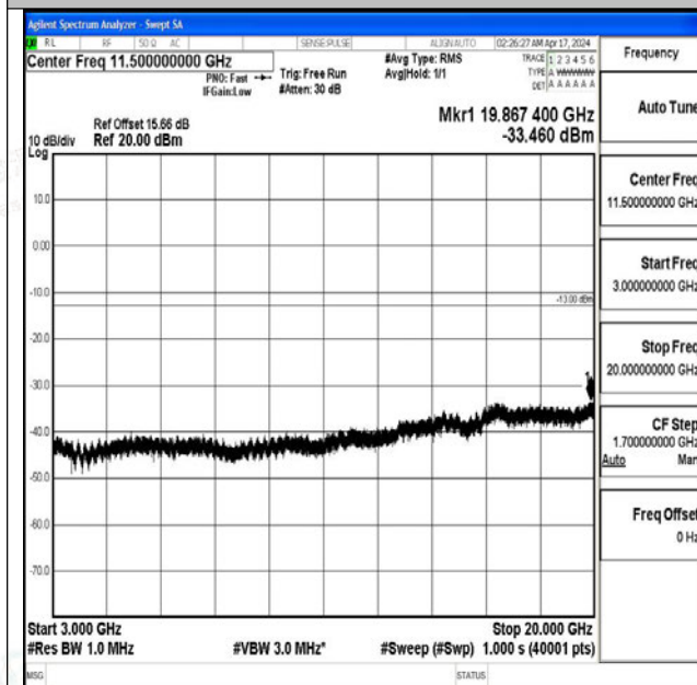
Band2_10MHz_QPSK_19150_1RB#0_3000~20000_300 0~20000
