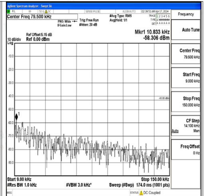
Band2_15MHz_16QAM_18675_1RB#0_0.009~0.15_0.0 09~0.15
