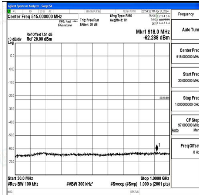
Band2_20MHz_QPSK_18700_1RB#0_30~1000_30~1000 0
