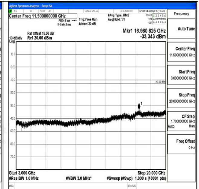
Band2_15MHz_16QAM_18675_1RB#0_3000~20000_30 00~20000
