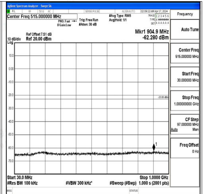
Band2_5MHz_16QAM_18900_1RB#0_30~1000_30~1000 0
