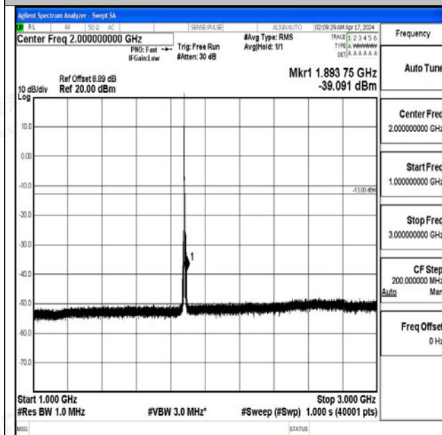
Band2_5MHz_16QAM_18900_1RB#0_1000~3000_1000~3000
