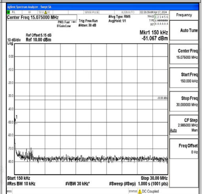
Band2_10MHz_QPSK_19150_1RB#0_0.15~30_0.15~30
