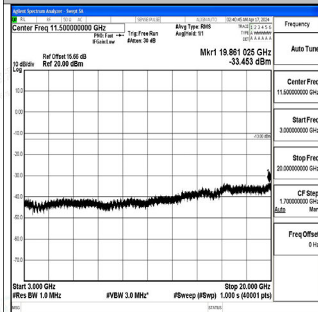
Band2_15MHz_QPSK_18900_1RB#0_3000~20000_300 0~20000
