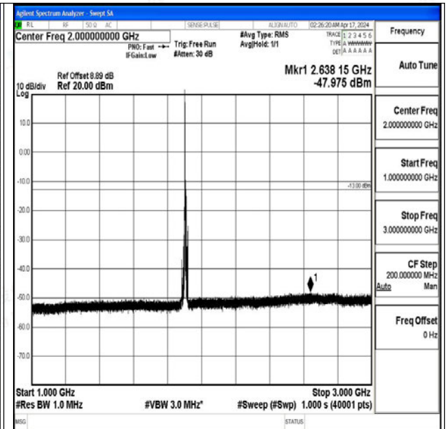
Band2_10MHz_QPSK_19150_1RB#0_1000~3000_1000 ~3000
