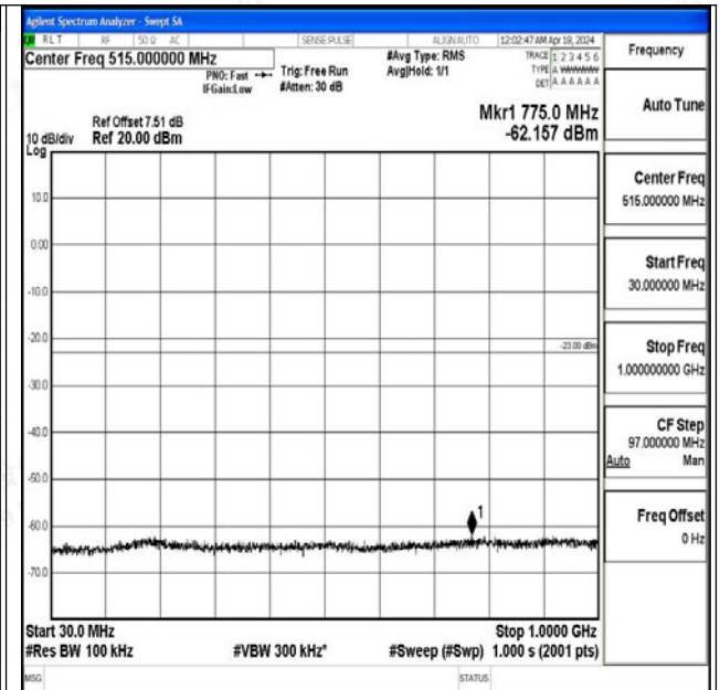
Band2_3MHz_16QAM_19185_1RB#0_30~1000_30~1000
