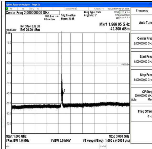
Band2_5MHz_QPSK_18625_1RB#0_1000~3000_1000~3000
