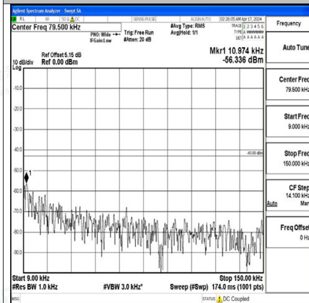
Band2_10MHz_QPSK_19150_1RB#0_0.009~0.15_0.009 ~0.15
