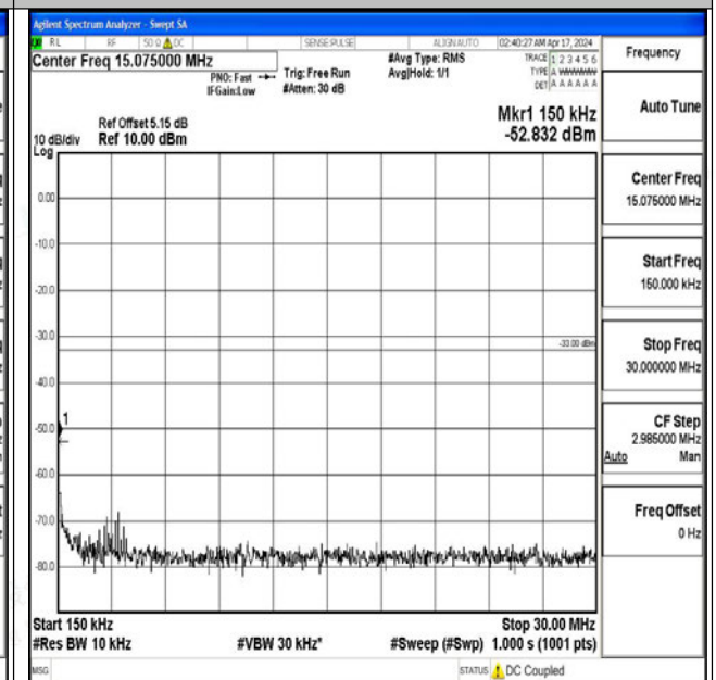
Band2_15MHz_QPSK_18900_1RB#0_0.15~30_0.15~30
