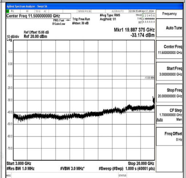
Band2_5MHz_16QAM_18900_1RB#0_3000~20000_3000~20000
