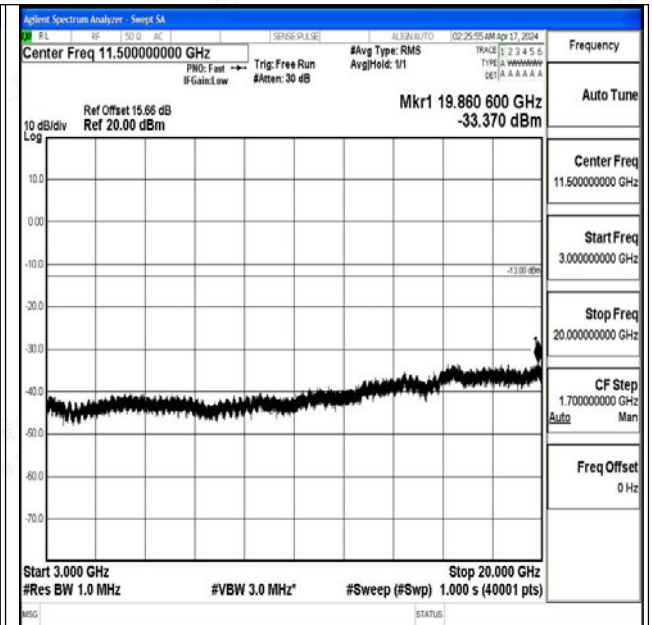
Band2_10MHz_16QAM_18900_1RB#0_3000~20000_30 00~20000
