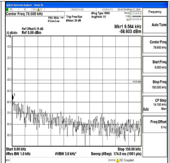
Band2_15MHz_16QAM_19125_1RB#0_0.009~0.15_0.0 09~0.15
