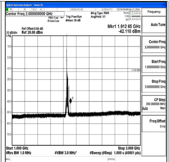
Band2_20MHz_QPSK_18700_1RB#0_1000~3000_1000~3000
