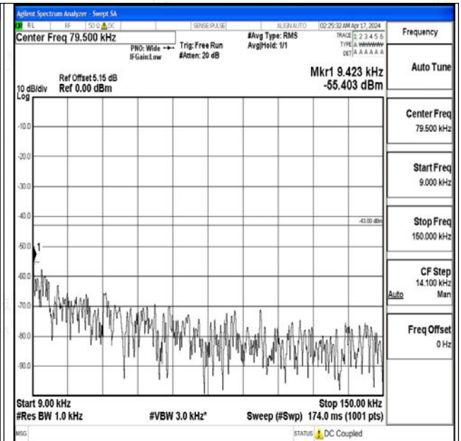
Band2_10MHz_16QAM_18900_1RB#0_0.009~0.15_0.0 09~0.15
