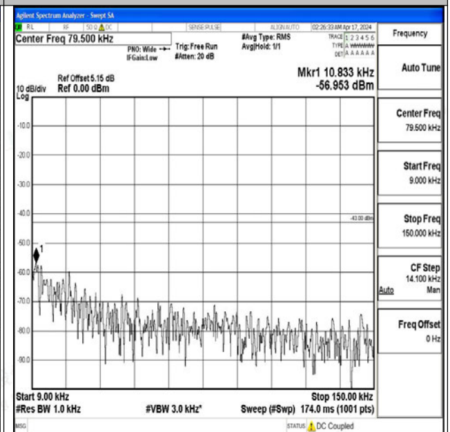
Band2_10MHz_16QAM_19150_1RB#0_0.009~0.15_0.0 09~0.15
