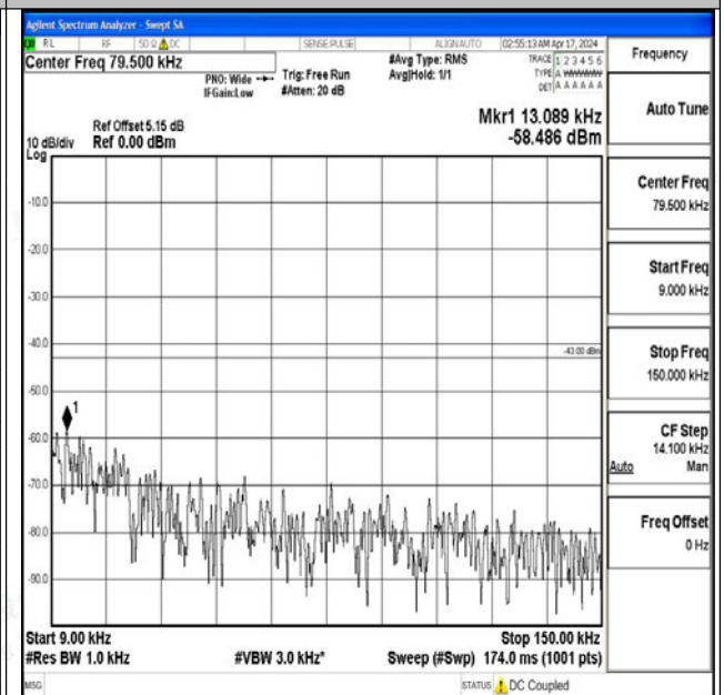
Band2_20MHz_16QAM_18700_1RB#0_0.009~0.15_0.009~0.15
