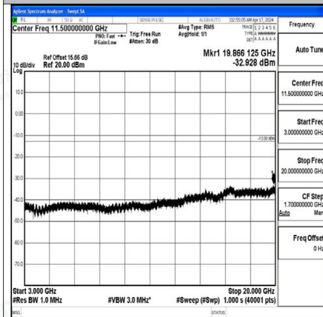
Band2_20MHz_QPSK_18700_1RB#0_3000~20000_3000~20000
