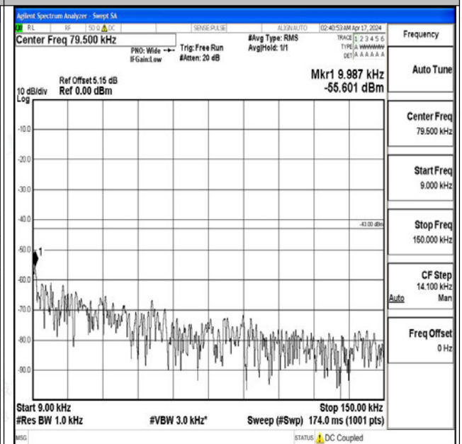
Band2_15MHz_16QAM_18900_1RB#0_0.009~0.15_0.0 09~0.15
