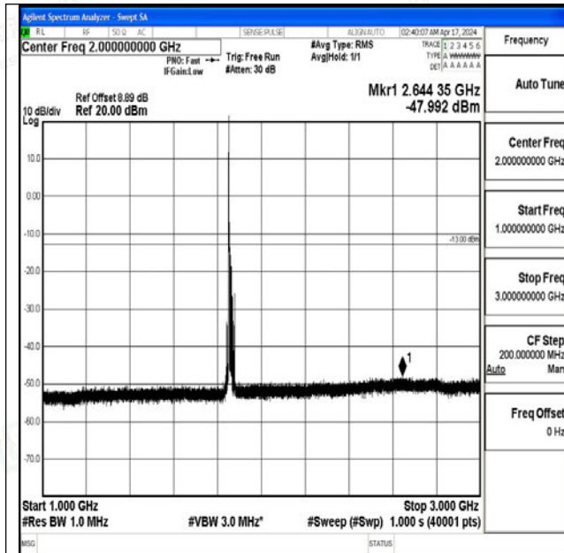
Band2_15MHz_16QAM_18675_1RB#0_1000~3000_100 0~3000
