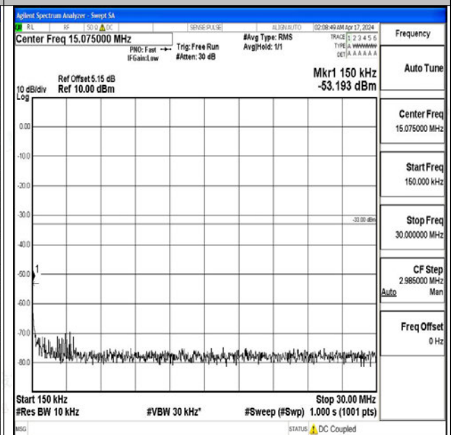
Band2_5MHz_QPSK_18900_1RB#0_0.15~30_0.15~30
