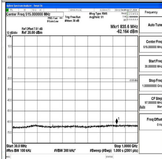
Band4_1.4MHz_QPSK_20393_1RB#0_30~1000_30~100 0
