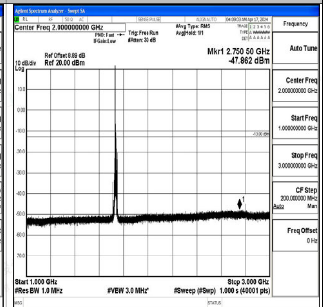
Band4_10MHz_QPSK_20175_1RB#0_1000~3000_1000~3000
