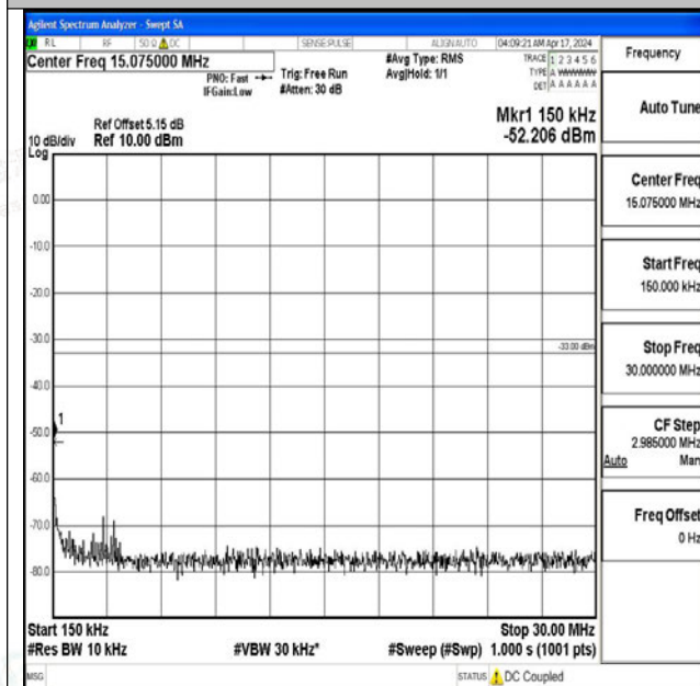
Band4_10MHz_16QAM_20175_1RB#0_0.15~30_0.15~3 0
