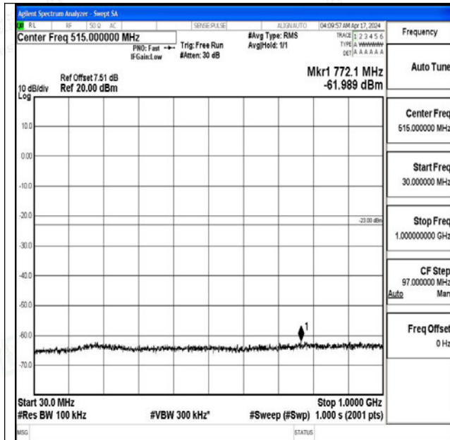
Band4_10MHz_QPSK_20350_1RB#0_30~1000_30~100 0
