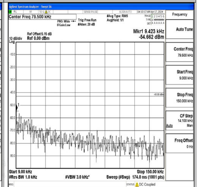
Band4_10MHz_16QAM_20350_1RB#0_0.009~0.15_0.0 09~0.15
