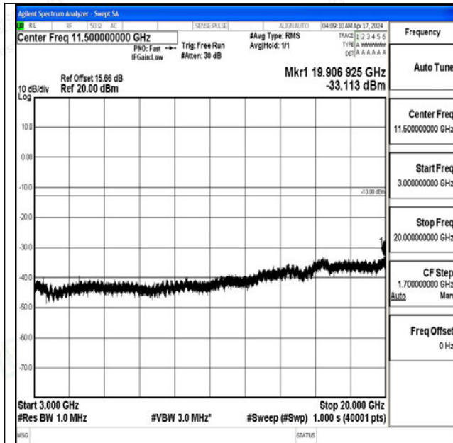
Band4_10MHz_QPSK_20175_1RB#0_3000~20000_300 0~20000
