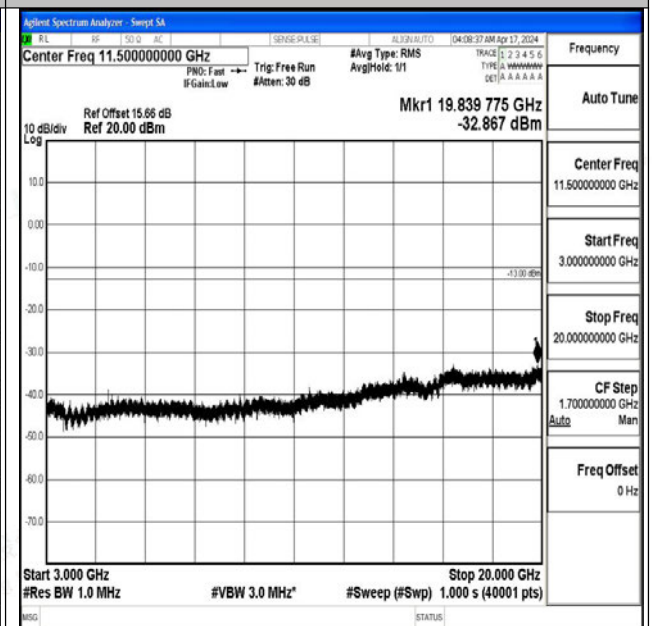
Band4_10MHz_16QAM_20000_1RB#0_3000~20000_30
