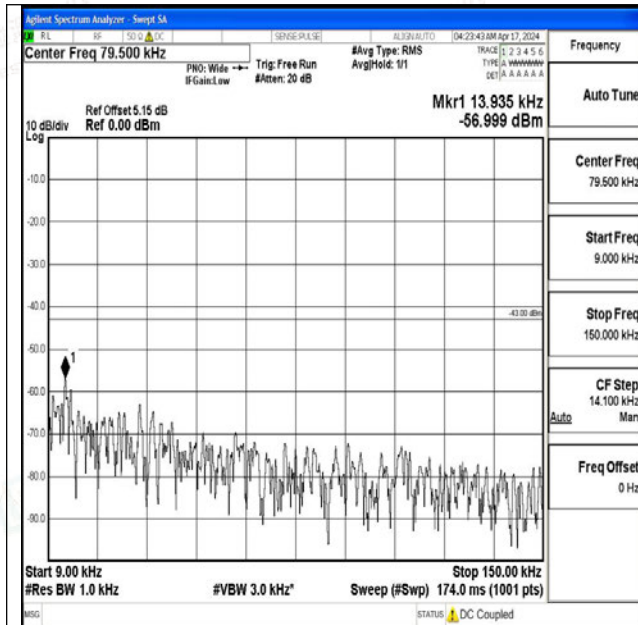
Band4_15MHz_QPSK_20025_1RB#0_0.009~0.15_0.009~0.15
