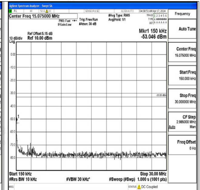
Band4_10MHz_QPSK_20175_1RB#0_0.15~30_0.15~30
