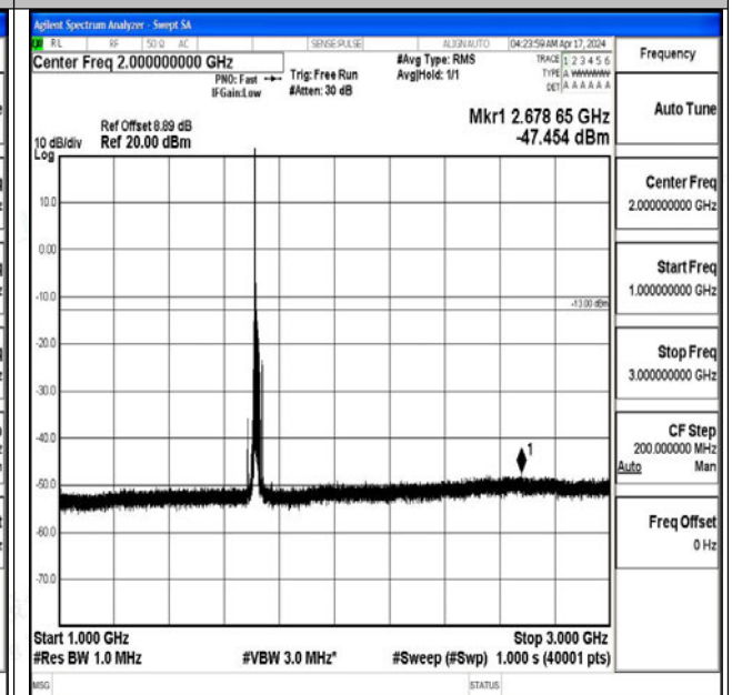
Band4_15MHz_QPSK_20025_1RB#0_1000~3000_1000~3000
