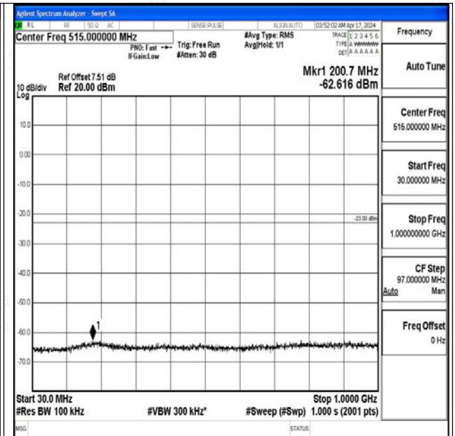
Band4_5MHz_16QAM_20175_1RB#0_30~1000_30~100
