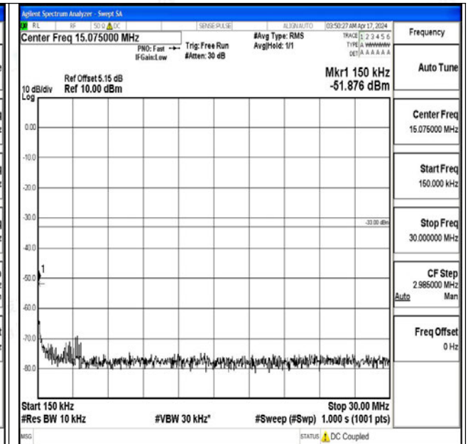
Band4_5MHz_QPSK_19975_1RB#0_0.15~30_0.15~30
