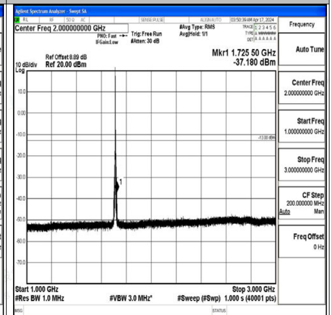
Band4_5MHz_QPSK_19975_1RB#0_1000~3000_1000~3000
