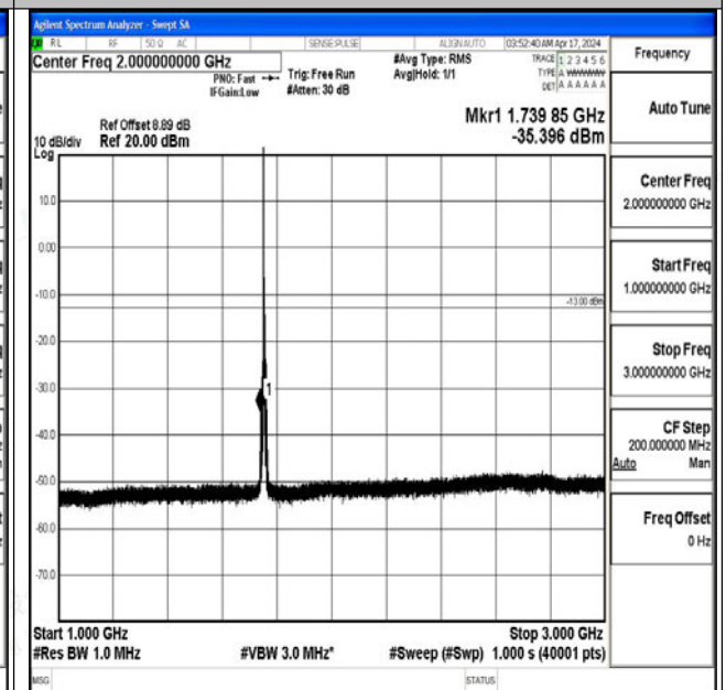
Band4_5MHz_QPSK_20375_1RB#0_1000~3000_1000~3000
