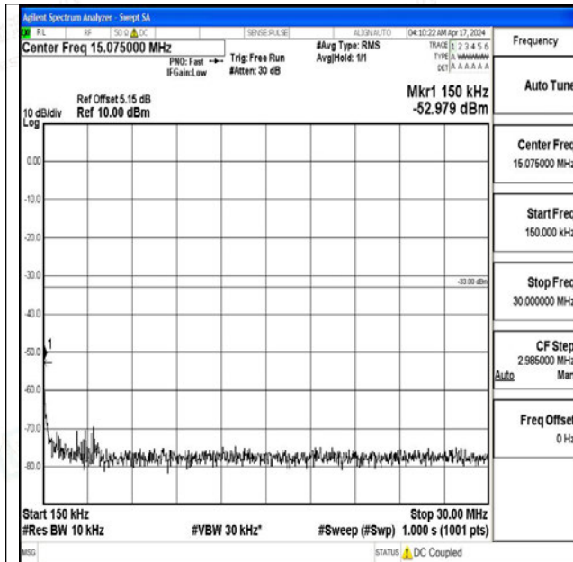
Band4_10MHz_16QAM_20350_1RB#0_0.15~30_0.15~3
