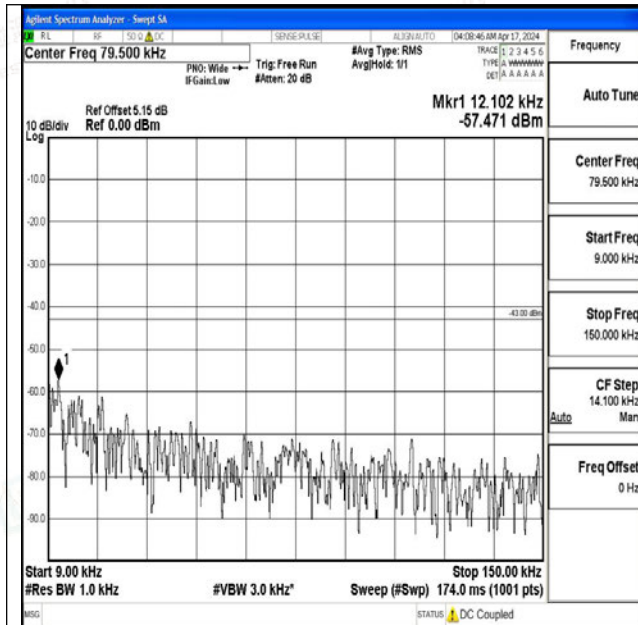
Band4_10MHz_QPSK_20175_1RB#0_0.009~0.15_0.009~0.15
