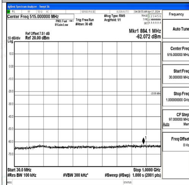
Band4_10MHz_QPSK_20175_1RB#0_30~1000_30~1000
