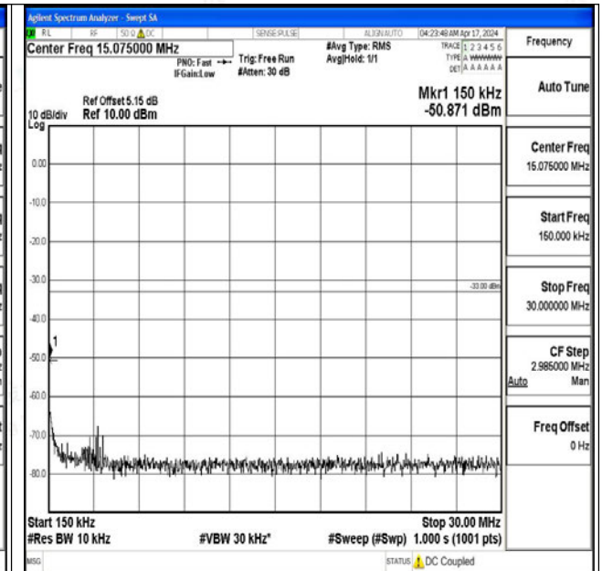
Band4_15MHz_QPSK_20025_1RB#0_0.15~30_0.15~30
