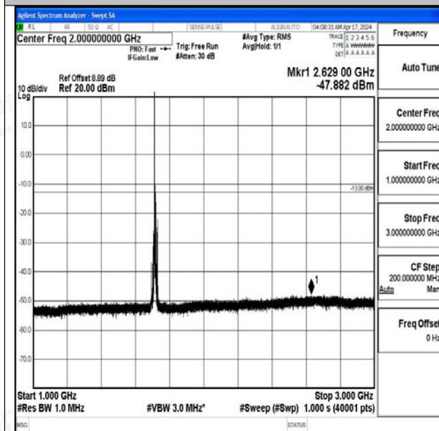
Band4_10MHz_16QAM_20000_1RB#0_1000~3000_100
