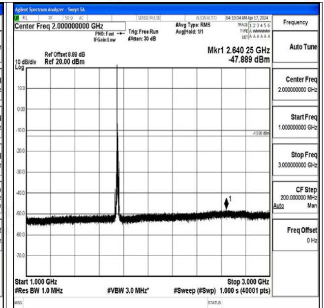
Band4_10MHz_QPSK_20350_1RB#0_1000~3000_1000 ~3000
