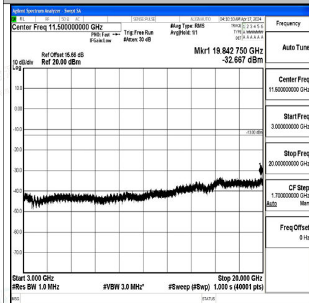
Band4_10MHz_QPSK_20350_1RB#0_3000~20000_300 0~20000
