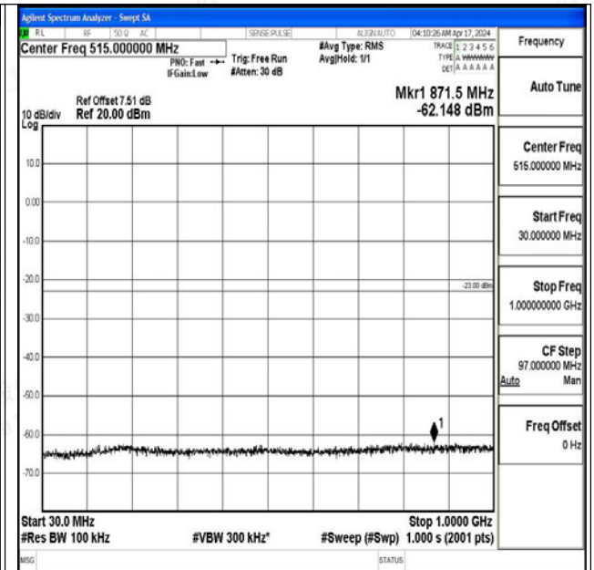
Band4_10MHz_16QAM_20350_1RB#0_30~1000_30~10
