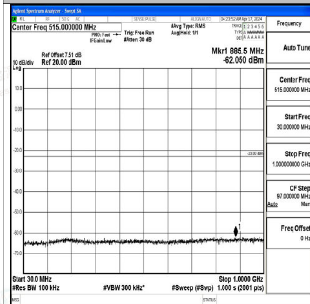
Band4_15MHz_QPSK_20025_1RB#0_30~1000_30~1000
