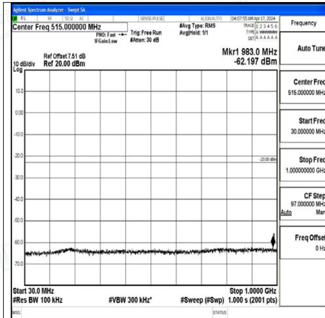
Band4_10MHz_QPSK_20000_1RB#0_30~1000_30~1000 0
