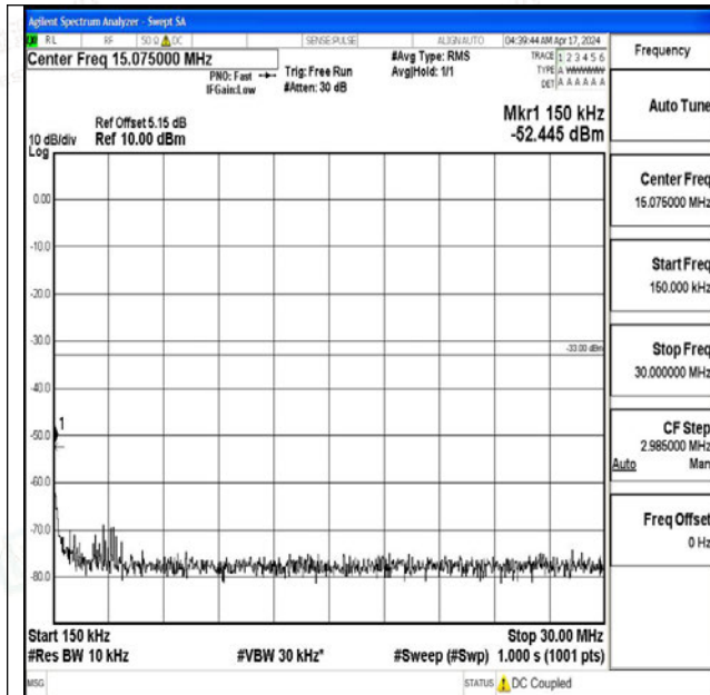
Band4_20MHz_16QAM_20050_1RB#0_0.15~30_0.15~3
