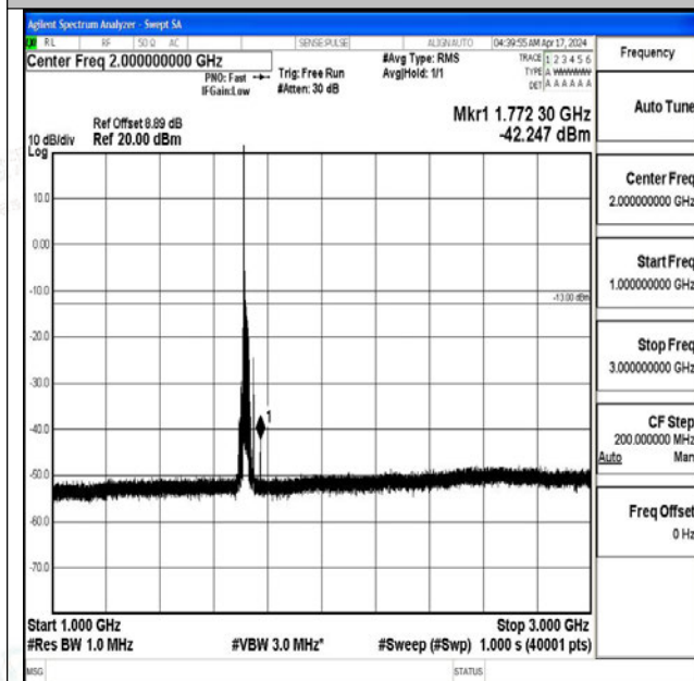
Band4_20MHz_16QAM_20050_1RB#0_1000~3000_100
