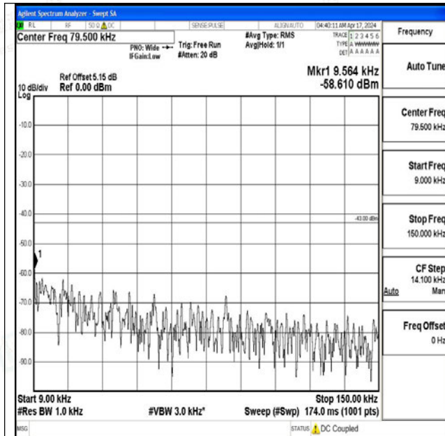
Band4_20MHz_QPSK_20175_1RB#0_0.009~0.15_0.009~0.15
