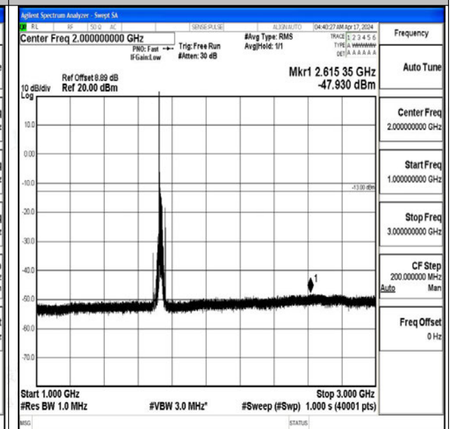
Band4_20MHz_QPSK_20175_1RB#0_1000~3000_1000~3000
