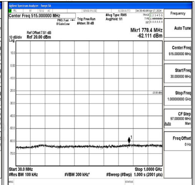
Band4_20MHz_16QAM_20050_1RB#0_30~1000_30~10
