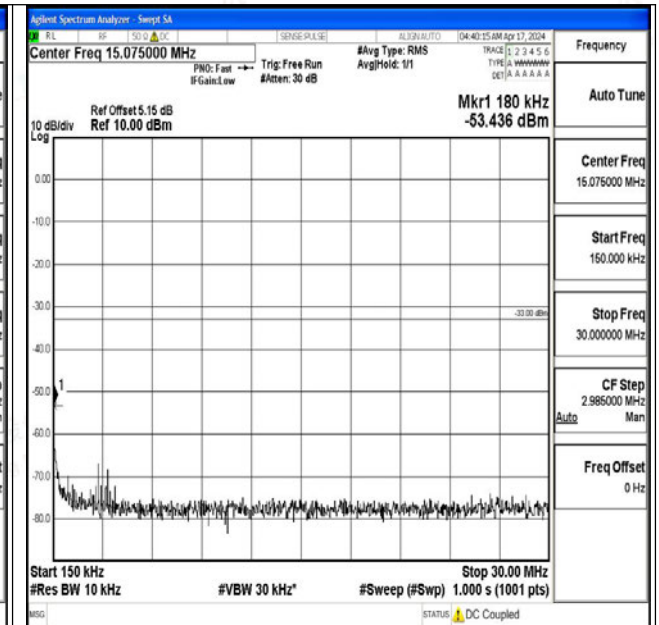
Band4_20MHz_QPSK_20175_1RB#0_0.15~30_0.15~30
