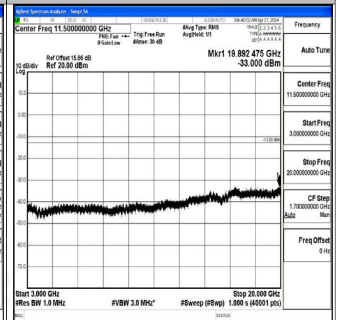
Band4_20MHz_16QAM_20050_1RB#0_3000~20000_30
