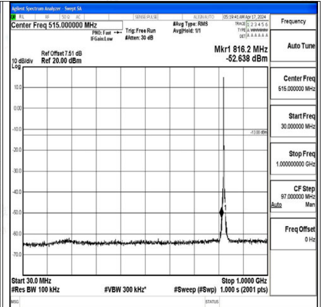
Band5_3MHz_16QAM_20415_1RB#0_30~1000_30~100
