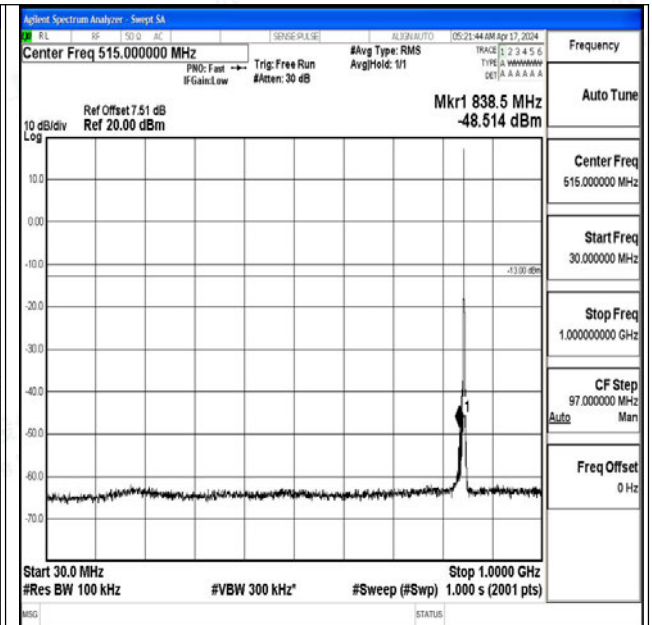
Band5_3MHz_16QAM_20635_1RB#0_30~1000_30~100
