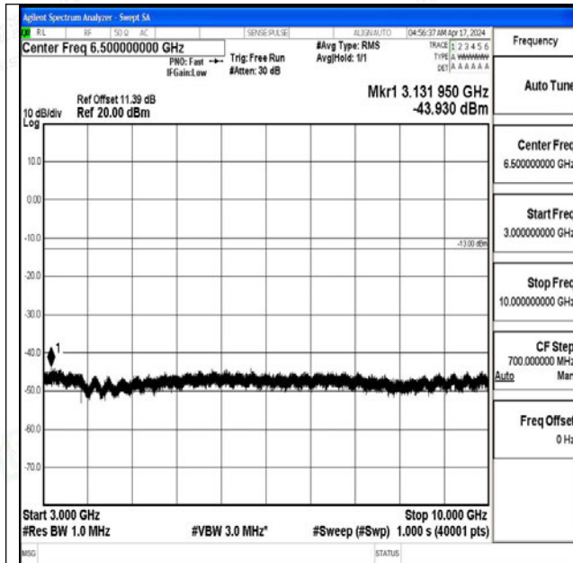
Band5_1.4MHz_QPSK_20643_1RB#0_3000~10000_300 0~10000
