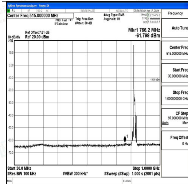
Band5_10MHz_QPSK_20450_1RB#0_30~1000_30~100
