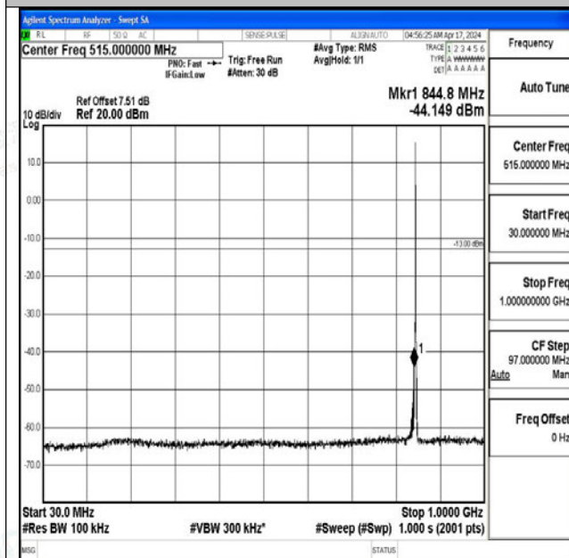
Band5_1.4MHz_QPSK_20643_1RB#0_30~1000_30~1000 0
