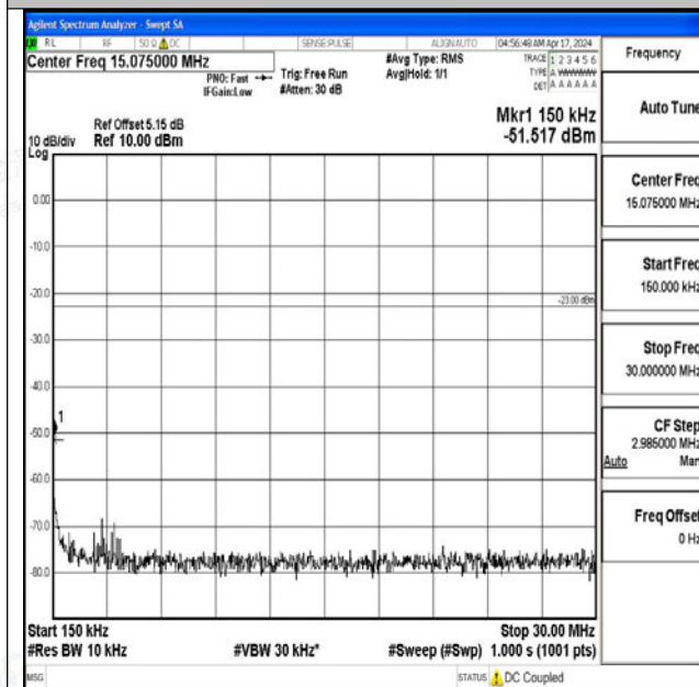
Band5_1.4MHz_16QAM_20643_1RB#0_0.15~30_0.15~ 30
