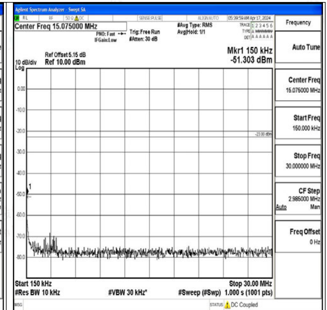
Band5_5MHz_QPSK_20625_1RB#0_0.15~30_0.15~30
