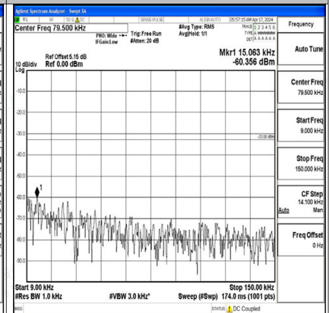
Band5_10MHz_16QAM_20450_1RB#0_0.009~0.15_0.0
