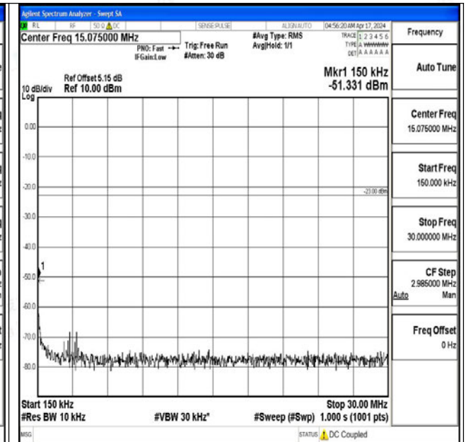
Band5_1.4MHz_QPSK_20643_1RB#0_0.15~30_0.15~30
