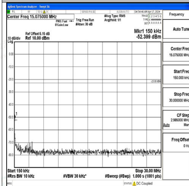
Band5_1.4MHz_16QAM_20407_1RB#0_0.15~30_0.15~ 30
