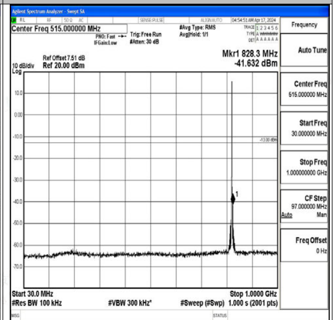
Band5_1.4MHz_16QAM_20407_1RB#0_30~1000_30~1 000
