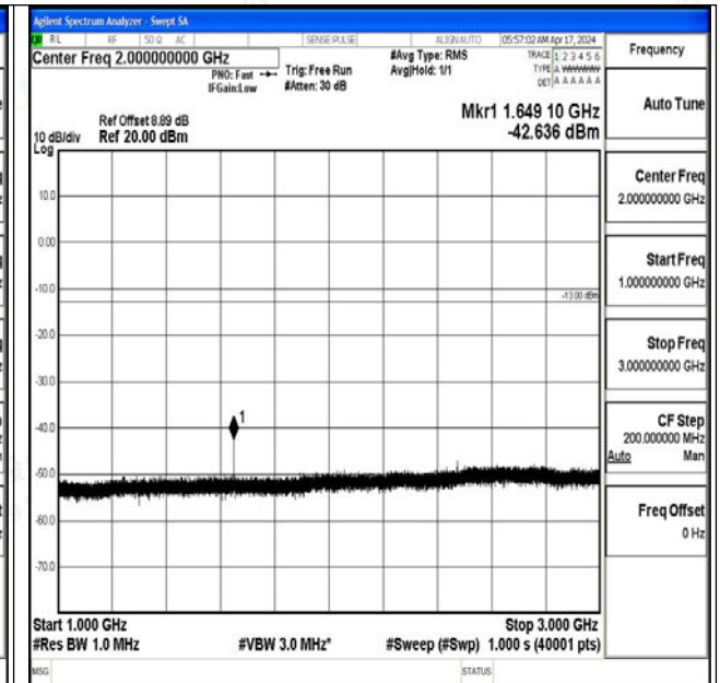
Band5_10MHz_QPSK_20450_1RB#0_1000~3000_1000
