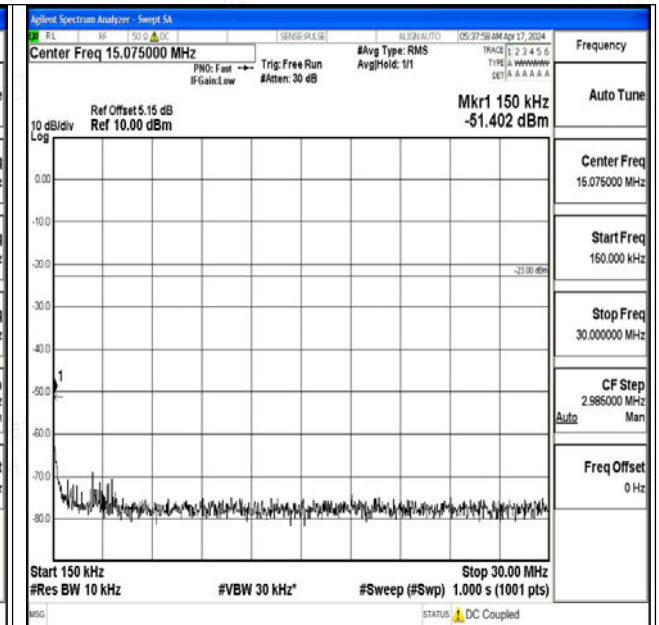
Band5_5MHz_QPSK_20425_1RB#0_0.15~30_0.15~30
