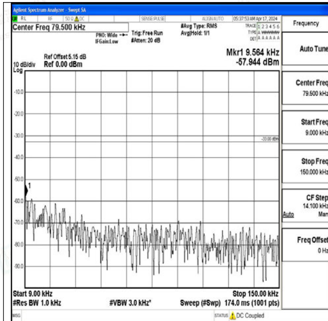
Band5_5MHz_QPSK_20425_1RB#0_0.009~0.15_0.009~0.15
