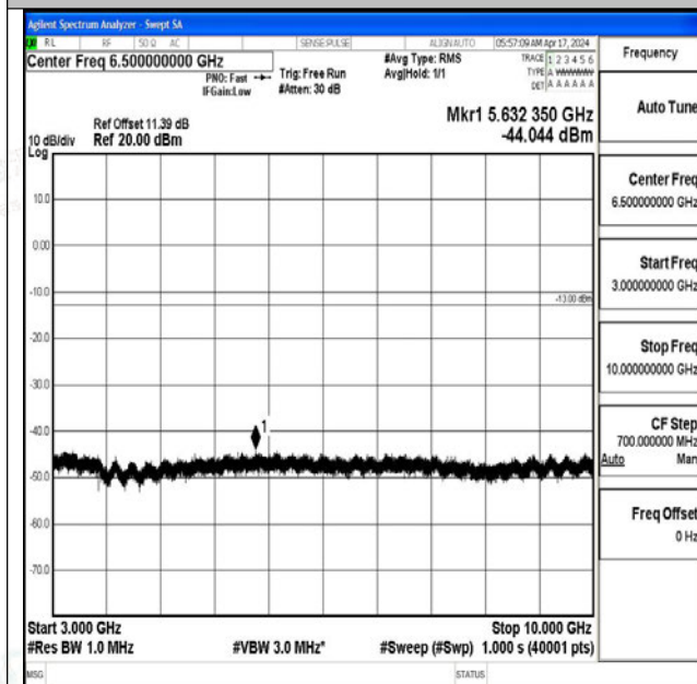
Band5_10MHz_QPSK_20450_1RB#0_3000~10000_300
