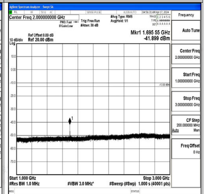
Band5_1.4MHz_QPSK_20643_1RB#0_1000~3000_1000 ~3000
