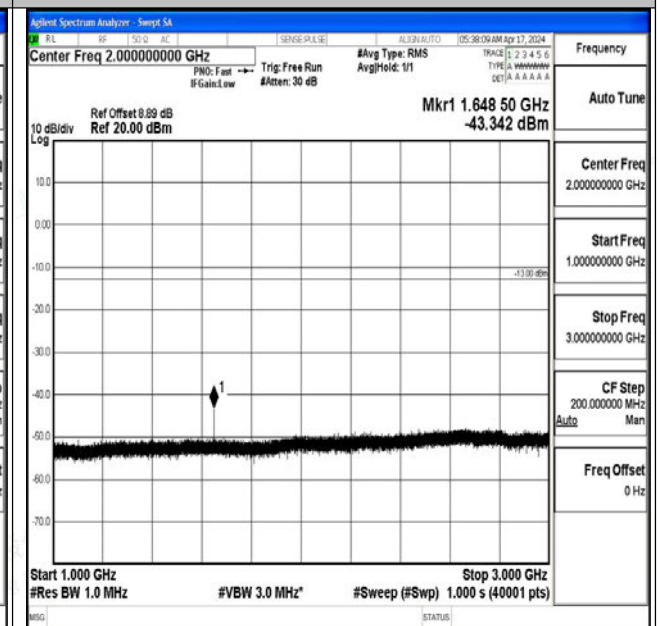
Band5_5MHz_QPSK_20425_1RB#0_1000~3000_1000~3000
