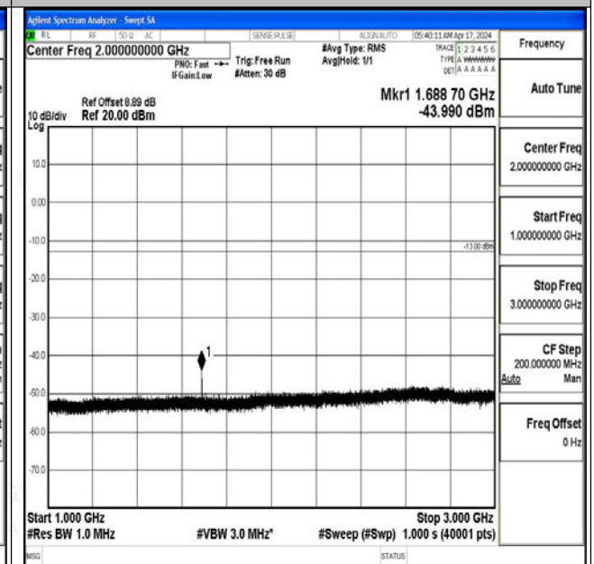
Band5_5MHz_QPSK_20625_1RB#0_1000~3000_1000~3000
