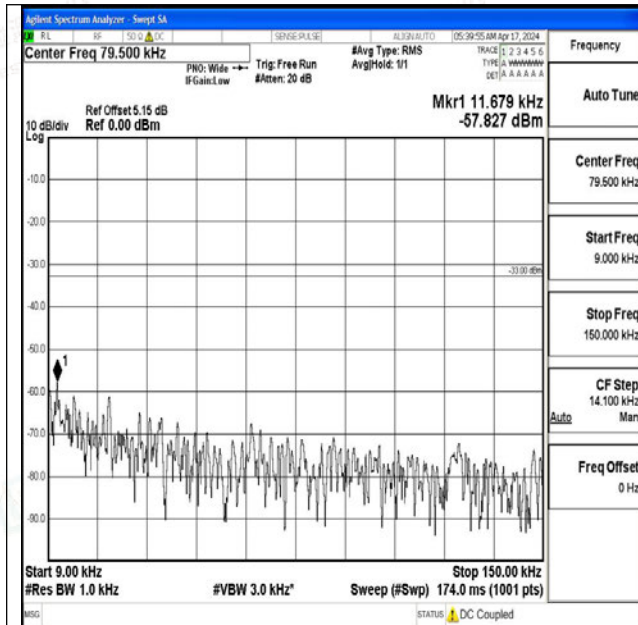
Band5_5MHz_QPSK_20625_1RB#0_0.009~0.15_0.009~0.15
