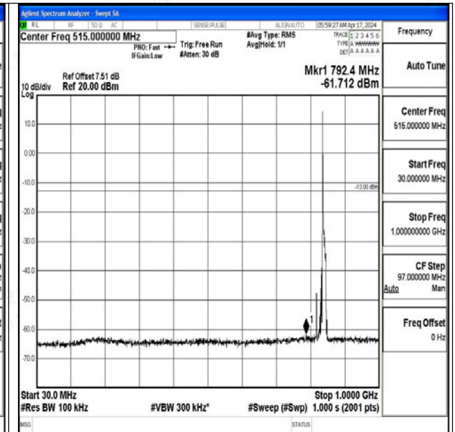
Band5_10MHz_16QAM_20600_1RB#0_30~1000_30~10
