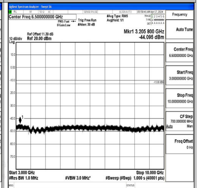
Band5_10MHz_16QAM_20600_1RB#0_3000~10000_30
