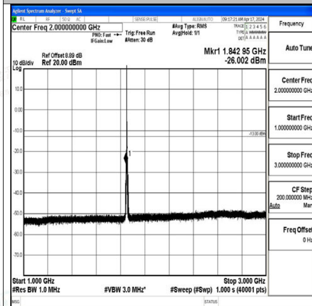
Band25_3MHz_16QAM_26055_1RB#0_1000~3000_100
