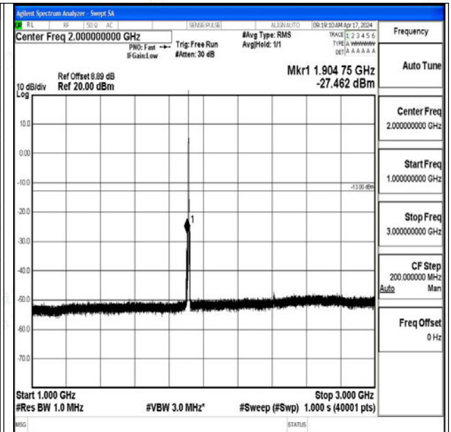
Band25_3MHz_QPSK_26675_1RB#0_1000~3000_1000~3000 ~3000
