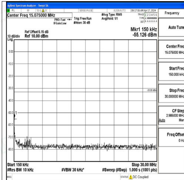
Band25_3MHz_16QAM_26055_1RB#0_0.15~30_0.15~3
