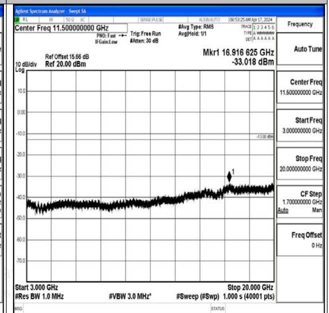
Band25_1.4MHz_16QAM_26365_1RB#0_3000~20000_ 3000~20000
