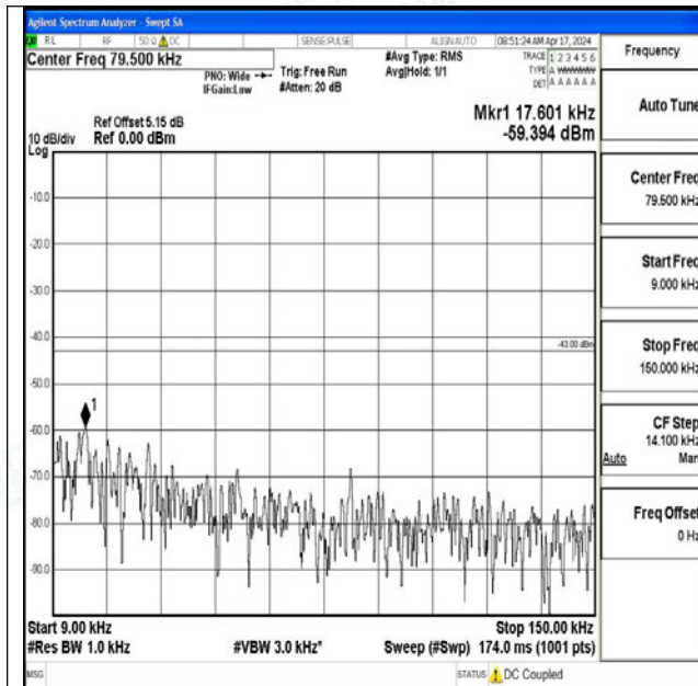
Band25_1.4MHz_QPSK_26047_1RB#0_0.009~0.15_0.0 09~0.15
