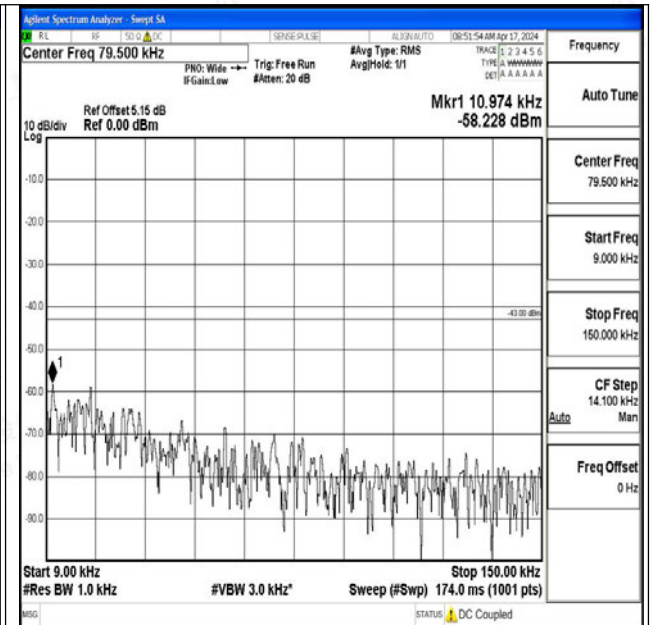
Band25_1.4MHz_16QAM_26047_1RB#0_0.009~0.15_0.009~0.15
