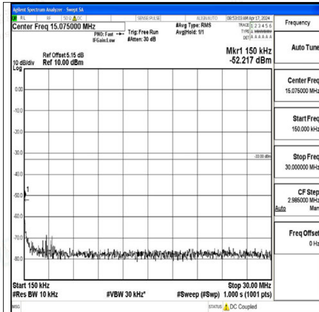
Band25_1.4MHz_16QAM_26365_1RB#0_0.15~30_0.15 ~30
