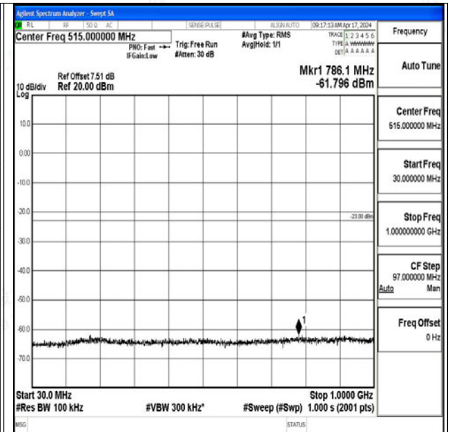
Band25_3MHz_16QAM_26055_1RB#0_30~1000_30~10
