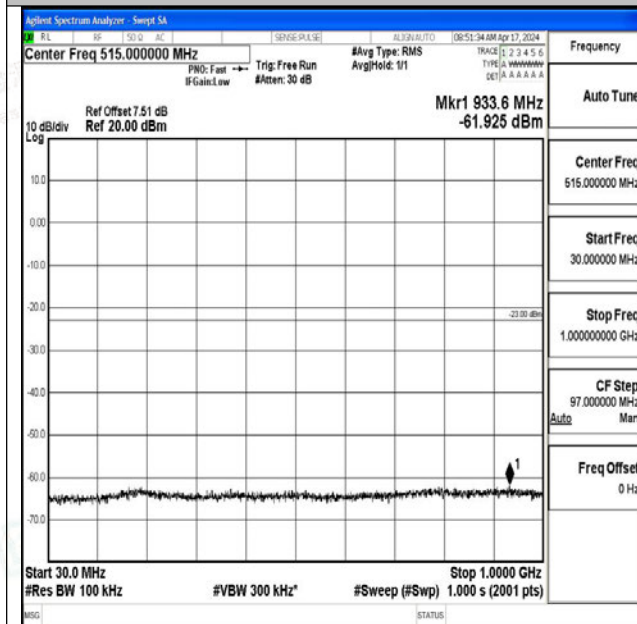
Band25_1.4MHz_QPSK_26047_1RB#0_30~1000_30~10 00
