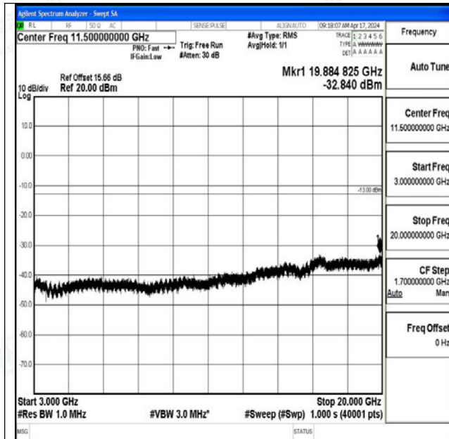
Band25_3MHz_QPSK_26365_1RB#0_3000~20000_300 0~20000
