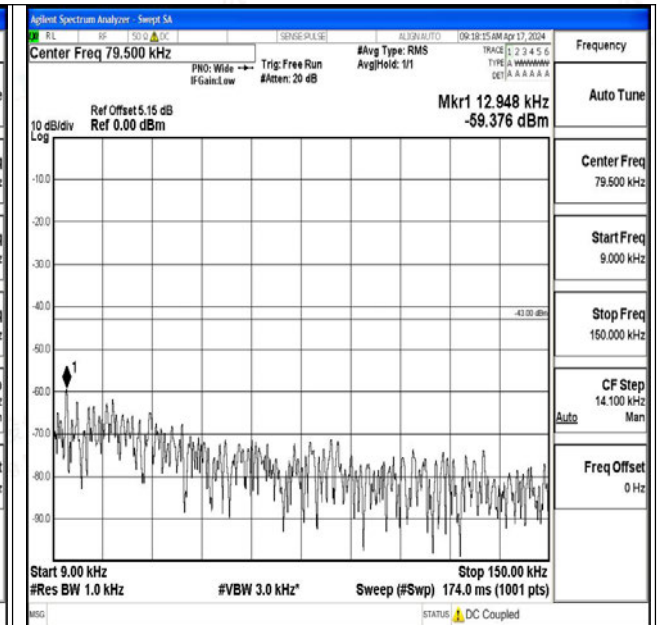
Band25_3MHz_16QAM_26365_1RB#0_0.009~0.15_0.0 09~0.15
