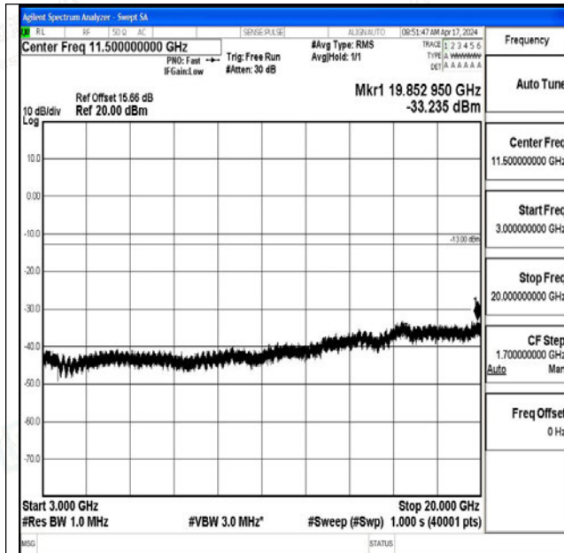
Band25_1.4MHz_QPSK_26047_1RB#0_3000~20000_3000~20000
