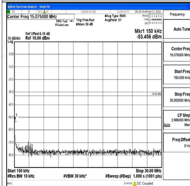
Band25_3MHz_16QAM_26365_1RB#0_0.15~30_0.15~3 0
