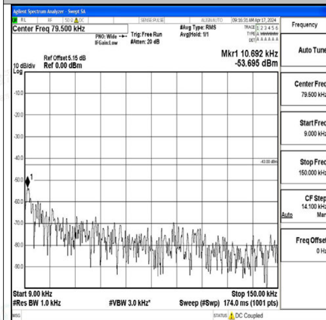
Band25_3MHz_QPSK_26055_1RB#0_0.009~0.15_0.009 ~0.15
