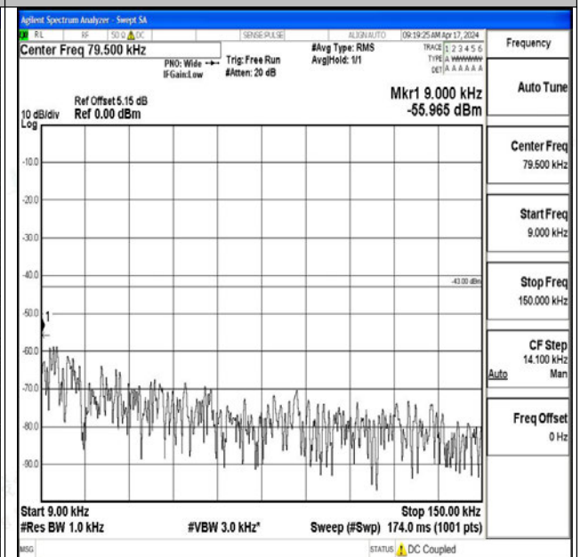
Band25_3MHz_16QAM_26675_1RB#0_0.009~0.15_0.009~0.15 09~0.15
