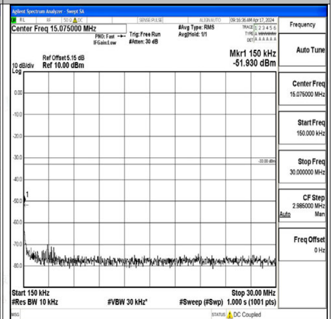
Band25_3MHz_QPSK_26055_1RB#0_0.15~30_0.15~30
