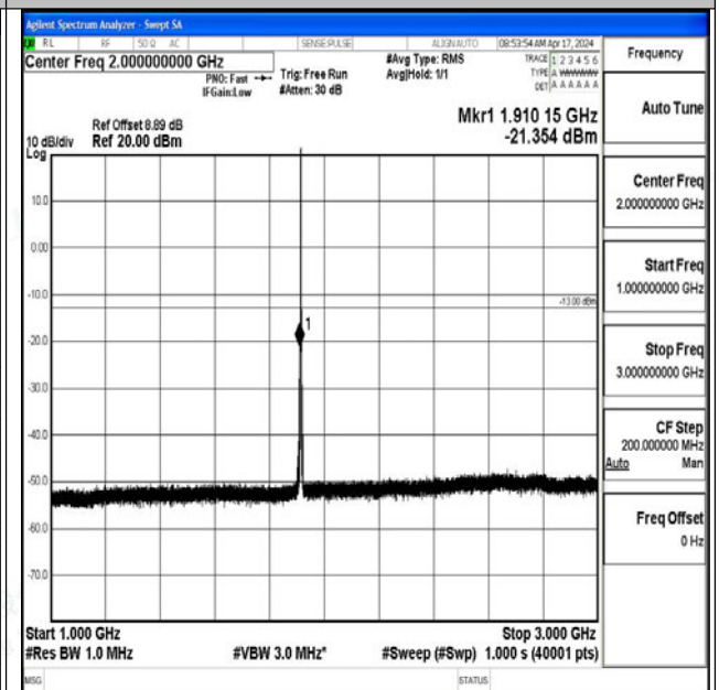
Band25_1.4MHz_QPSK_26683_1RB#0_1000~3000_100
