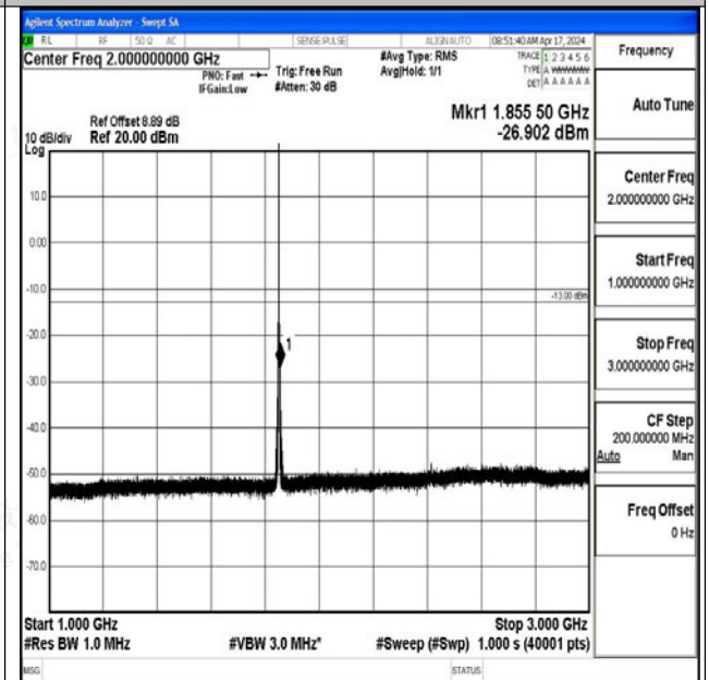
Band25_1.4MHz_QPSK_26047_1RB#0_1000~3000_100 0~3000
