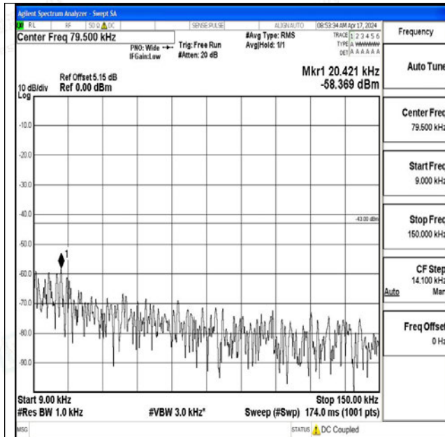
Band25_1.4MHz_QPSK_26683_1RB#0_0.009~0.15_0.0
