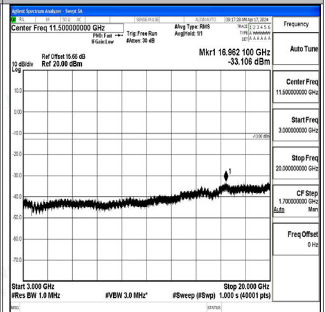
Band25_3MHz_16QAM_26055_1RB#0_3000~20000_30
