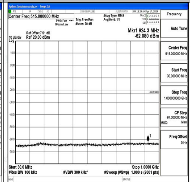
Band25_3MHz_16QAM_26365_1RB#0_30~1000_30~10 00
