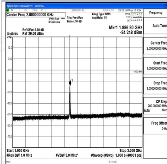
Band25_1.4MHz_16QAM_26365_1RB#0_1000~3000_1 000~3000
