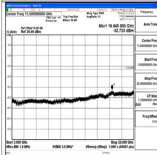
Band25_3MHz_QPSK_26675_1RB#0_3000~20000_3000~20000 0~20000
