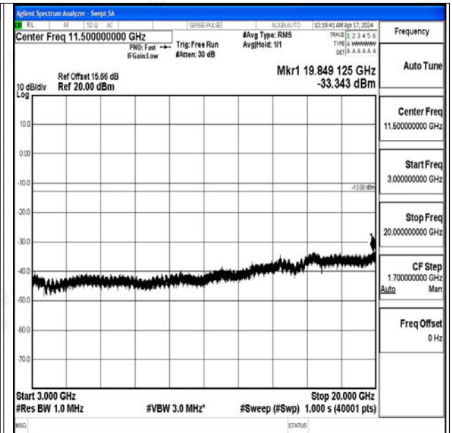
Band25_15MHz_16QAM_26115_1RB#0_3000~20000_3000~20000
