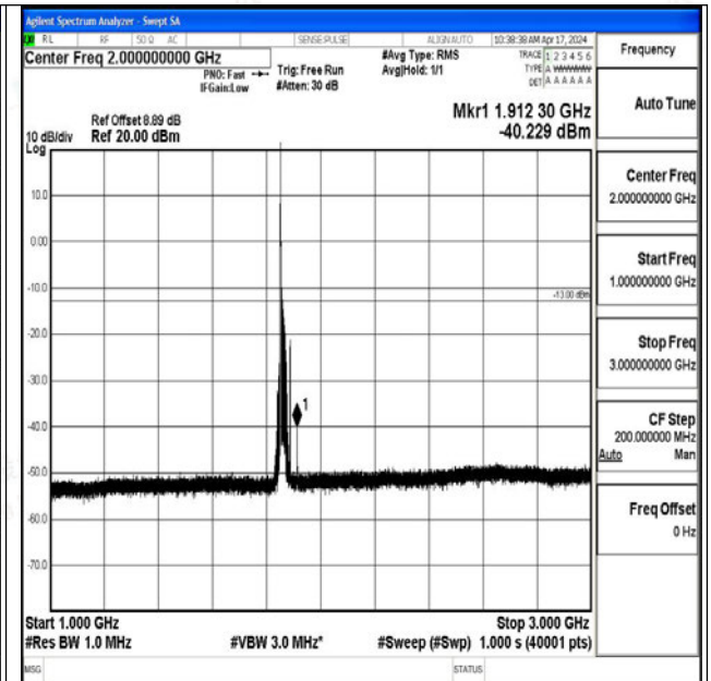
Band25_20MHz_QPSK_26140_1RB#0_1000~3000_1000~3000
