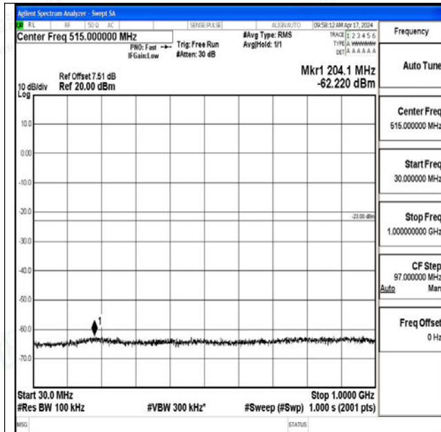
Band25_10MHz_QPSK_26090_1RB#0_30~1000_30~1000
