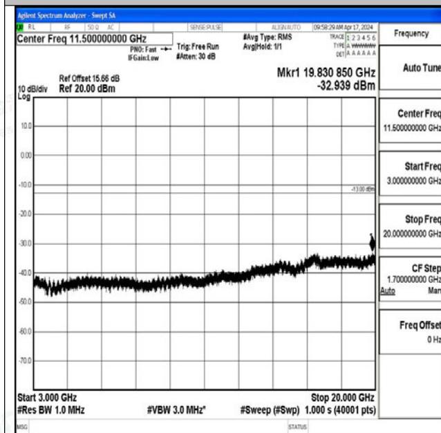
Band25_10MHz_QPSK_26090_1RB#0_3000~20000_3000~20000
