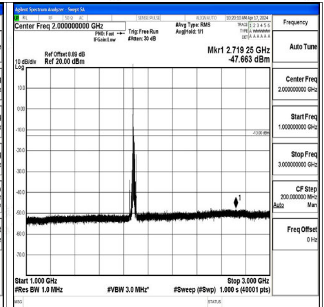
Band25_15MHz_QPSK_26365_1RB#0_1000~3000_1000~3000
