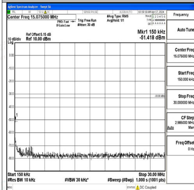
Band25_15MHz_16QAM_26115_1RB#0_0.15~30_0.15~30
