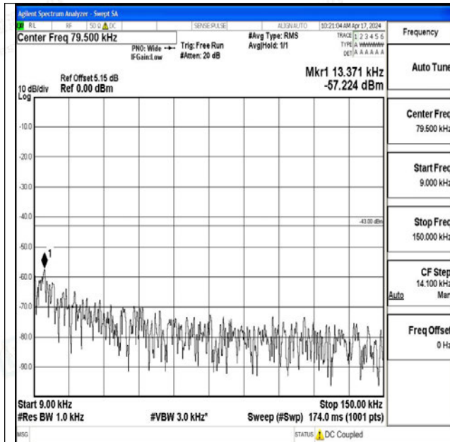
Band25_15MHz_QPSK_26615_1RB#0_0.009~0.15_0.00 9~0.15
