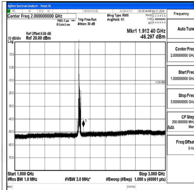
Band25_15MHz_16QAM_26115_1RB#0_1000~3000_1000~3000
