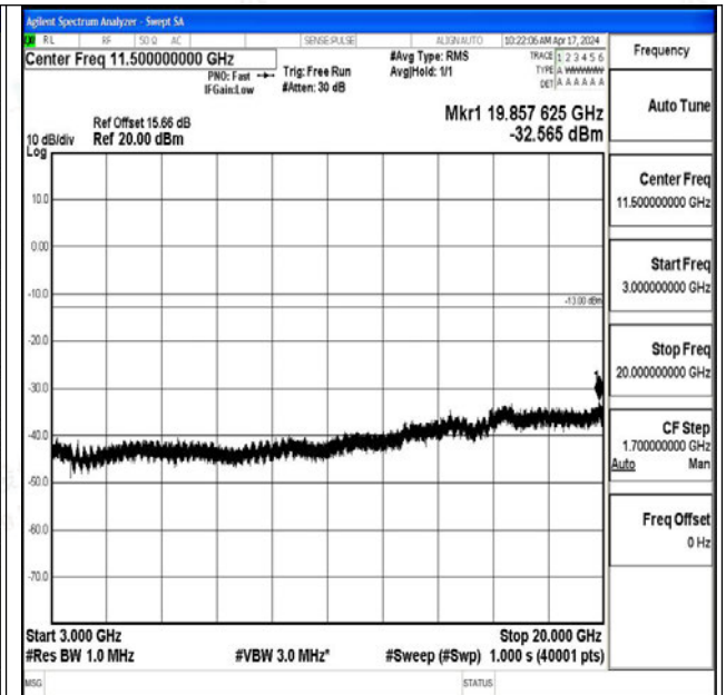
Band25_15MHz_16QAM_26615_1RB#0_3000~20000_3 000~20000
