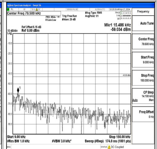
Band25_15MHz_16QAM_26365_1RB#0_0.009~0.15_0.009~0.15
