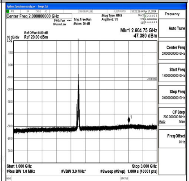
Band25_15MHz_QPSK_26615_1RB#0_1000~3000_100 0~3000
