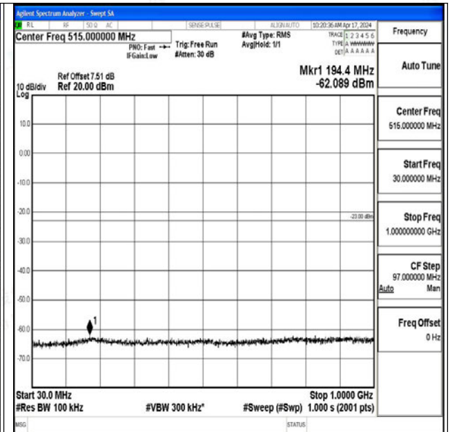
Band25_15MHz_16QAM_26365_1RB#0_30~1000_30~1000
