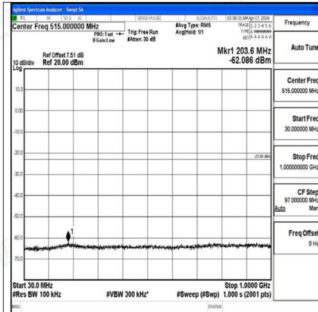
Band25_20MHz_QPSK_26140_1RB#0_30~1000_30~1000
