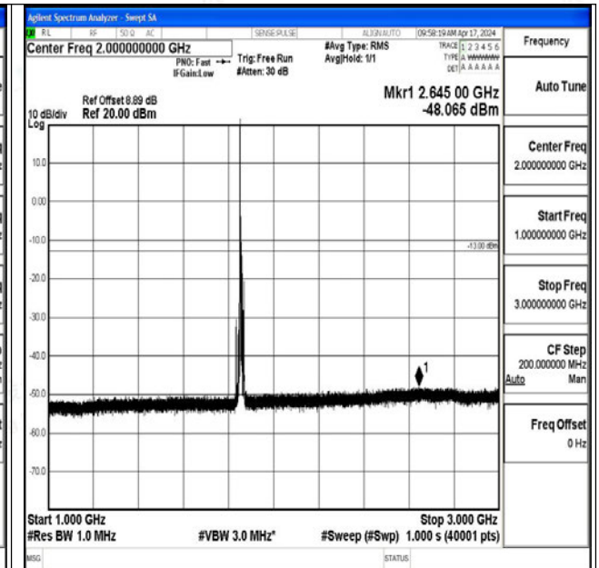
Band25_10MHz_QPSK_26090_1RB#0_1000~3000_1000~3000
