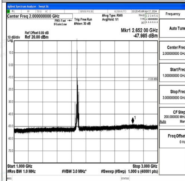
Band25_15MHz_16QAM_26365_1RB#0_1000~3000_1000~3000
