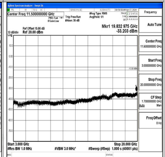
Band25_10MHz_16QAM_26090_1RB#0_3000~20000_3000~20000
