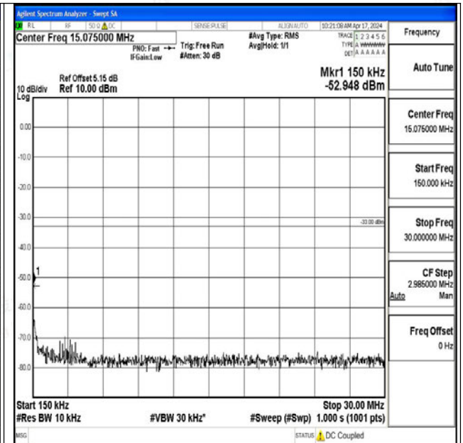
Band25_15MHz_QPSK_26615_1RB#0_0.15~30_0.15~3 0
