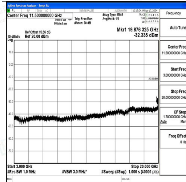
Band25_15MHz_QPSK_26115_1RB#0_3000~20000_3000~20000
