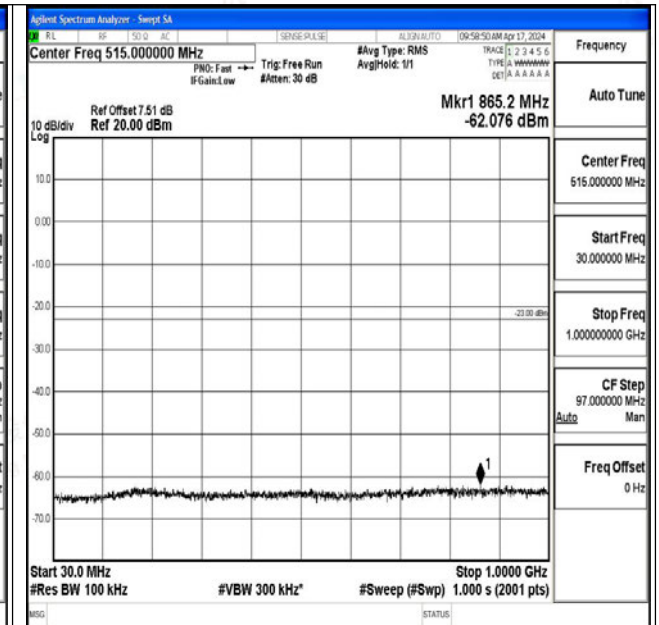
Band25_10MHz_16QAM_26090_1RB#0_30~1000_30~1000
