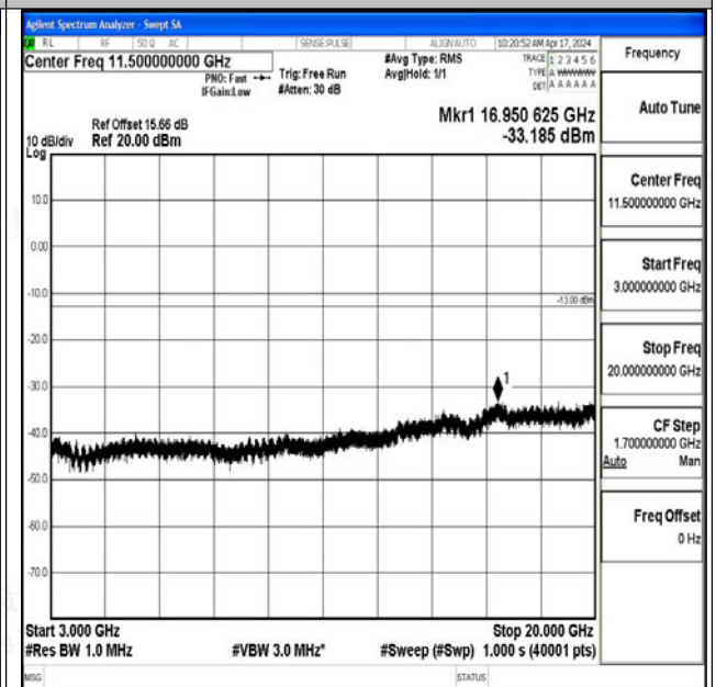
Band25_15MHz_16QAM_26365_1RB#0_3000~20000_3000~20000
