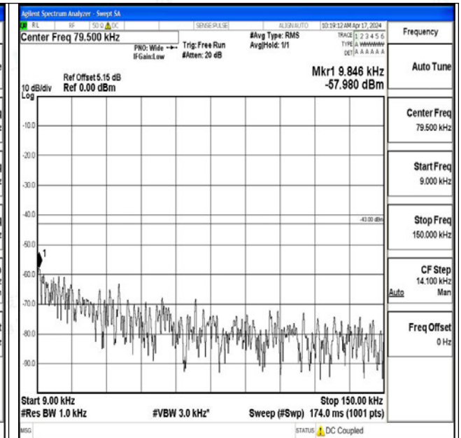
Band25_15MHz_16QAM_26115_1RB#0_0.009~0.15_0.009~0.15
