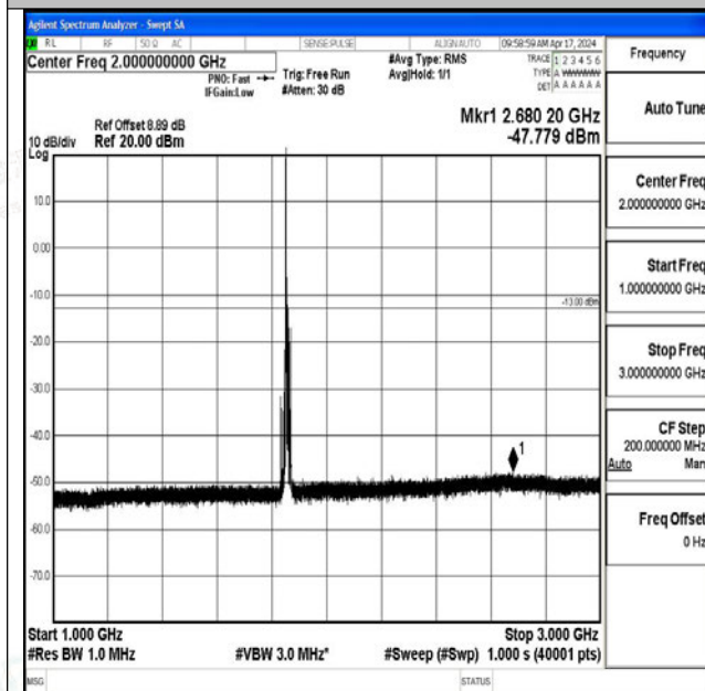
Band25_10MHz_16QAM_26090_1RB#0_1000~3000_1000~3000
