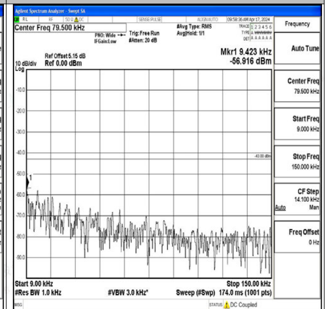
Band25_10MHz_16QAM_26090_1RB#0_0.009~0.15_0.009~0.15
