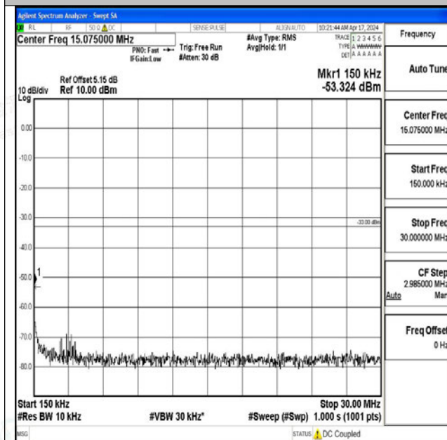
Band25_15MHz_16QAM_26615_1RB#0_0.15~30_0.15~ 30
