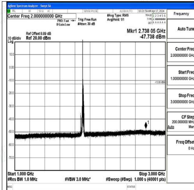
Band25_15MHz_16QAM_26615_1RB#0_1000~3000_10 00~3000
