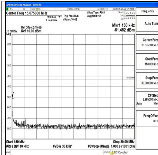
Band25_15MHz_16QAM_26365_1RB#0_0.15~30_0.15~30
