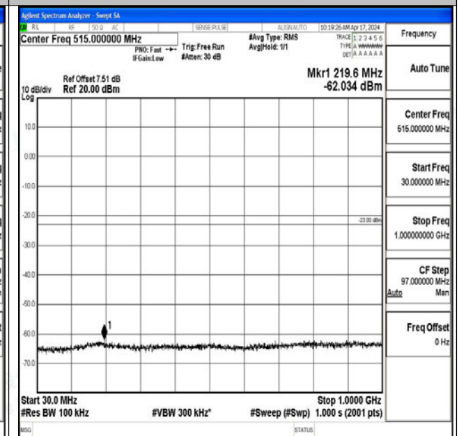
Band25_15MHz_16QAM_26115_1RB#0_30~1000_30~1000
