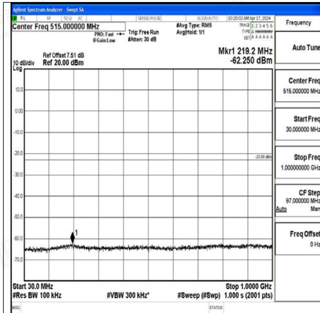
Band25_15MHz_QPSK_26365_1RB#0_30~1000_30~1000
