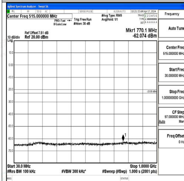
Band25_15MHz_QPSK_26615_1RB#0_30~1000_30~10 00
