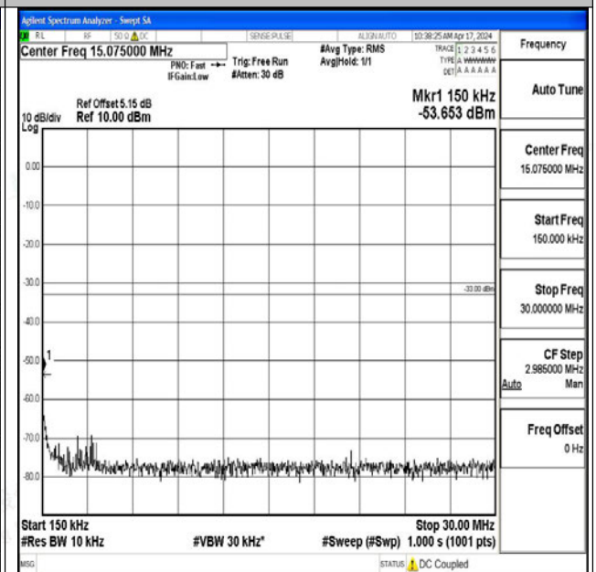
Band25_20MHz_QPSK_26140_1RB#0_0.15~30_0.15~3 0
