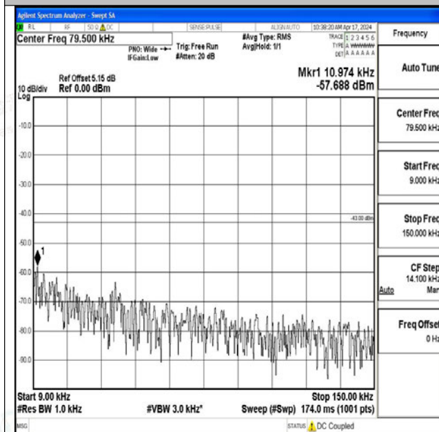
Band25_20MHz_QPSK_26140_1RB#0_0.009~0.15_0.00 9~0.15
