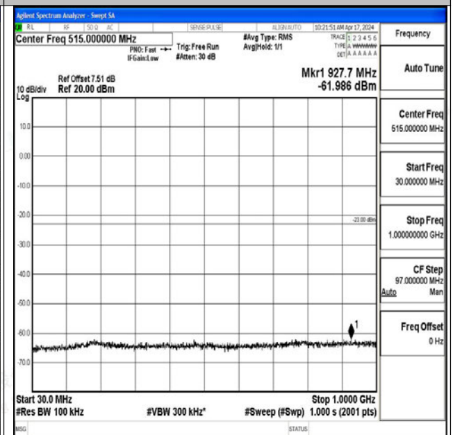
Band25_15MHz_16QAM_26615_1RB#0_30~1000_30~1 000
