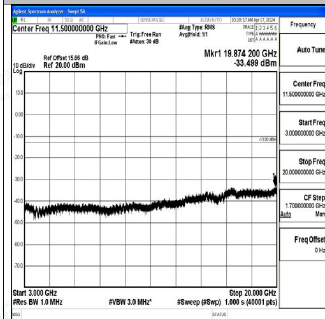
Band25_15MHz_QPSK_26365_1RB#0_3000~20000_3000~20000
