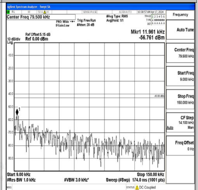
Band25_20MHz_16QAM_26140_1RB#0_0.009~0.15_0.009~0.15
