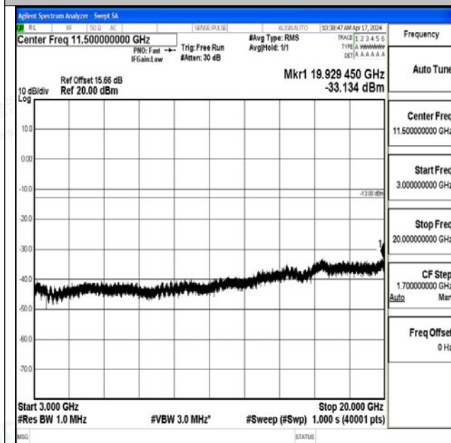
Band25_20MHz_QPSK_26140_1RB#0_3000~20000_3000~20000
