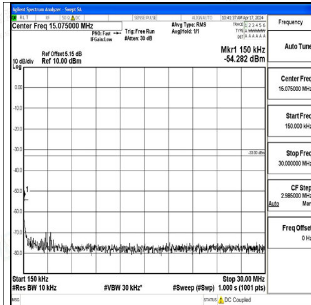
Band25_20MHz_16QAM_26590_1RB#0_0.15~30_0.15~30
