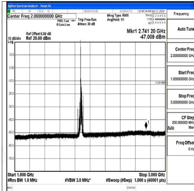
Band25_20MHz_16QAM_26365_1RB#0_1000~3000_10 00~3000
