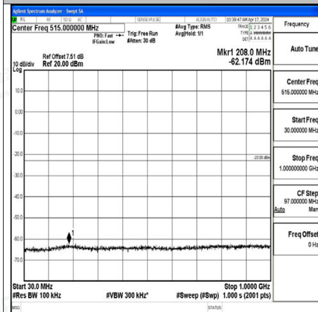
Band25_20MHz_QPSK_26365_1RB#0_30~1000_30~10 00
