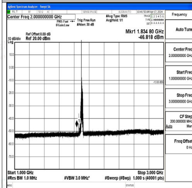
Band25_20MHz_16QAM_26590_1RB#0_1000~3000_1000~3000
