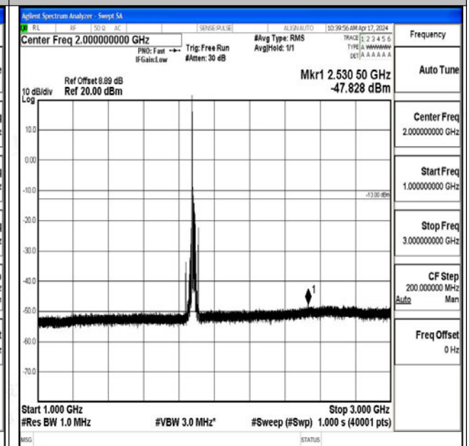
Band25_20MHz_QPSK_26365_1RB#0_1000~3000_100 0~3000
