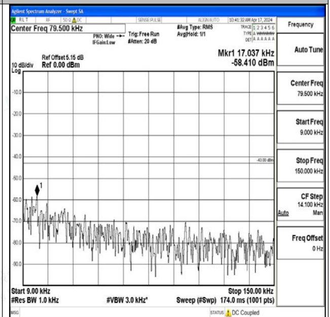
Band25_20MHz_16QAM_26590_1RB#0_0.009~0.15_0.009~0.15
