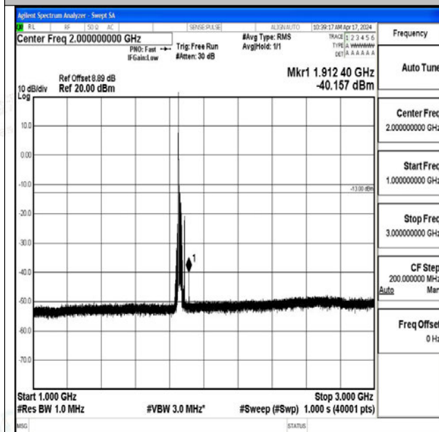
Band25_20MHz_16QAM_26140_1RB#0_1000~3000_1000~3000
