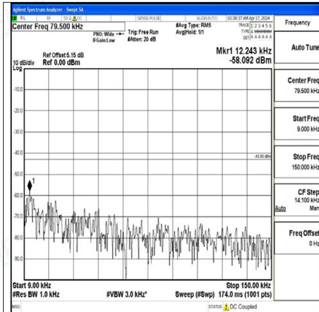
Band25_20MHz_QPSK_26365_1RB#0_0.009~0.15_0.00 9~0.15
