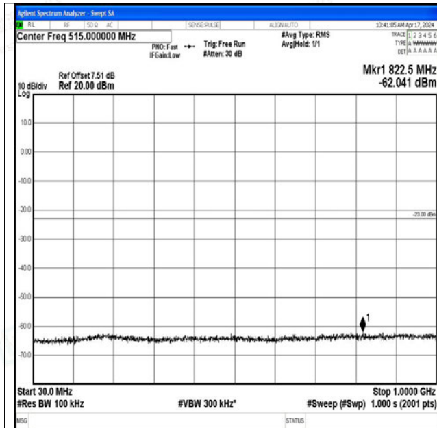
Band25_20MHz_QPSK_26590_1RB#0_30~1000_30~1000
