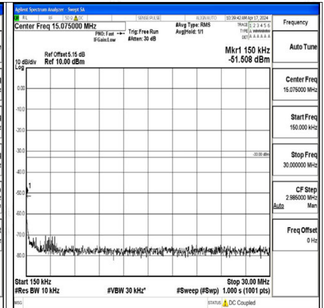
Band25_20MHz_QPSK_26365_1RB#0_0.15~30_0.15~3 0
