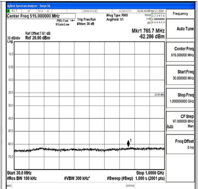
Band25_20MHz_16QAM_26590_1RB#0_30~1000_30~1000
