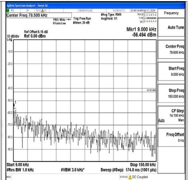
Band25_20MHz_16QAM_26365_1RB#0_0.009~0.15_0. 009~0.15
