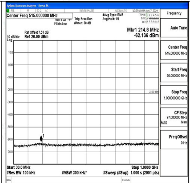
Band25_20MHz_16QAM_26140_1RB#0_30~1000_30~1000
