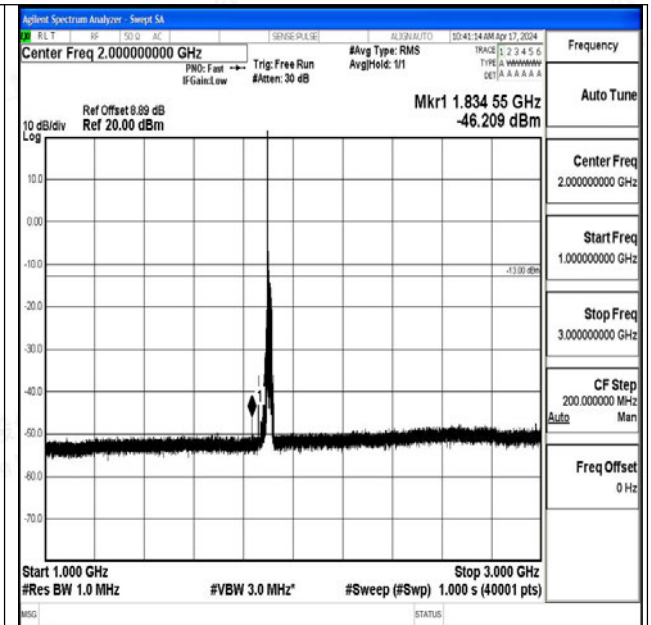
Band25_20MHz_QPSK_26590_1RB#0_1000~3000_1000~3000
