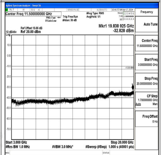
Band25_20MHz_16QAM_26590_1RB#0_3000~20000_3000~20000
