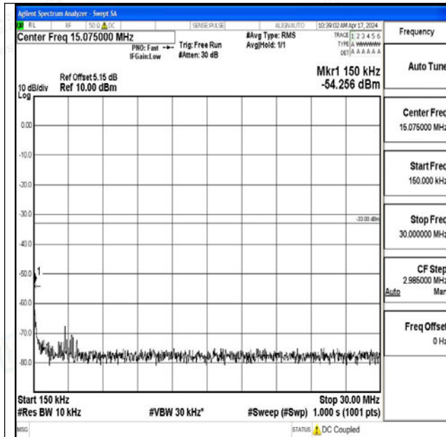
Band25_20MHz_16QAM_26140_1RB#0_0.15~30_0.15~30
