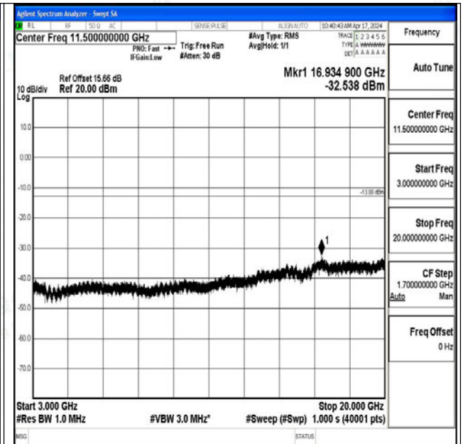
Band25_20MHz_16QAM_26365_1RB#0_3000~20000_3 000~20000
