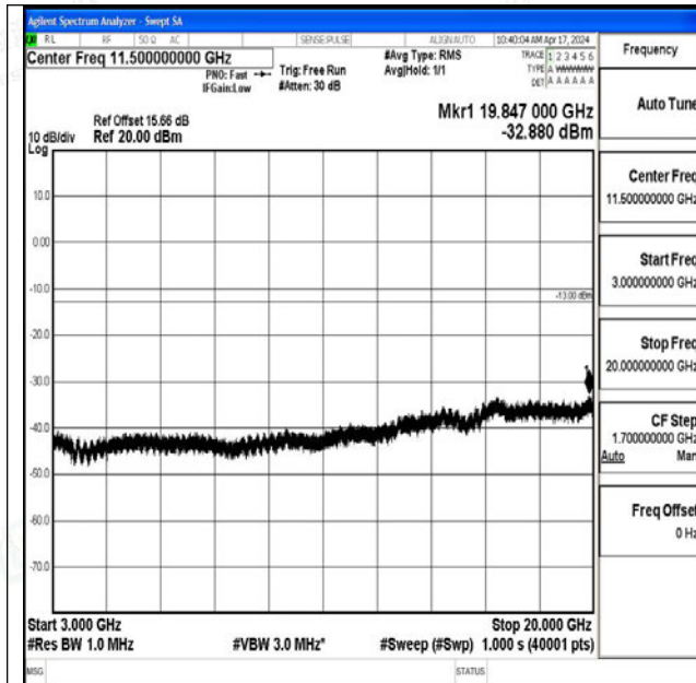
Band25_20MHz_QPSK_26365_1RB#0_3000~20000_30 00~20000
