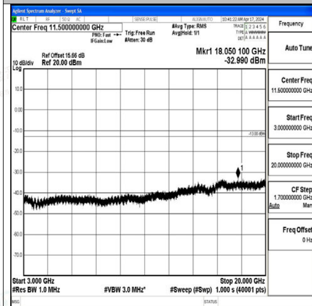
Band25_20MHz_QPSK_26590_1RB#0_3000~20000_3000~20000
