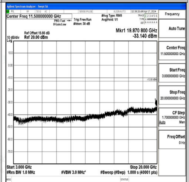
Band25_20MHz_16QAM_26140_1RB#0_3000~20000_3000~20000
