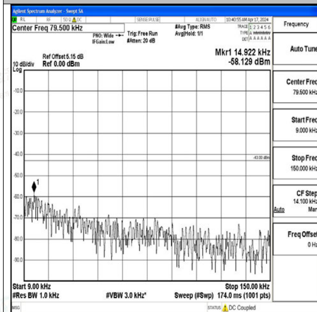
Band25_20MHz_QPSK_26590_1RB#0_0.009~0.15_0.00 9~0.15
