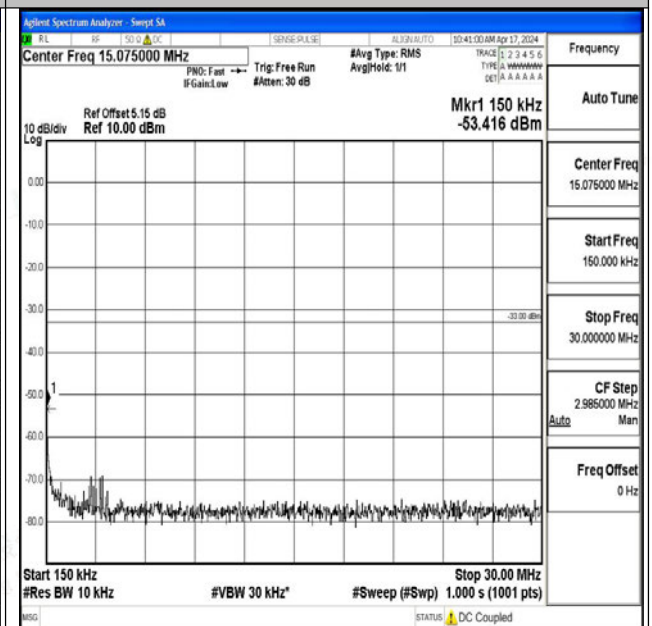
Band25_20MHz_QPSK_26590_1RB#0_0.15~30_0.15~3 0
