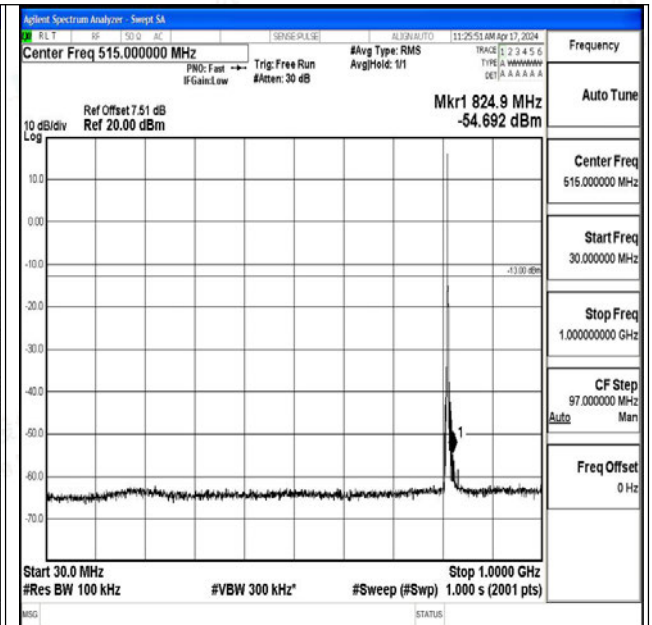
Band26_3MHz_16QAM_26705_1RB#0_30~1000_30~10
