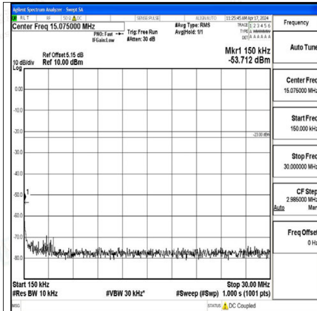
Band26_3MHz_16QAM_26705_1RB#0_0.15~30_0.15~3
