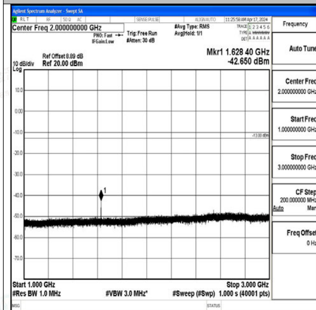
Band26_3MHz_16QAM_26705_1RB#0_1000~3000_100
