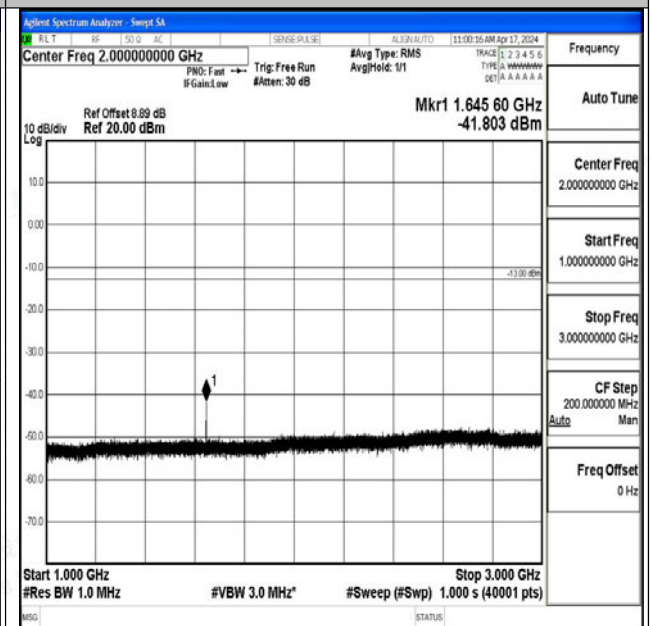
Band26_1.4MHz_QPSK_26783_1RB#0_1000~3000_100 0~3000
