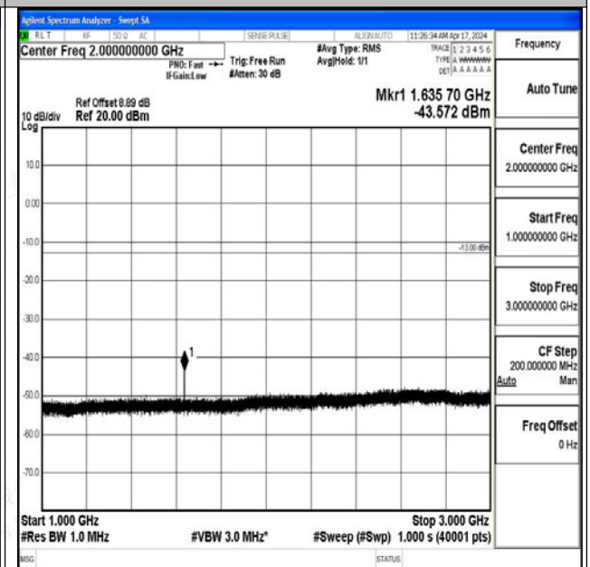
Band26_3MHz_QPSK_26740_1RB#0_1000~3000_1000 ~3000
