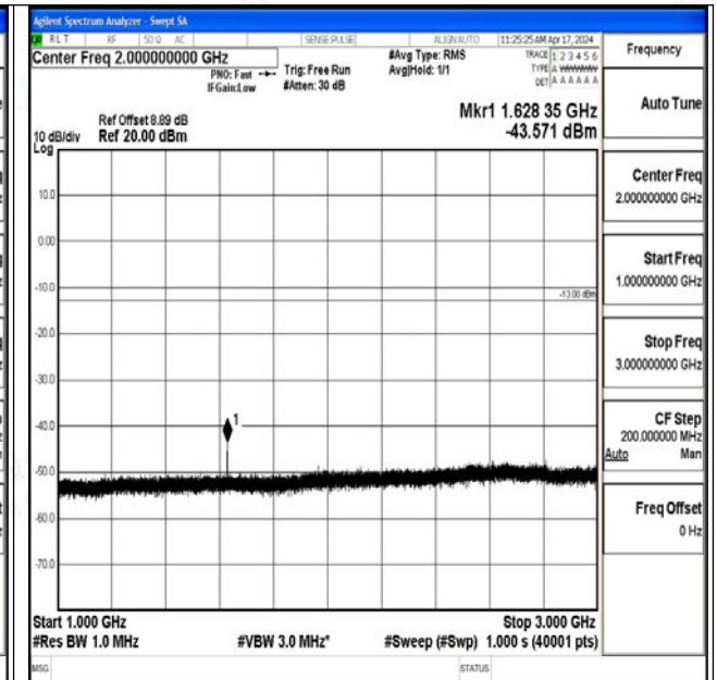
Band26_3MHz_QPSK_26705_1RB#0_1000~3000_1000 ~3000
