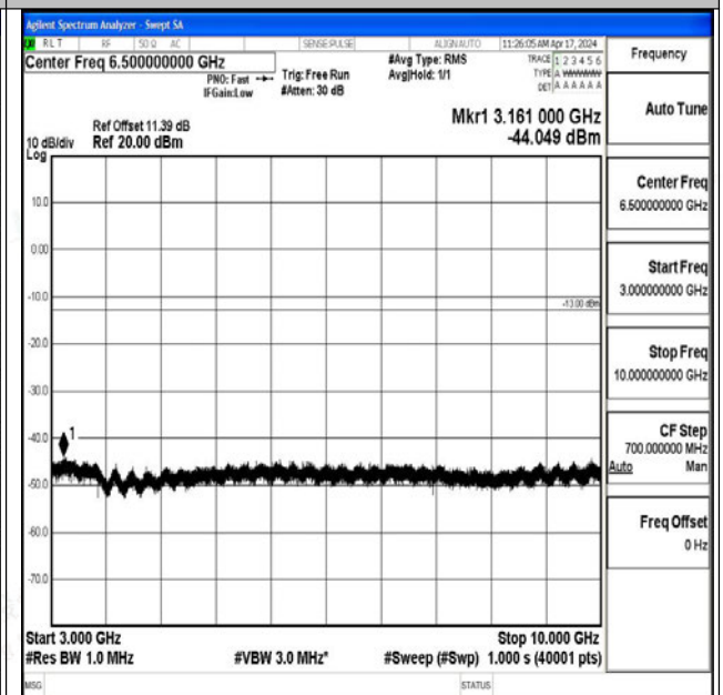
Band26_3MHz_16QAM_26705_1RB#0_3000~10000_30
