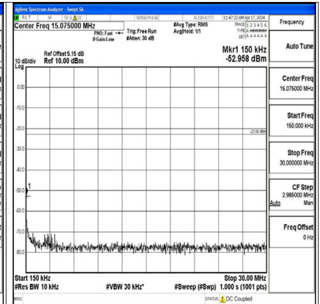
Band26_5MHz_QPSK_26715_1RB#0_0.15~30_0.15~30
