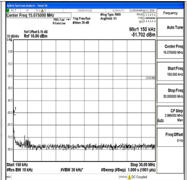
Band26_1.4MHz_QPSK_26783_1RB#0_0.15~30_0.15~3 0
