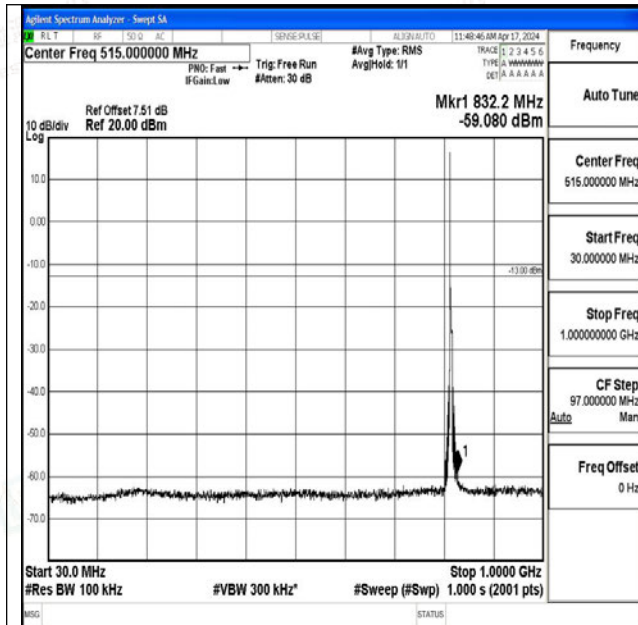
Band26_5MHz_QPSK_26740_1RB#0_30~1000_30~1000 0
