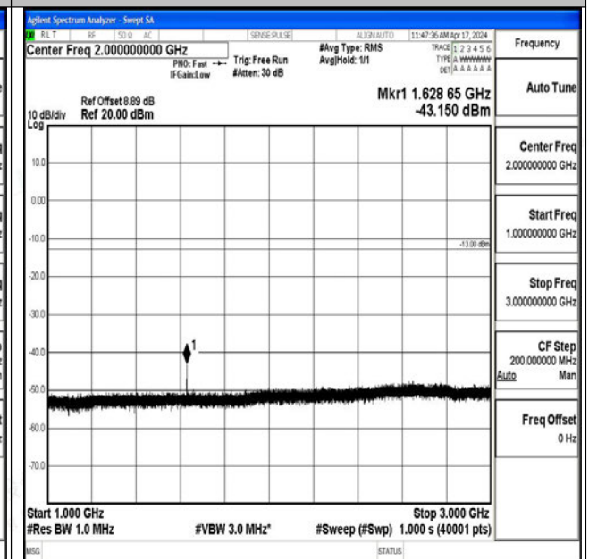
Band26_5MHz_QPSK_26715_1RB#0_1000~3000_1000 ~3000
