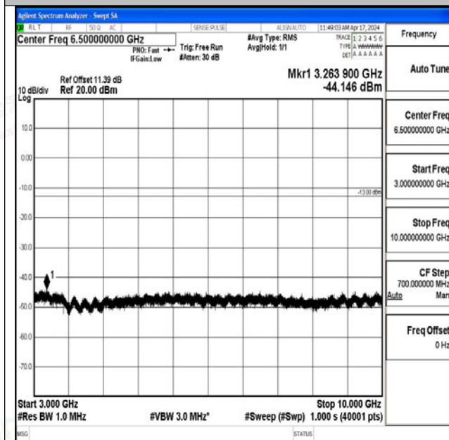
Band26_5MHz_QPSK_26740_1RB#0_3000~10000_300 0~10000
