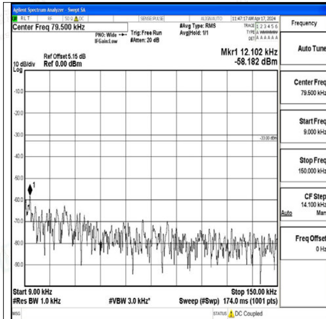
Band26_5MHz_QPSK_26715_1RB#0_0.009~0.15_0.009 ~0.15
