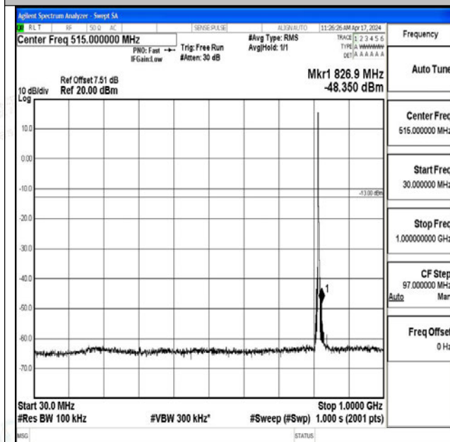
Band26_3MHz_QPSK_26740_1RB#0_30~1000_30~1000 0
