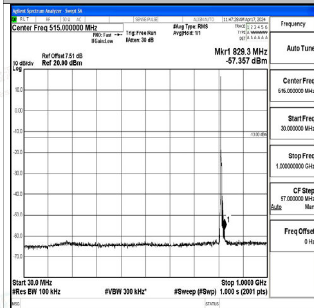
Band26_5MHz_QPSK_26715_1RB#0_30~1000_30~1000 0
