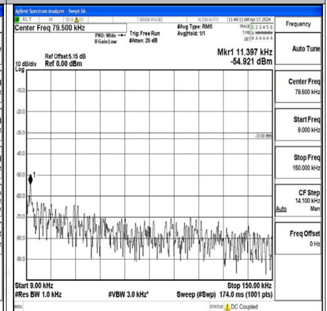
Band26_5MHz_16QAM_26740_1RB#0_0.009~0.15_0.0 09~0.15
