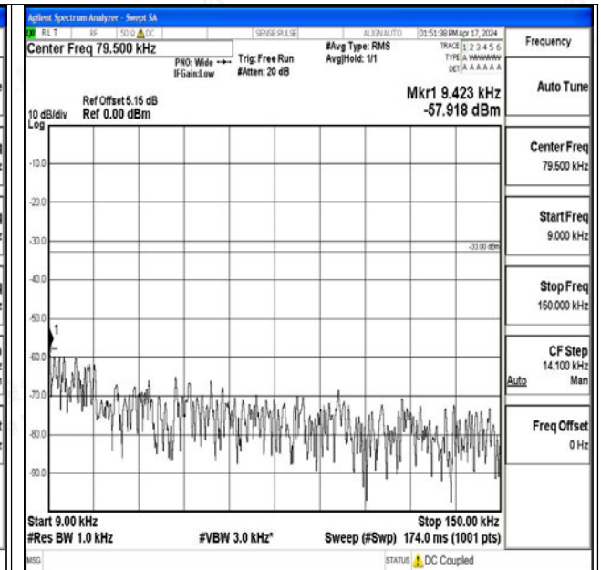
Band26_15MHz_16QAM_26865_1RB#0_0.009~0.15_0. 009~0.15
