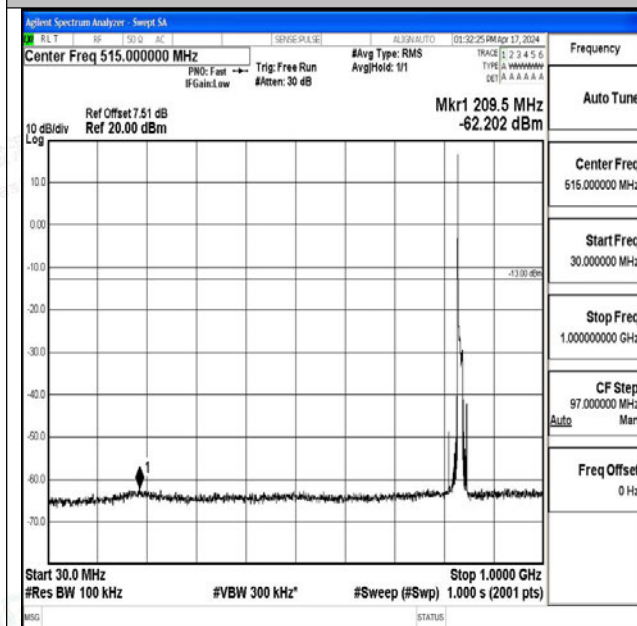
Band26_10MHz_QPSK_26915_1RB#0_30~1000_30~10 00
