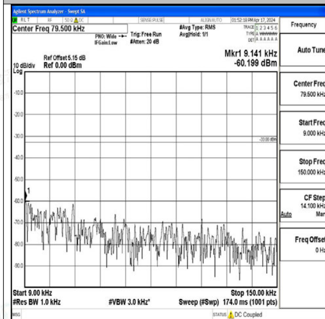
Band26_15MHz_QPSK_26915_1RB#0_0.009~0.15_0.00 9~0.15
