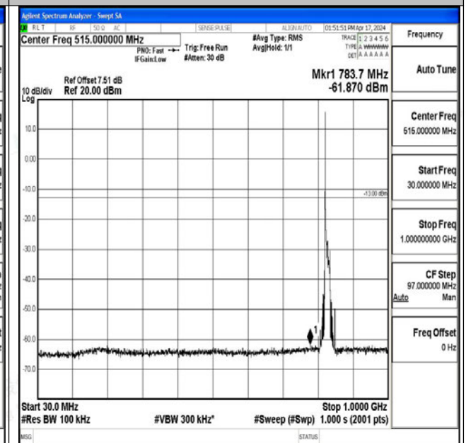
Band26_15MHz_16QAM_26865_1RB#0_30~1000_30~1 000
