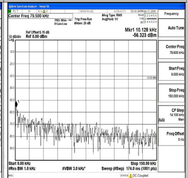
Band26_10MHz_16QAM_26840_1RB#0_0.009~0.15_0.009~0.15
