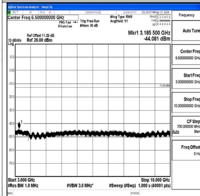
Band26_10MHz_QPSK_26990_1RB#0_3000~10000_3000~10000
