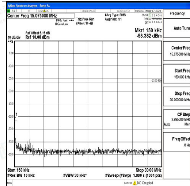
Band26_15MHz_16QAM_26915_1RB#0_0.15~30_0.15~30
