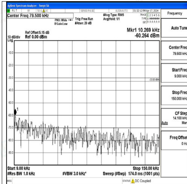
Band26_10MHz_QPSK_26915_1RB#0_0.009~0.15_0.00 9~0.15
