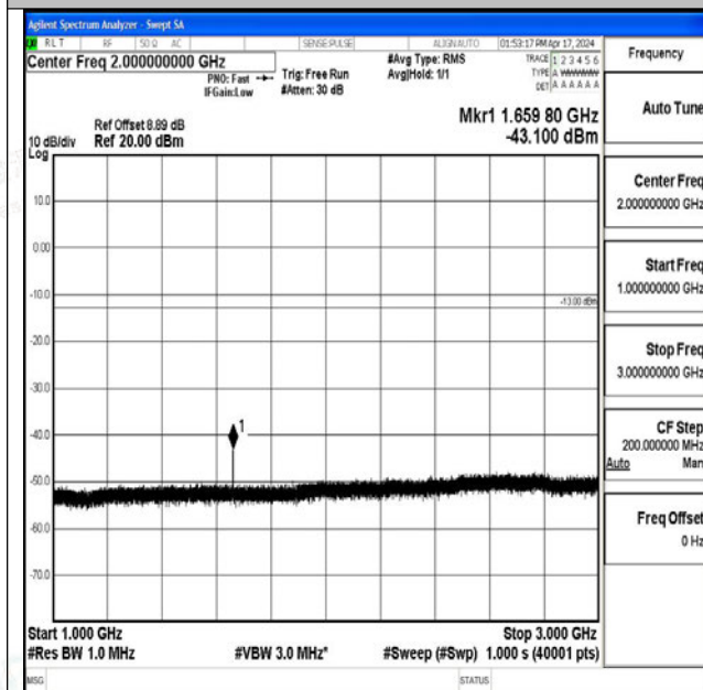
Band26_15MHz_16QAM_26915_1RB#0_1000~3000_1000~3000
