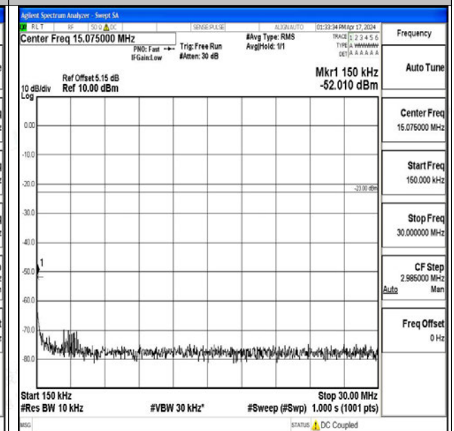
Band26_10MHz_QPSK_26990_1RB#0_0.15~30_0.15~3 0
