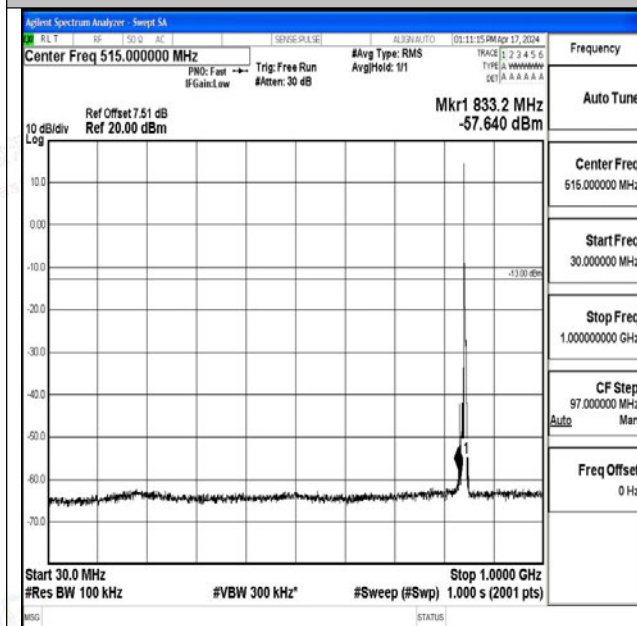
Band26_5MHz_QPSK_27015_1RB#0_30~1000_30~1000
