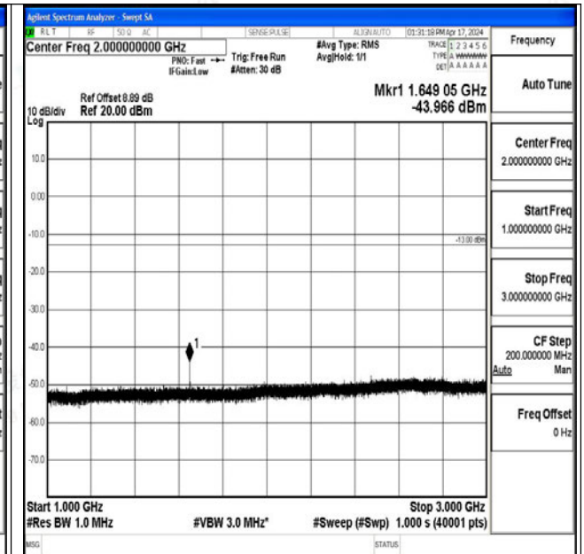
Band26_10MHz_QPSK_26840_1RB#0_1000~3000_1000~3000
