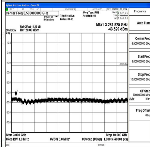
Band26_10MHz_QPSK_26840_1RB#0_3000~10000_3000~10000
