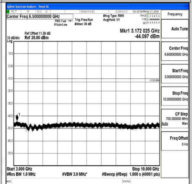
Band26_5MHz_16QAM_26915_1RB#0_3000~10000_30
