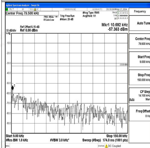
Band26_10MHz_QPSK_26990_1RB#0_0.009~0.15_0.00 9~0.15
