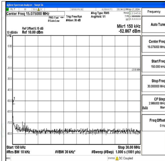
Band26_10MHz_16QAM_26990_1RB#0_0.15~30_0.15~30
