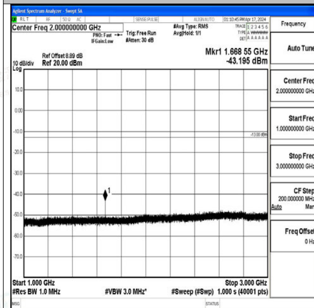
Band26_5MHz_16QAM_26915_1RB#0_1000~3000_100
