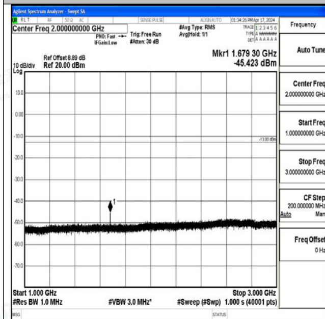
Band26_10MHz_16QAM_26990_1RB#0_1000~3000_1000~3000
