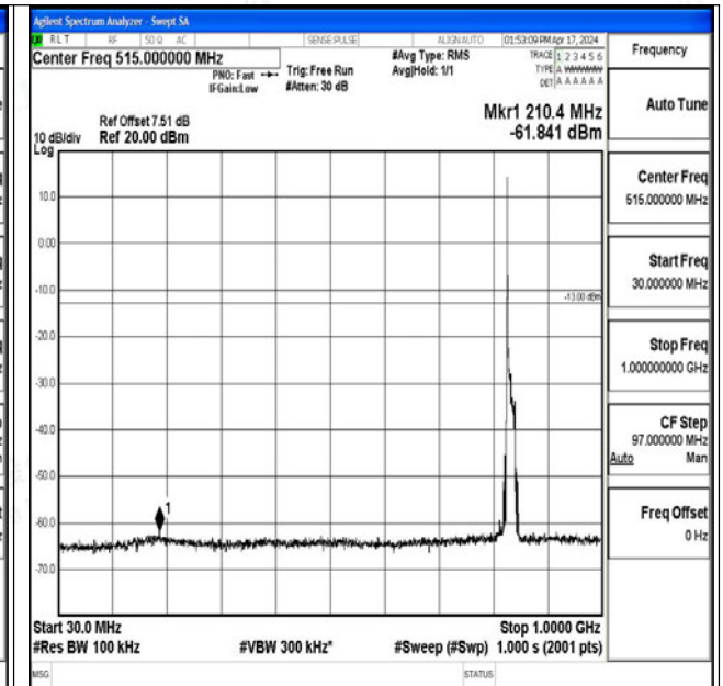
Band26_15MHz_16QAM_26915_1RB#0_30~1000_30~1000
