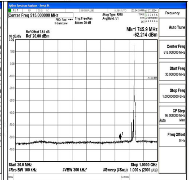
Band26_10MHz_16QAM_26990_1RB#0_30~1000_30~1000
