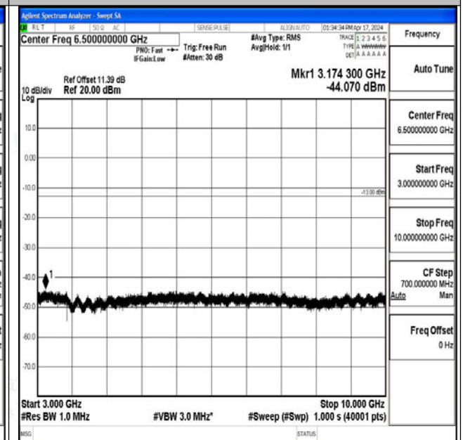
Band26_10MHz_16QAM_26990_1RB#0_3000~10000_3000~10000
