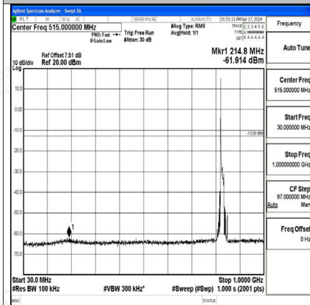
Band26_15MHz_QPSK_26865_1RB#0_30~1000_30~10 00
