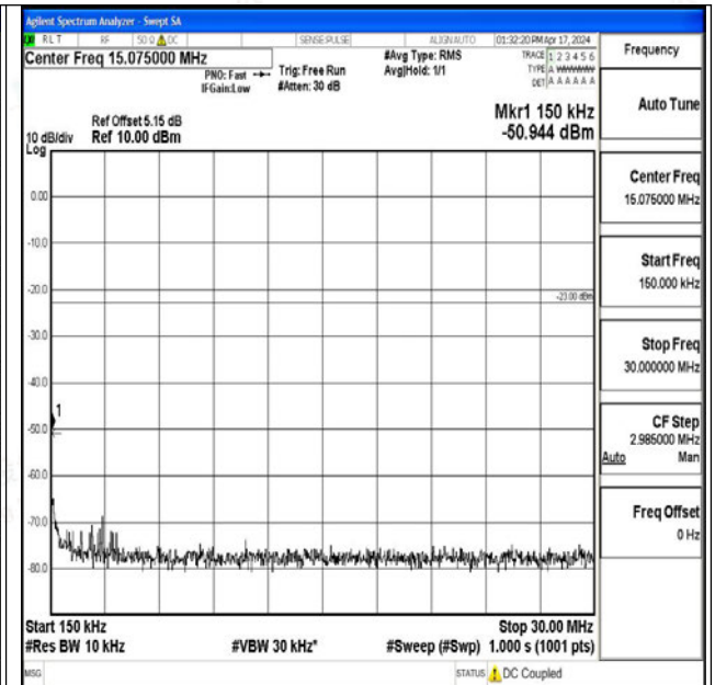
Band26_10MHz_QPSK_26915_1RB#0_0.15~30_0.15~3 0
