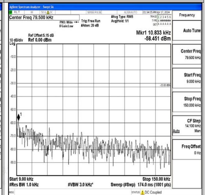
Band26_10MHz_16QAM_26990_1RB#0_0.009~0.15_0.009~0.15
