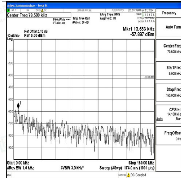
Band26_15MHz_QPSK_26965_1RB#0_0.009~0.15_0.00 9~0.15
