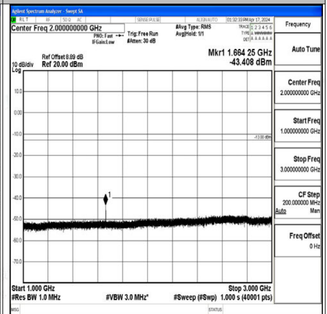
Band26_10MHz_QPSK_26915_1RB#0_1000~3000_100 0~3000
