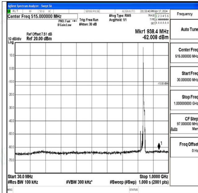
Band26_10MHz_QPSK_26990_1RB#0_30~1000_30~1000
