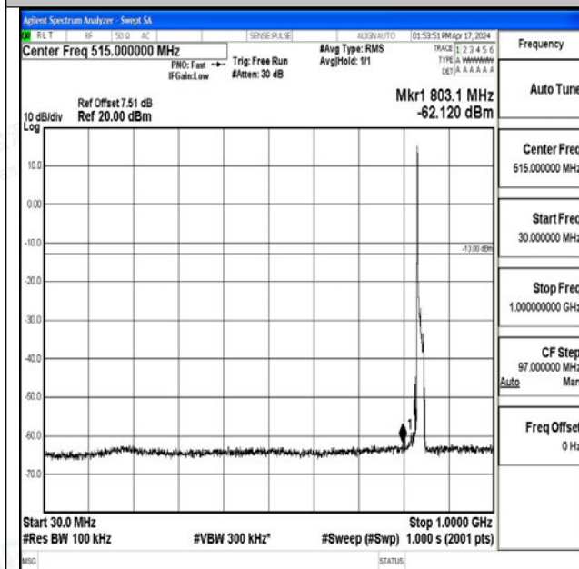
Band26_15MHz_QPSK_26965_1RB#0_30~1000_30~10 00
