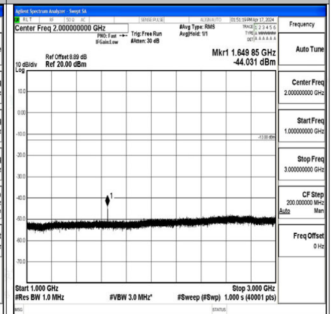
Band26_15MHz_QPSK_26865_1RB#0_1000~3000_100 0~3000
