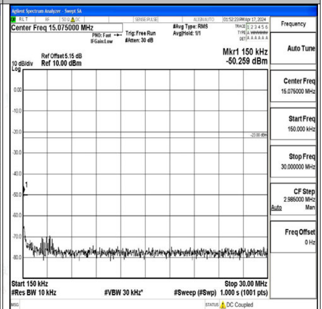
Band26_15MHz_QPSK_26915_1RB#0_0.15~30_0.15~3 0
