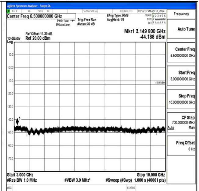
Band26_15MHz_16QAM_26865_1RB#0_3000~10000_3 000~10000
