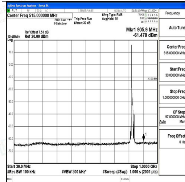
Band26_10MHz_QPSK_26840_1RB#0_30~1000_30~1000
