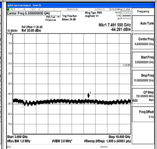
Band26_15MHz_16QAM_26915_1RB#0_3000~10000_3000~10000
