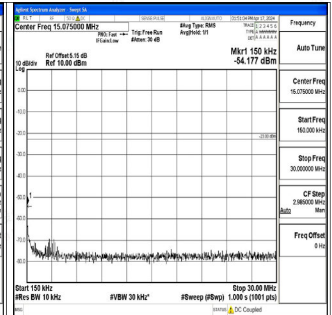
Band26_15MHz_QPSK_26865_1RB#0_0.15~30_0.15~3 0
