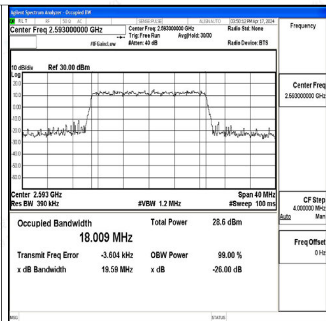
Band41-20MHz-16QAM-40620-100RB#0-PASS
