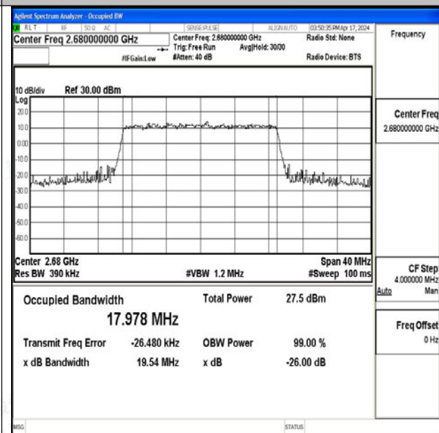
Band41-20MHz-16QAM-41490-100RB#0-PASS
