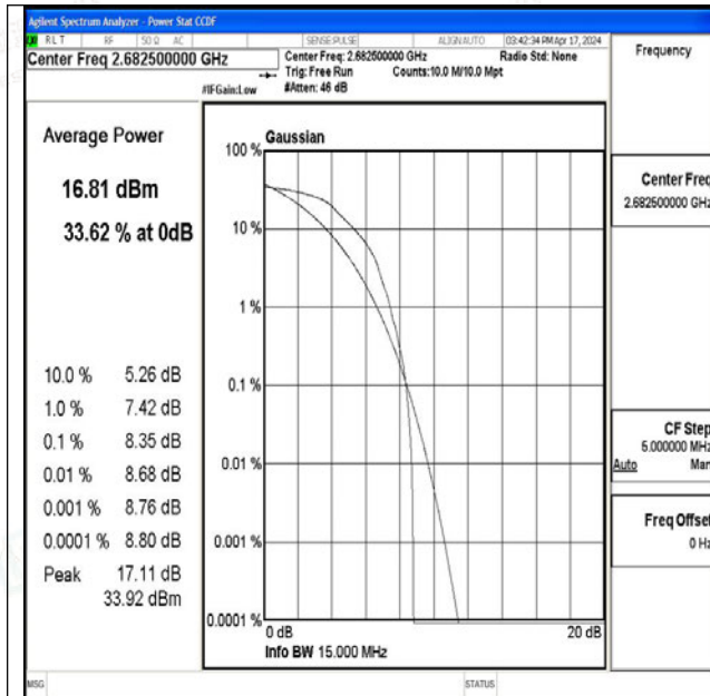
Band41-15MHz-QPSK-41515-1RB#0-PASS
