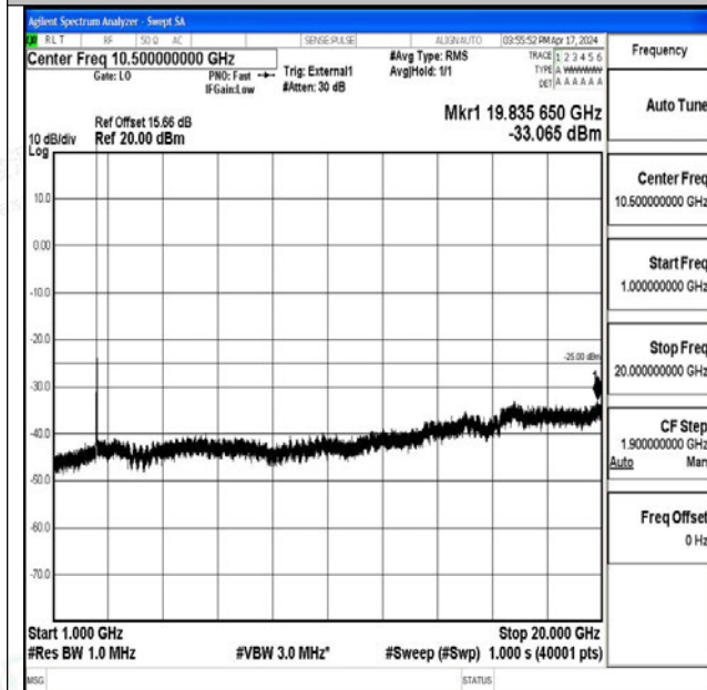
Band41_20MHz_16QAM_39750_1RB#0_1000~20000_1000~20000
