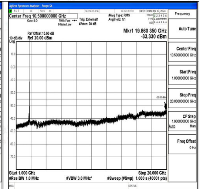
Band41_20MHz_QPSK_41490_1RB#0_1000~20000_1000~20000
