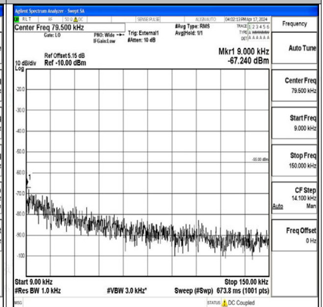
Band41_20MHz_16QAM_41490_1RB#0_0.009~0.15_0.009~0.15
