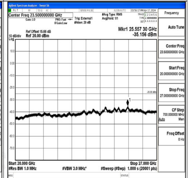
Band41_20MHz_16QAM_39750_1RB#0_20000~27000_20000~27000
