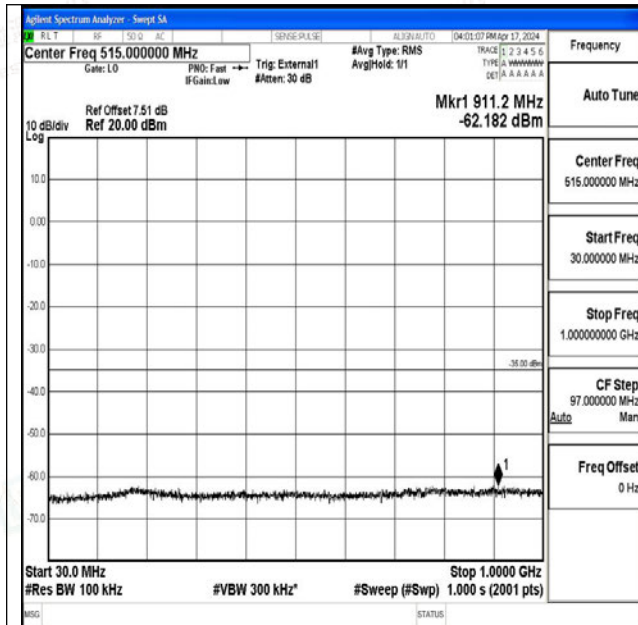
Band41_20MHz_QPSK_41490_1RB#0_30~1000_30~1000
