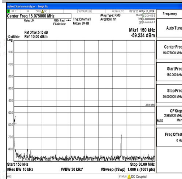
Band41_20MHz_16QAM_40620_1RB#0_0.15~30_0.15~30 30
