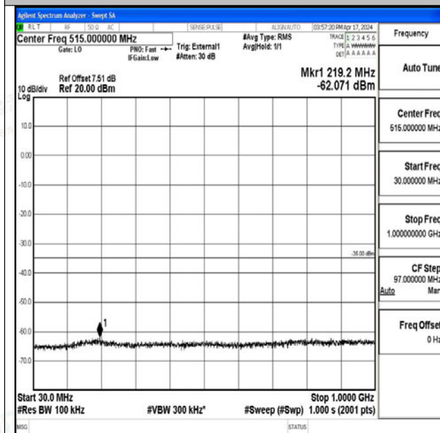
Band41_20MHz_QPSK_40620_1RB#0_30~1000_30~10 00
