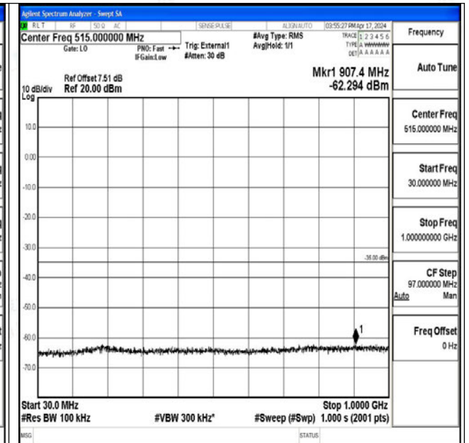
Band41_20MHz_16QAM_39750_1RB#0_30~1000_30~1000
