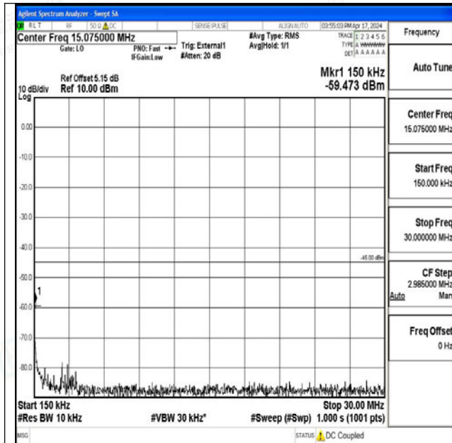
Band41_20MHz_16QAM_39750_1RB#0_0.15~30_0.15~30
