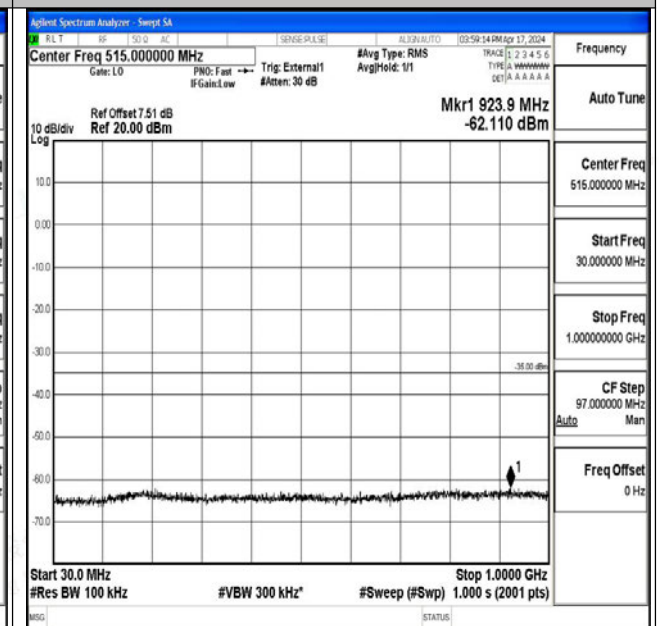
Band41_20MHz_16QAM_40620_1RB#0_30~1000_30~1000 000
