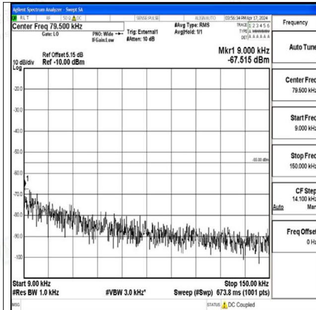
Band41_20MHz_QPSK_40620_1RB#0_0.009~0.15_0.00 9~0.15
