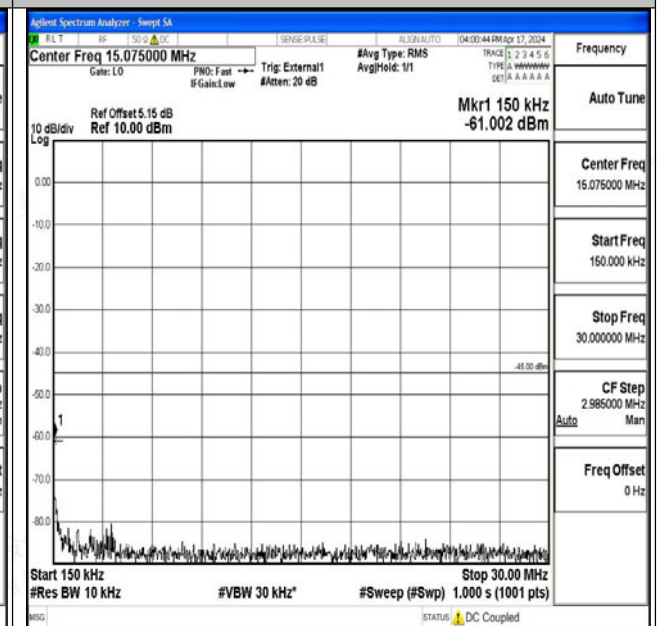
Band41_20MHz_QPSK_41490_1RB#0_0.15~30_0.15~3 0
