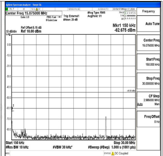
Band41_20MHz_QPSK_40620_1RB#0_0.15~30_0.15~3 0
