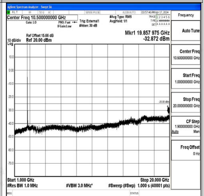
Band41_20MHz_QPSK_40620_1RB#0_1000~20000_10 00~20000
