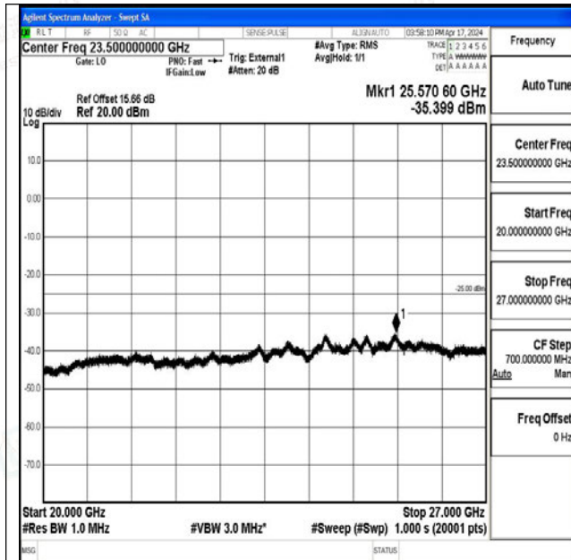
Band41_20MHz_QPSK_40620_1RB#0_20000~27000_2 0000~27000
