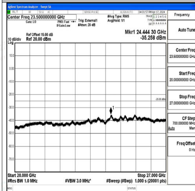
Band41_20MHz_QPSK_41490_1RB#0_20000~27000_20000~27000
