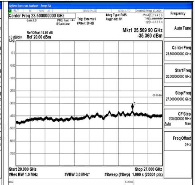
Band41_20MHz_16QAM_40620_1RB#0_20000~27000_ 20000~27000
