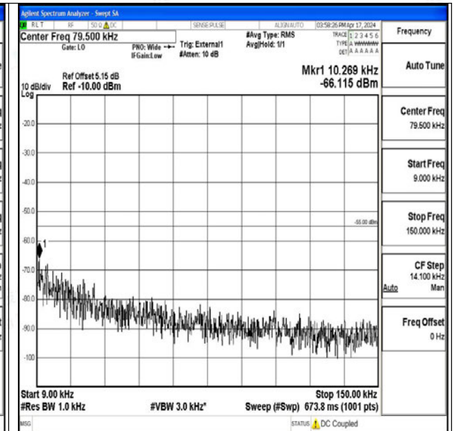
Band41_20MHz_16QAM_40620_1RB#0_0.009~0.15_0 009~0.15
