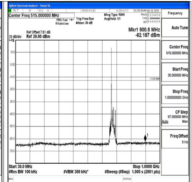
Band71_15MHz_16QAM_133297_1RB#0_30~1000_30~1000
