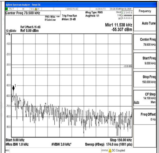
Band71_15MHz_16QAM_133197_1RB#0_0.009~0.15_0.009~0.15
