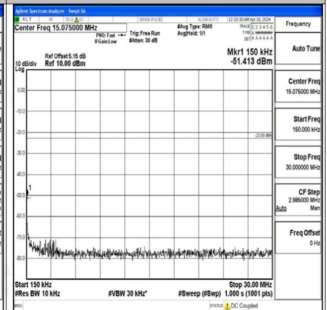
Band71_5MHz_QPSK_133447_1RB#0_0.15~30_0.15~3 0
