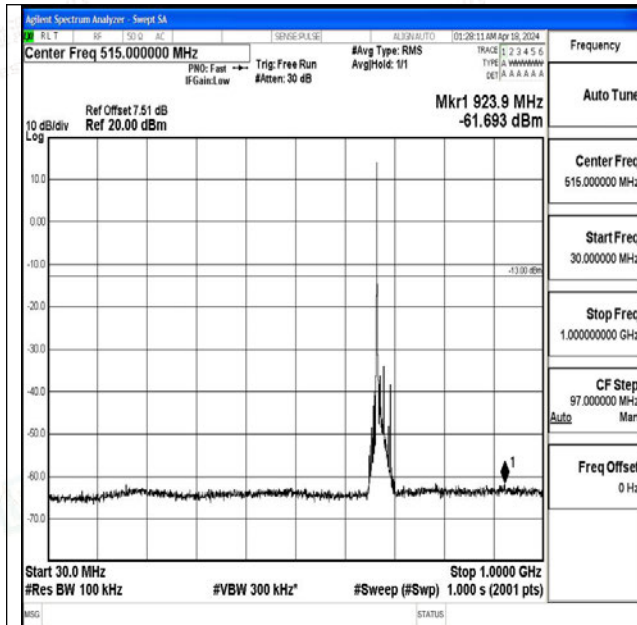
Band71_15MHz_QPSK_133297_1RB#0_30~1000_30~1000
