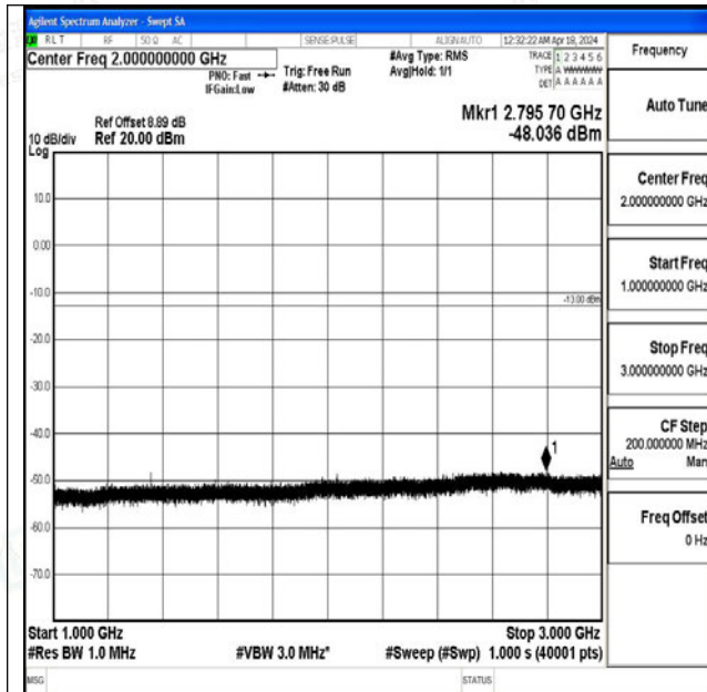
Band71_5MHz_16QAM_133297_1RB#0_1000~3000_10 00~3000
