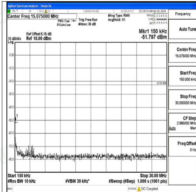
Band71_15MHz_16QAM_133297_1RB#0_0.15~30_0.15~30
