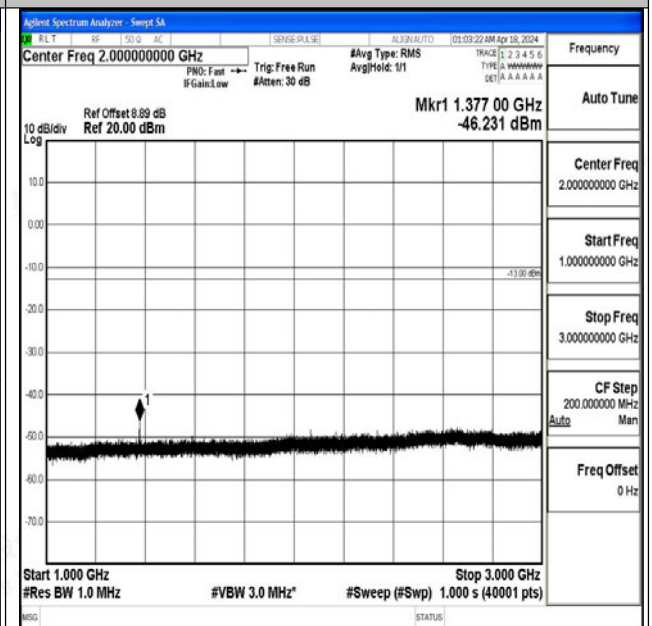
Band71_10MHz_QPSK_133422_1RB#0_1000~3000_10 00~3000
