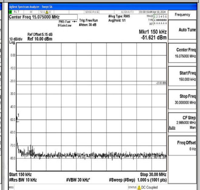
Band71_10MHz_QPSK_133297_1RB#0_0.15~30_0.15~30
