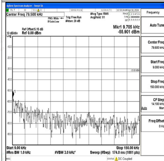
Band71_5MHz_QPSK_133447_1RB#0_0.009~0.15_0.00 9~0.15
