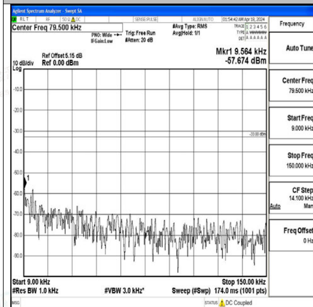
Band71_20MHz_QPSK_133222_1RB#0_0.009~0.15_0.0 09~0.15
