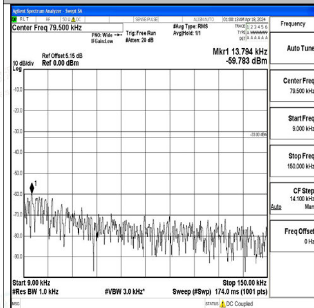
Band71_10MHz_QPSK_133297_1RB#0_0.009~0.15_0.009~0.15
