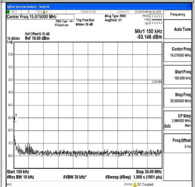
Band71_15MHz_QPSK_133297_1RB#0_0.15~30_0.15~30
