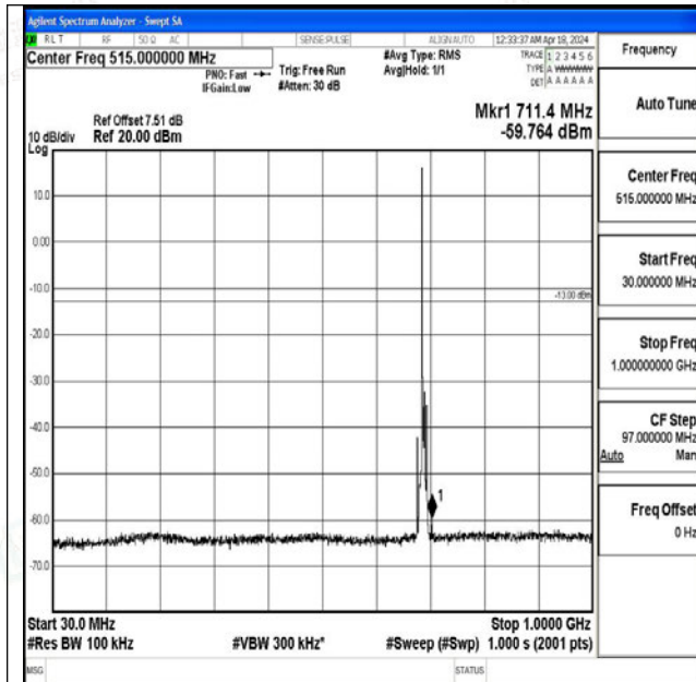
Band71_5MHz_QPSK_133447_1RB#0_30~1000_30~10 00
