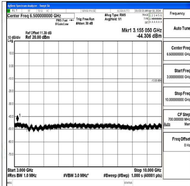
Band71_10MHz_QPSK_133422_1RB#0_3000~10000_3 000~10000
