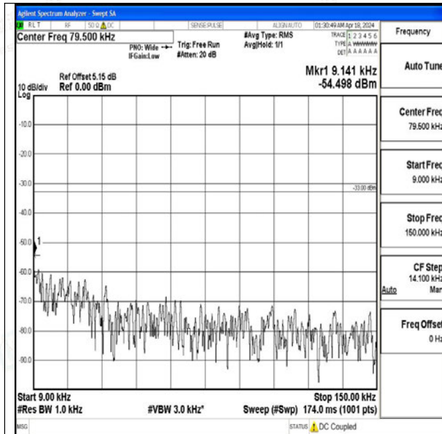
Band71_15MHz_QPSK_133397_1RB#0_0.009~0.15_0.09~0.15
