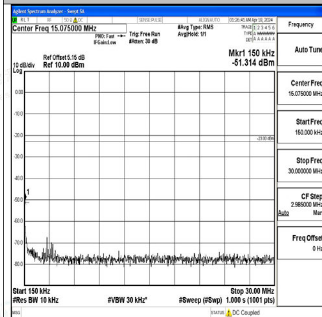
Band71_15MHz_16QAM_133197_1RB#0_0.15~30_0.15~30
