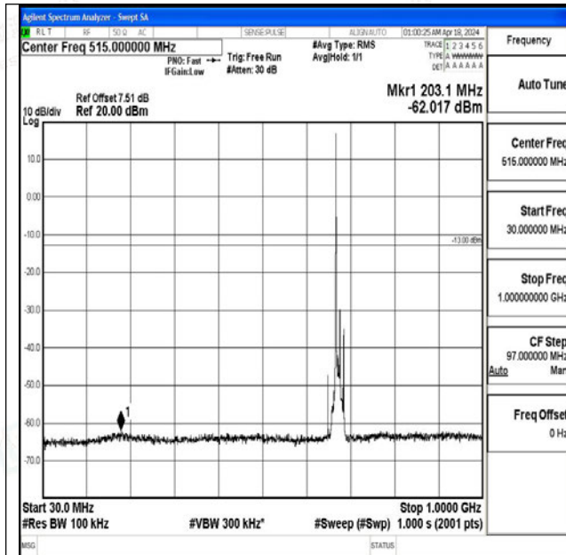
Band71_10MHz_QPSK_133297_1RB#0_30~1000_30~1000
