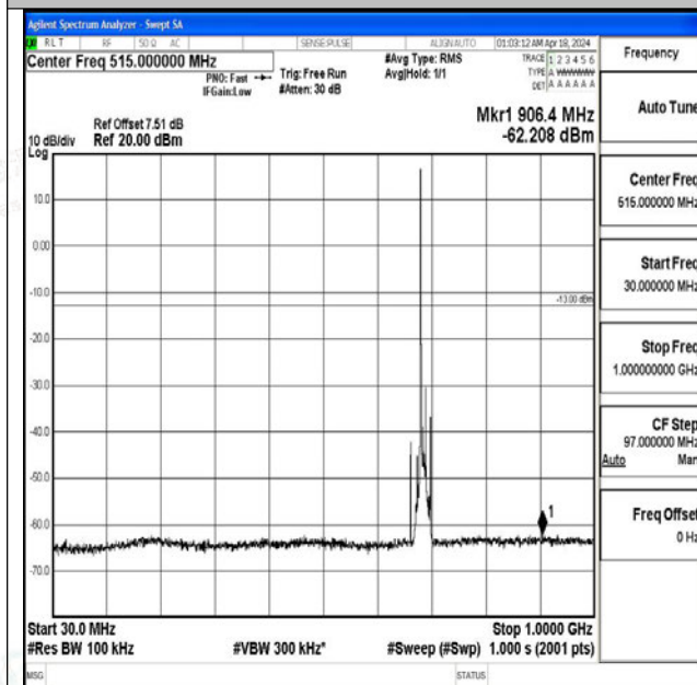
Band71_10MHz_QPSK_133422_1RB#0_30~1000_30~1 000
