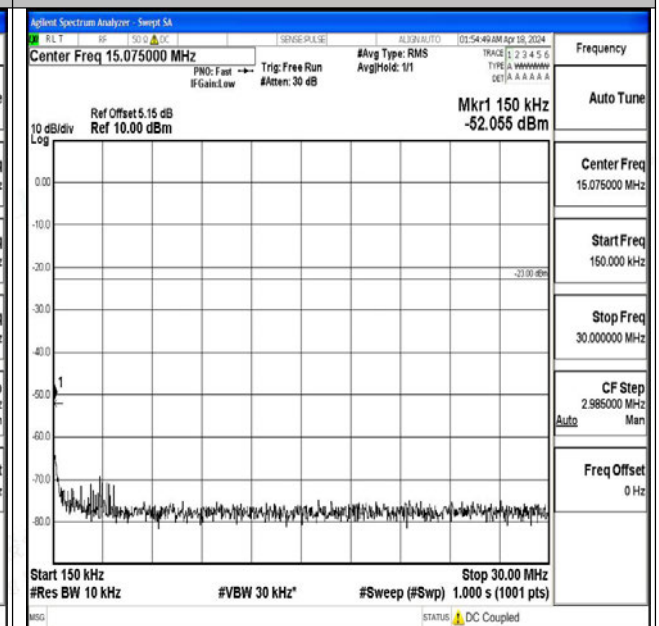
Band71_20MHz_QPSK_133222_1RB#0_0.15~30_0.15~ 30
