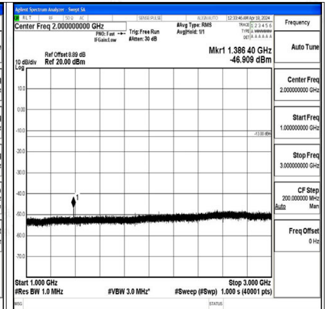
Band71_5MHz_QPSK_133447_1RB#0_1000~3000_100 0~3000
