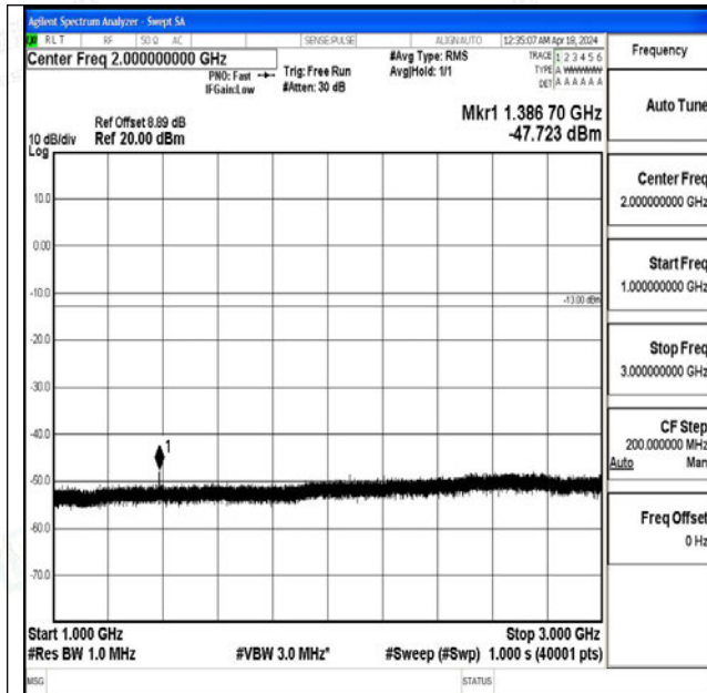
Band71_5MHz_16QAM_133447_1RB#0_1000~3000_10 00~3000
