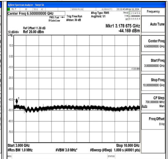
Band71_15MHz_16QAM_133397_1RB#0_3000~10000_ 3000~10000
