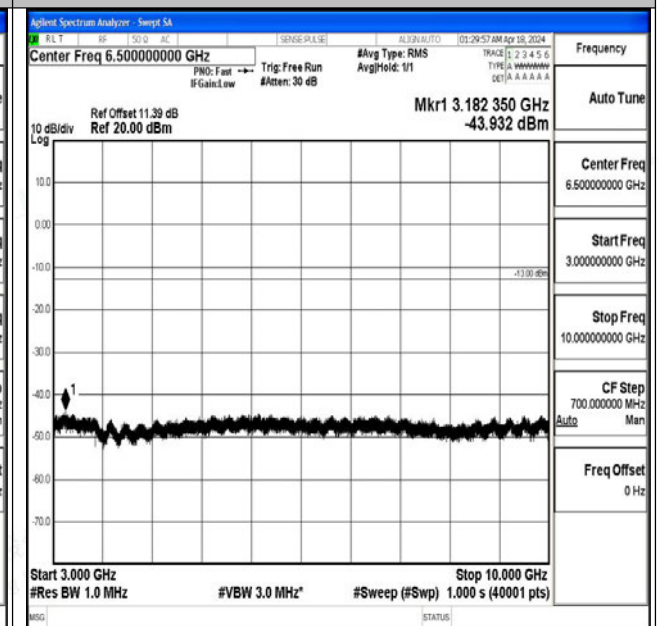
Band71_15MHz_16QAM_133297_1RB#0_3000~10000_3000~10000
