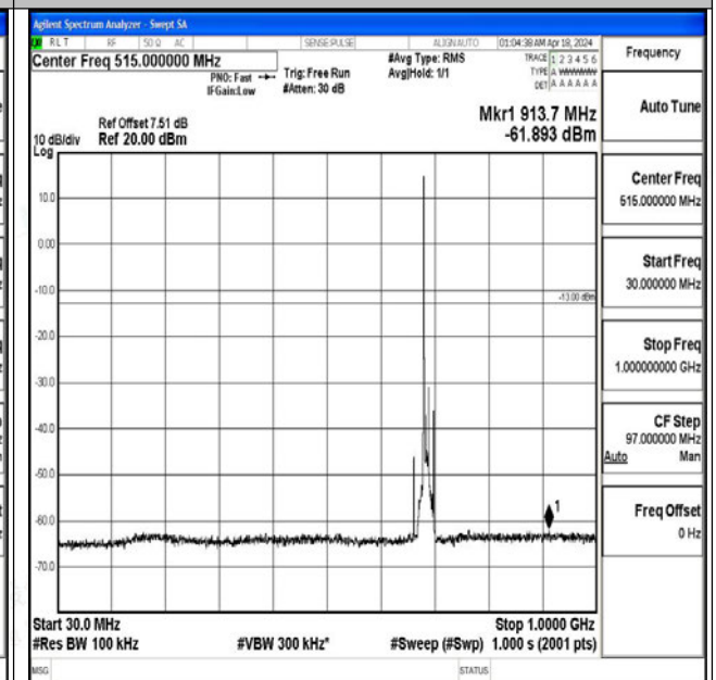
Band71_10MHz_16QAM_133422_1RB#0_30~1000_30~ 1000
