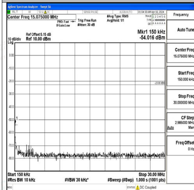
Band71_10MHz_16QAM_133422_1RB#0_0.15~30_0.15 ~30
