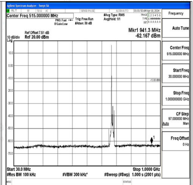
Band71_10MHz_16QAM_133297_1RB#0_30~1000_30~1000
