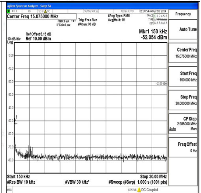
Band71_15MHz_QPSK_133397_1RB#0_0.15~30_0.15~30
