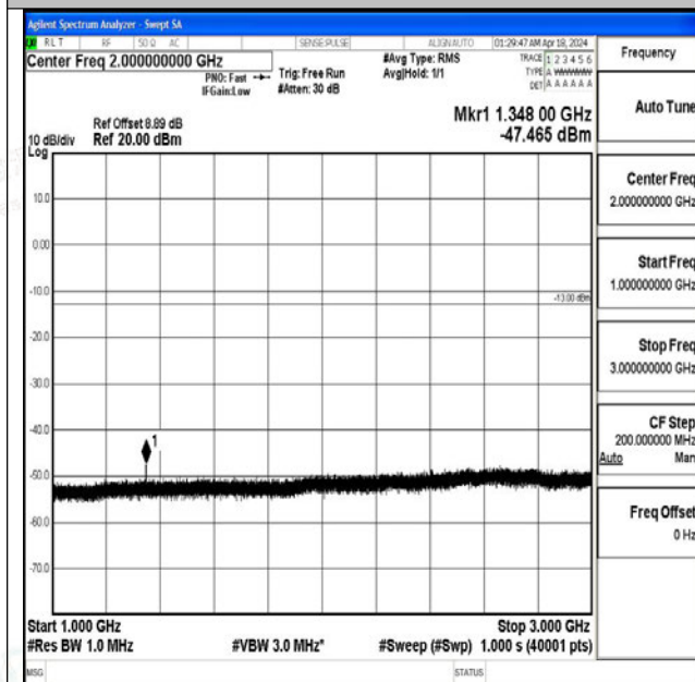
Band71_15MHz_16QAM_133297_1RB#0_1000~3000_1000~3000
