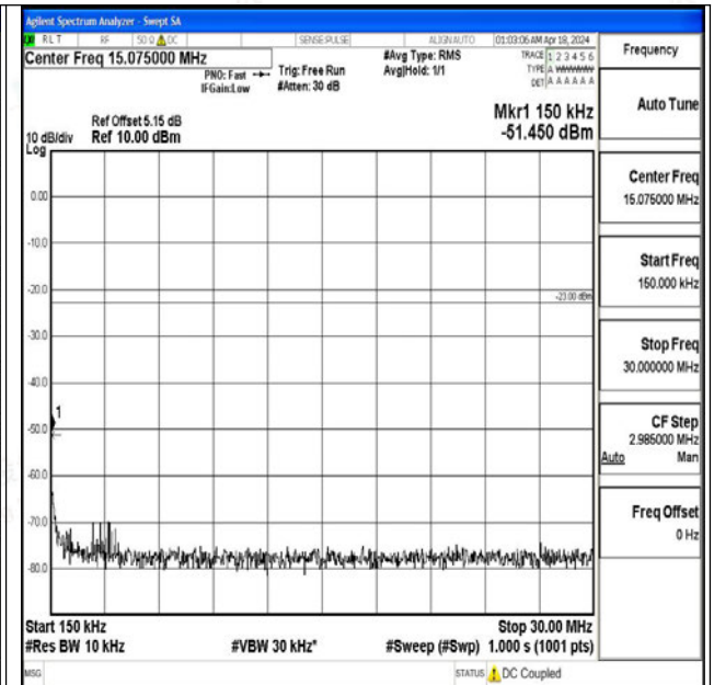
Band71_10MHz_QPSK_133422_1RB#0_0.15~30_0.15~ 30
