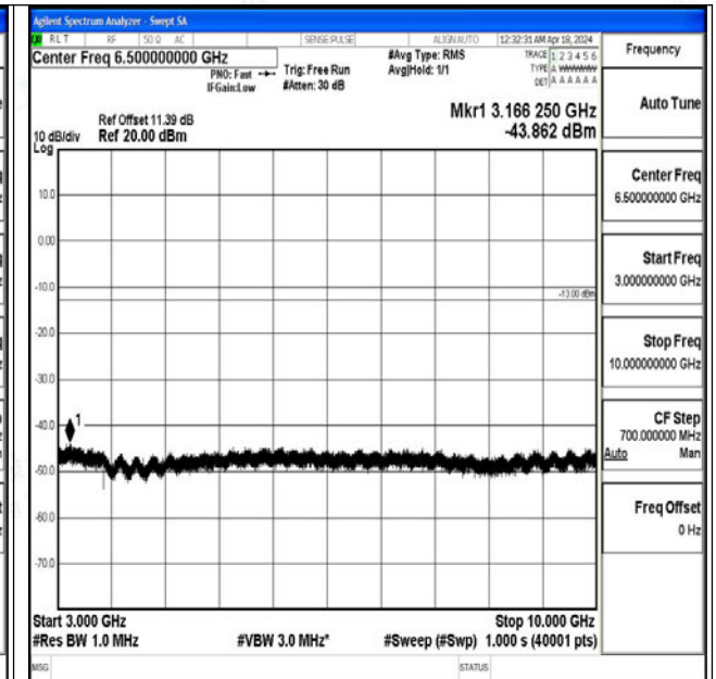
Band71_5MHz_16QAM_133297_1RB#0_3000~10000_3 000~10000
