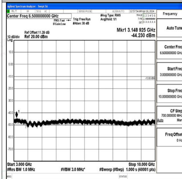
Band71_10MHz_QPSK_133172_1RB#0_3000~10000_3000~10000
