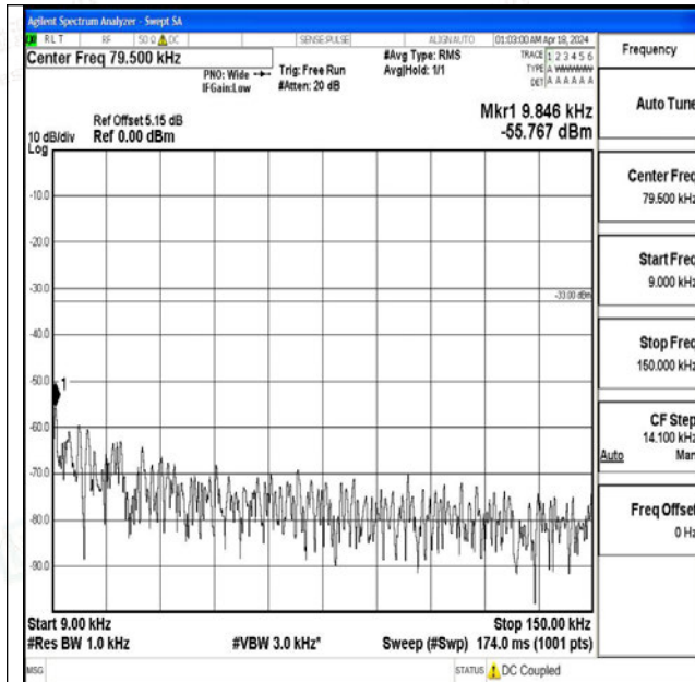
Band71_10MHz_QPSK_133422_1RB#0_0.009~0.15_0.0 09~0.15
