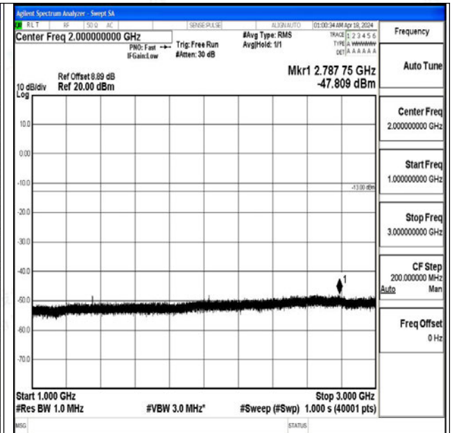
Band71_10MHz_QPSK_133297_1RB#0_1000~3000_1000~3000
