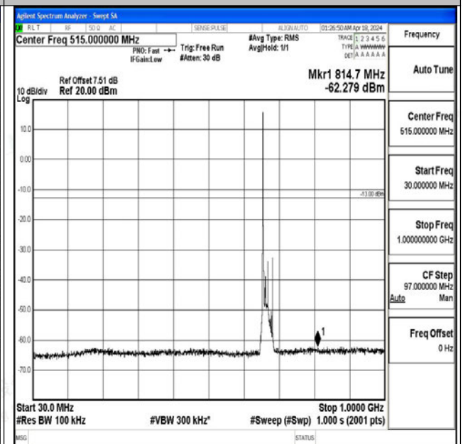
Band71_15MHz_16QAM_133197_1RB#0_30~1000_30~1000
