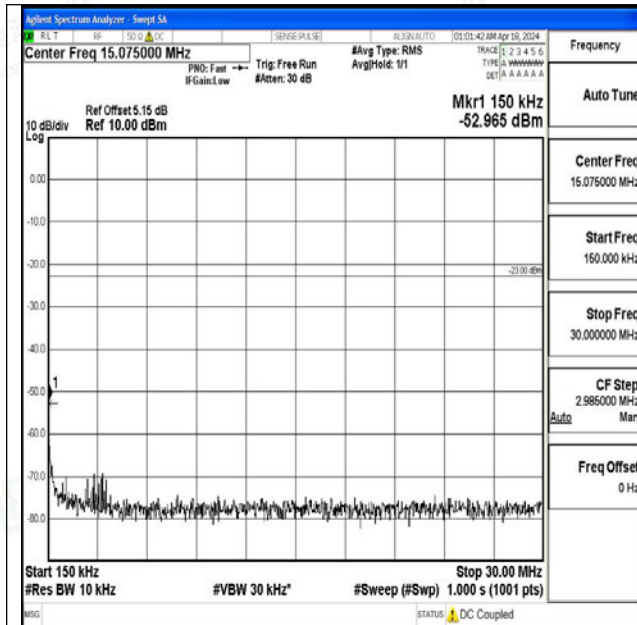
Band71_10MHz_16QAM_133297_1RB#0_0.15~30_0.15~30
