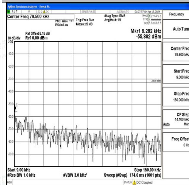
Band71_15MHz_QPSK_133297_1RB#0_0.009~0.15_0.009~0.15
