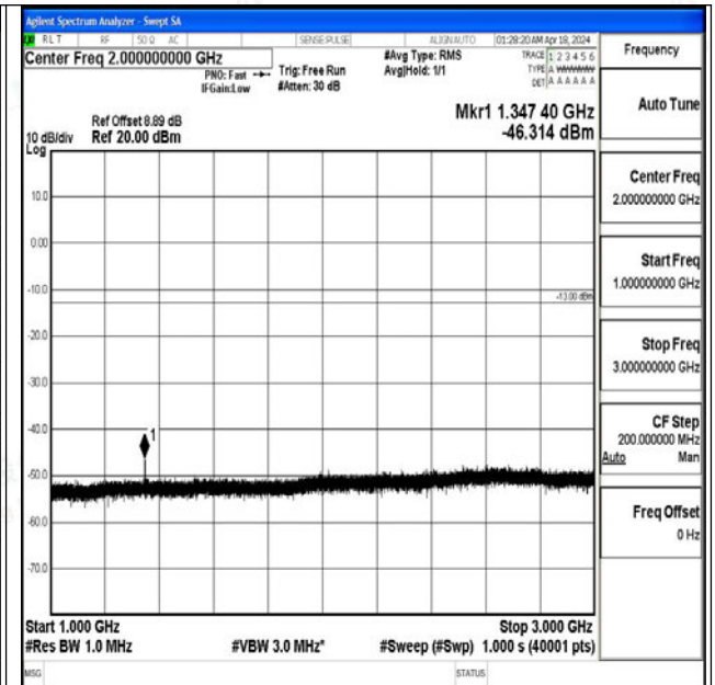
Band71_15MHz_QPSK_133297_1RB#0_1000~3000_1000~3000
