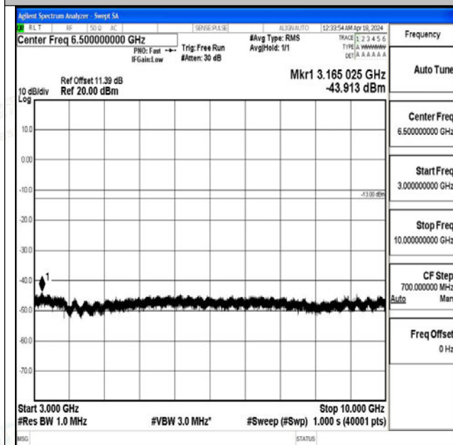
Band71_5MHz_QPSK_133447_1RB#0_3000~10000_30 00~10000
