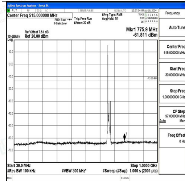
Band71_10MHz_QPSK_133172_1RB#0_30~1000_30~1000
