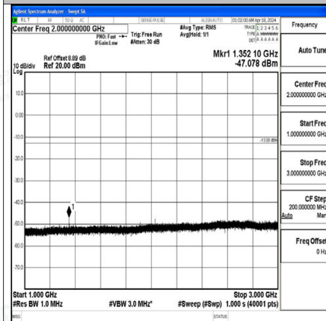
Band71_10MHz_16QAM_133297_1RB#0_1000~3000_1000~3000
