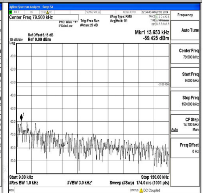
Band71_5MHz_16QAM_133447_1RB#0_0.009~0.15_0. 009~0.15
