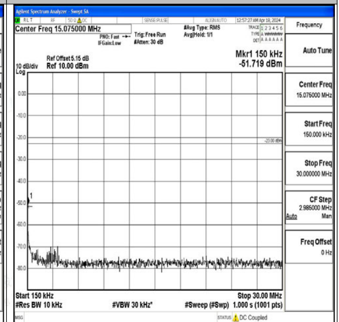
Band71_10MHz_QPSK_133172_1RB#0_0.15~30_0.15~ 30
