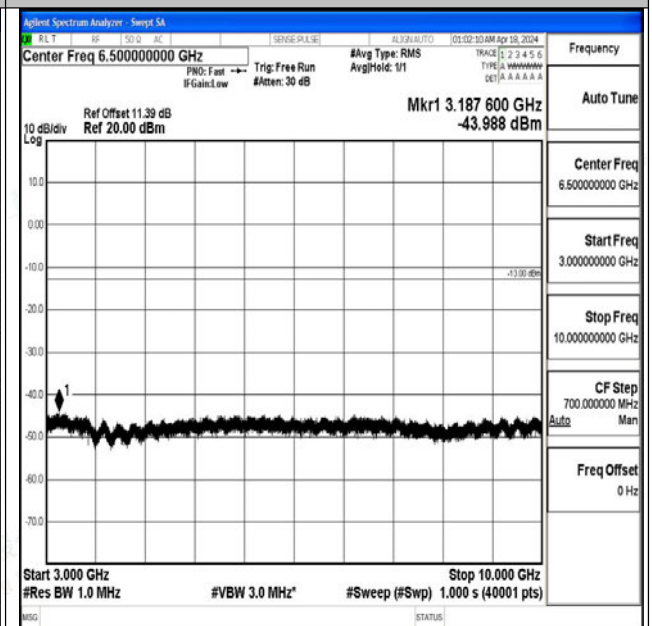
Band71_10MHz_16QAM_133297_1RB#0_3000~10000_3000~10000
