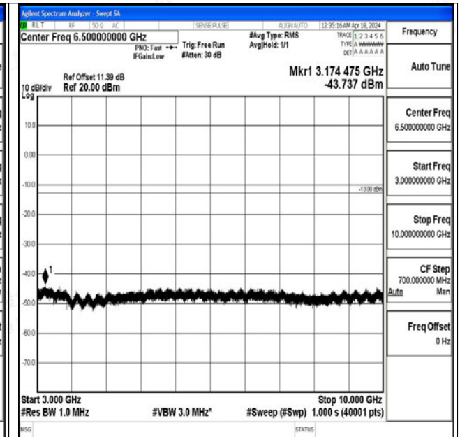
Band71_5MHz_16QAM_133447_1RB#0_3000~10000_3 000~10000
