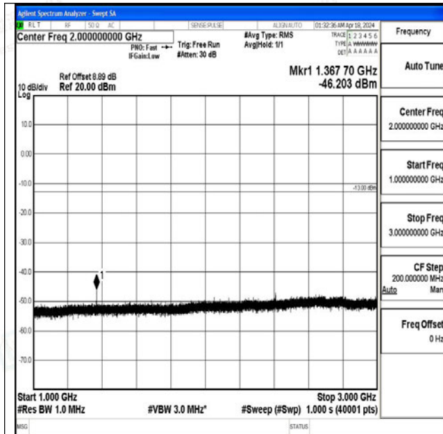
Band71_15MHz_16QAM_133397_1RB#0_1000~3000_1 000~3000
