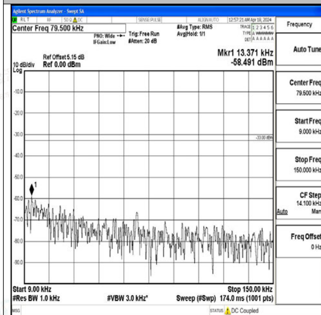
Band71_10MHz_QPSK_133172_1RB#0_0.009~0.15_0.0 09~0.15
