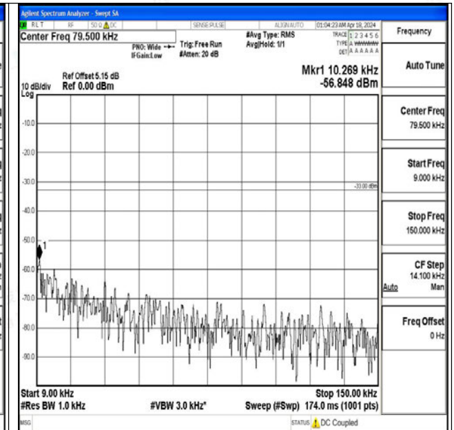
Band71_10MHz_16QAM_133422_1RB#0_0.009~0.15_0 .009~0.15
