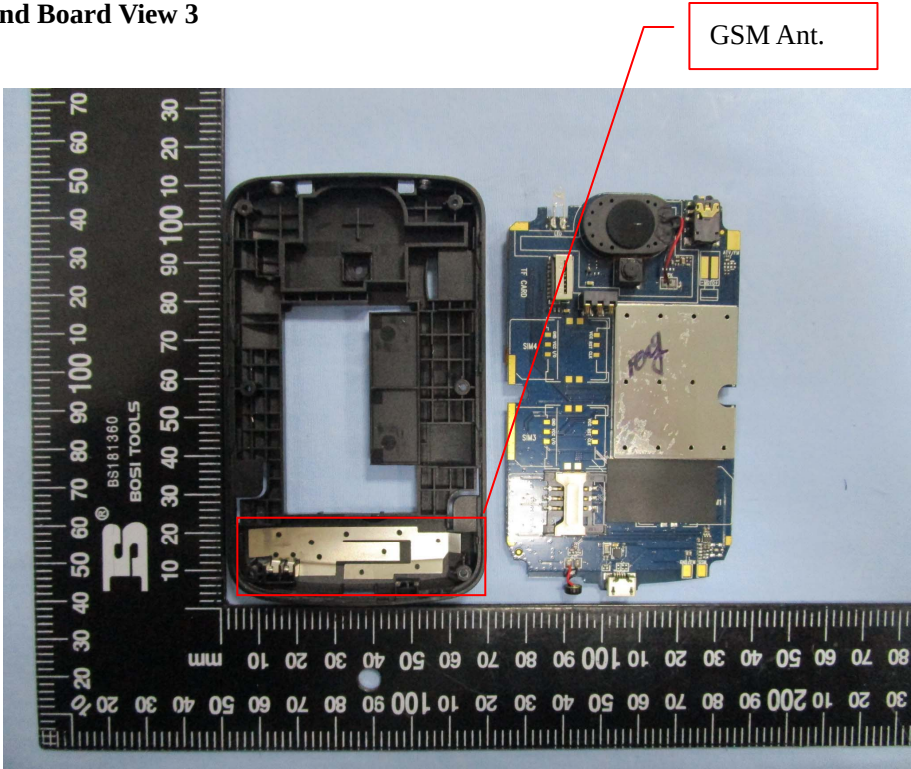
EUT Housing and Board View 3
