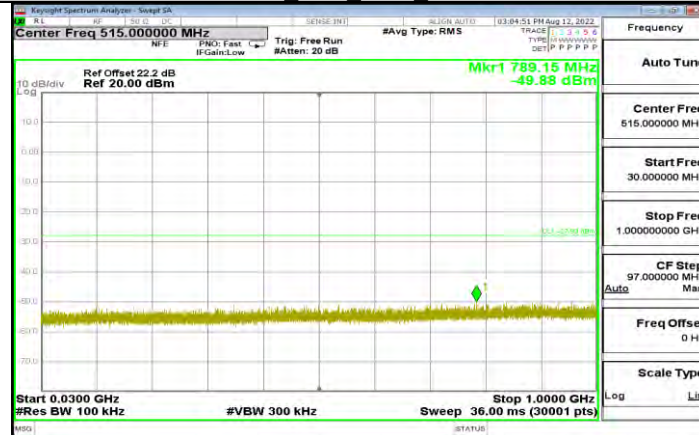
11N20SISO Ant1 2437 30~1000
