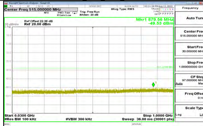
11N20SISO Ant1 2462 30~1000
