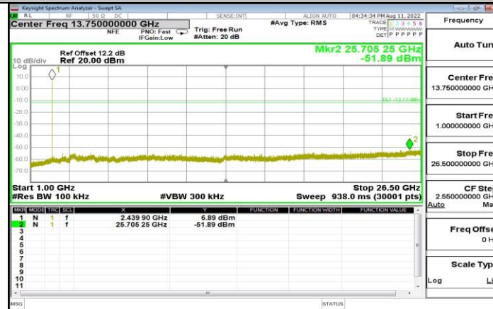
BLE_1M_Ant1_2440_1000~26500
