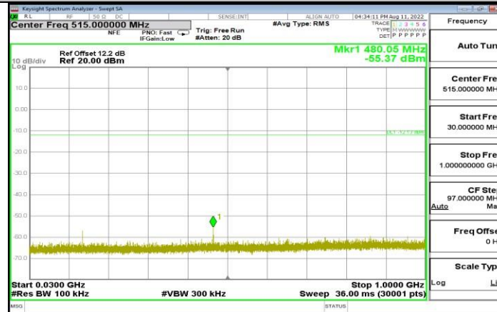
BLE_1M_Ant1_2440_30~1000
