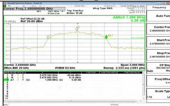
3DH5_Ant1_2480
