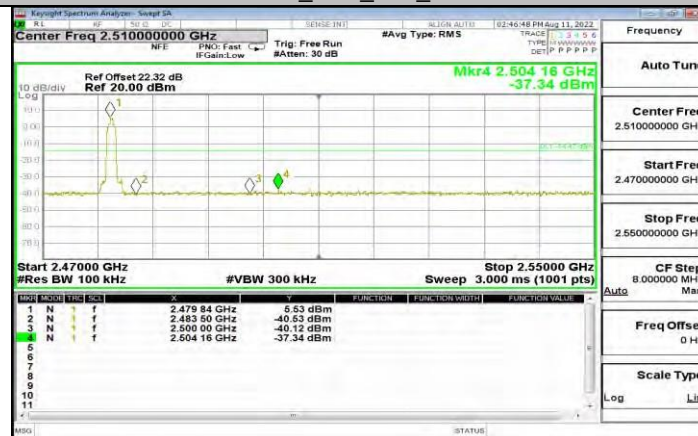
3DH5_Ant1_High_2480
