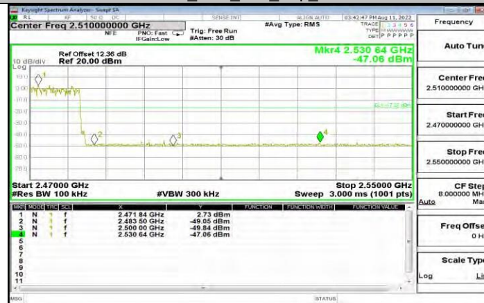
3DH5_Ant1_High_Hop_2480
