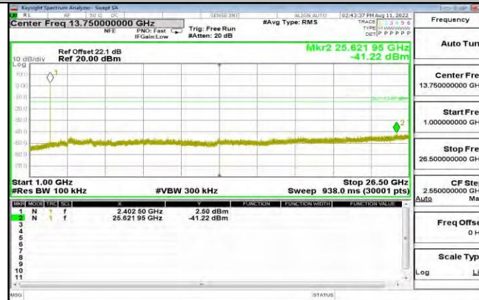
3DH5_Ant1_2402_1000~26500
