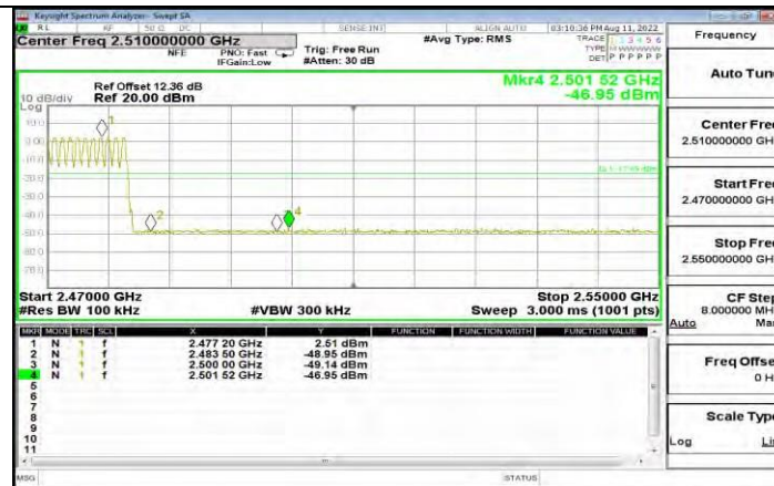
DH5_Ant1_High_Hop_2480
