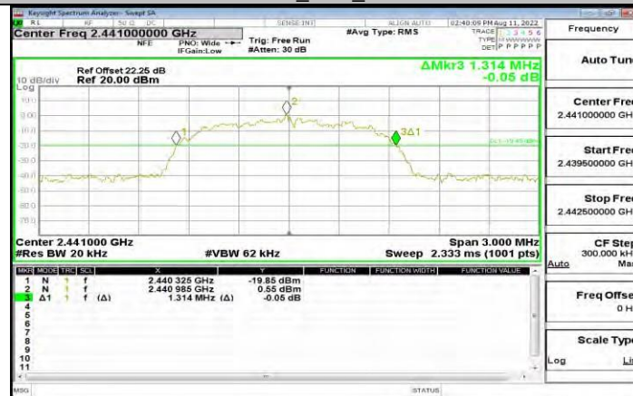
3DH5_Ant1_2441
