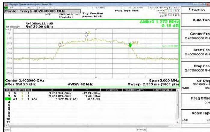
3DH5_Ant1_2402
