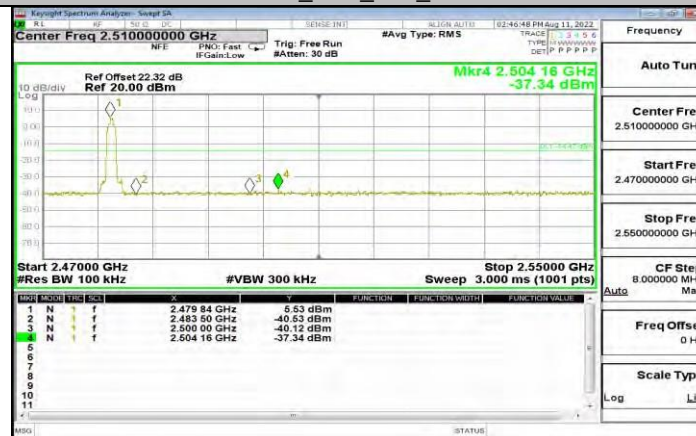
3DH5_Ant1_High_2480
