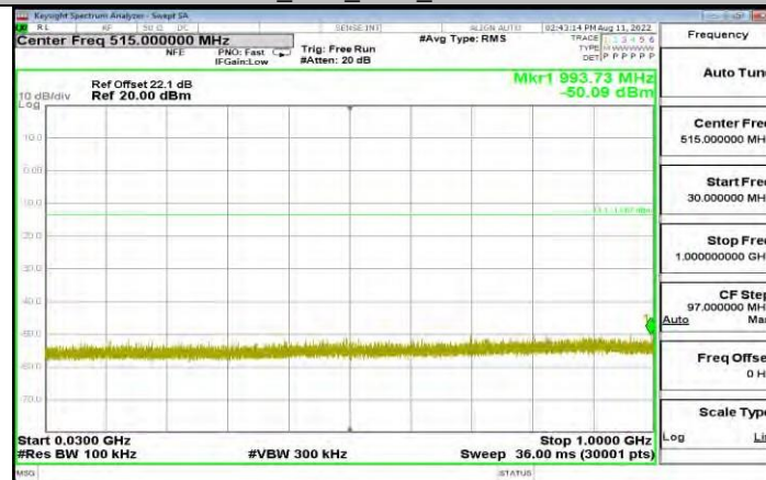
3DH5_Ant1_2402_30-1000
