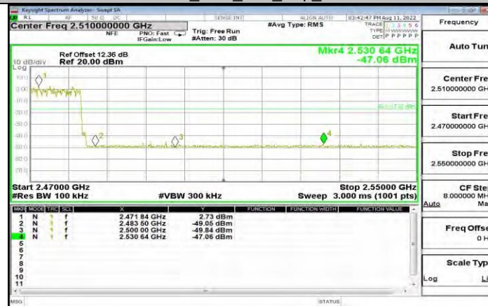
3DH5_Ant1_High_Hop_2480
