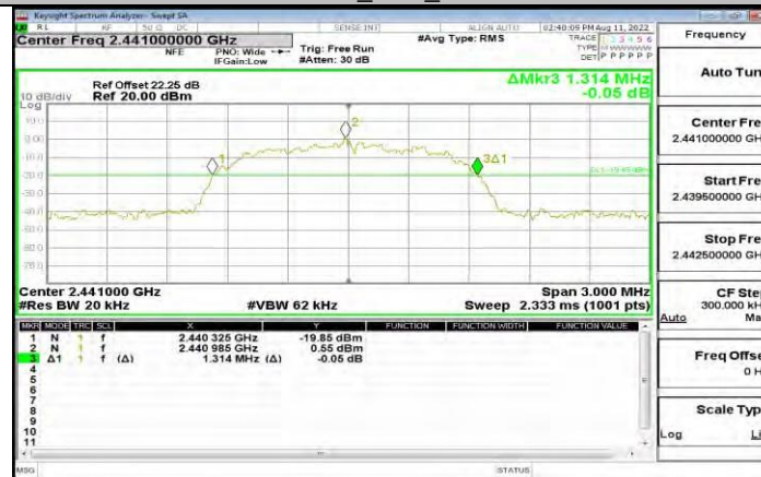
3DH5_Ant1_2441
