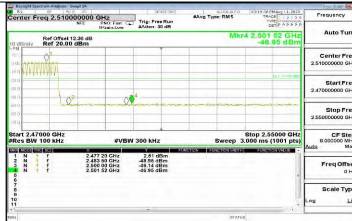
DH5_Ant1_High_Hop_2480
