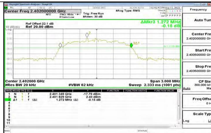
3DH5_Ant1_2402
