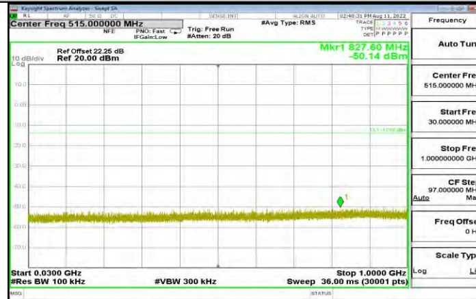
3DH5_Ant1_2441_30-1000
