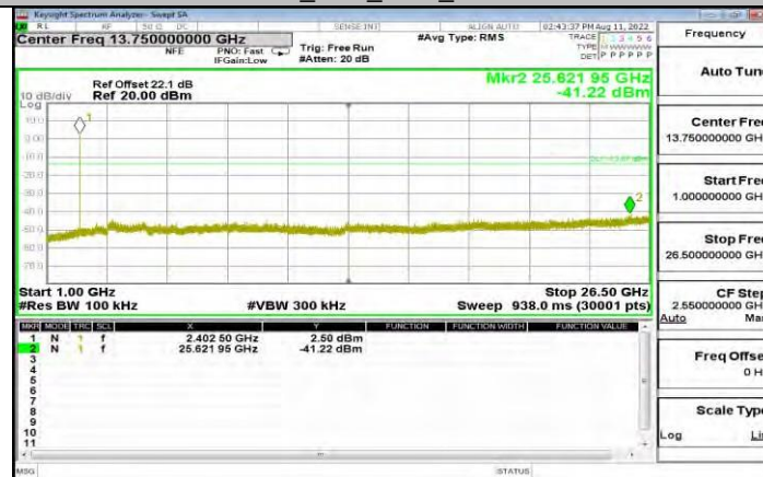
3DH5_Ant1_2402_1000-26500
