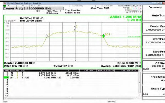
3DH5_Ant1_2480
