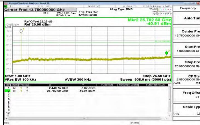
DH5_Ant1_2441_1000-26500
