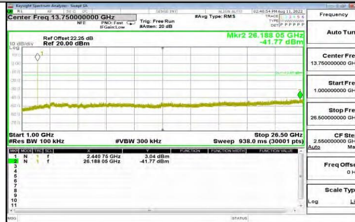
3DH5_Ant1_2441_1000-26500
