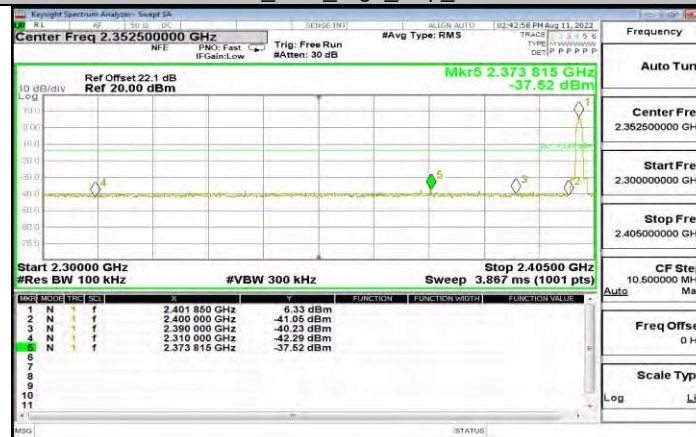
3DH5_Ant1_Low_2402
