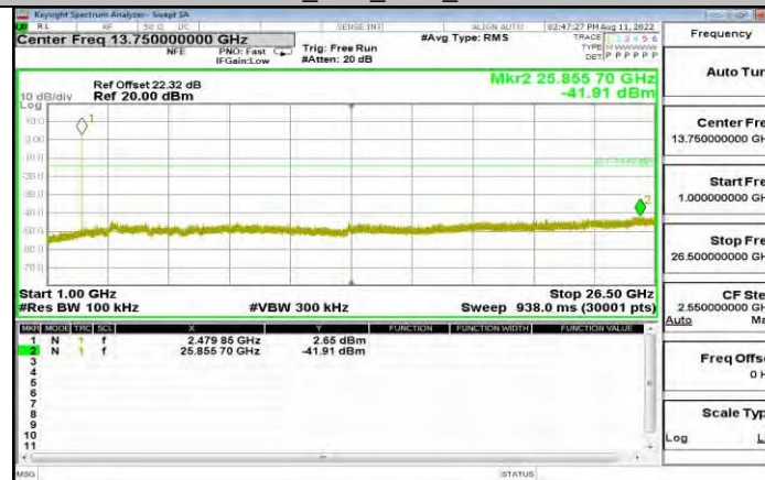
3DH5_Ant1_2480_1000-26500
