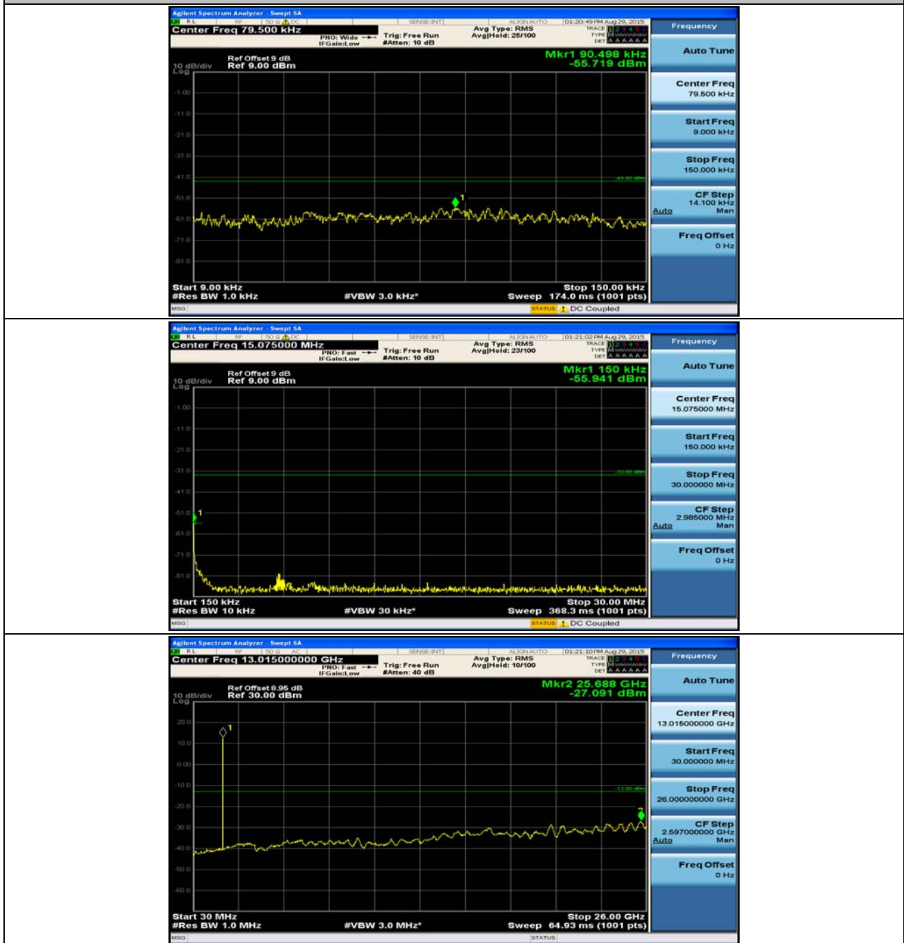
(Channel Bandwidth: 5 MHz)_HCH_QPSK_1RB#12
