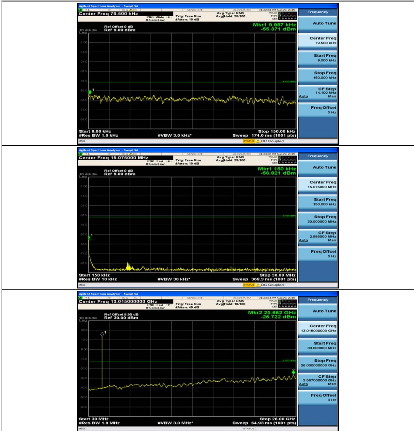
(Channel Bandwidth: 5 MHz)_HCH_16QAM_1RB#24
