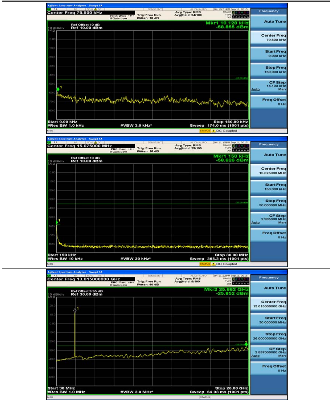
(Channel Bandwidth:15 MHz)_LCH_QPSK_1RB#74
