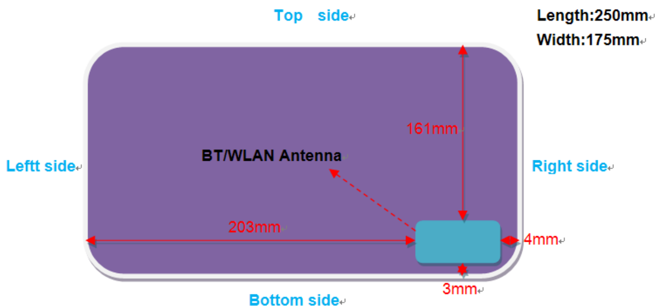
Figure 2: The antenna positions of the DUT
