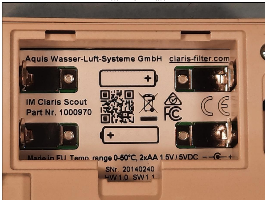
Photo 7: EUT A - label
