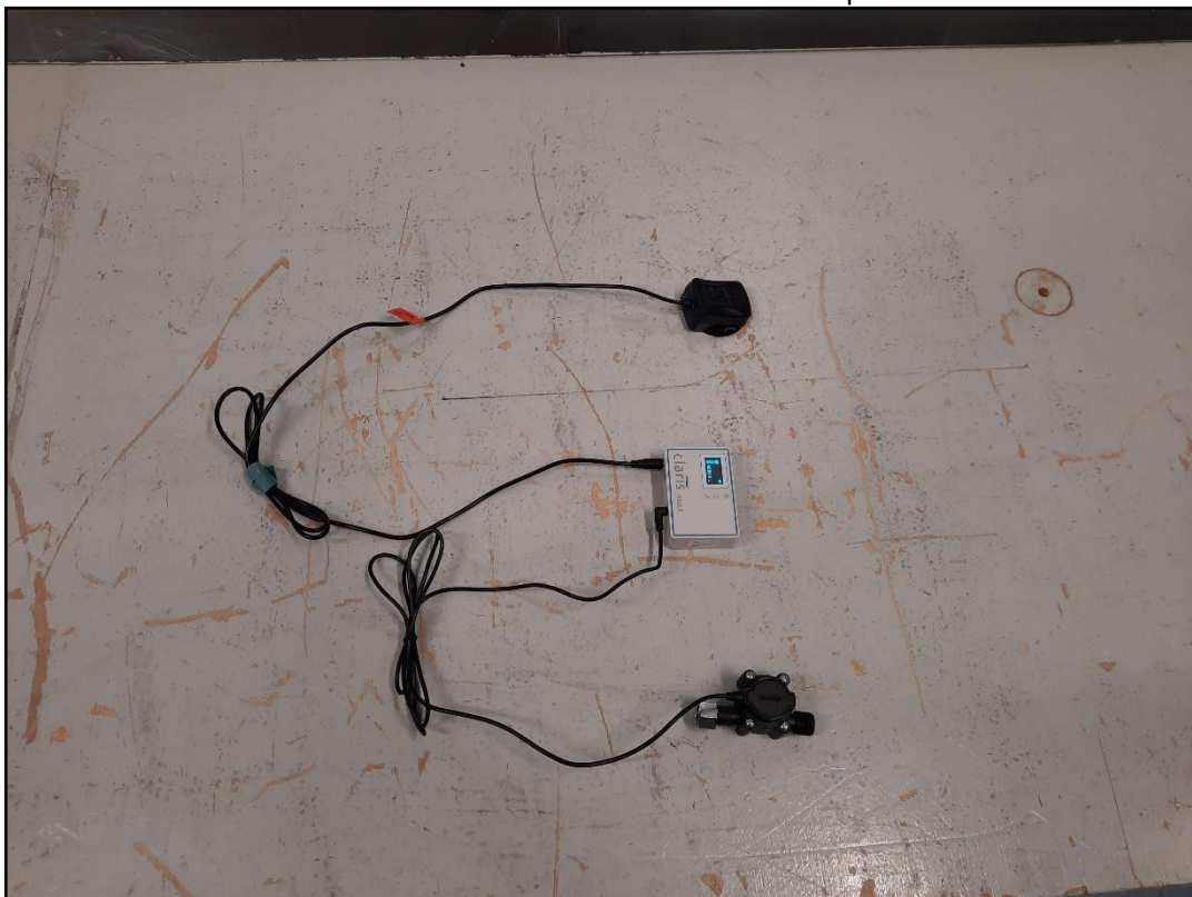
Photo 4: Conducted emission test setup
