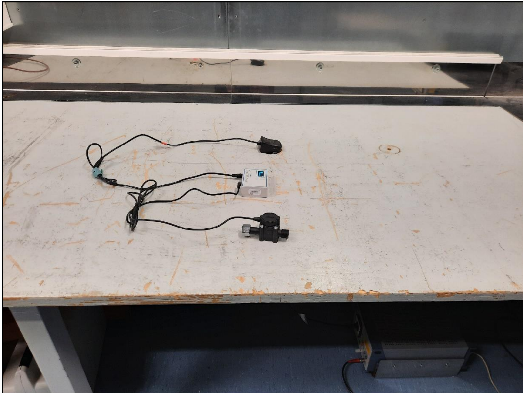
Photo 5: Conducted emission test setup
