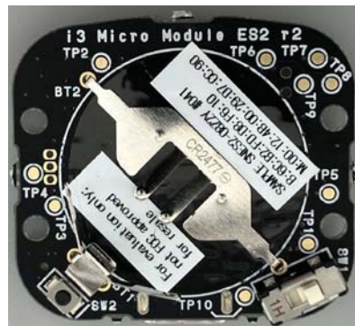
Wireless MCU on the PCB (Bottom)
