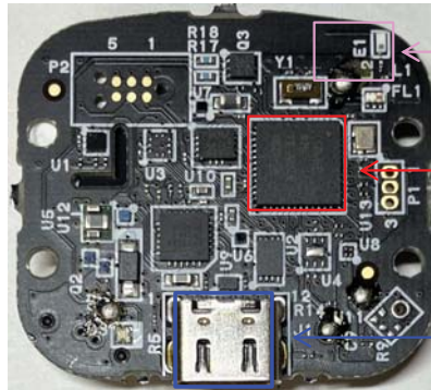
Wireless MCU on the PCB (Top)
