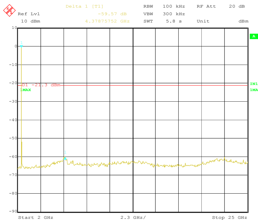
Figure 20 Conducted Spurious emission Plot between 2GHz–25GHz_Lower Ch
