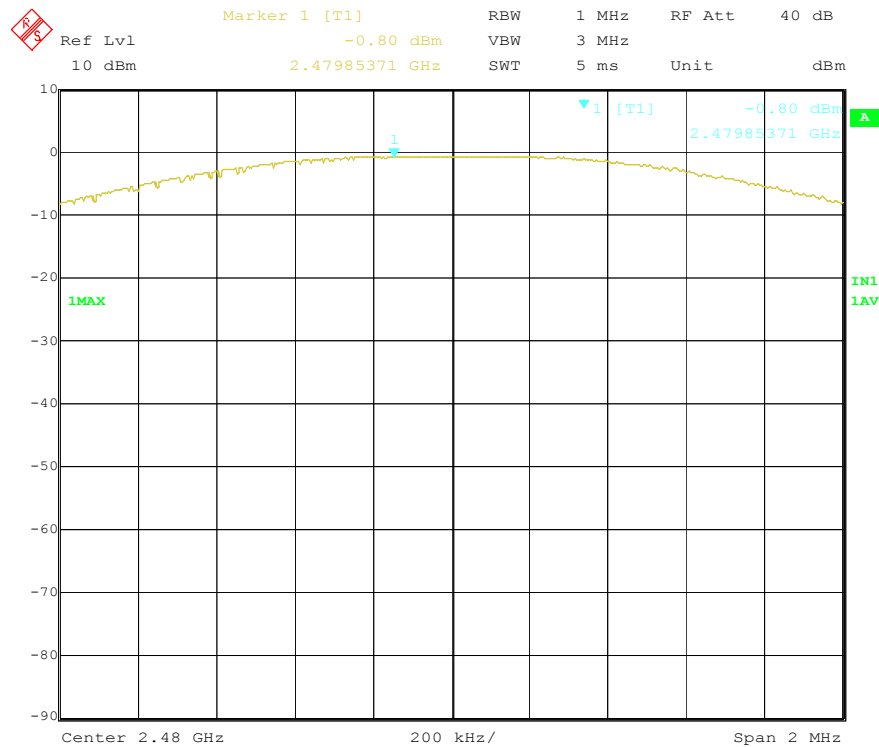
Figure 14 Maximum Peak Output Power(Higher ch_2480.000MHz)
