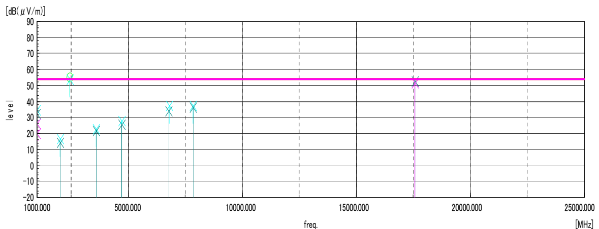
Figure 27 Radiated Emission (1-25GHz)
