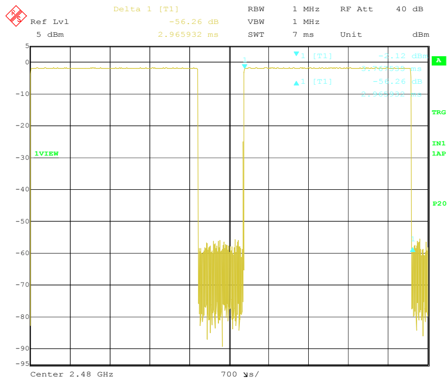
Figure 11 Package Transfer Time Plot_DH5
