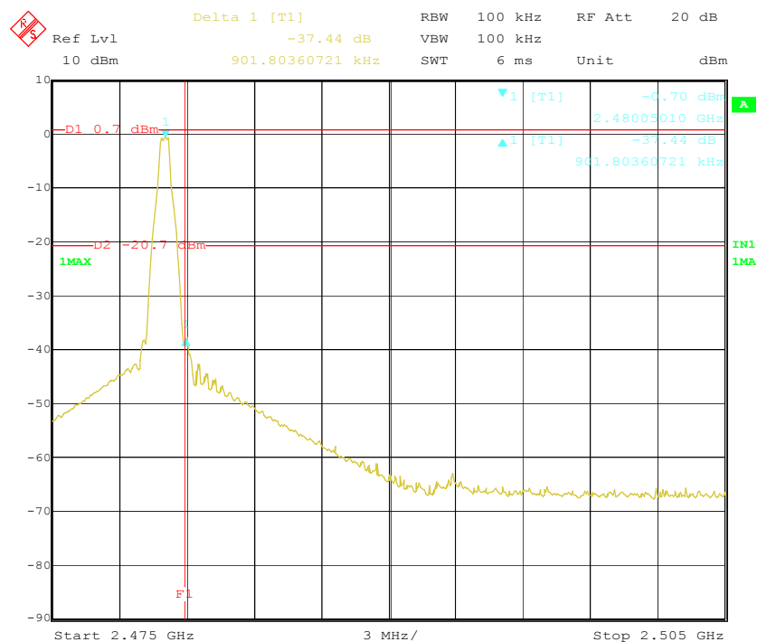
Figure 16 High Band Edge Plot on Channel 78_2480.000MHz
