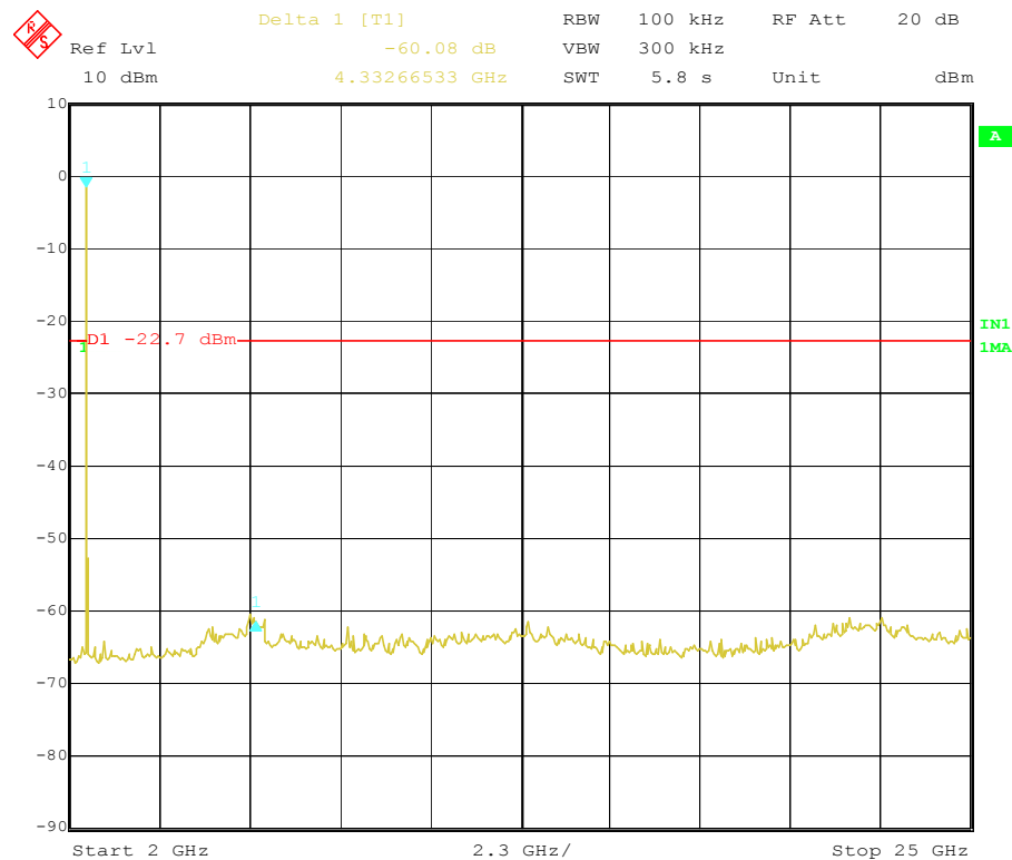
Figure 24 Conducted Spurious emission Plot between 2GHz–25GHz_Higher Ch
