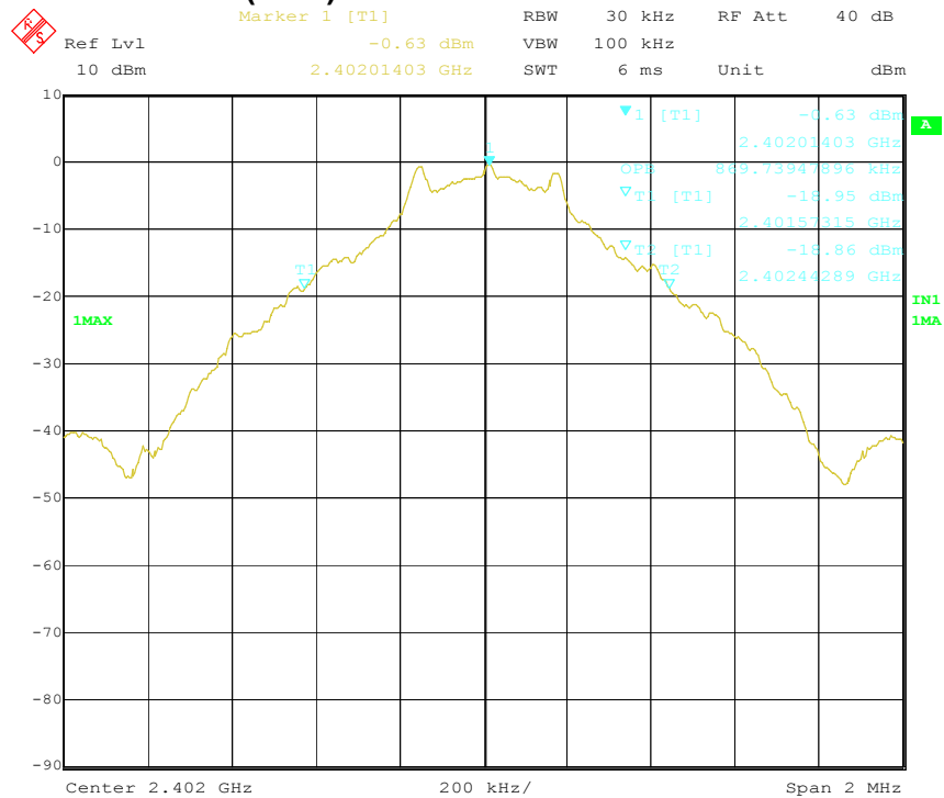
Figure 1 20dB Bandwidth(Lower ch_2402.000MHz)
