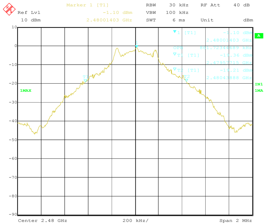
Figure 3 20dB Bandwidth(Higher ch_2480.000MHz)
