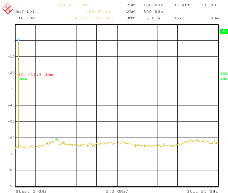
Figure 22 Conducted Spurious emission Plot between 2GHz–25GHz_Middle Ch
