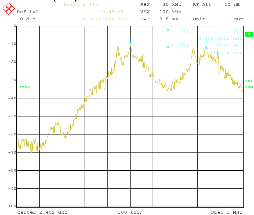
Figure 4 Carrier Frequency Separation (Lower)
