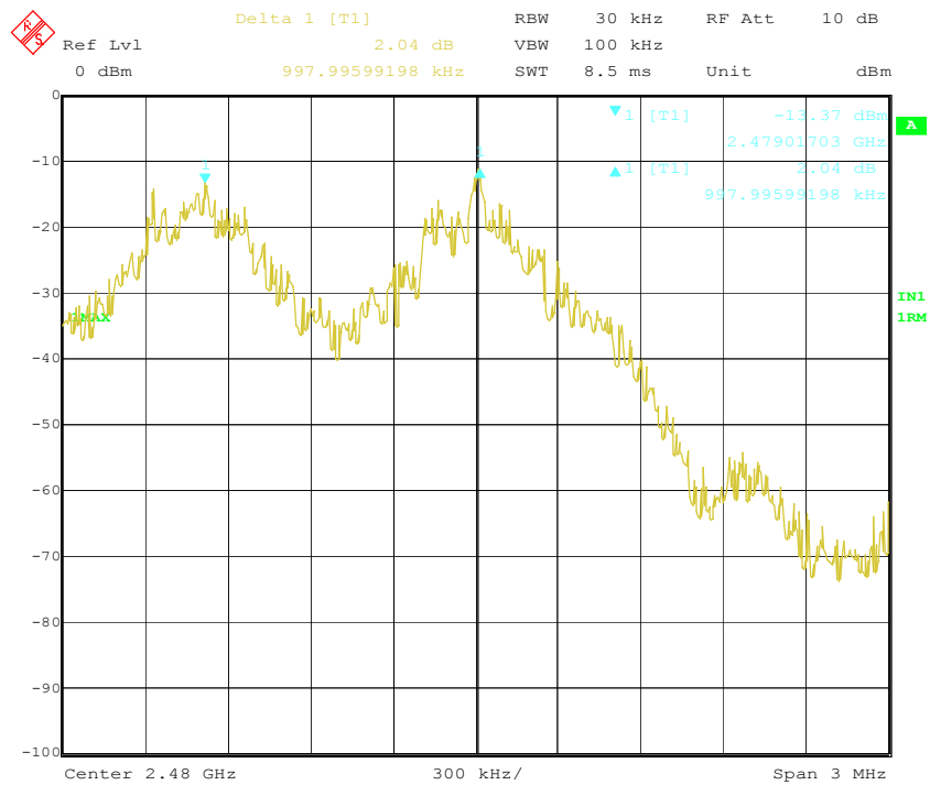
Figure 6 Carrier Frequency Separation (Higher)
