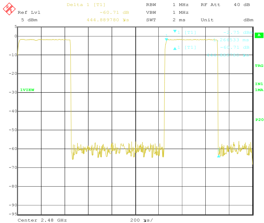
Figure 9 Package Transfer Time Plot_DH1
