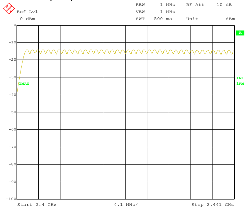
Figure 7 Number of Hopping Channel Plot channel 00-38
