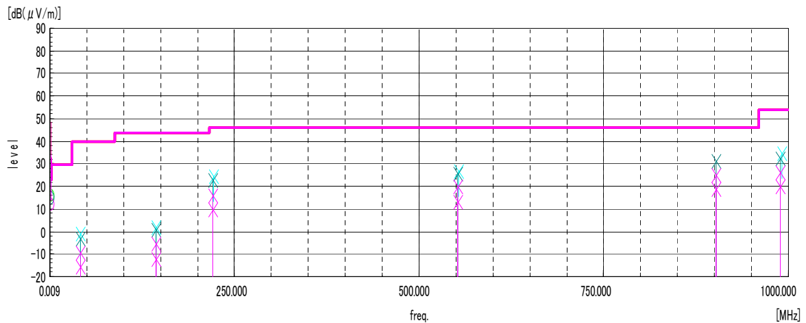
Figure 26 Radiated Emission (9kHz-1000MHz)
