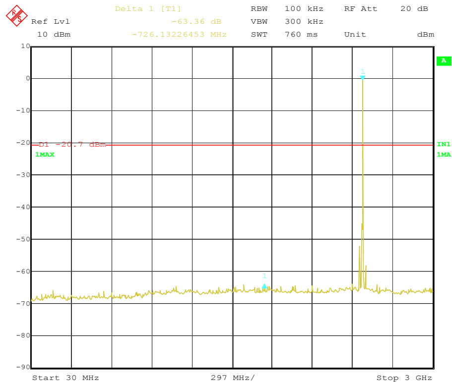
Figure 23 Conducted Spurious emission Plot between 30MHz–3GHz_Higher Ch
