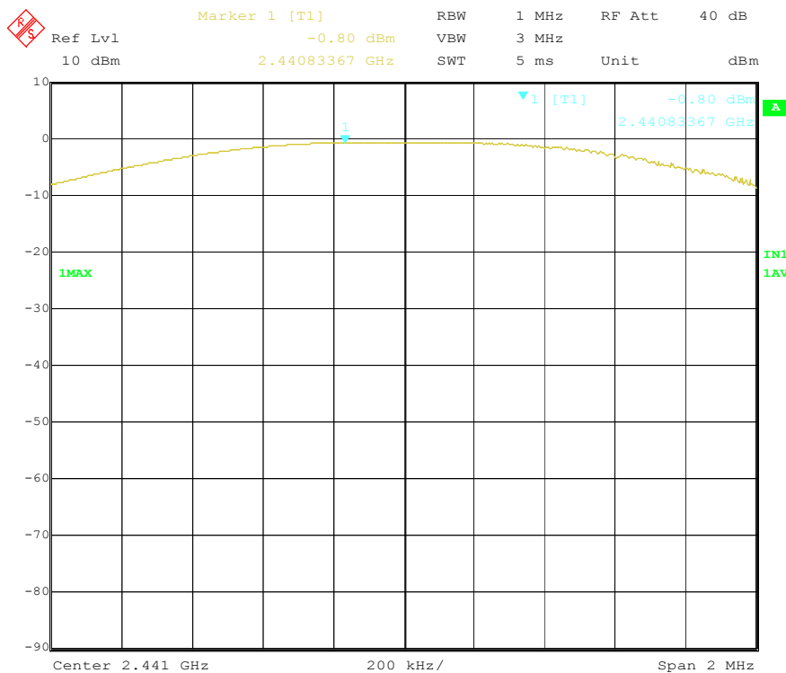
Figure 13 Maximum Peak Output Power(Middle ch_2441.000MHz)
