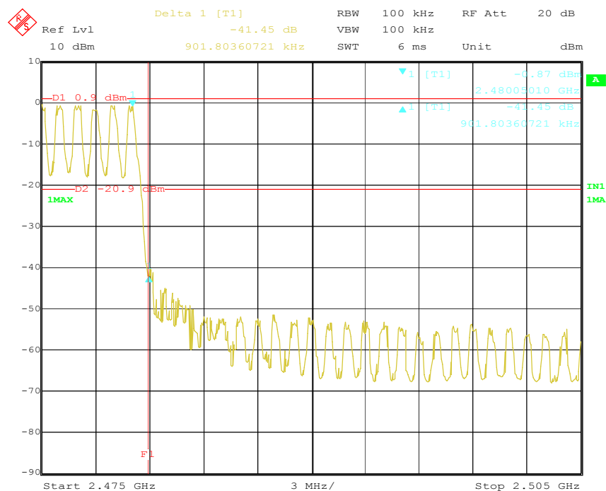
Figure 18 Hopping Band Edge Plot on 2480.000MHz
