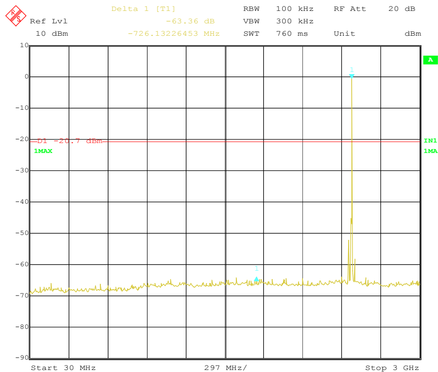
Figure 21 Conducted Spurious emission Plot between 30MHz–3GHz_Middle Ch
