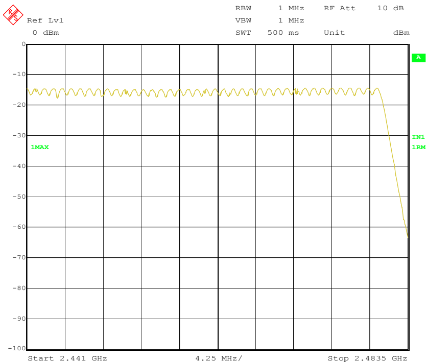
Figure 8 Number of Hopping Channel Plot channel 39-78
