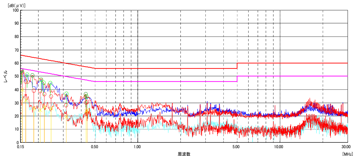
Figure 25 Line Conducted Measurement
