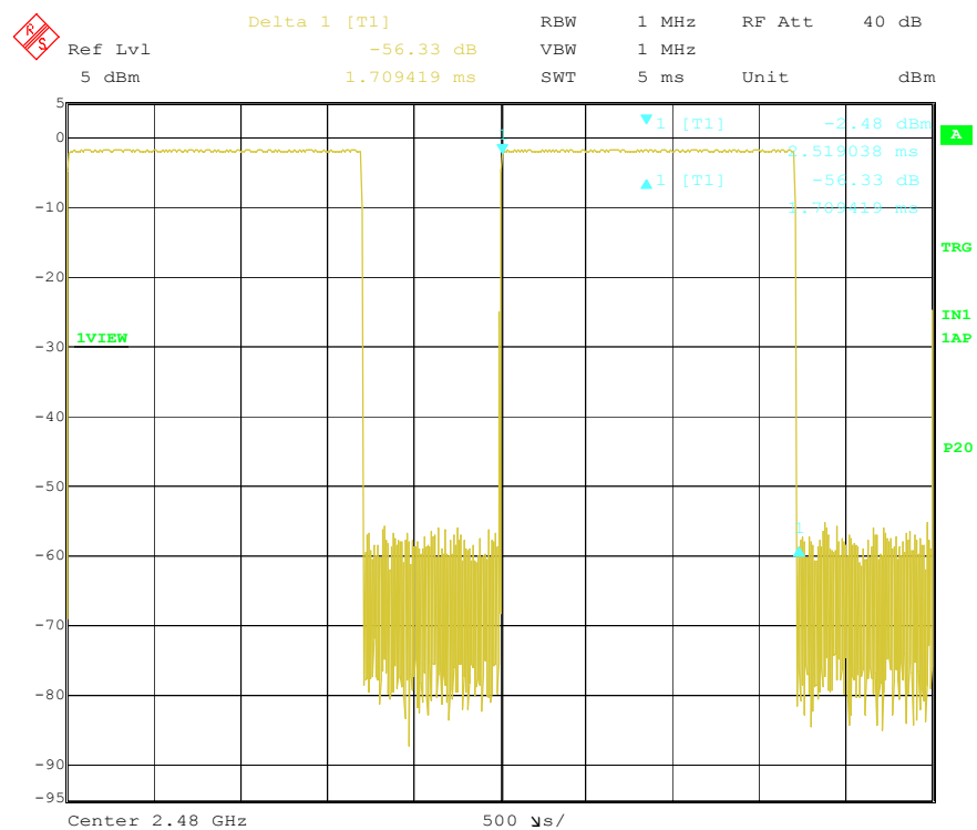
Figure 10 Package Transfer Time Plot_DH3
