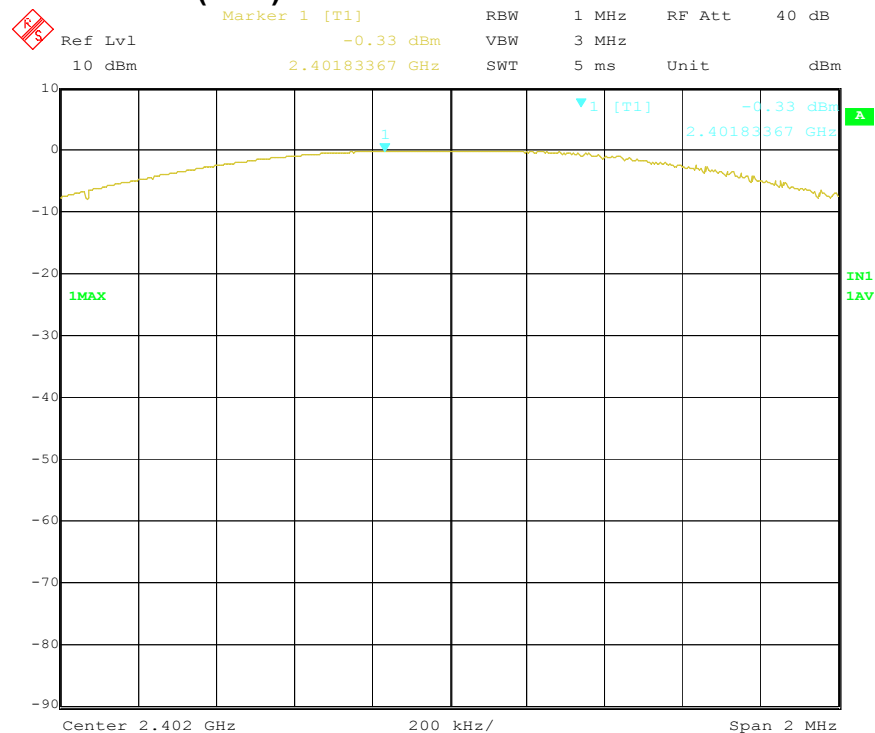
Figure 12 Maximum Peak Output Power(Lower ch_2402.000MHz)
