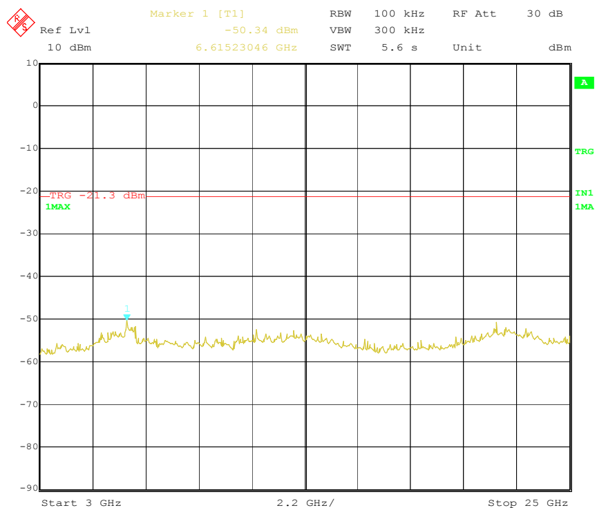
Figure 12 Conducted Spurious emission Plot between 3GHz–25GHz_Middle Ch
