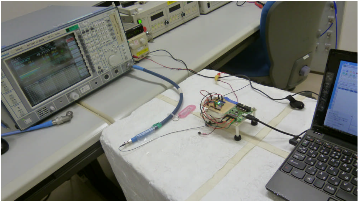
Photo6 Test setup for conducted
