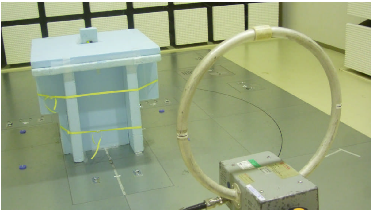
Photo3 Test setup for radiated (9kHz-30MHz)
