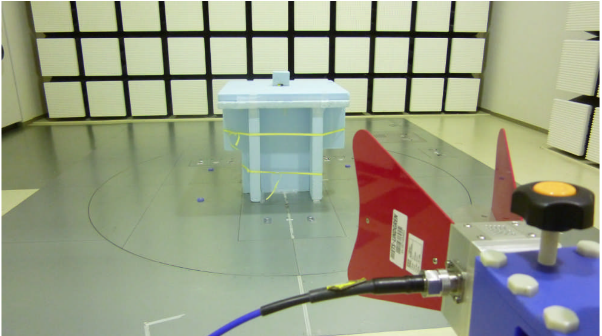
Photo2 Test setup for radiated (above 1GHz)
