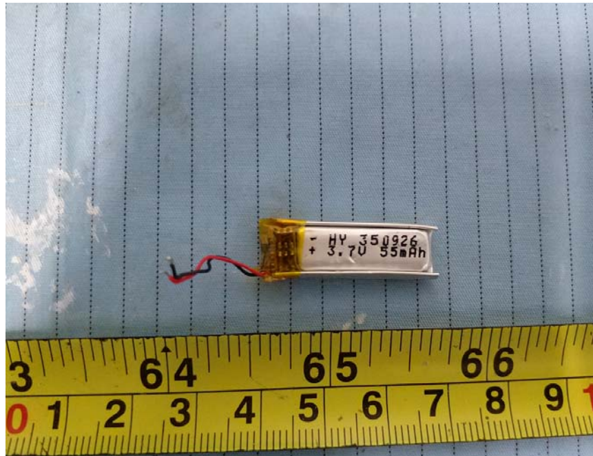
EUT – Battery Top View
