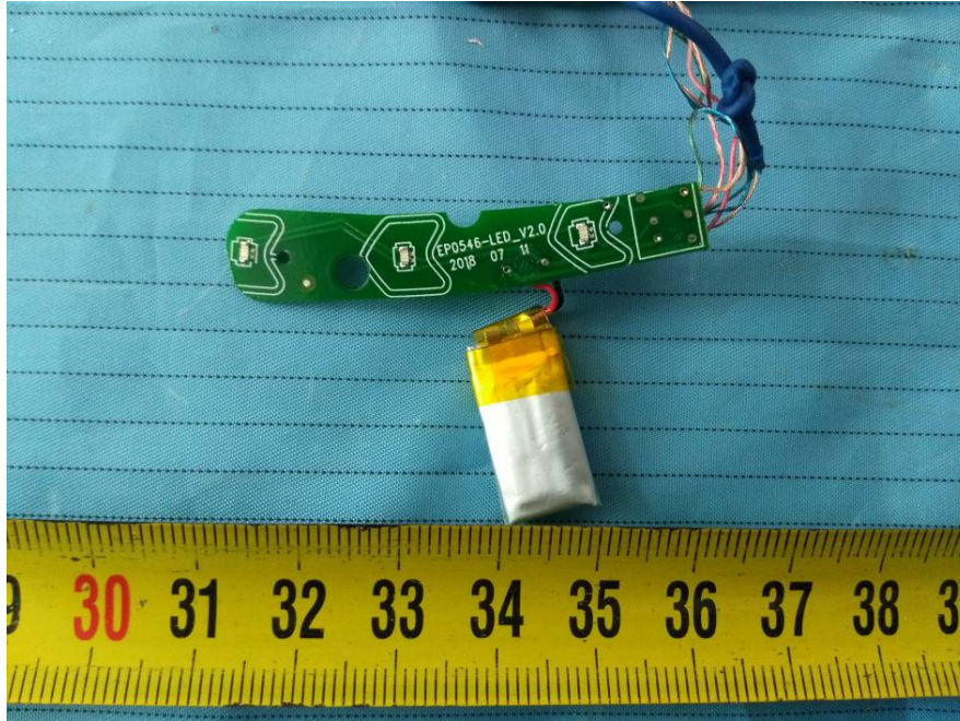
EUT – LED Board& Battery Front View
