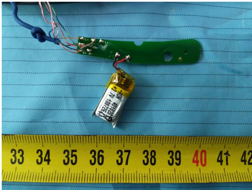
EUT – LED Board& Battery Rear View
