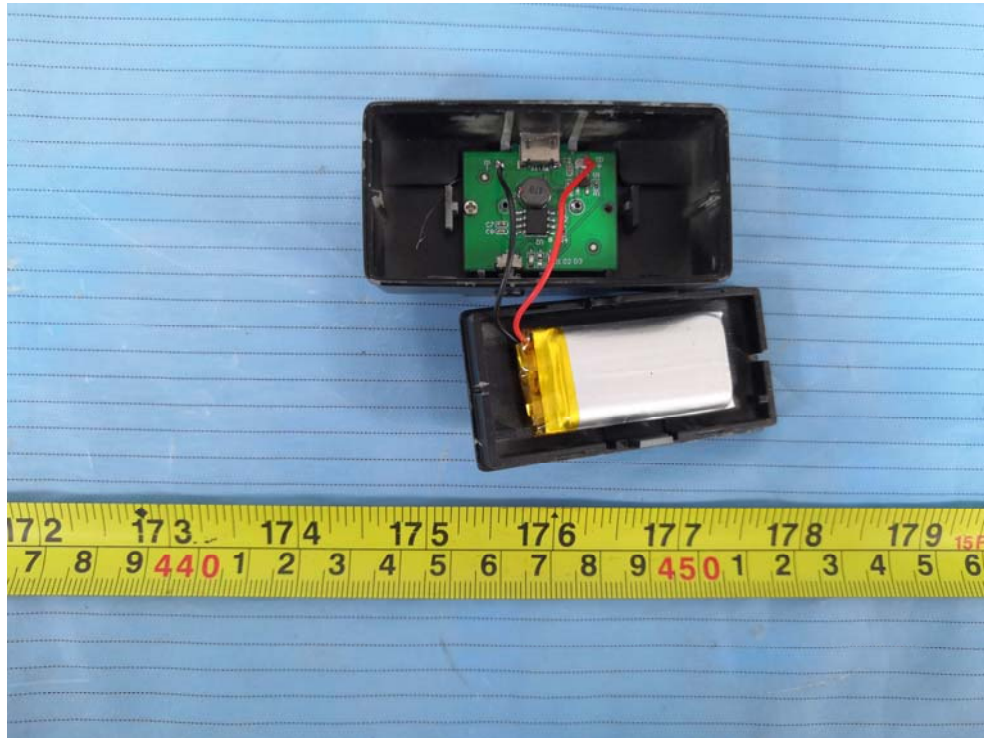
Charging box
