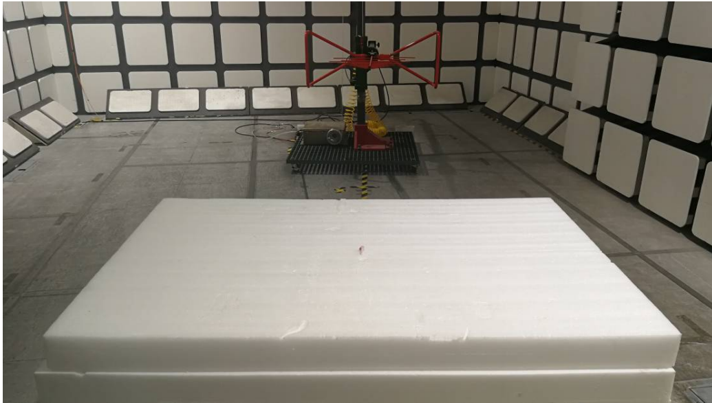
Radiated Spurious Emissions View (Below 1 GHz)
