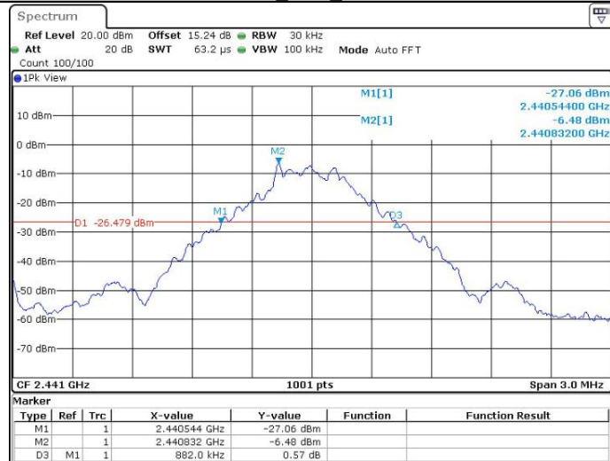
DH1_Ant1_2441
