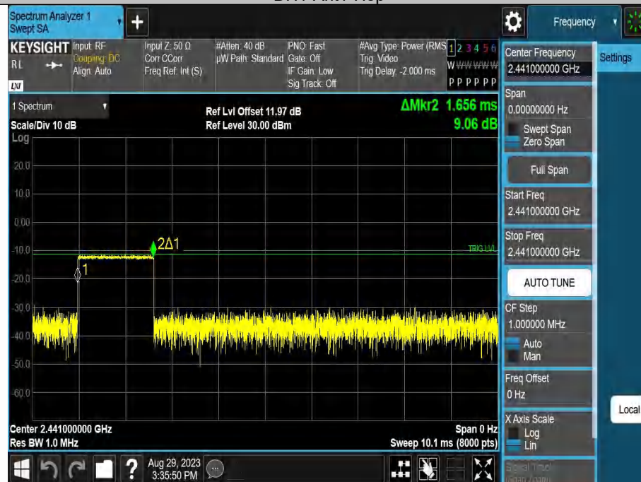
DH3-Ant1-Hop
