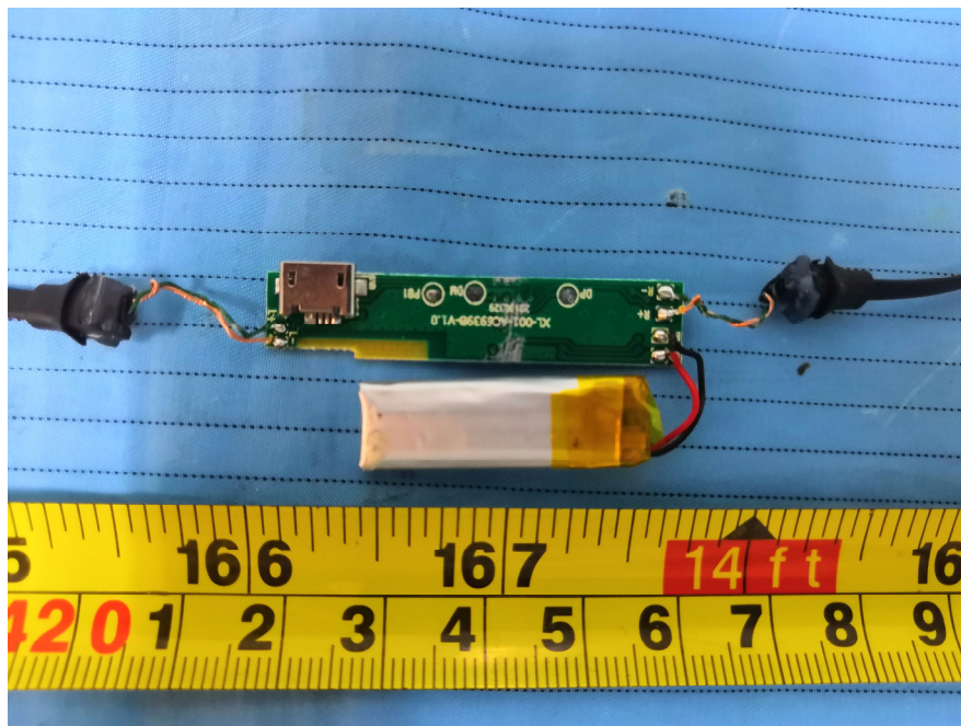
EUT – Main Board and Battery Bottom View
