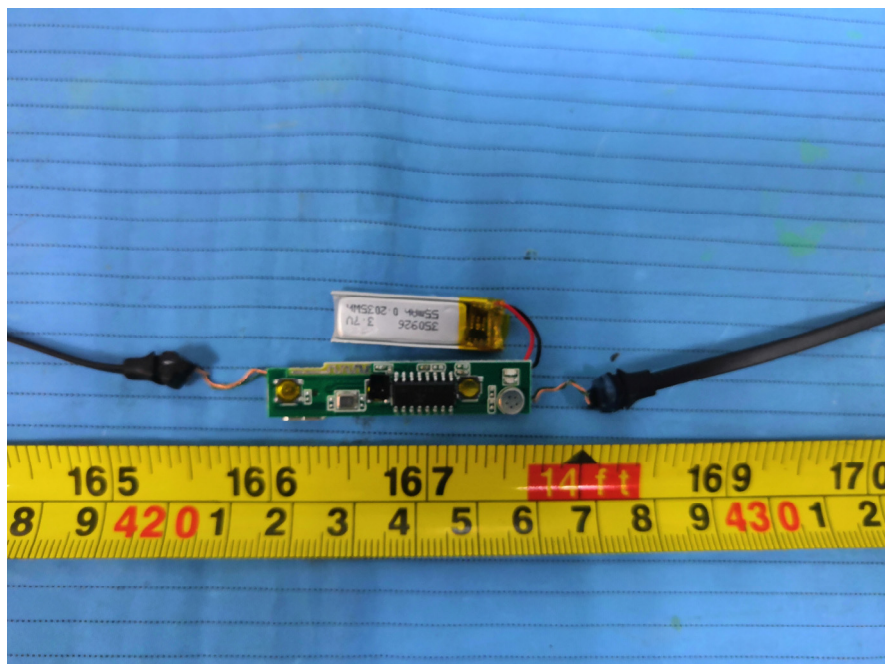
EUT – Main Board and Battery Top View
